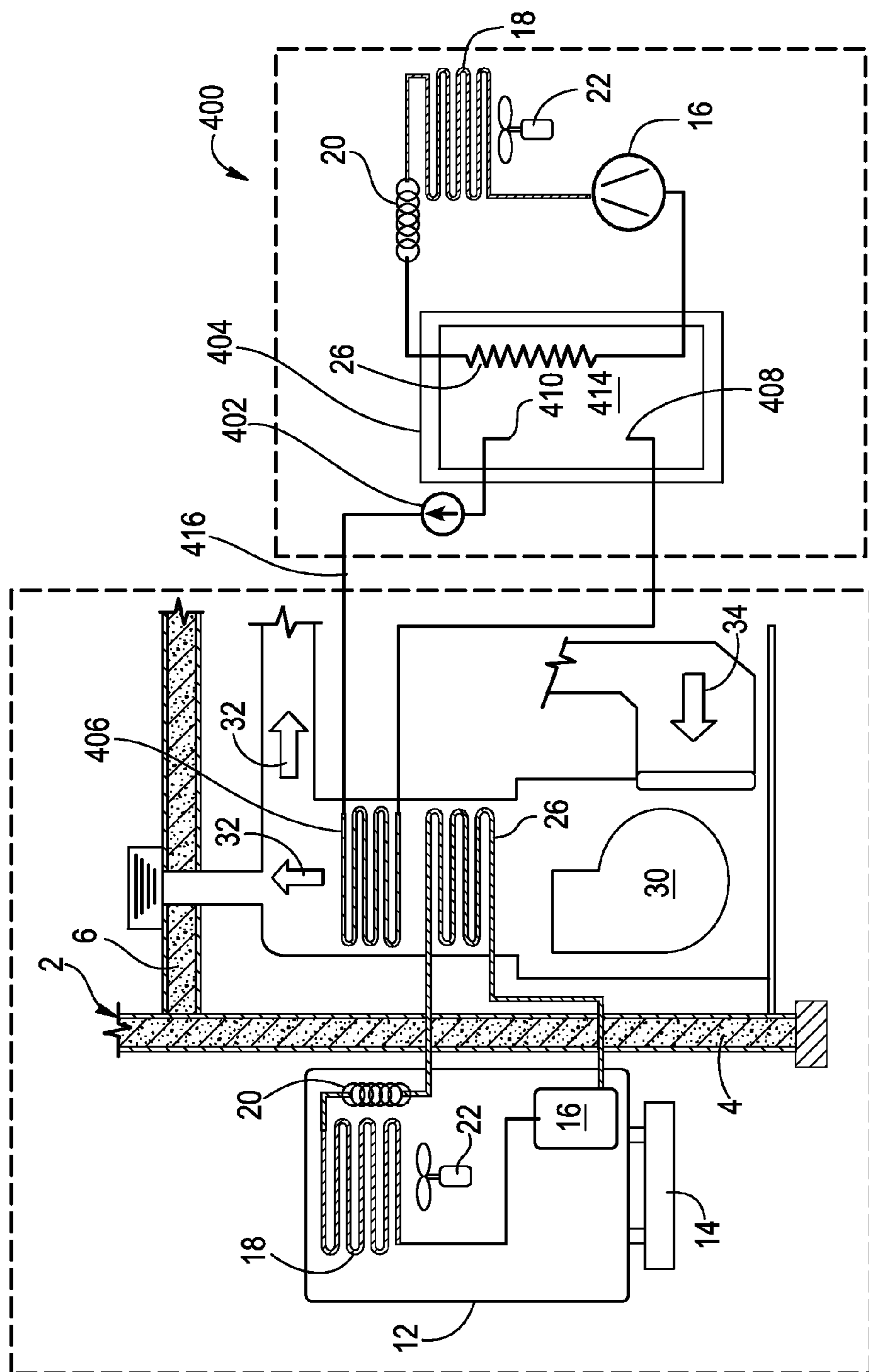
RESIDENTIAL HVAC THERMAL STORAGE SYSTEM
