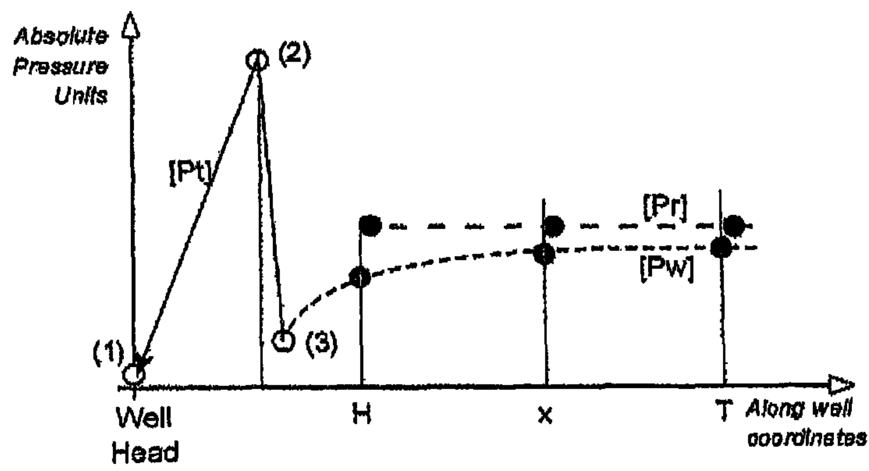
Figure 11
