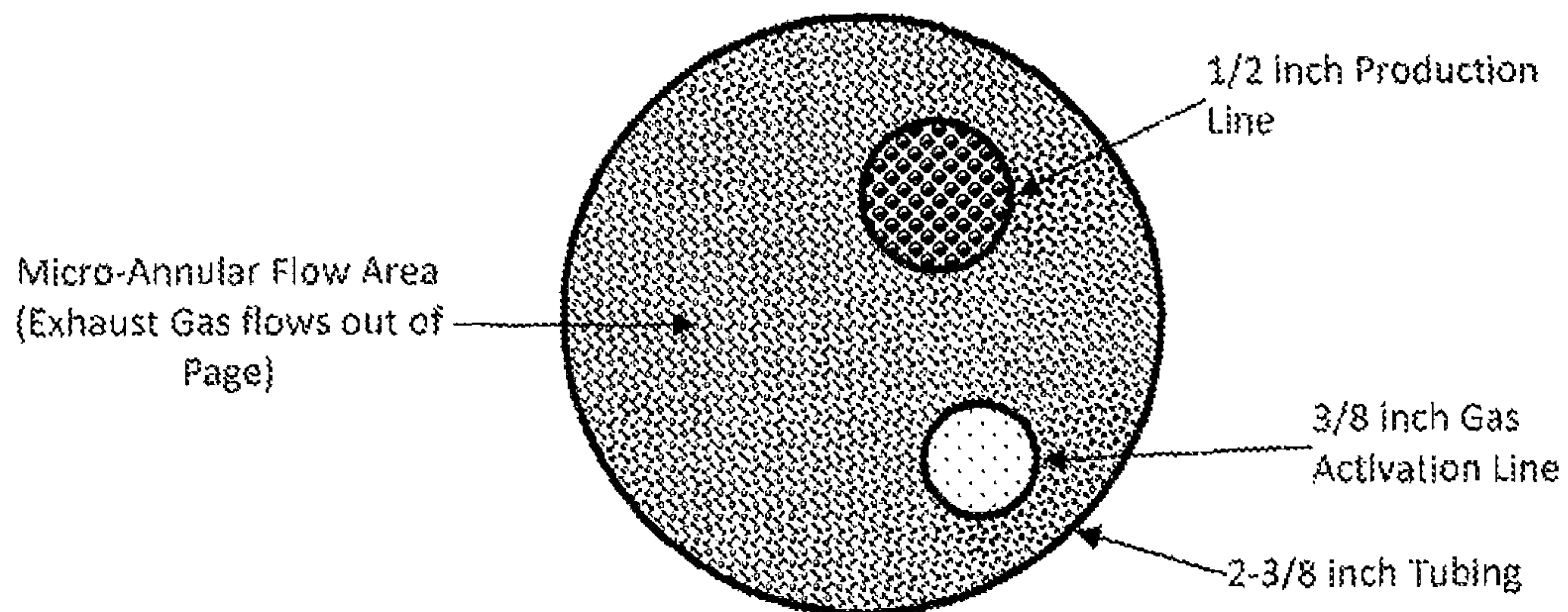
Figure 32
