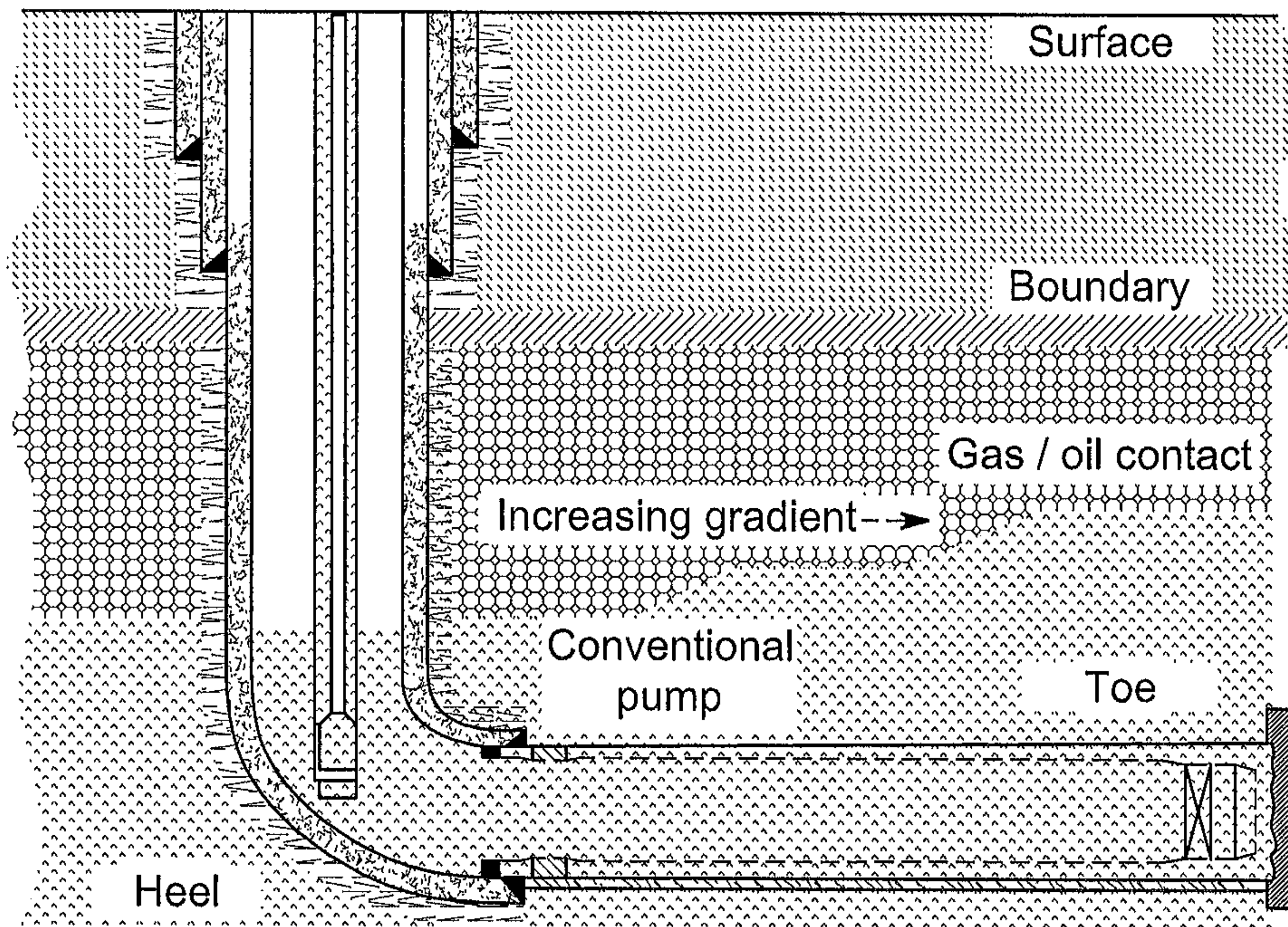
FIG. 2 PRIOR ART
