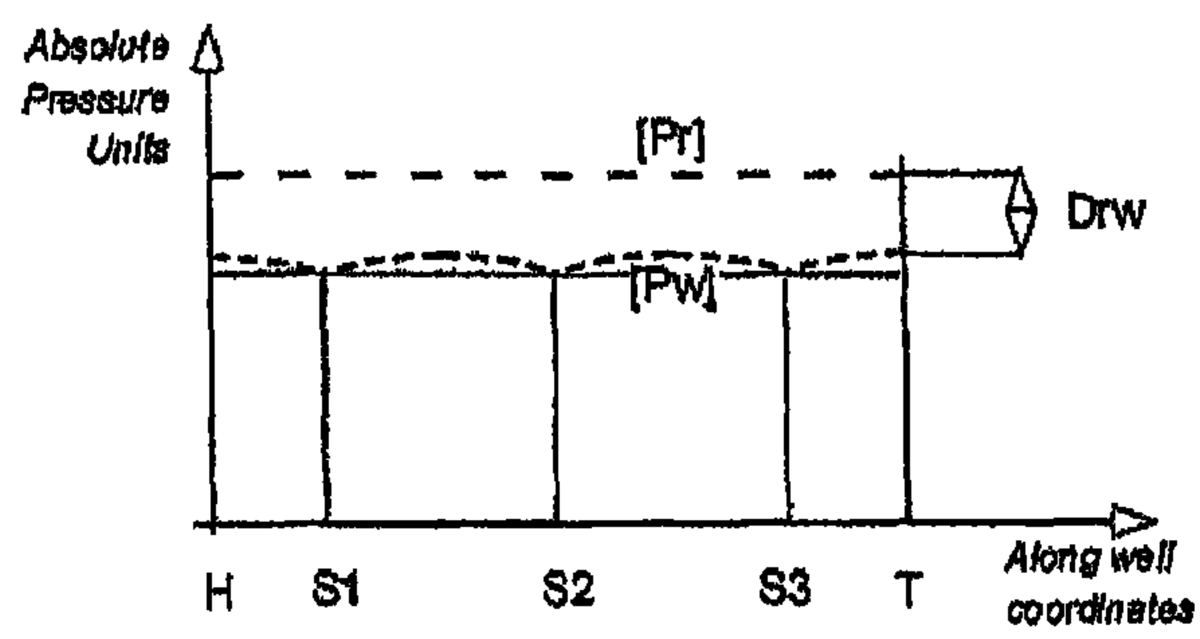
Figure 10
