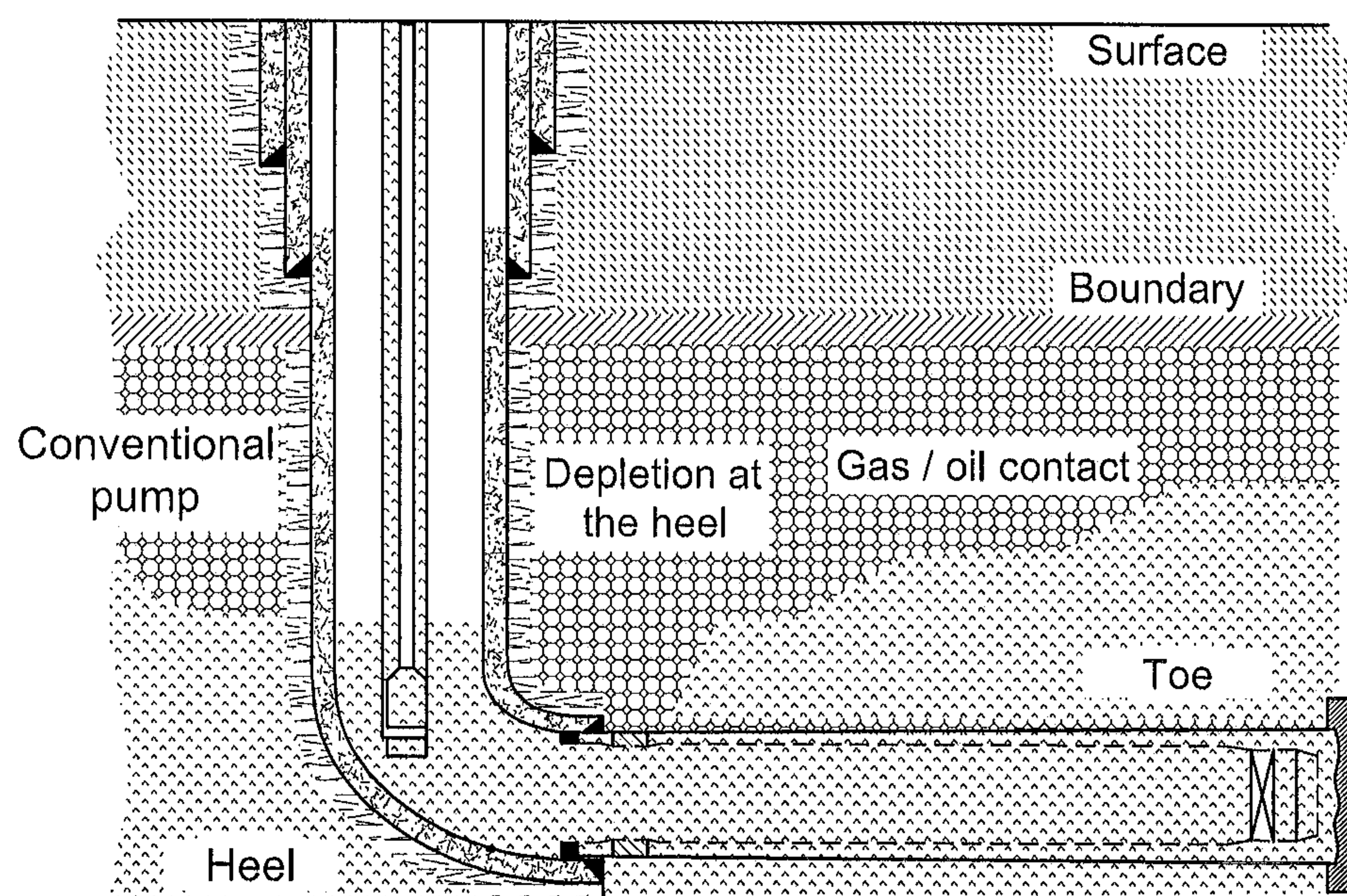
FIG. 3 PRIOR ART
