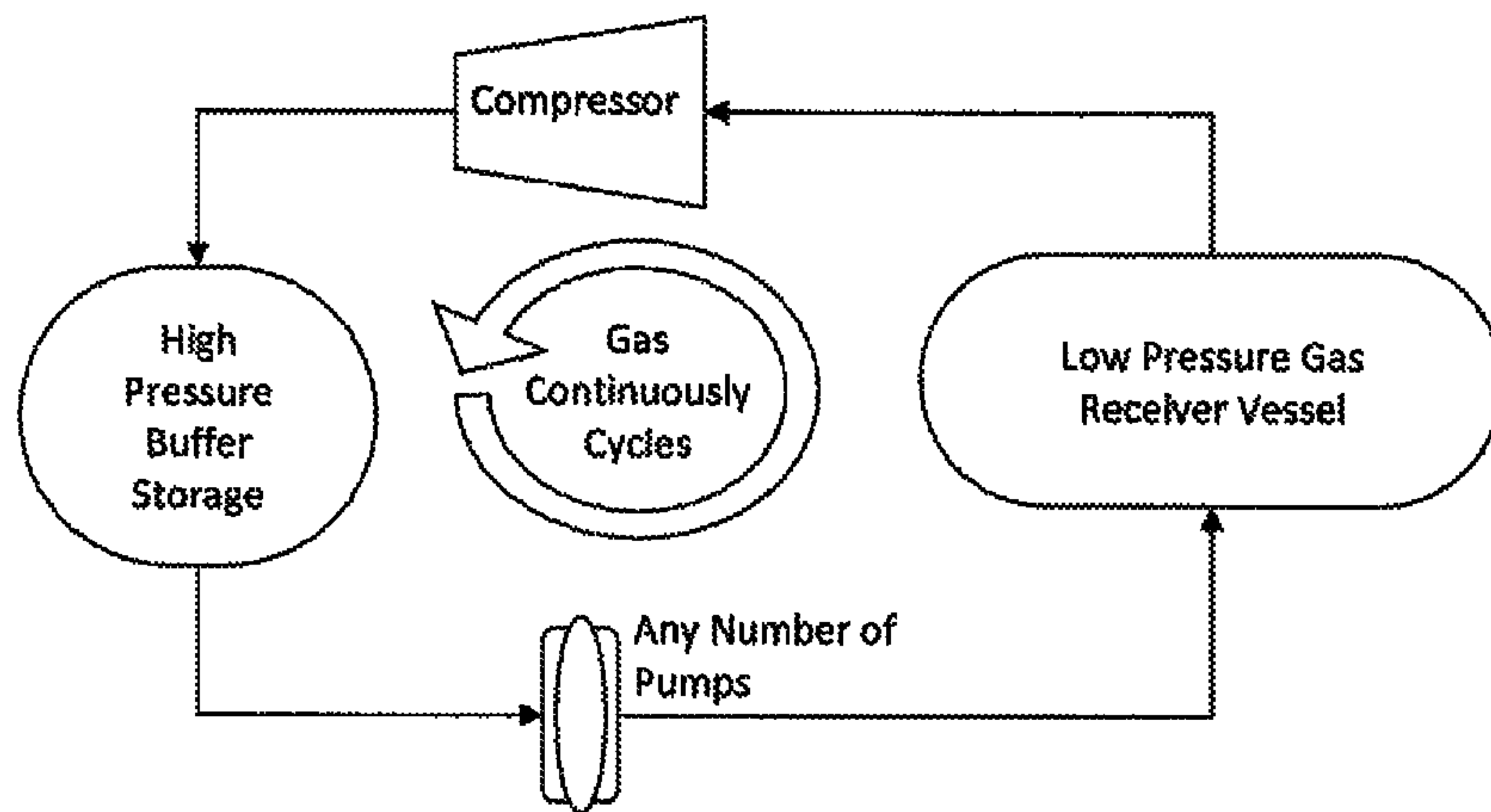
Figure 30
