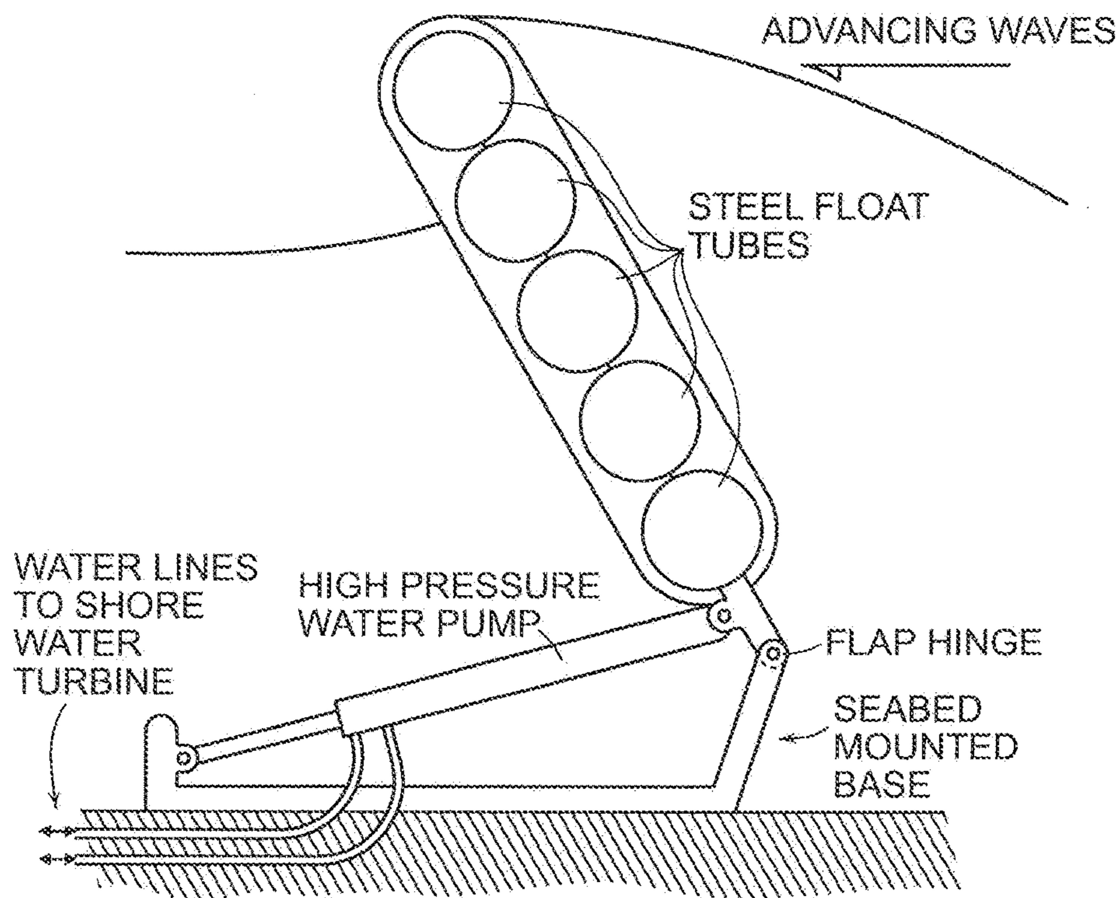
Aquamarine "Oyster" (Related Art)
