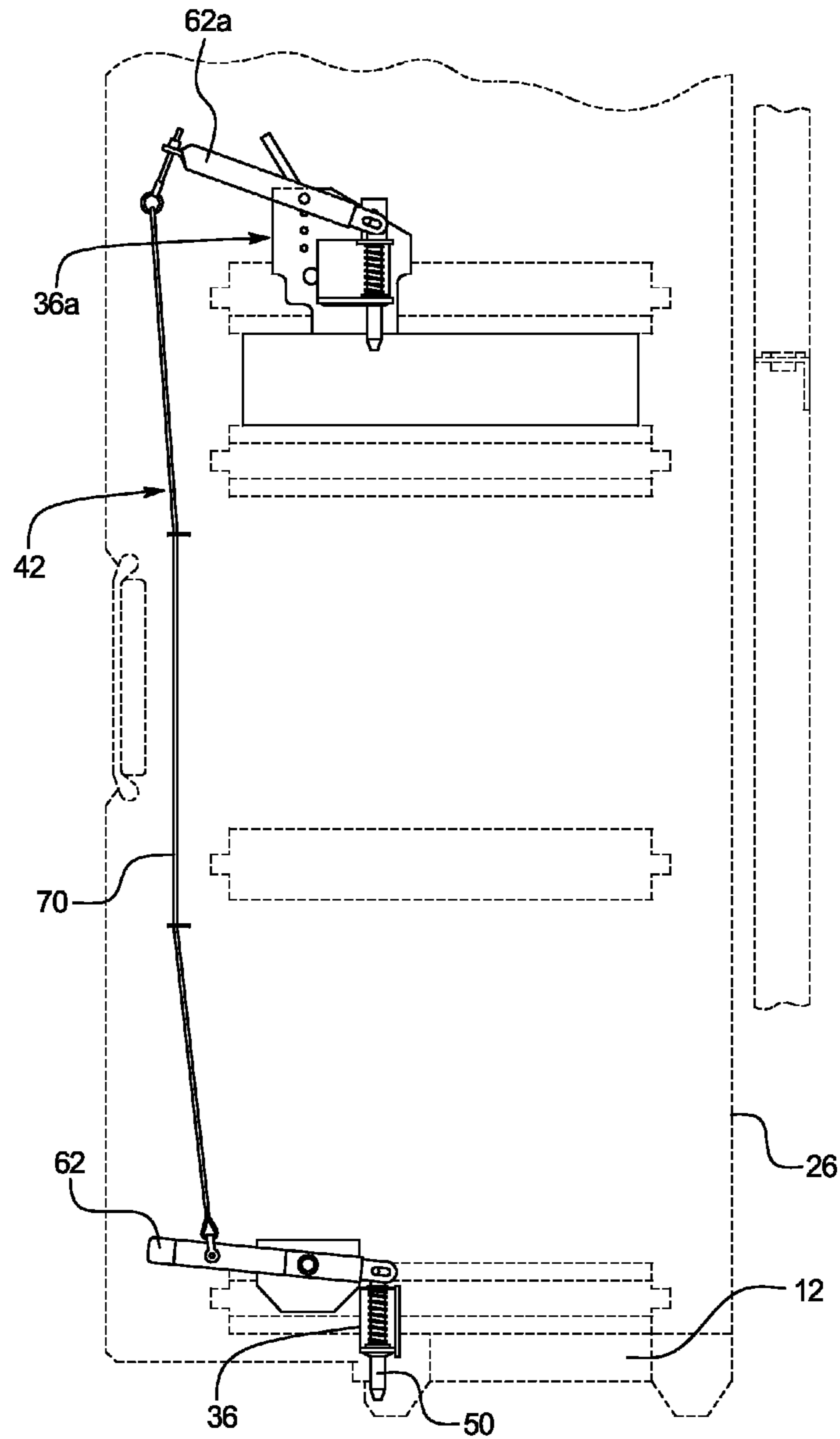
FIG. 6 PRIOR ART
