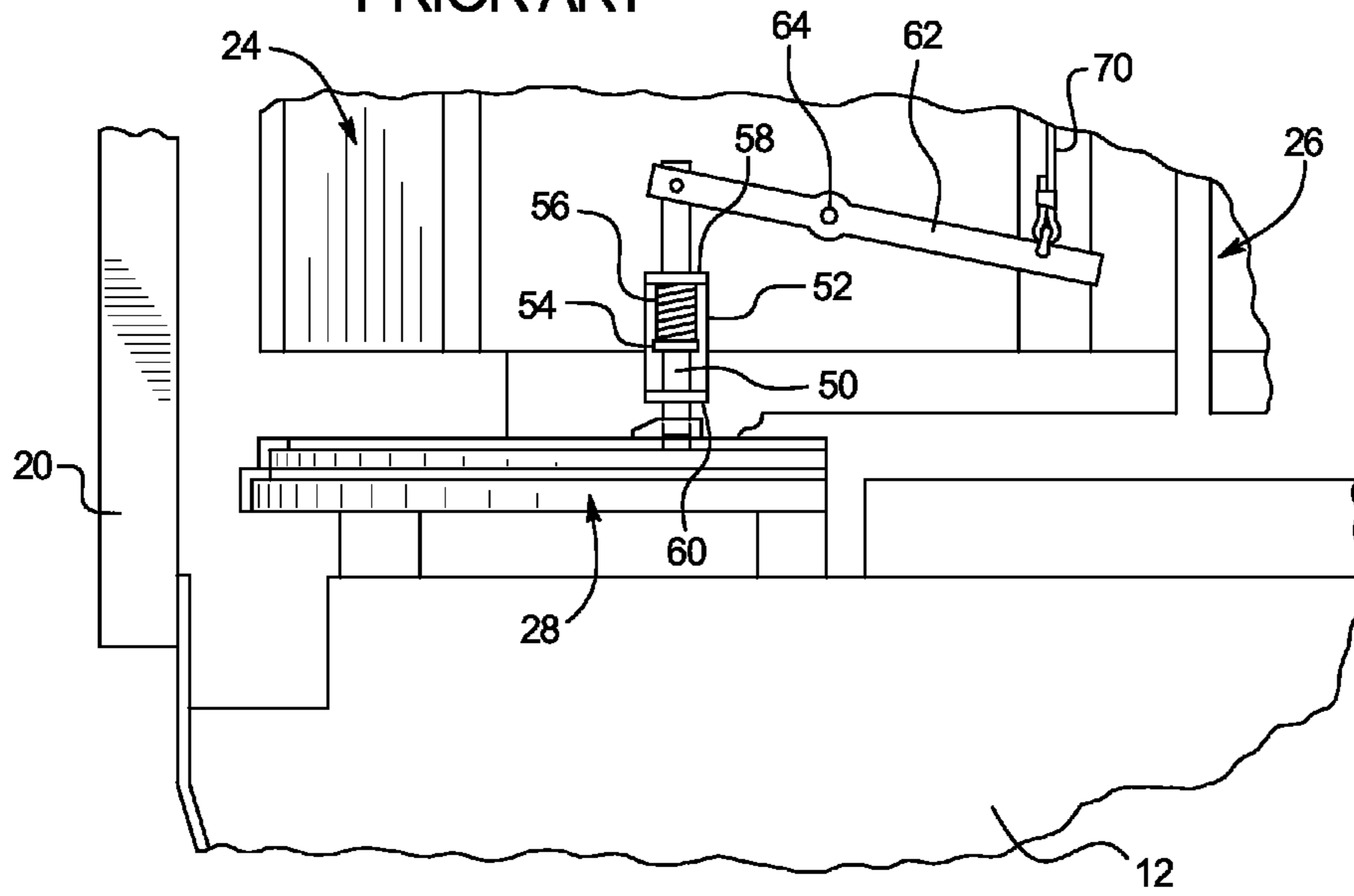
FIG. 4 PRIOR ART
