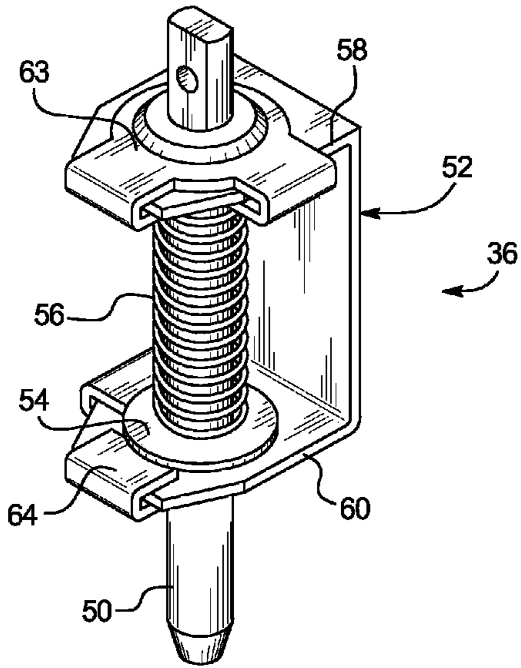
FIG. 7 PRIOR ART
