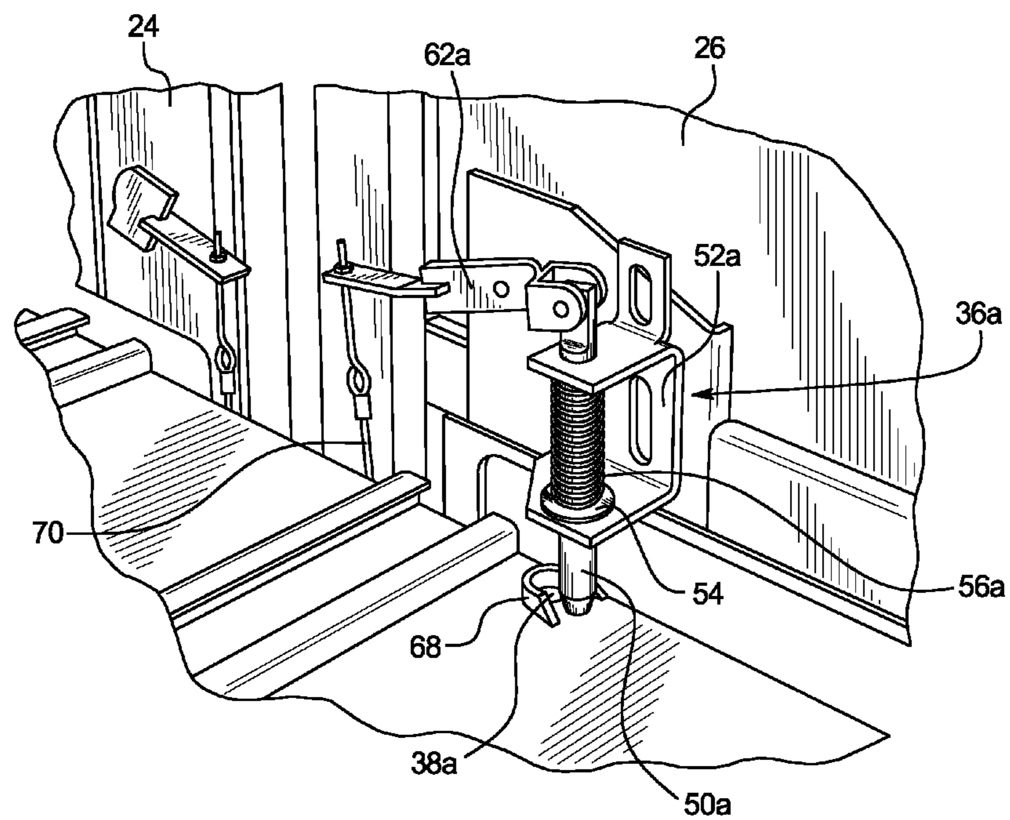
FIG. 5 PRIOR ART
