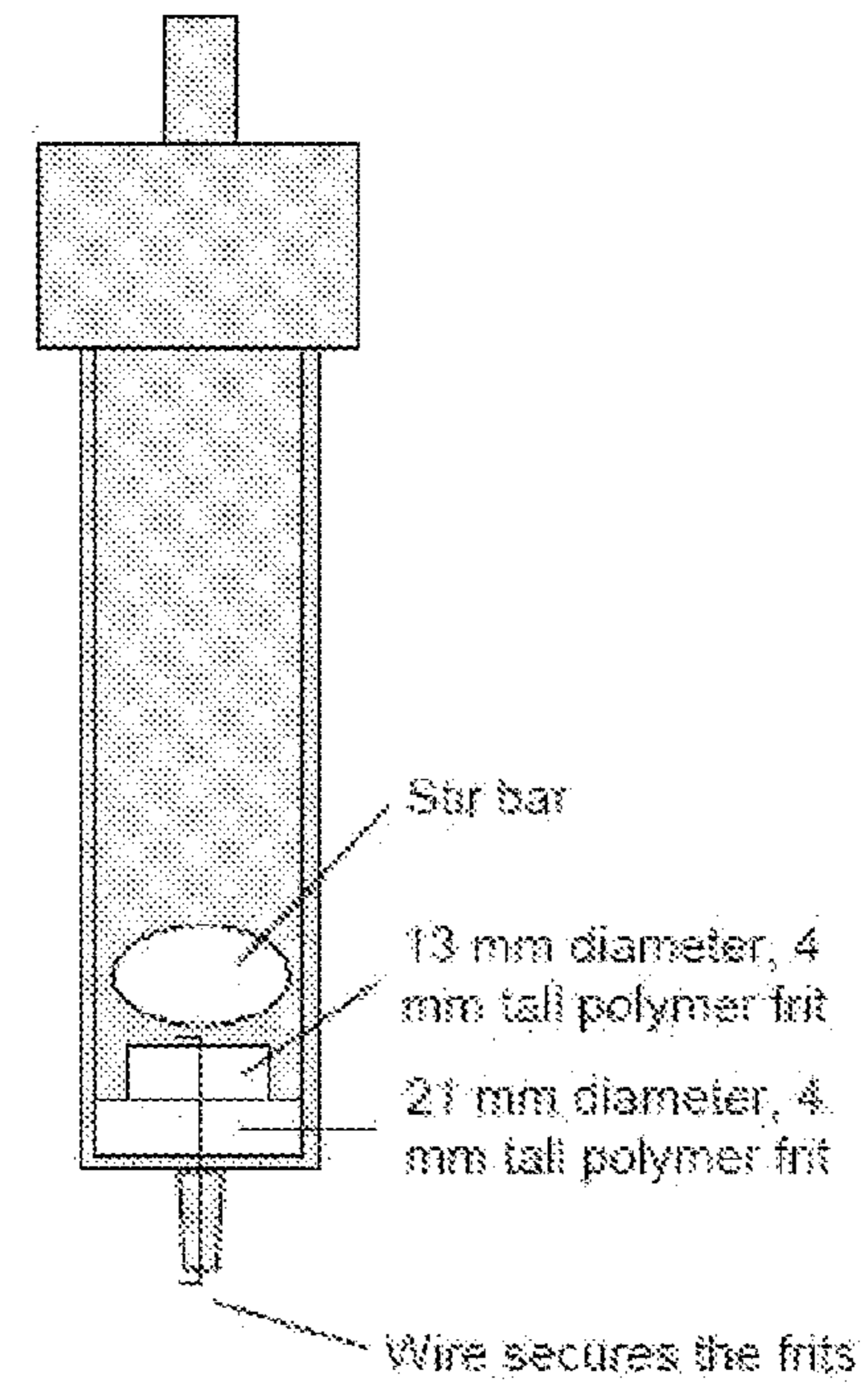
Reaction Tube
