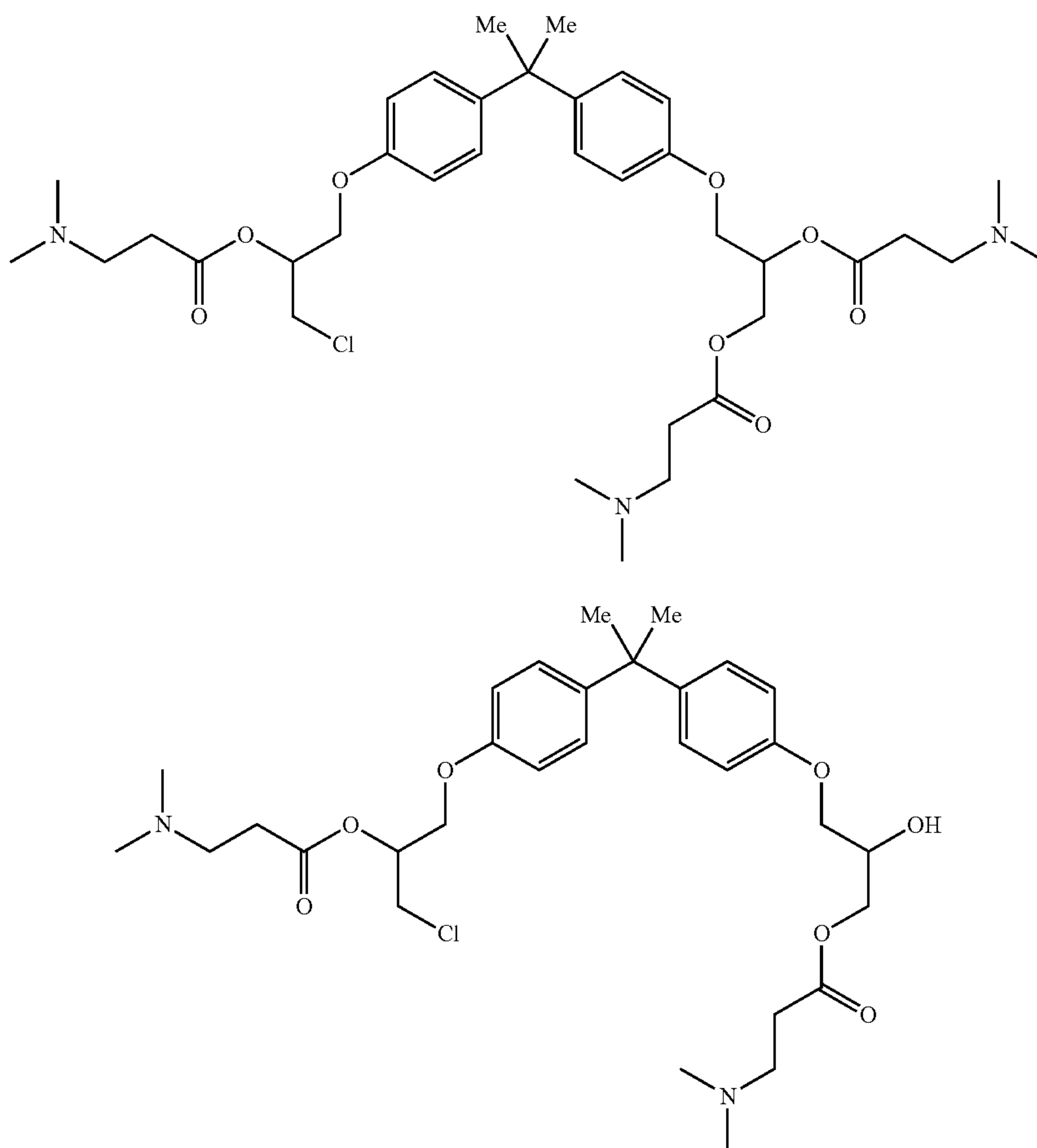
Tri-Gly-BADGE x HCL x H 2 O
