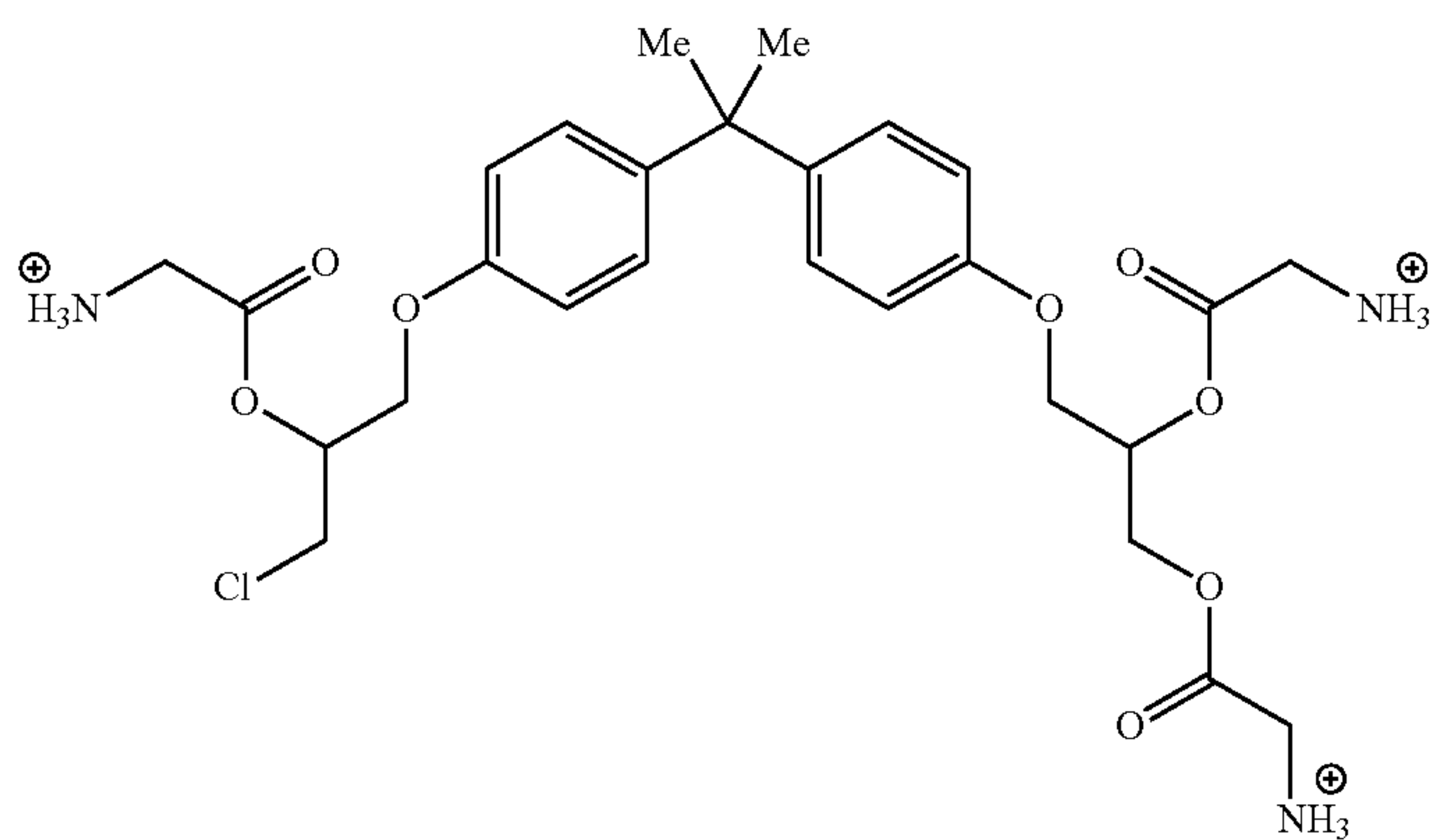
Tri-Gly-BADGE x HCL x H 2 O
