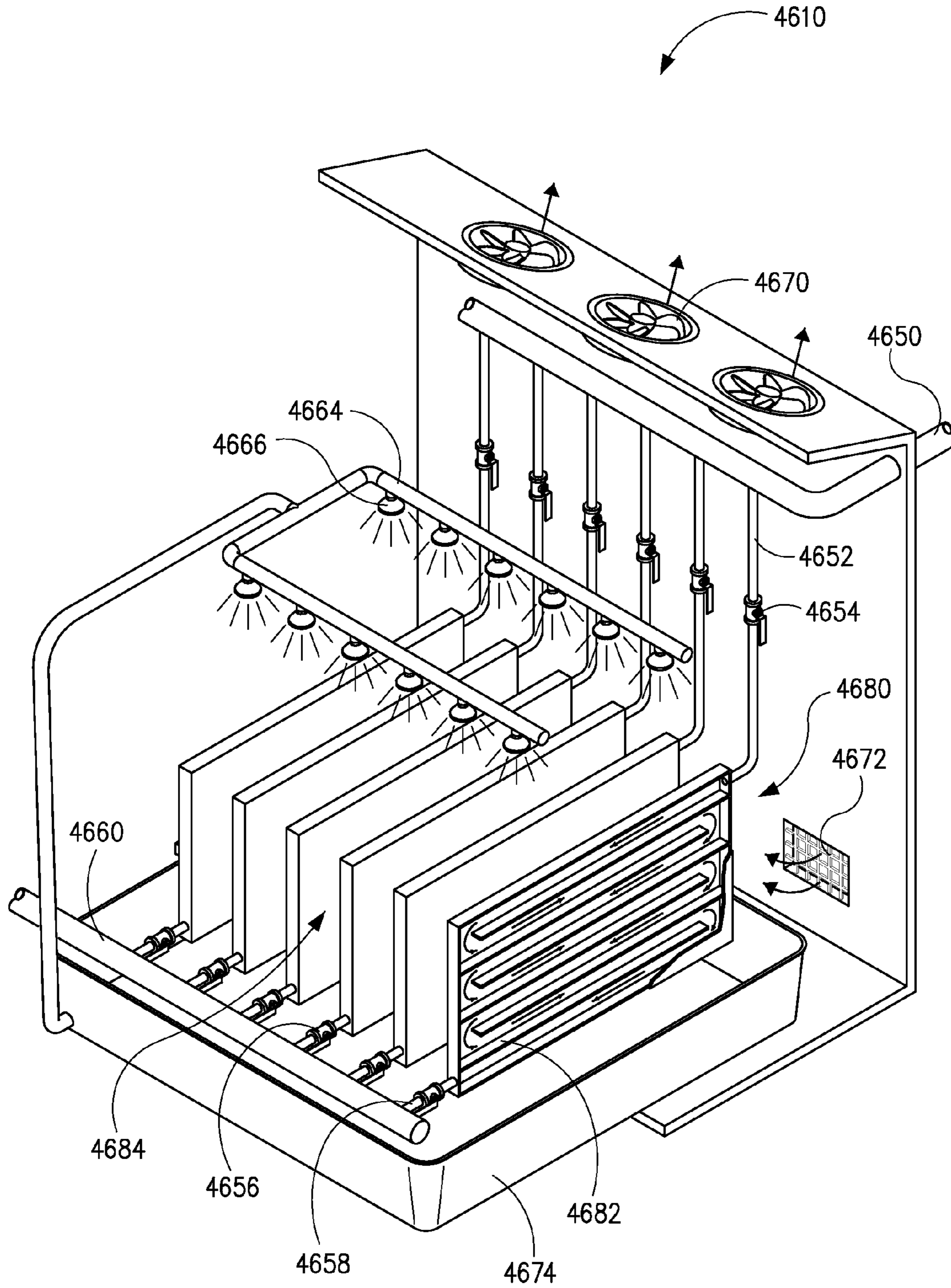
FIGURE 20
