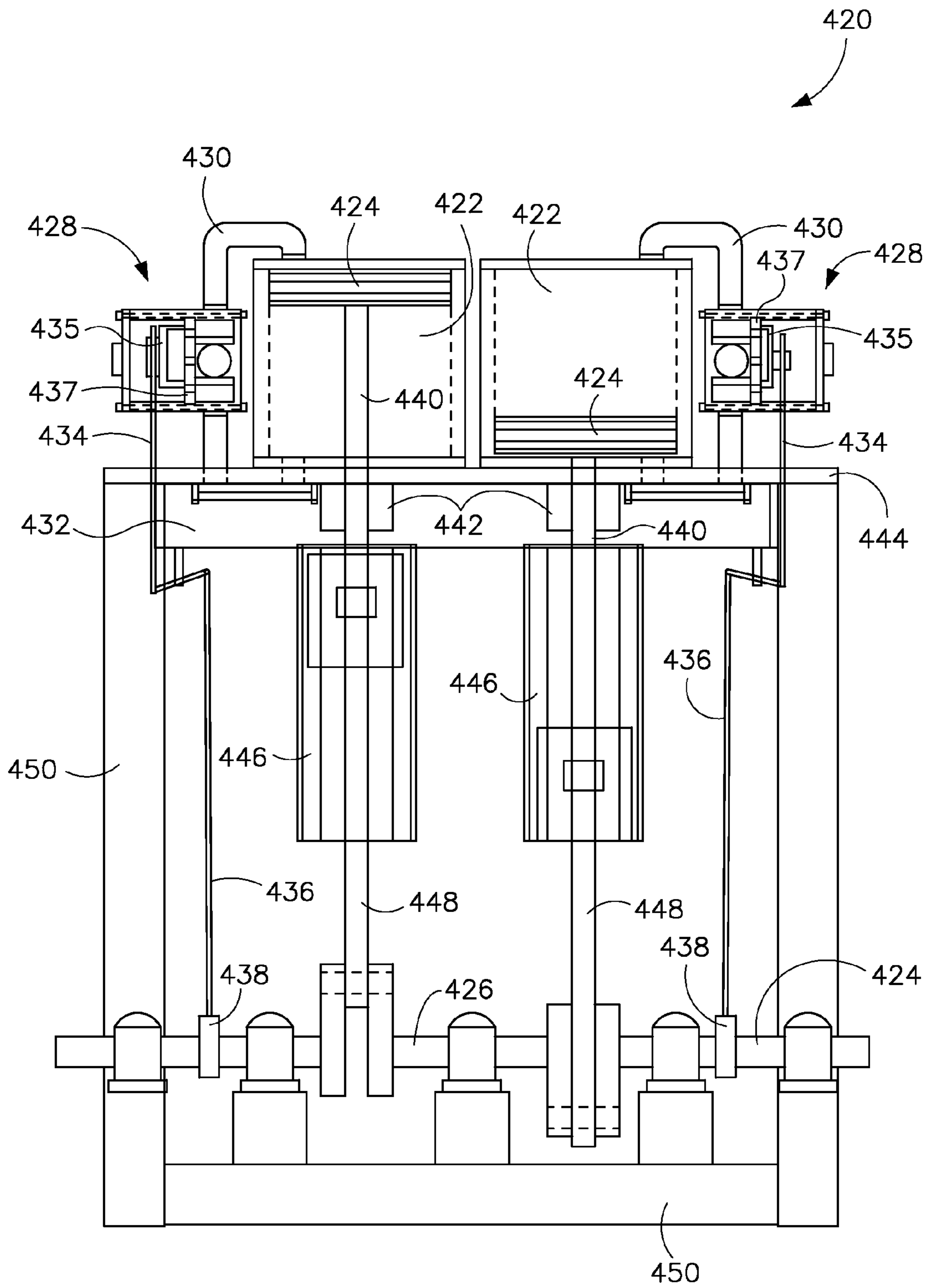
FIGURE 4B
