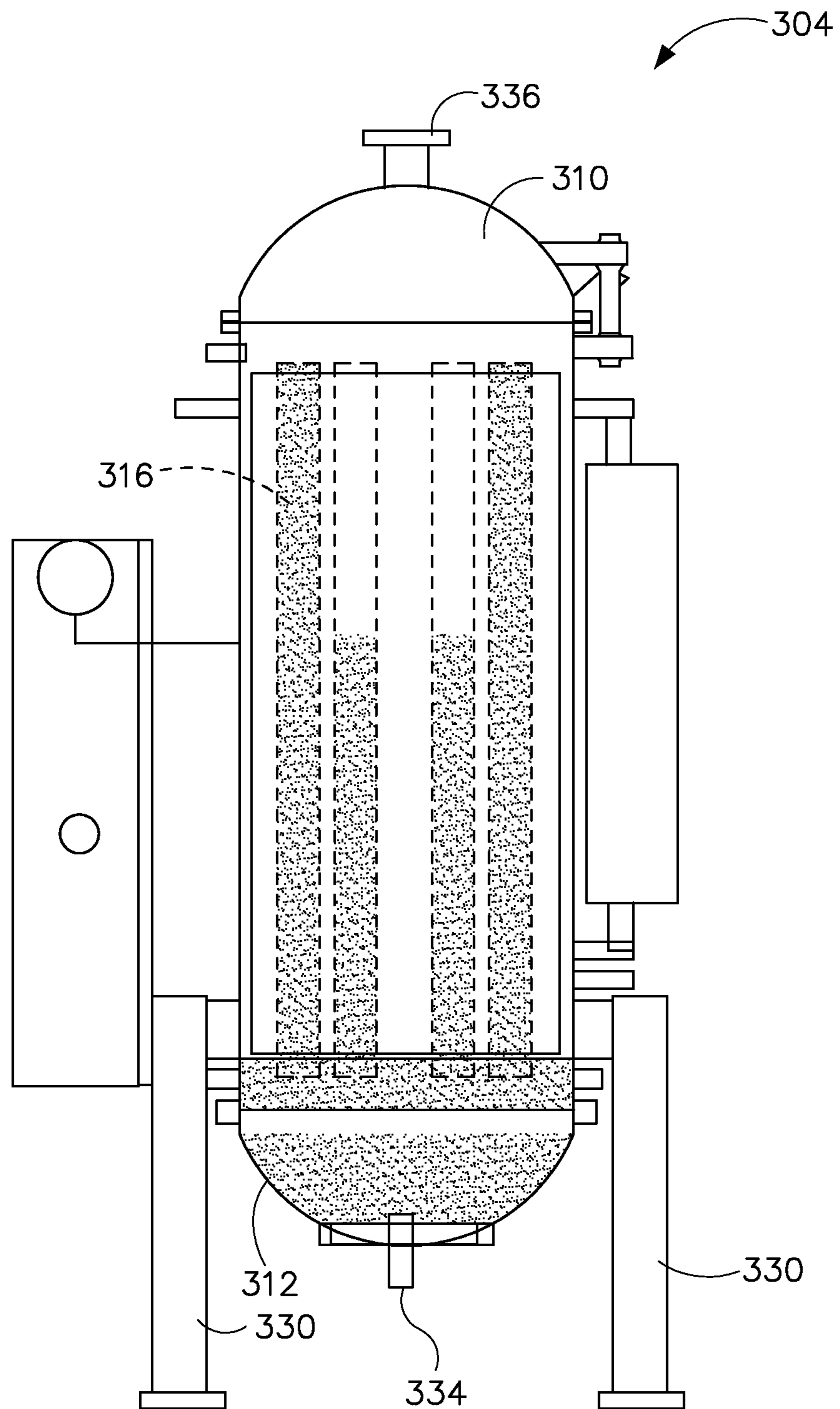
FIGURE 3
