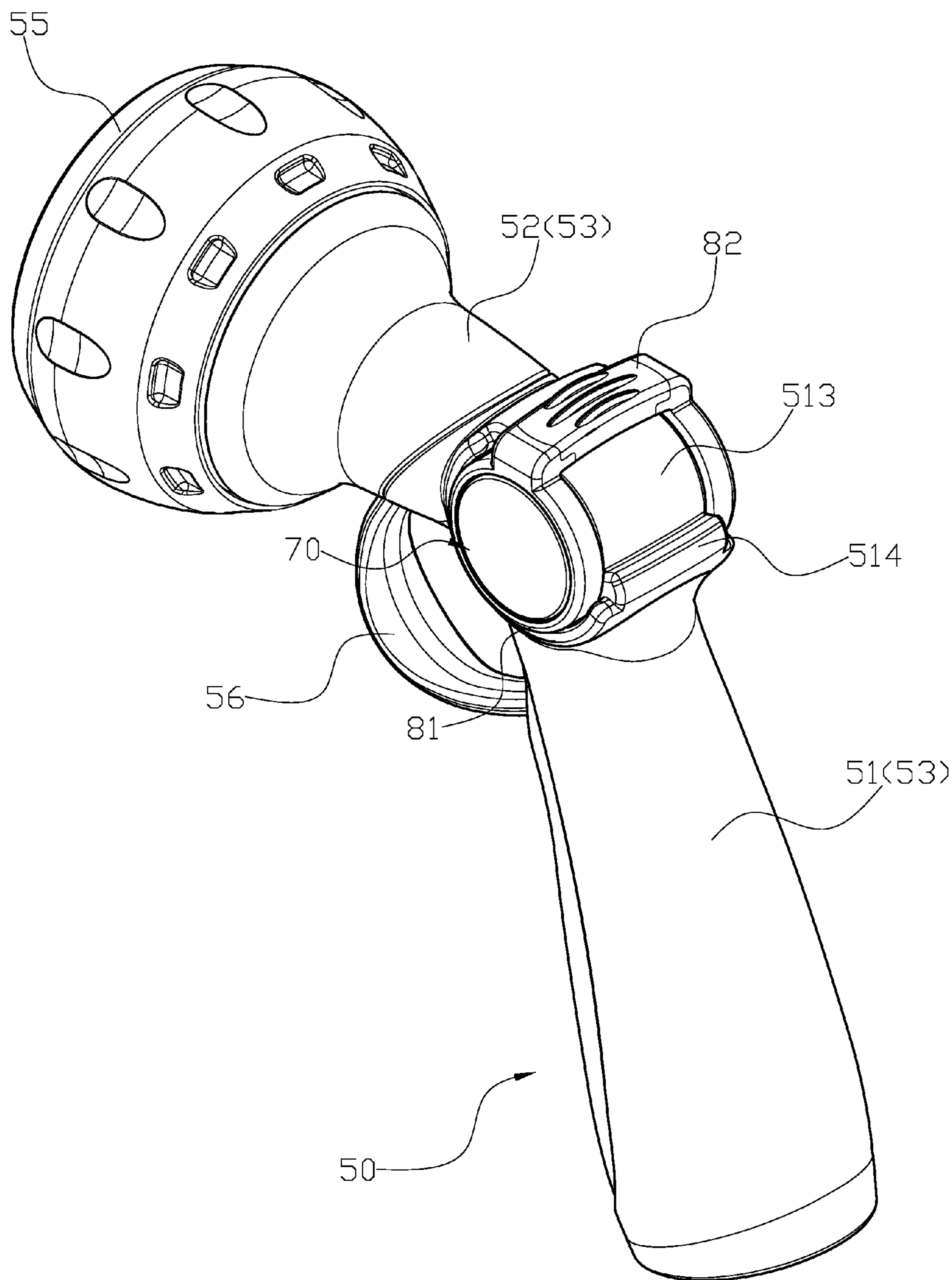
FIG. 7 PRIOR ART
