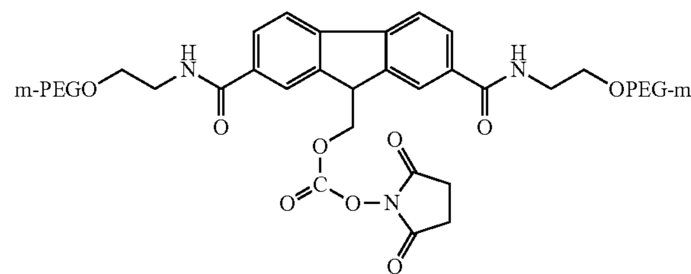
mPEG 2 -C 2 -fomc-20K-N-Hydroxysuccinimide Derivative, 20 kDa, ("mPEG 2 -C 2 -fmoc-20K- NHS")
