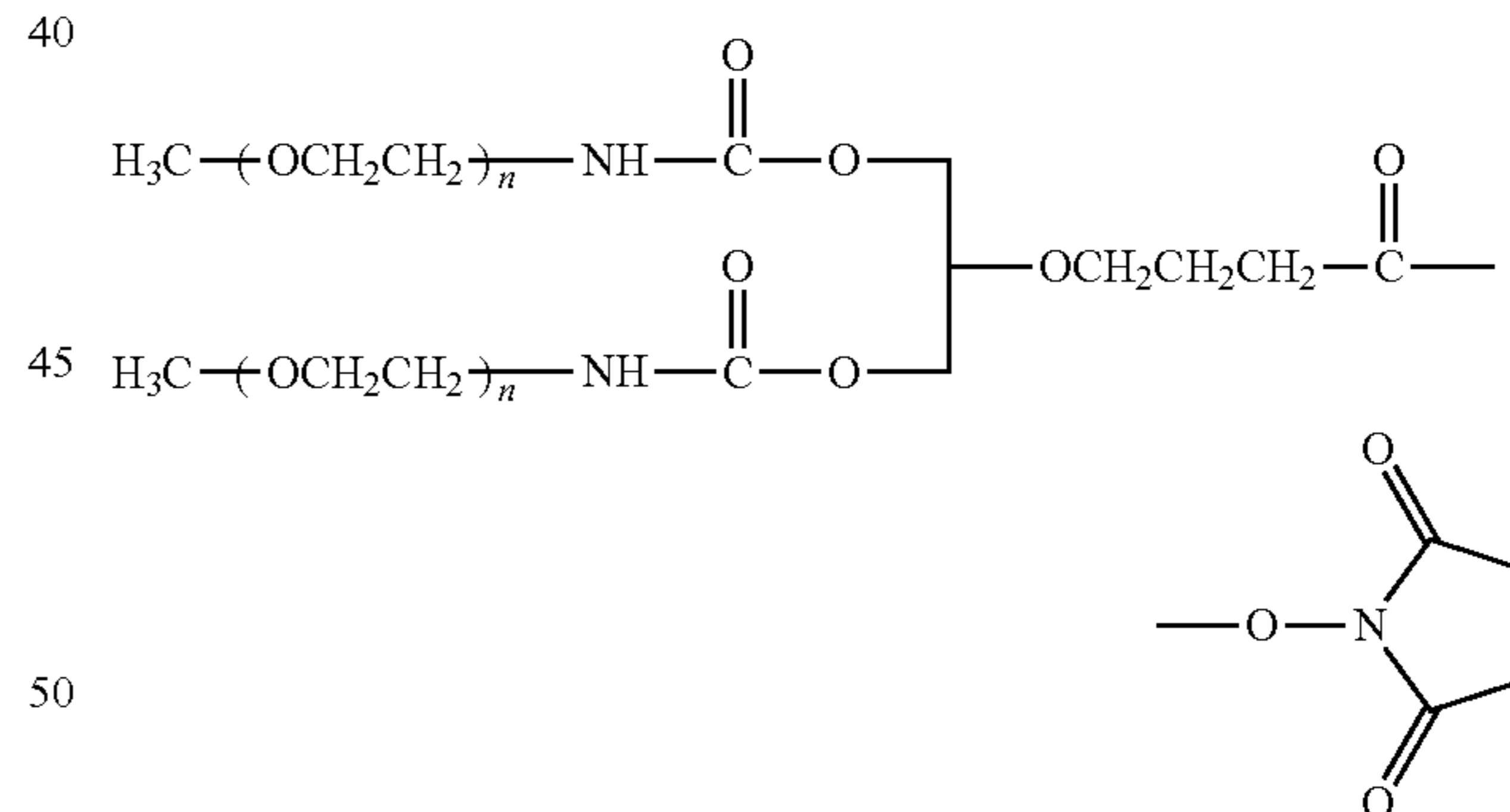
mPEG2-ru-20K-N-Hydroxysuccinimidyl Derivative, 20 kDa, ("mPEG2-ru-20K-NHS")
