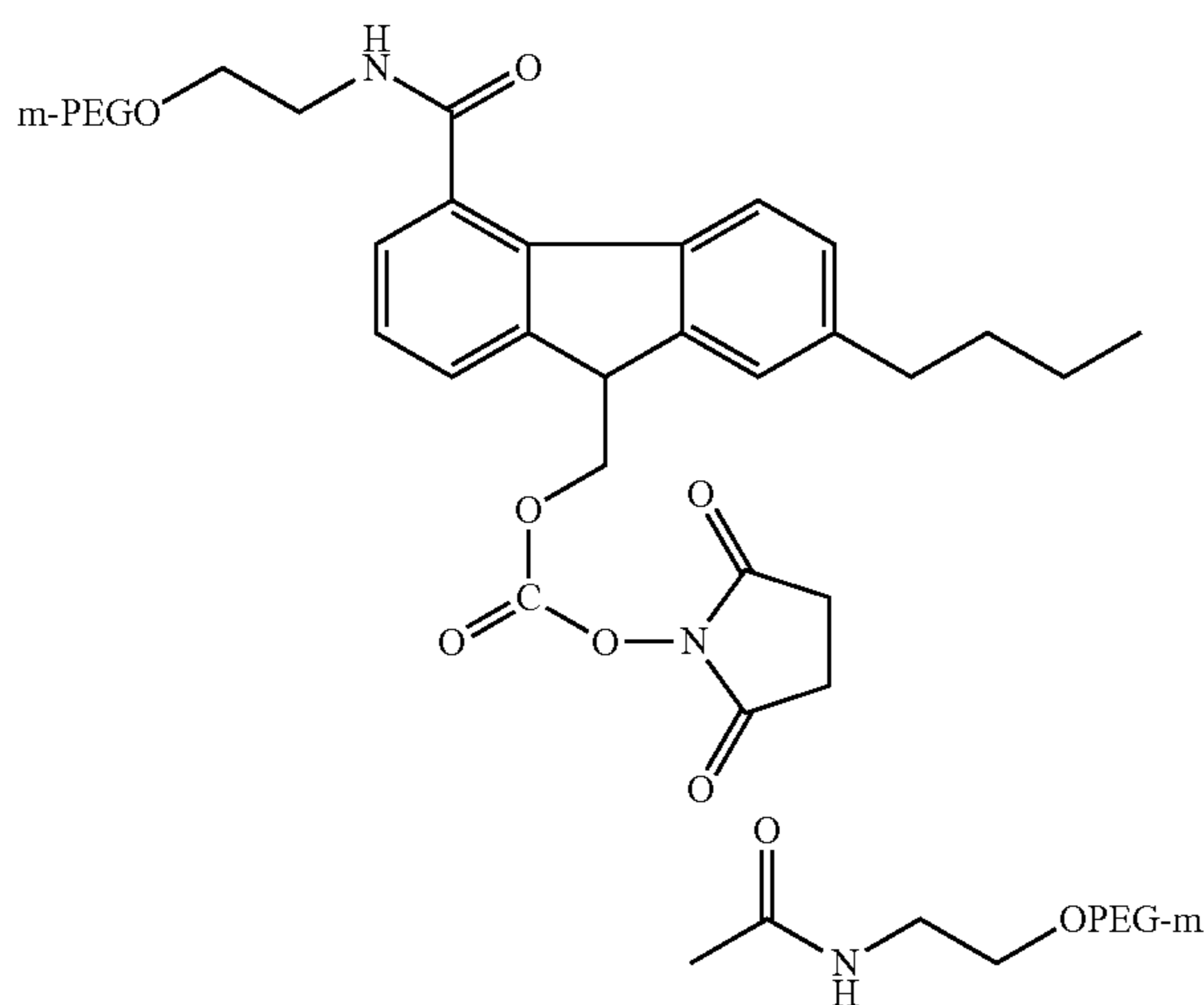
mPEG2-CAC-fmoc-20K-N-Hydroxysuccinimide Derivative, 20 kDa, ("mPEG2-CAC-fmoc-20K- NHS")
