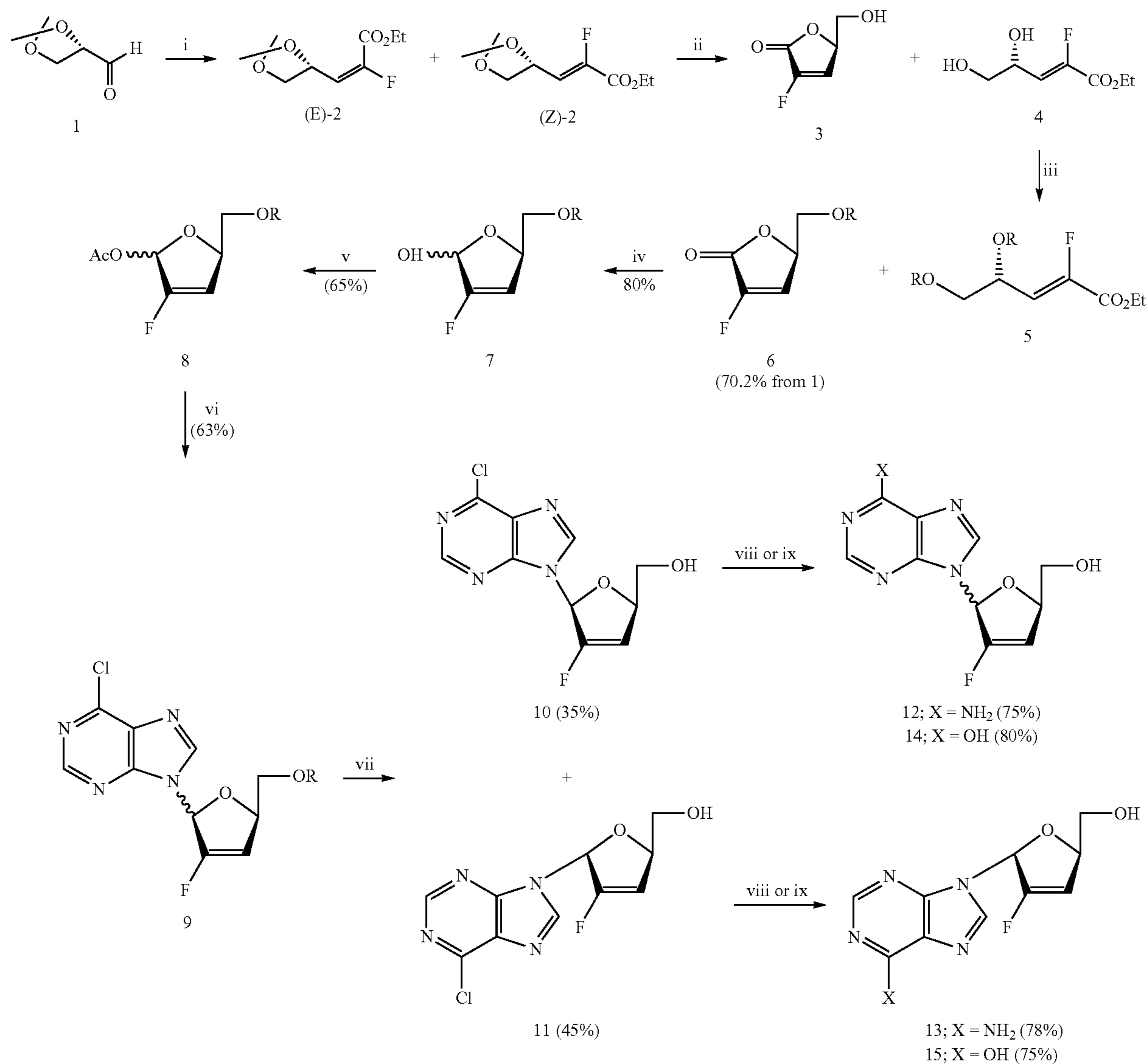
Scheme 10. Synthesis of L-2'-Fluoro-d4Adenine and -Hypoxanthine by Direct Condensation
