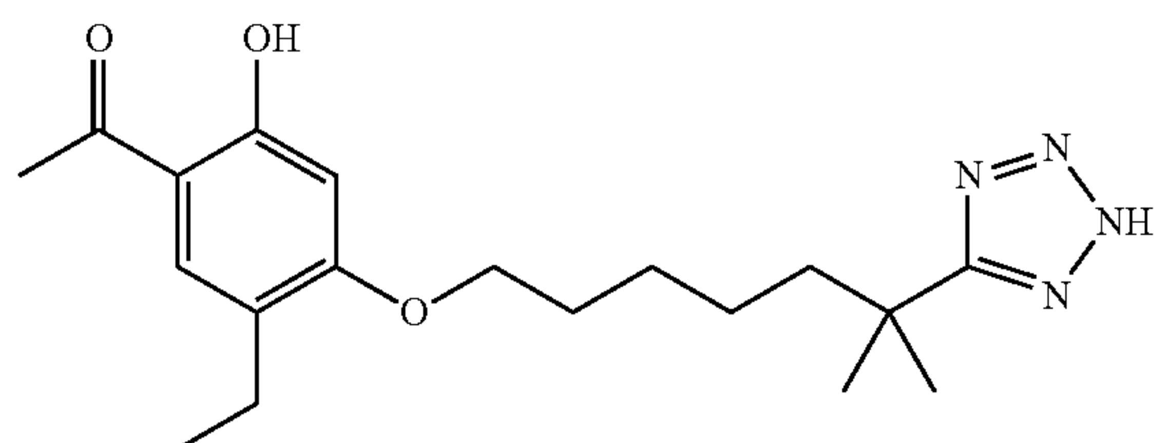
1-(5-ethyl-2-hydroxy-4-((6-methyl-6-(2H-tetrazol-5-yl)heptyl)oxy)phenyl)ethanone
