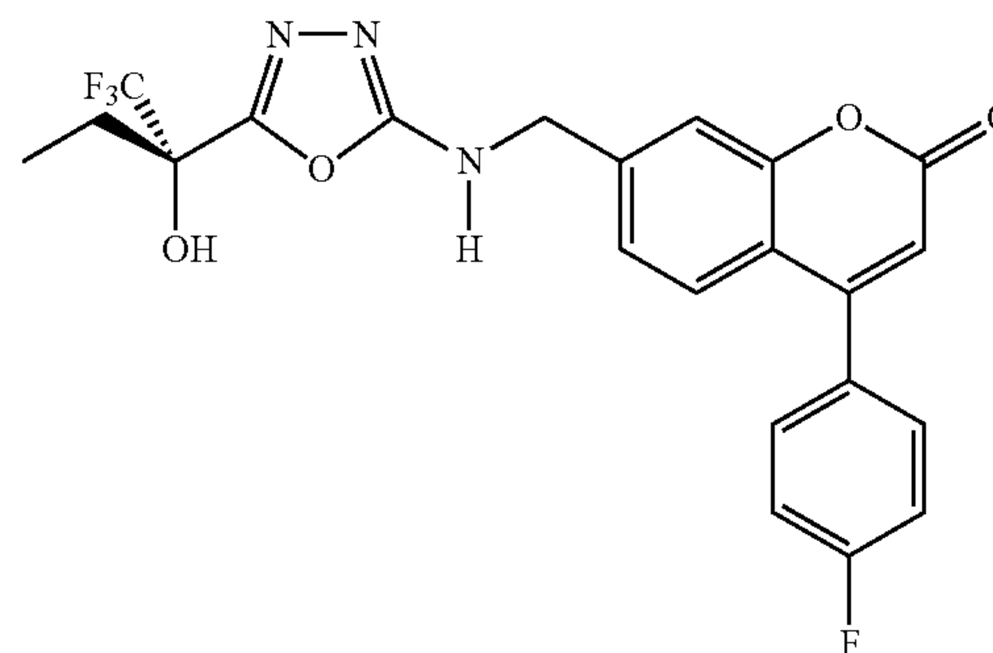
(S)-16
