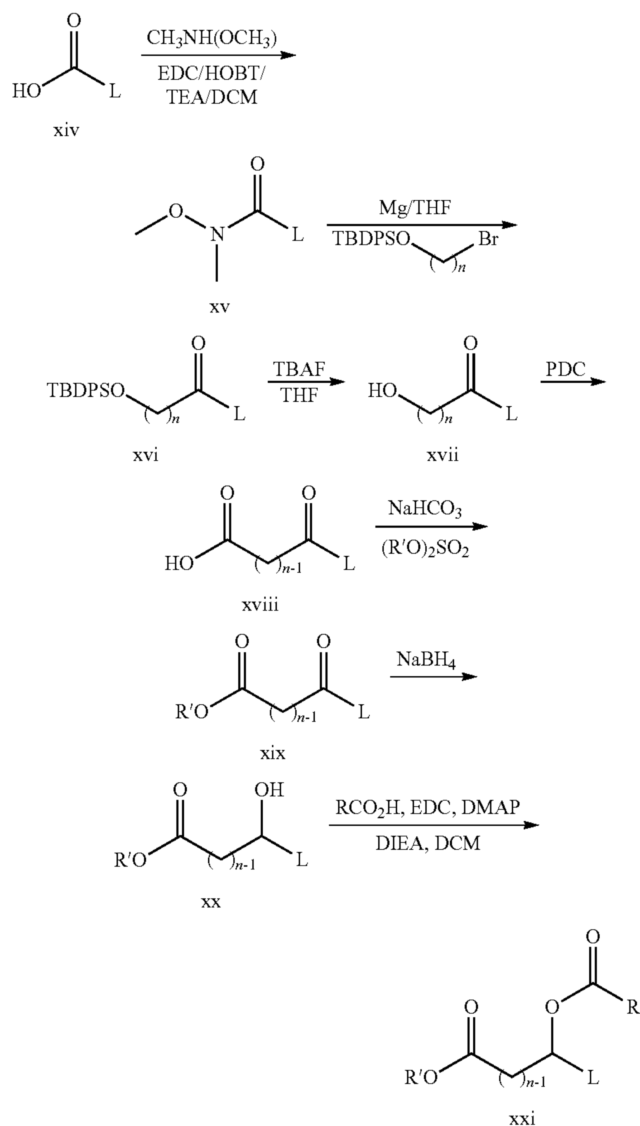
GENERAL SCHEME 4
