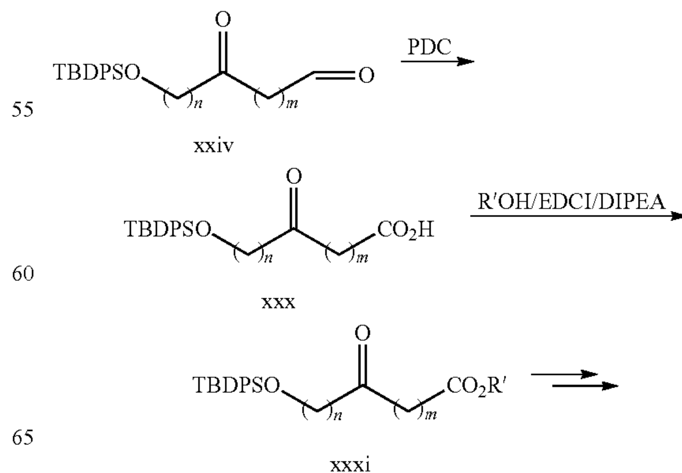
GENERAL SCHEME 5
