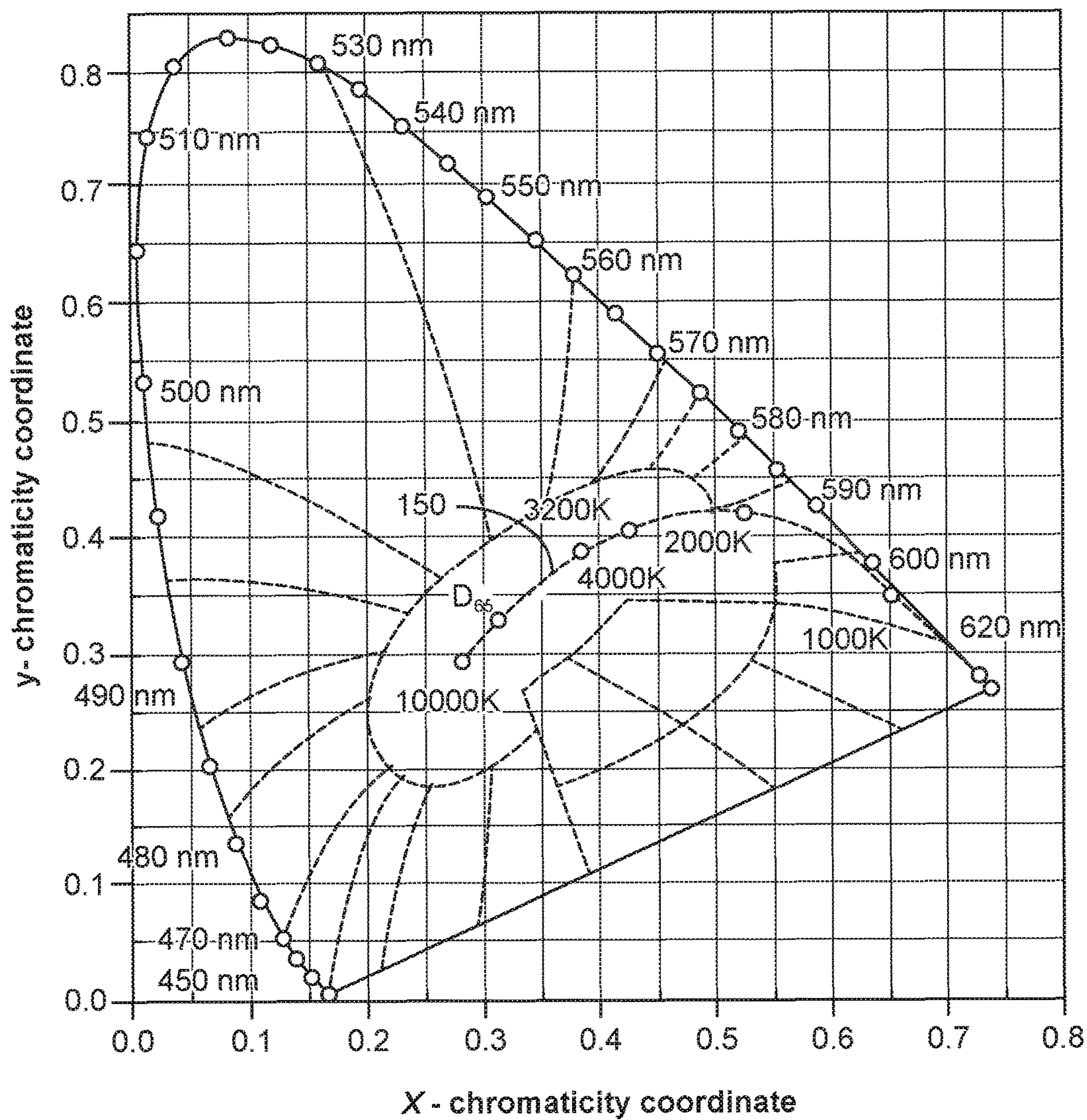
FIG. 3 PRIOR ART
