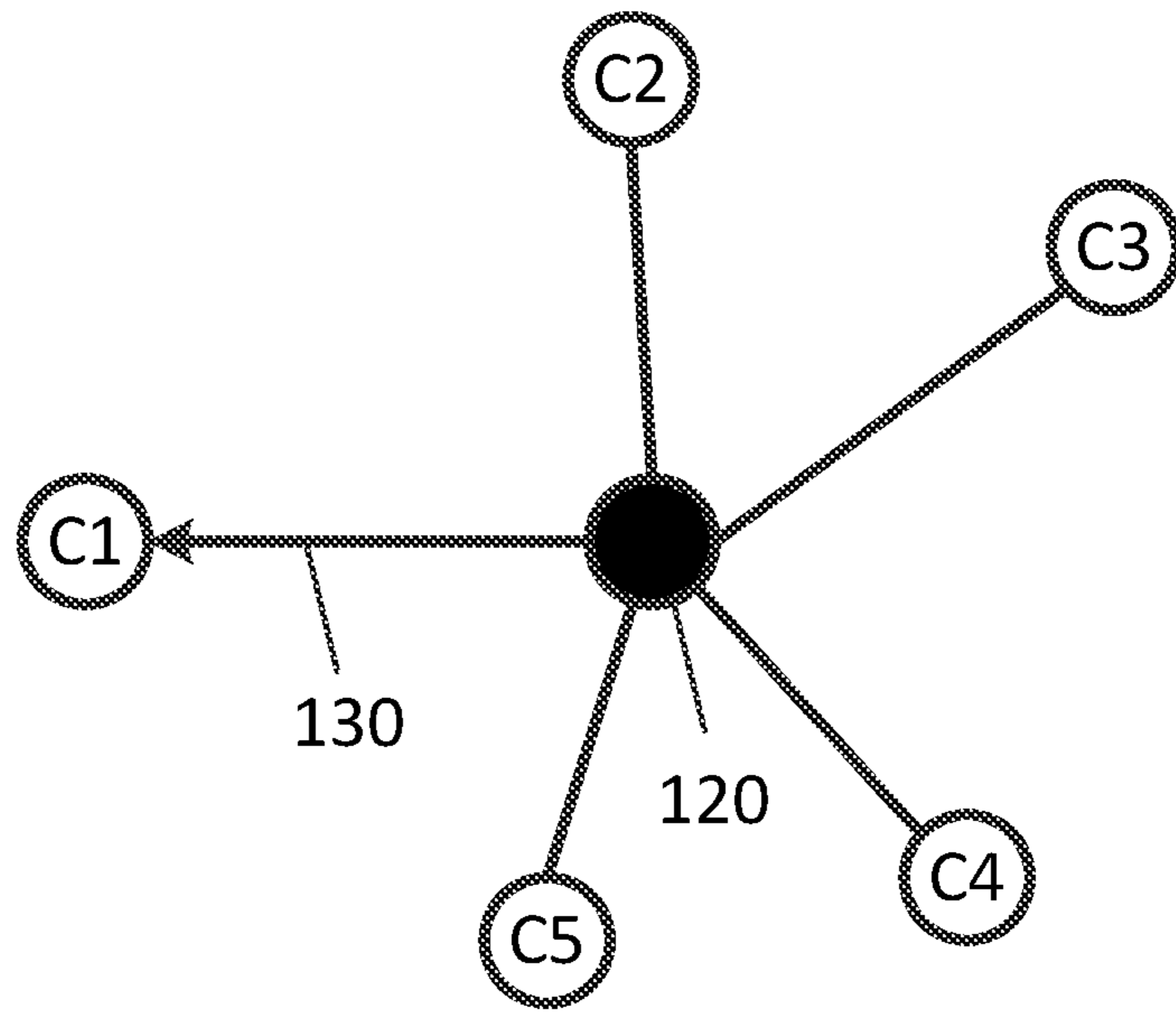
Client Server 110
