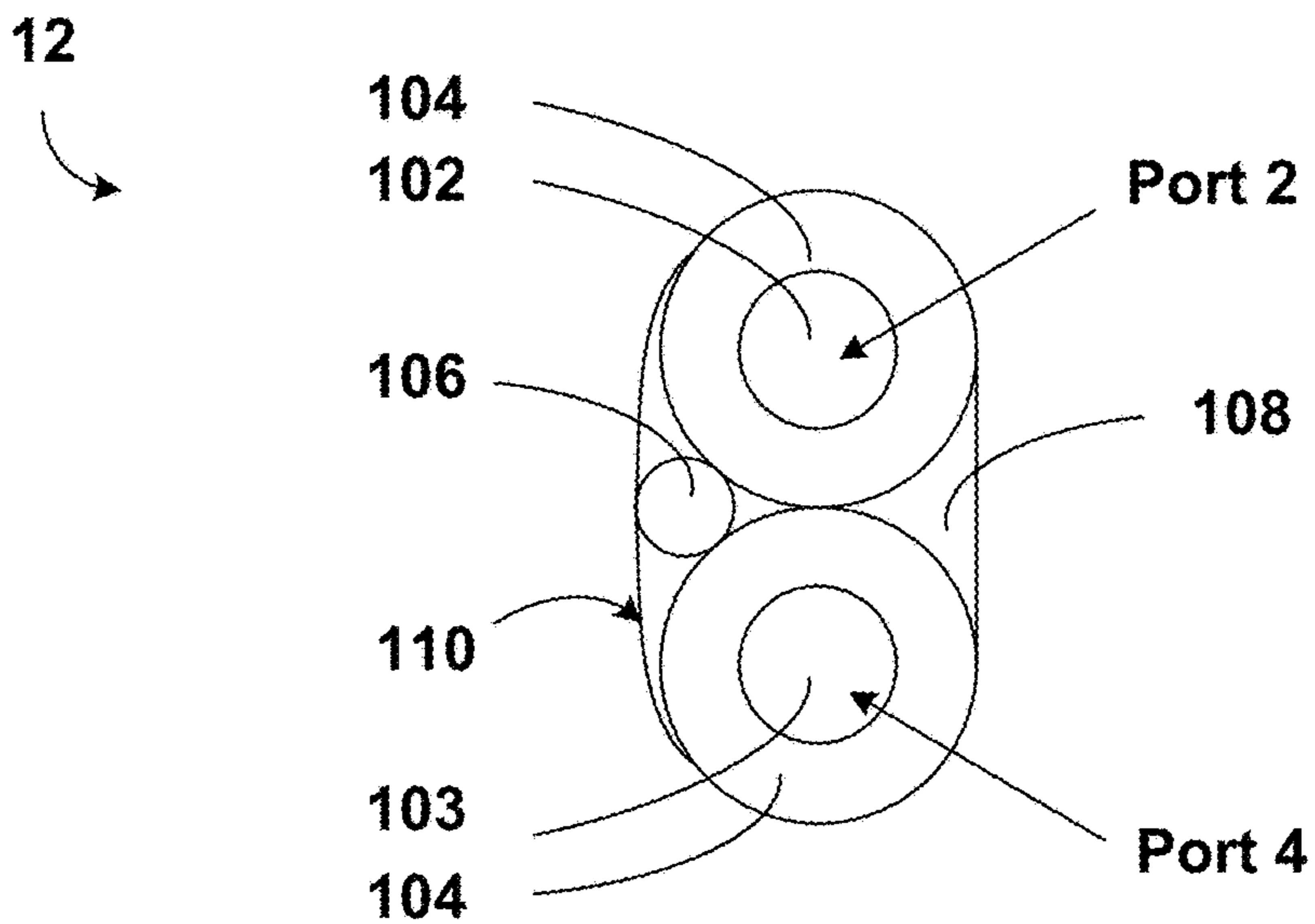
Figure 3 Section B-B
