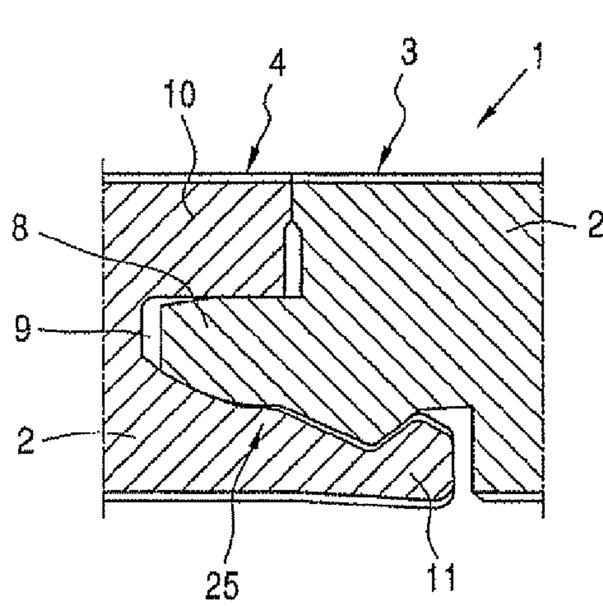
FIG. 4 PRIOR ART
