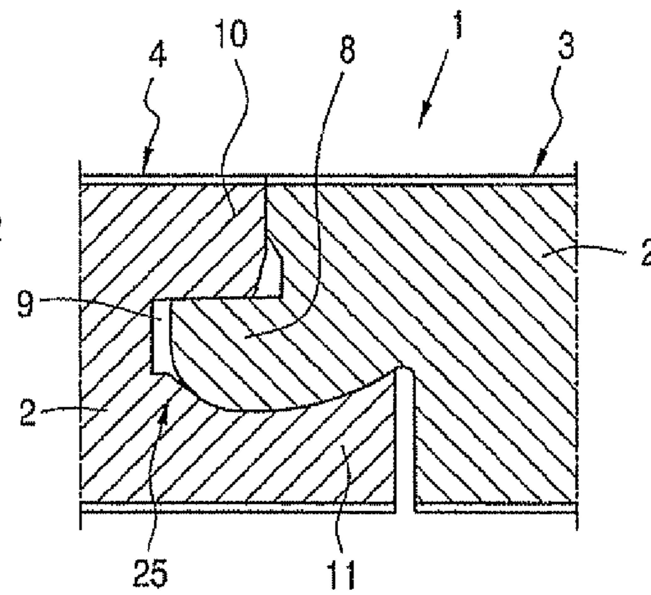
FIG. 5 PRIOR ART
