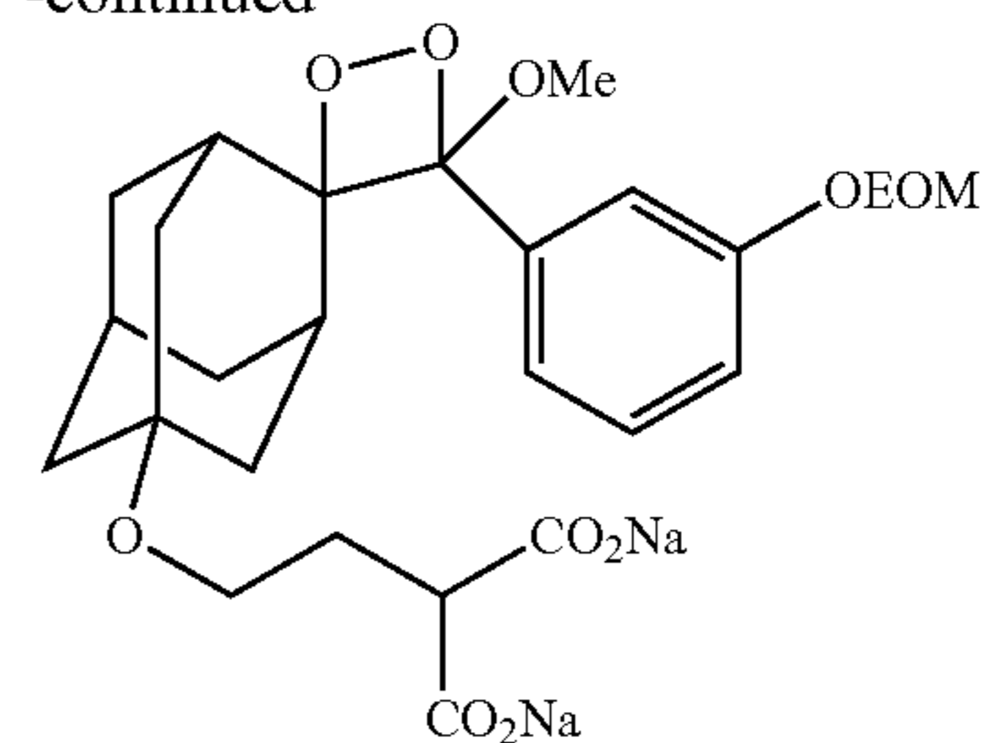
bis-CO 2 Na-Ad-Ph-OEOM dxt (Compound 15)
