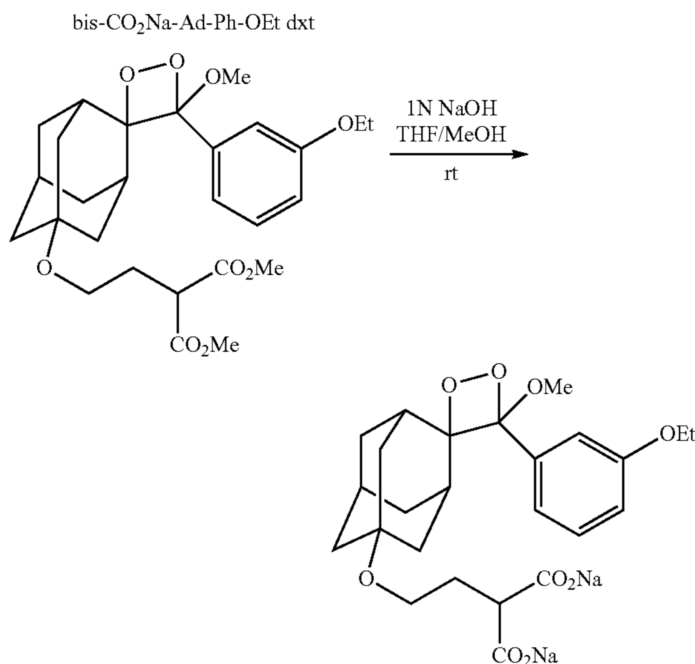
bis-CO 2 Na-Ad-Ph-OEt dxt (Compound 14)
