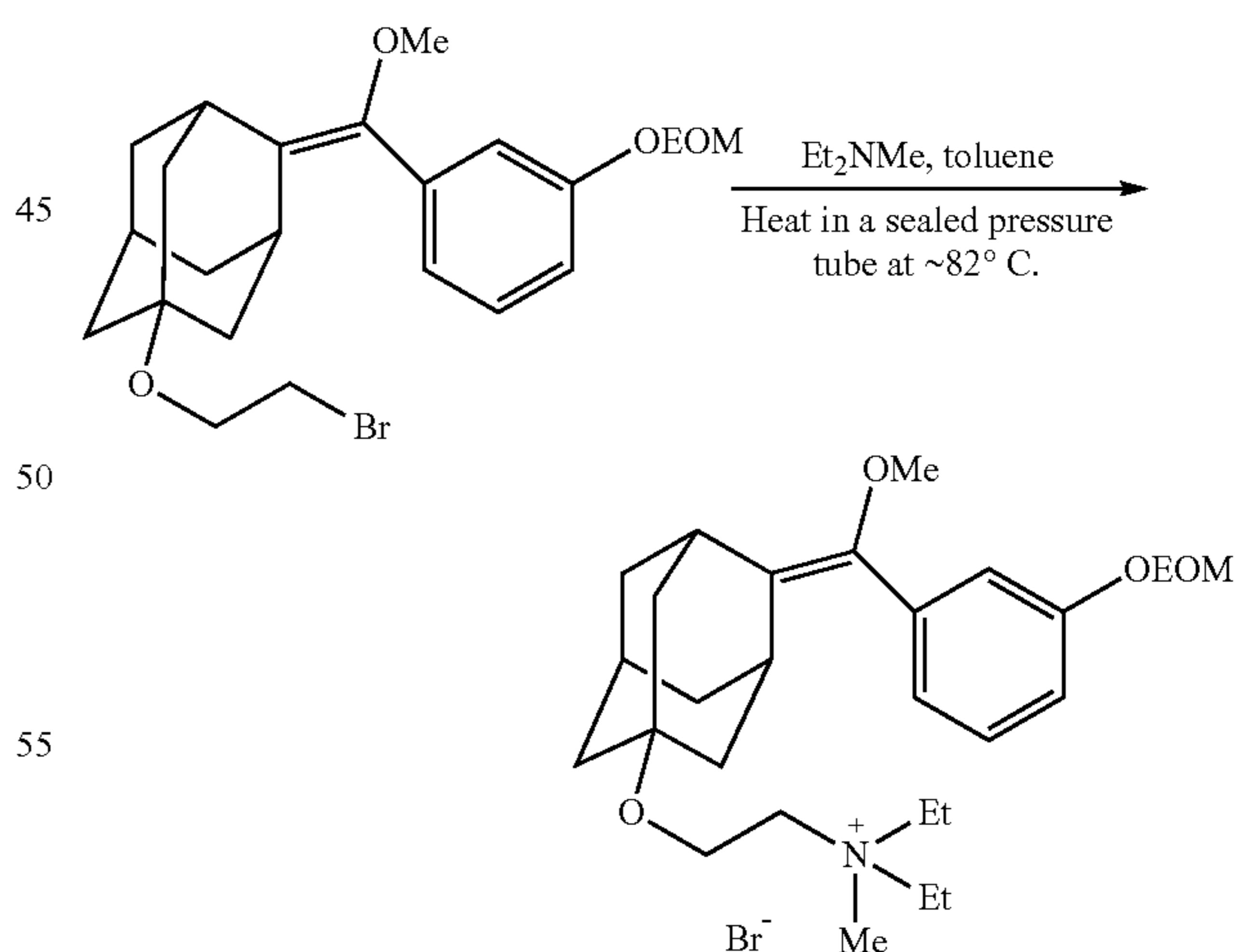
Q + -Amino-Ad-Ph-OEt EE (Compound 12a)
