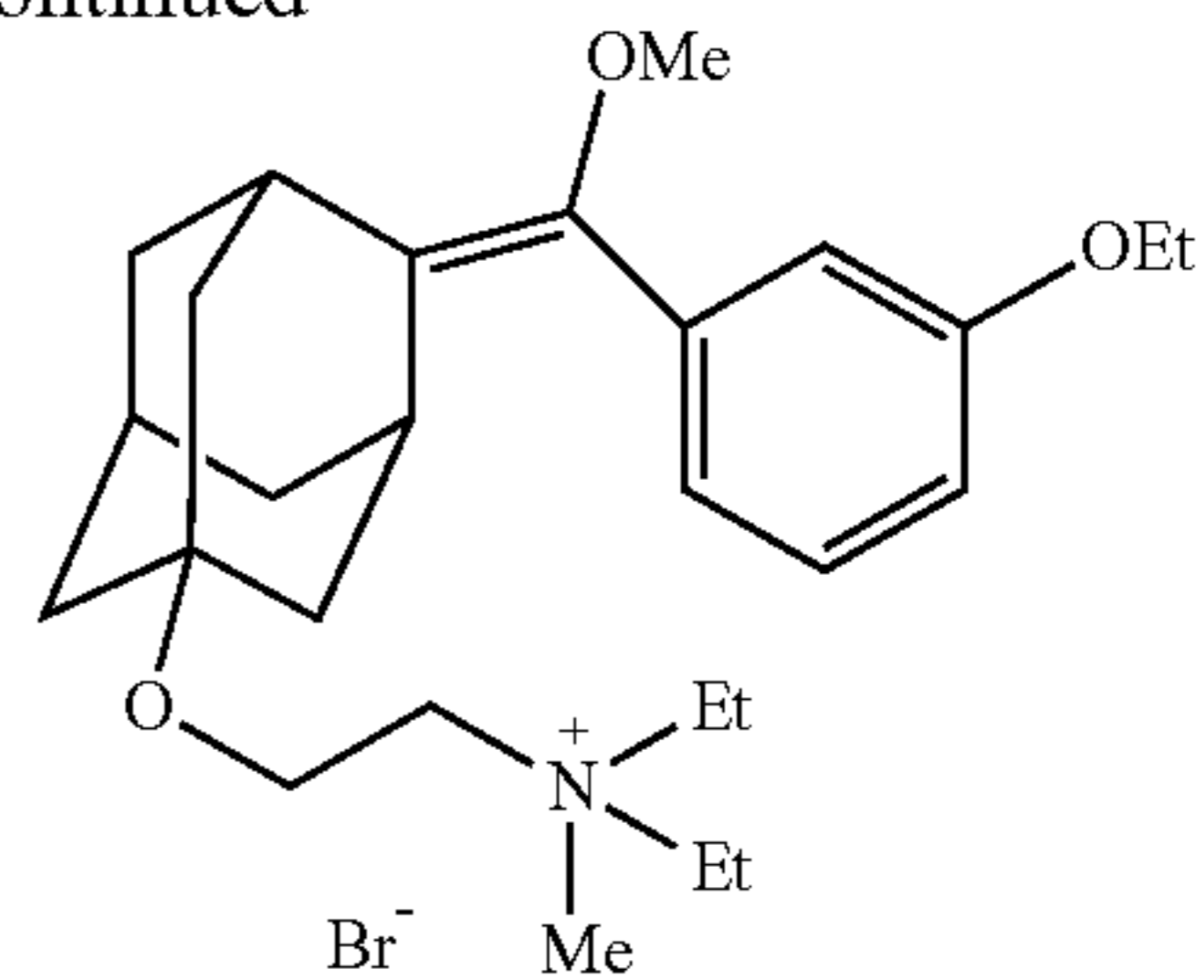
Q + -Amino-Ad-Ph-OEt EE (Compound 12a)
