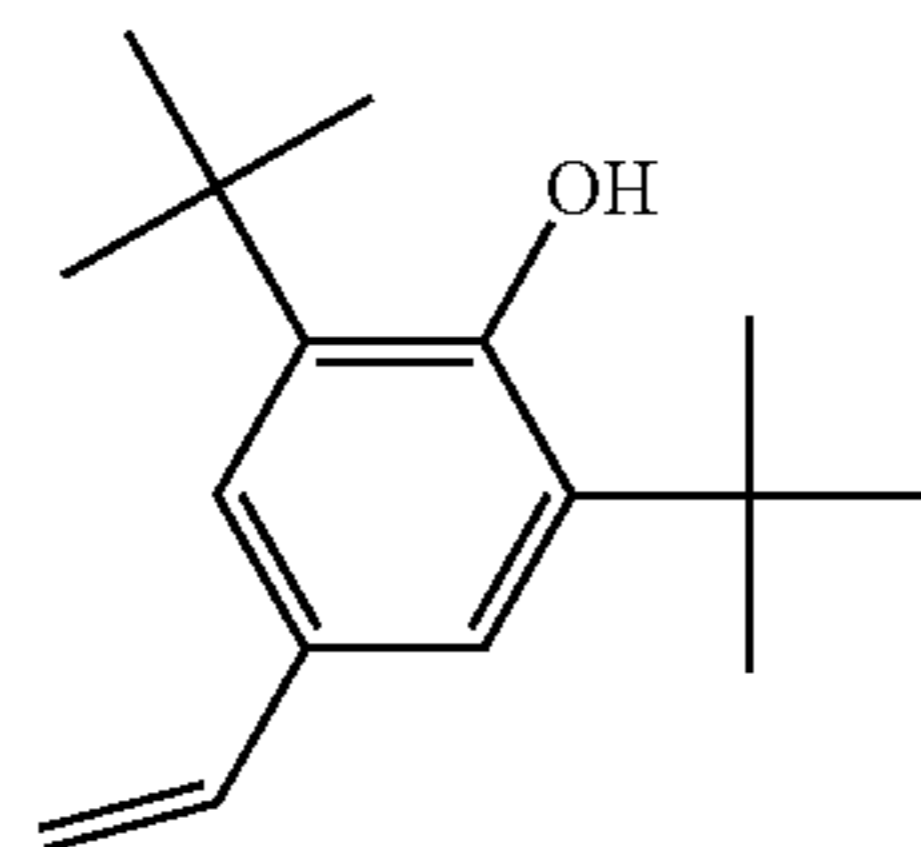
2,6-di-tert-butyl-4-vinylphenol
