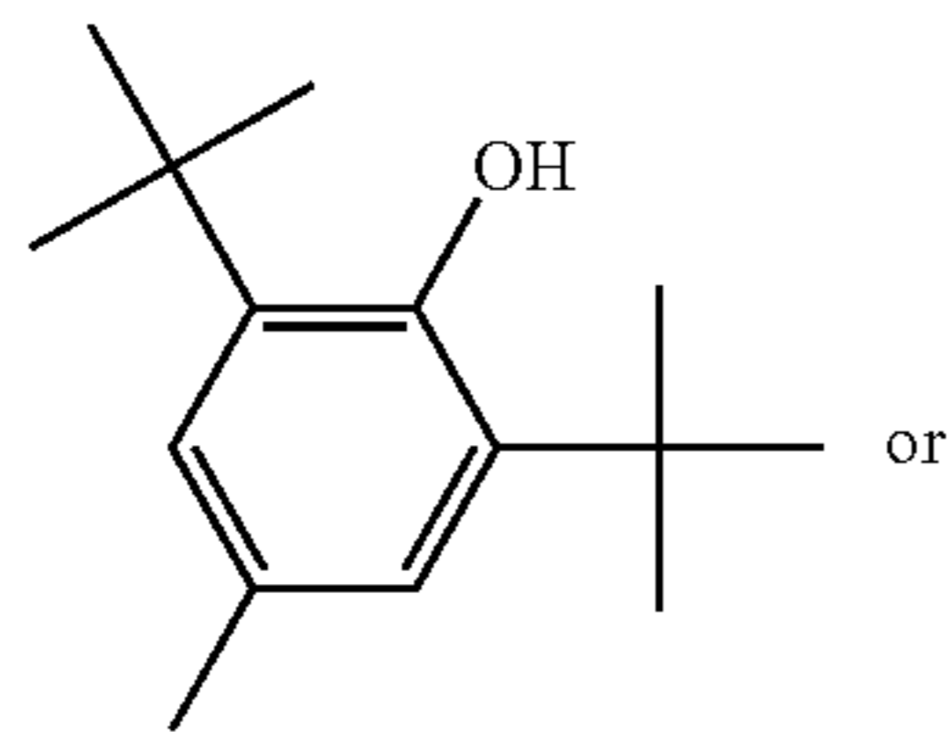
2,6-bis(1,1-dimethylethyl)-4-methylphenol (BHT)
