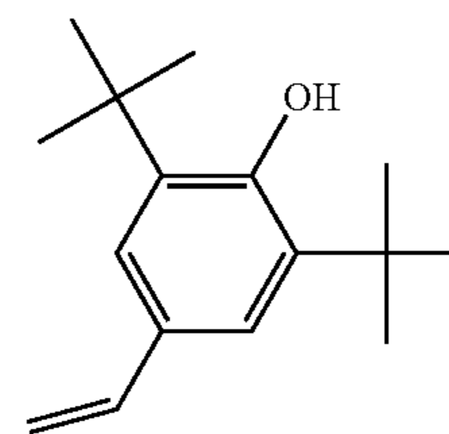
2,6-di-tert-butyl-4-vinylphenol
