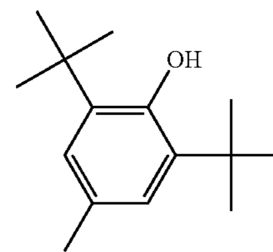
2,6-bis(1,1-dimethylethyl)-4-methylphenol (BHT)
