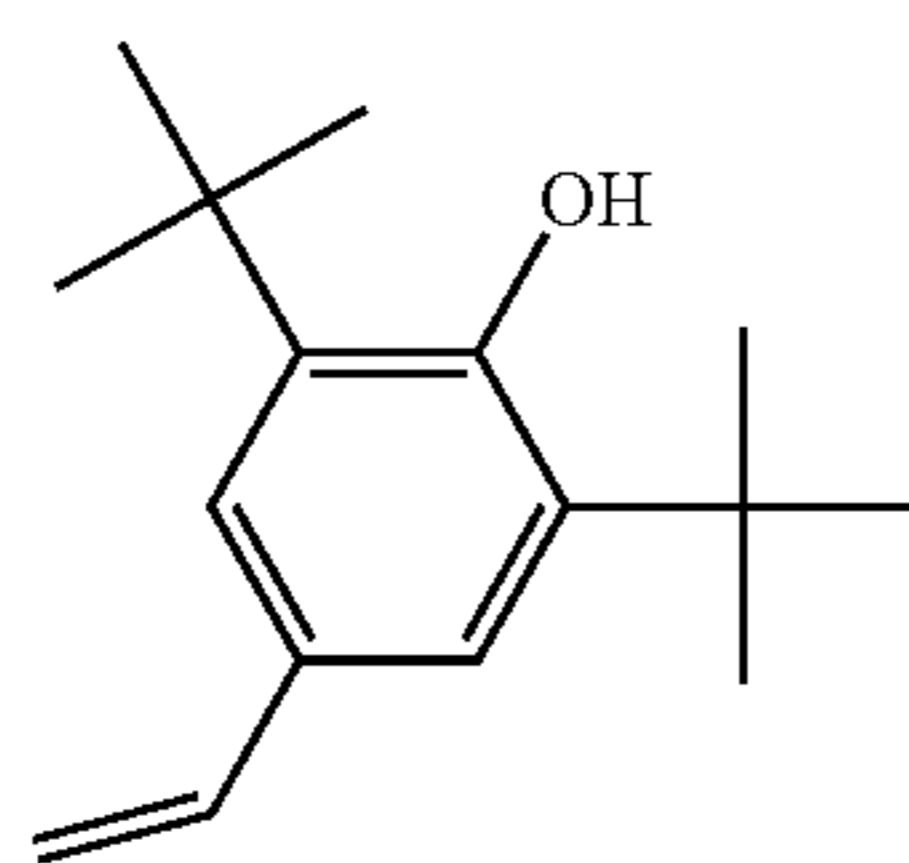
2,6-di-tert-butyl-4-vinylphenol
