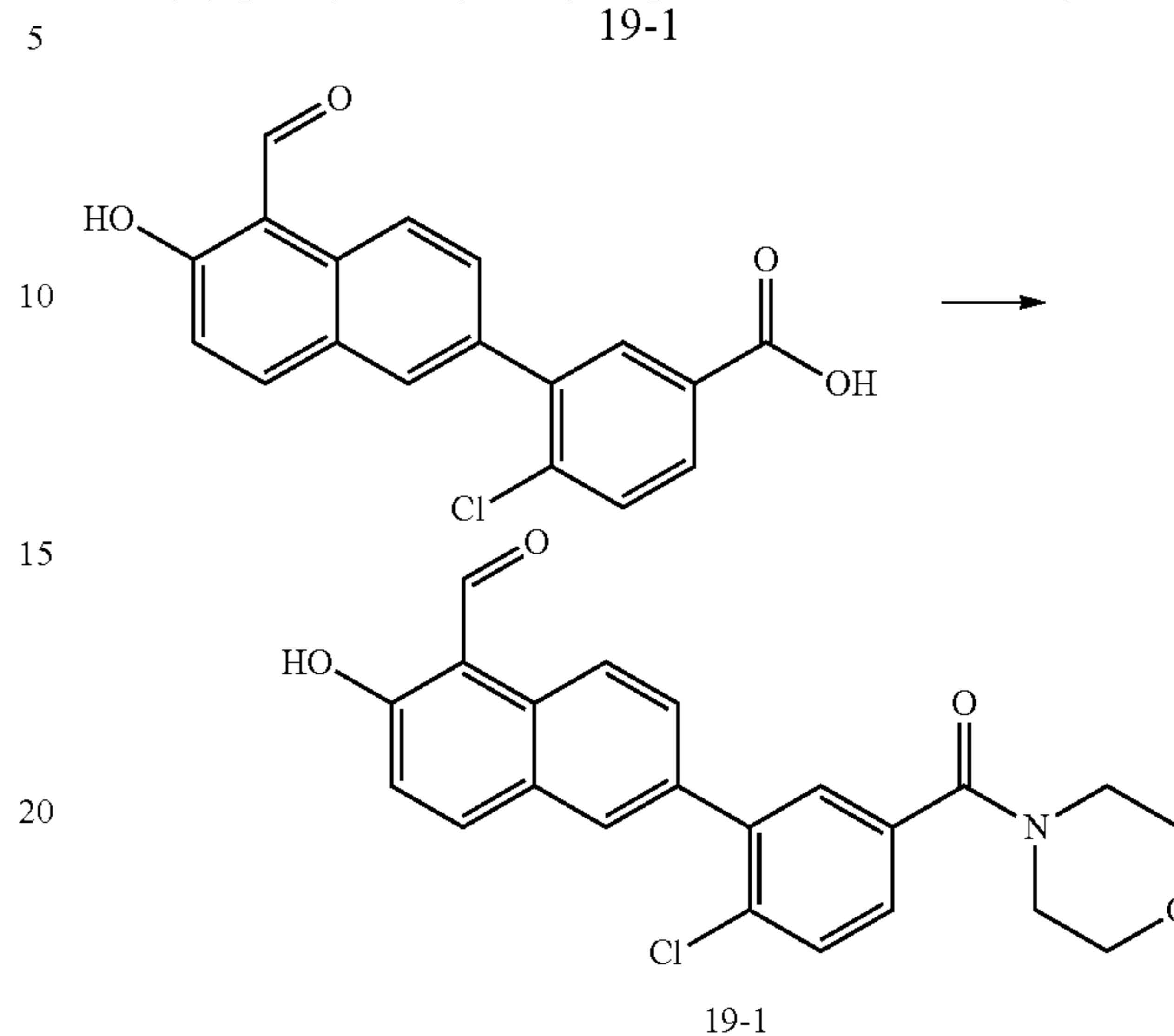
Synthesis of 6-[2-Chloro-5-(morpholine-4-carbonyl)-phenyl]-2-hydroxy-naphthalene-1-carbaldehyde 19-1
