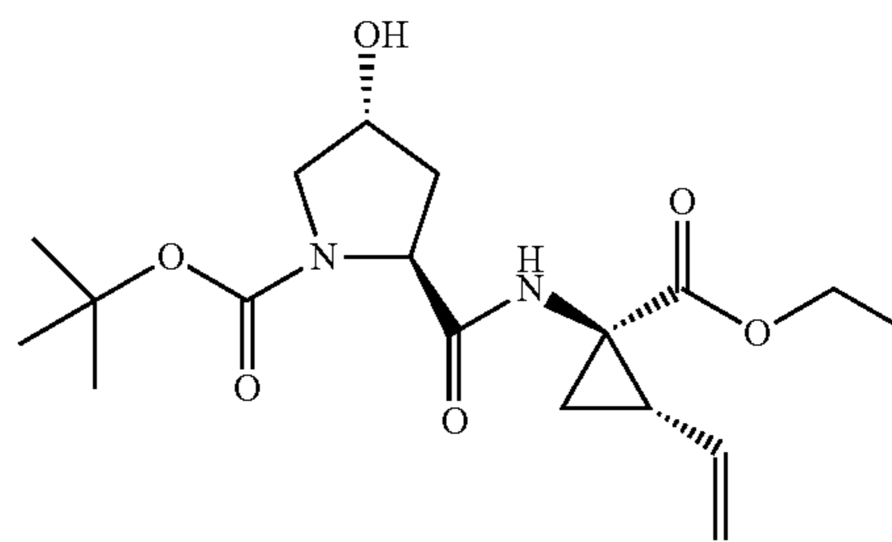
2-(1-Ethoxycarbonyl-2-vinyl-cyclopropylcarbamoyl)-4-hydroxy-pyrrolidine-1-carboxylic acid tert-butyl ester (132)
