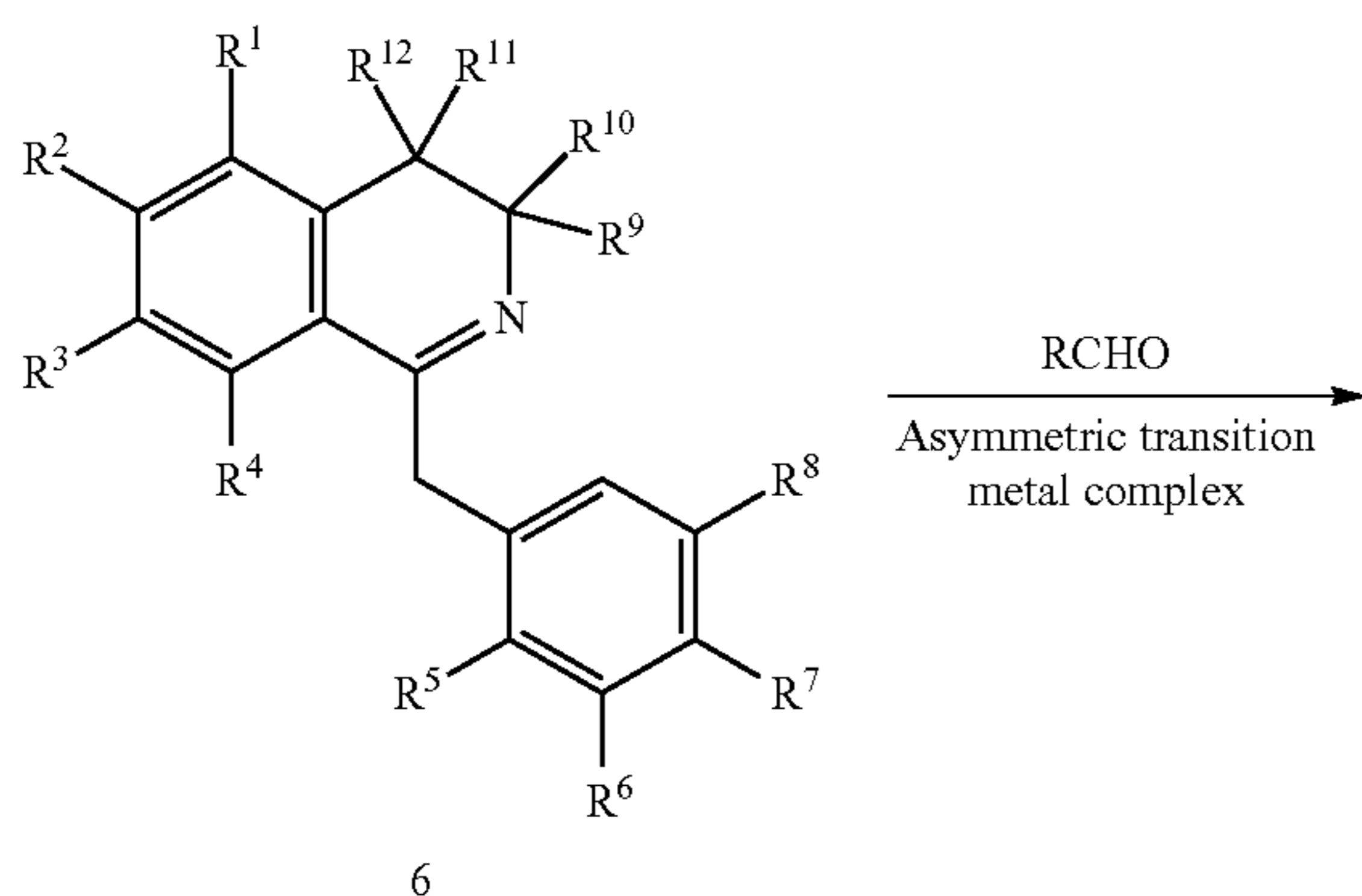
Reaction Scheme 2
