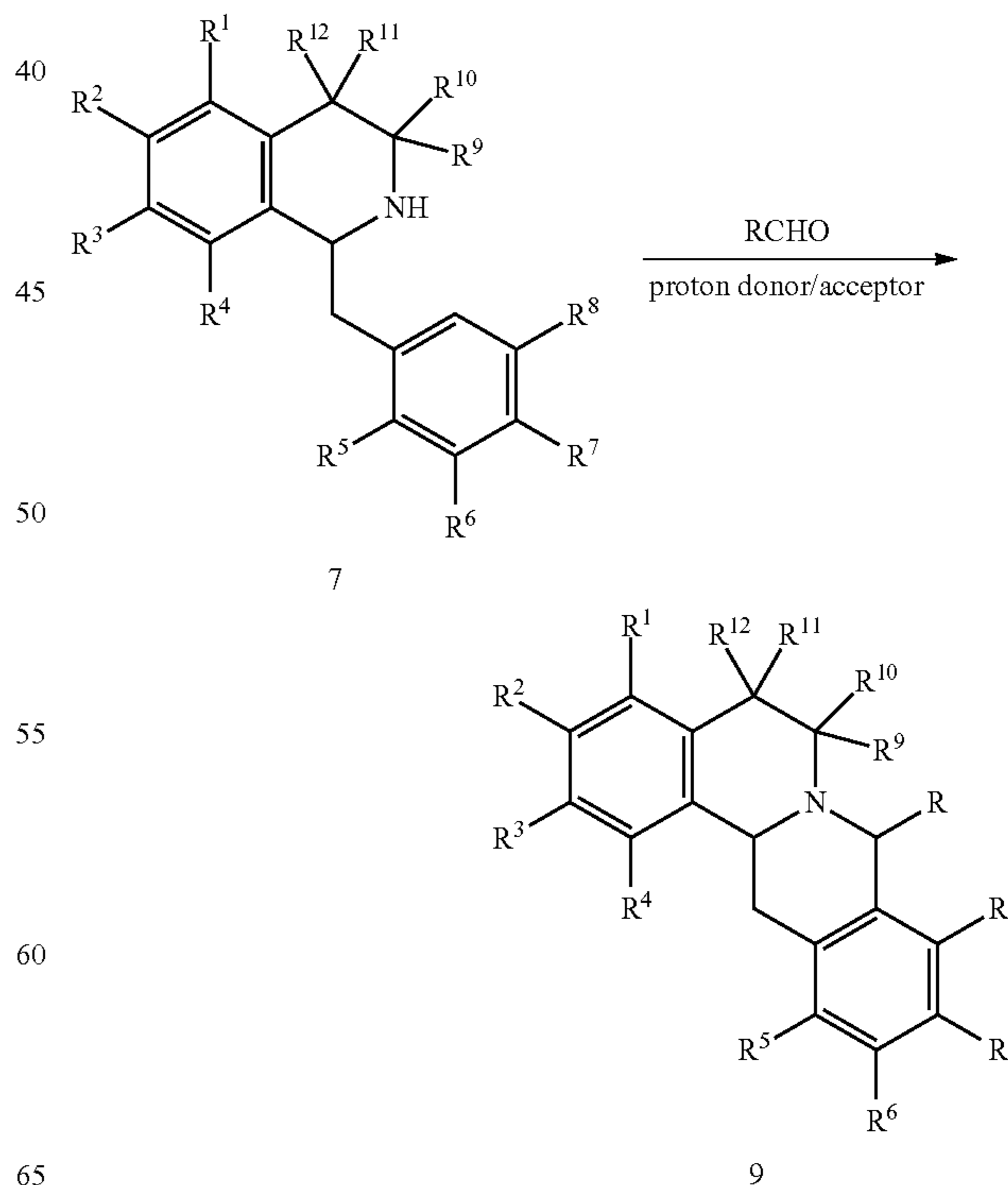
Reaction Scheme 1
