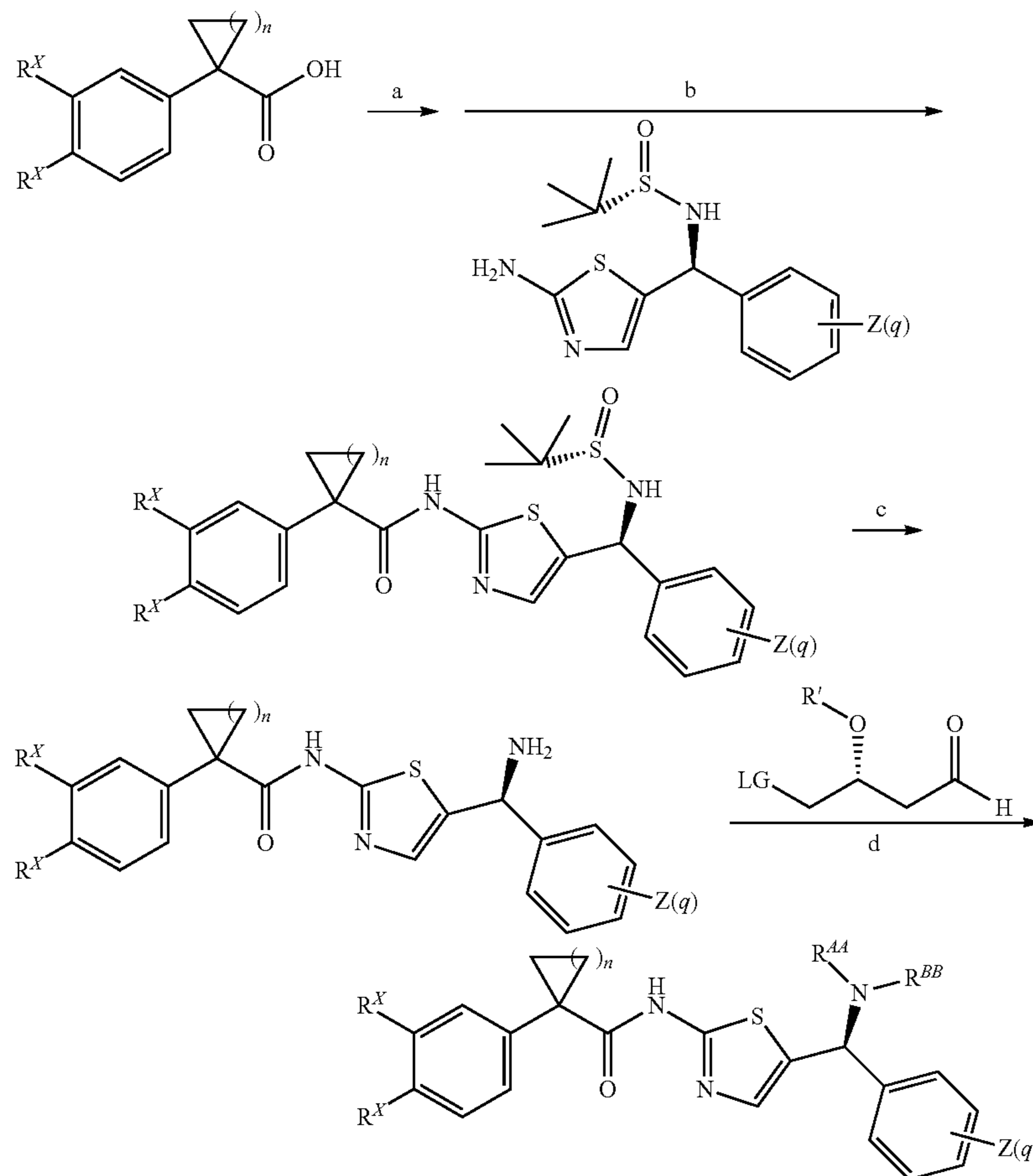
Scheme III, Step C:
