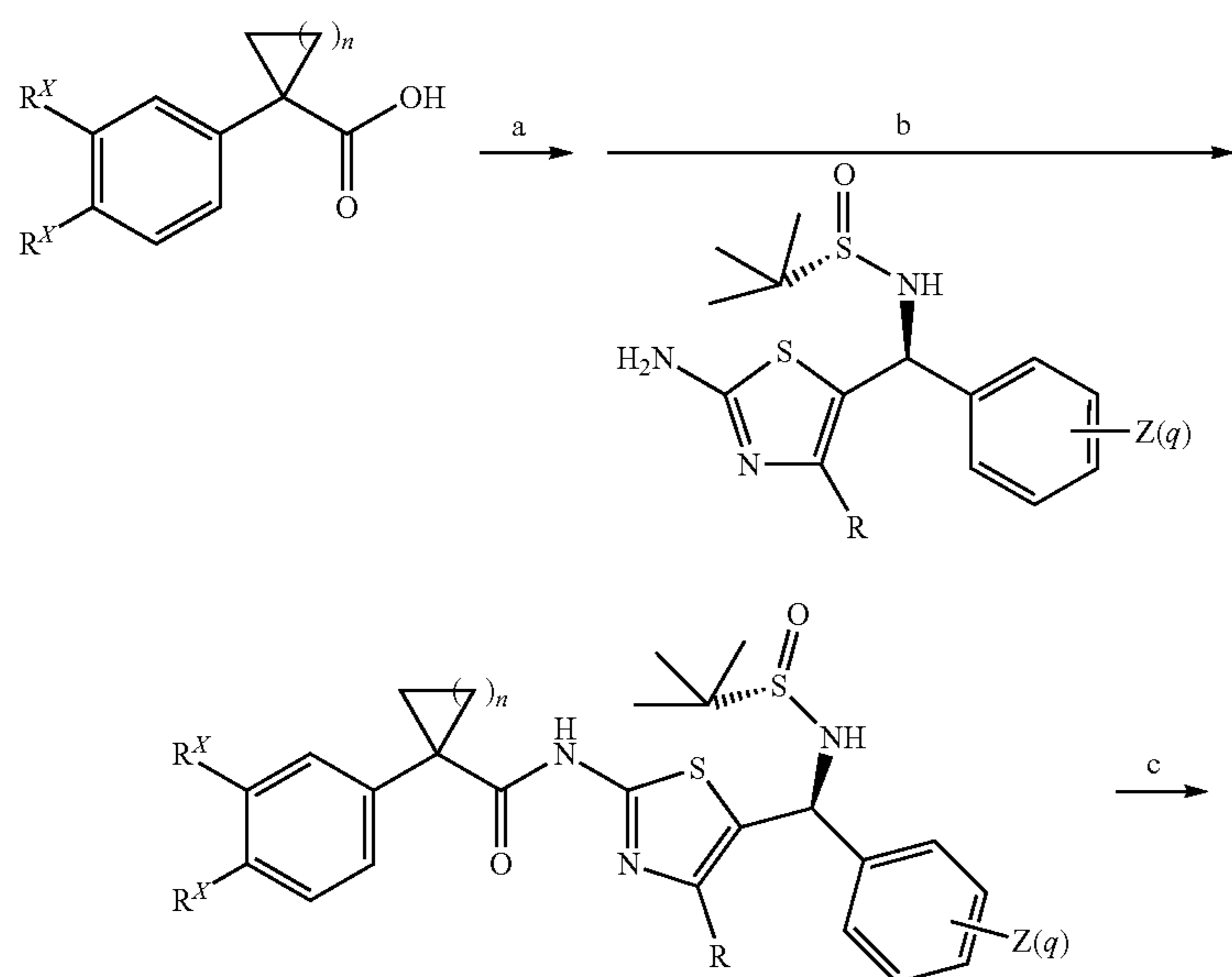
Scheme C:
