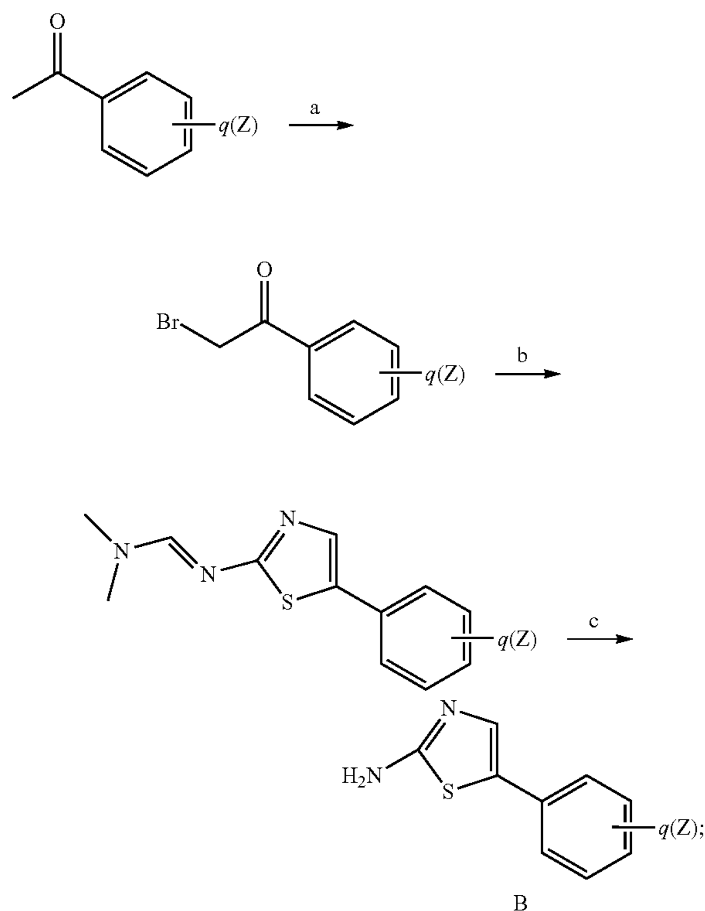
Scheme I-B:
