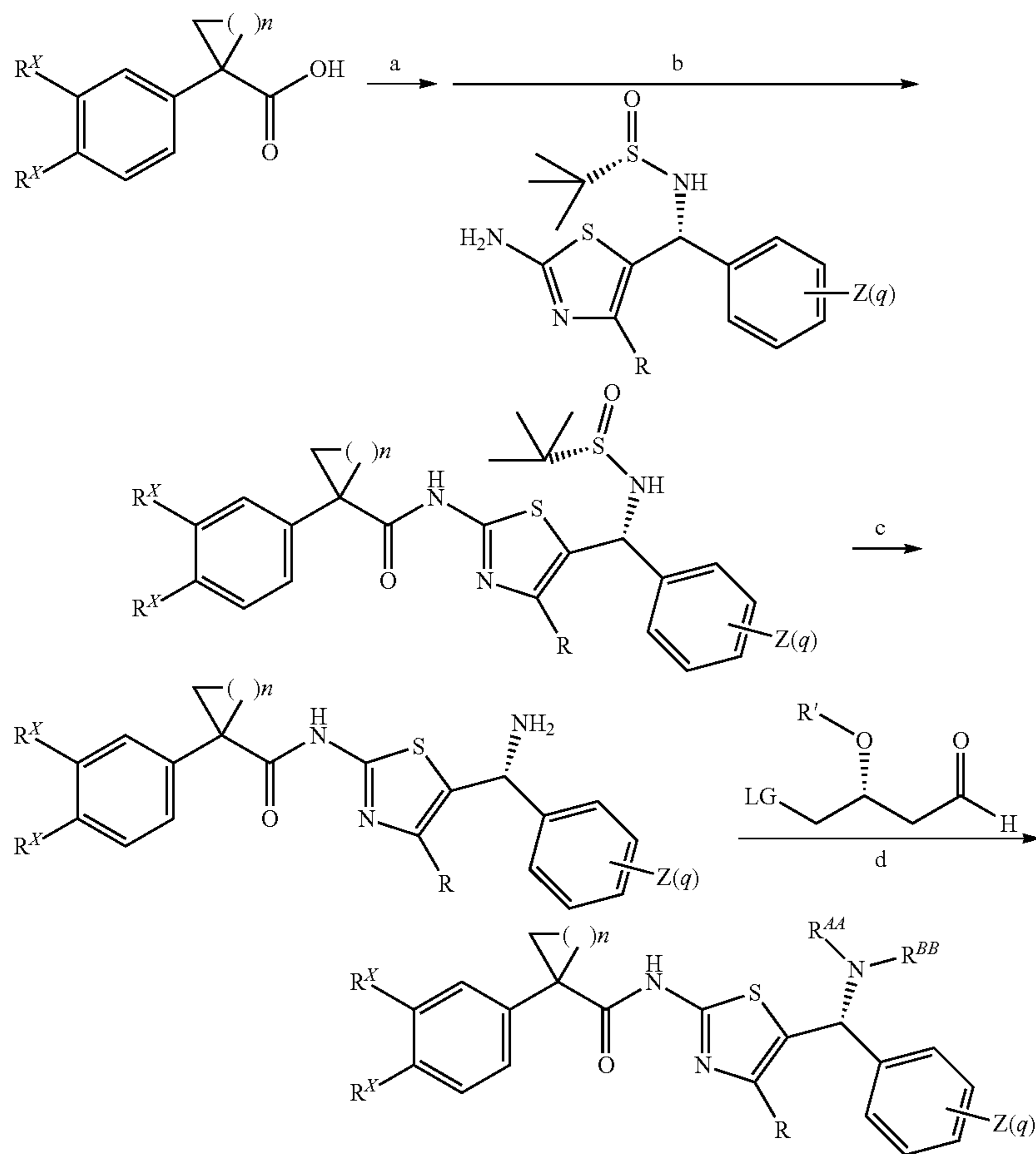
Scheme B:
