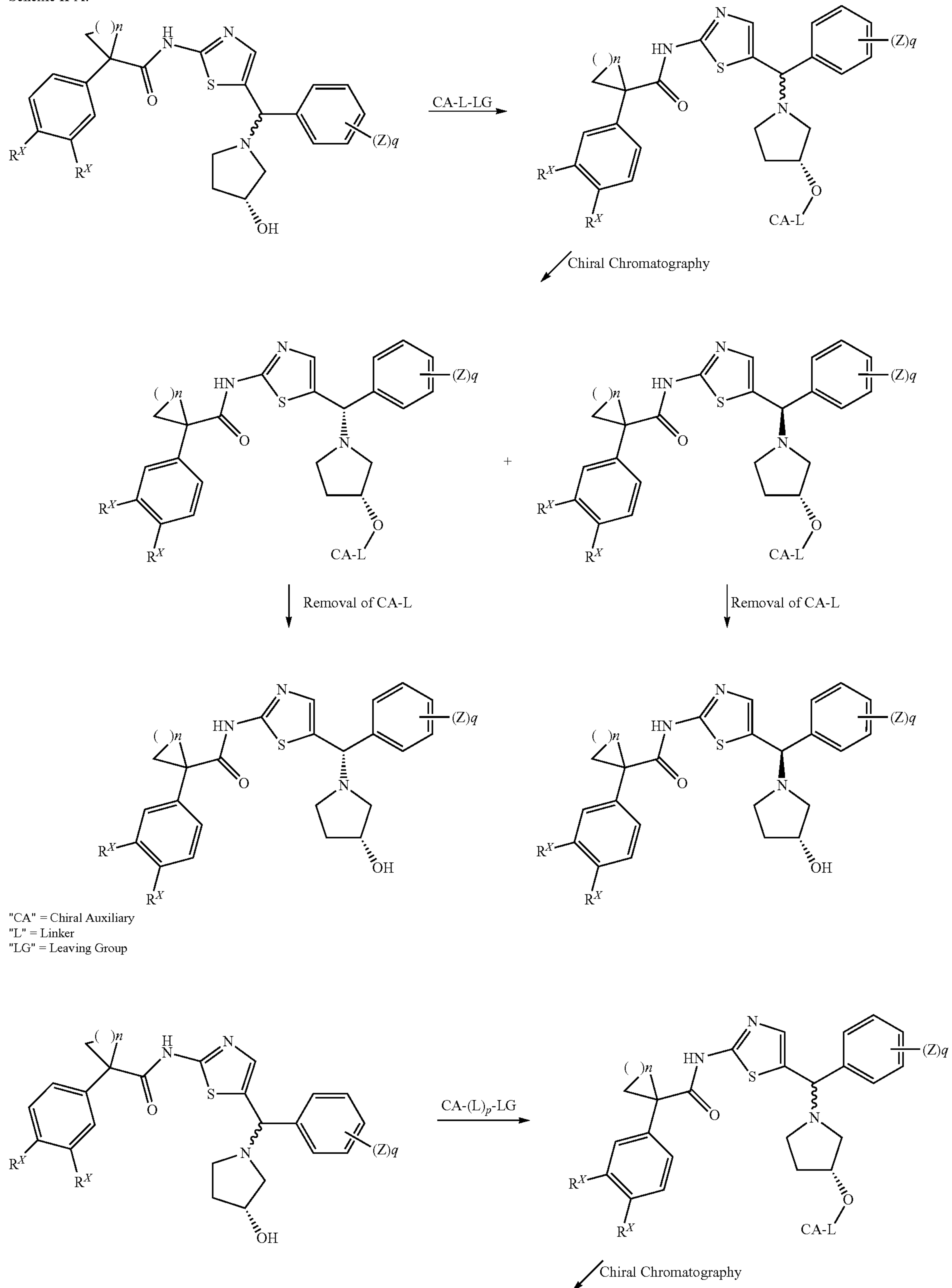
Scheme II-A:
