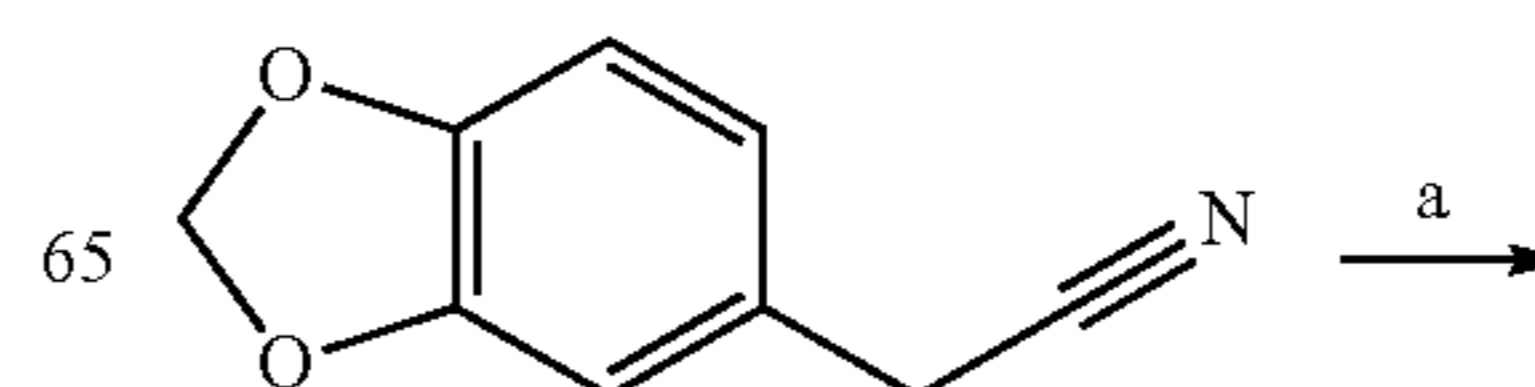
Scheme I-D:
