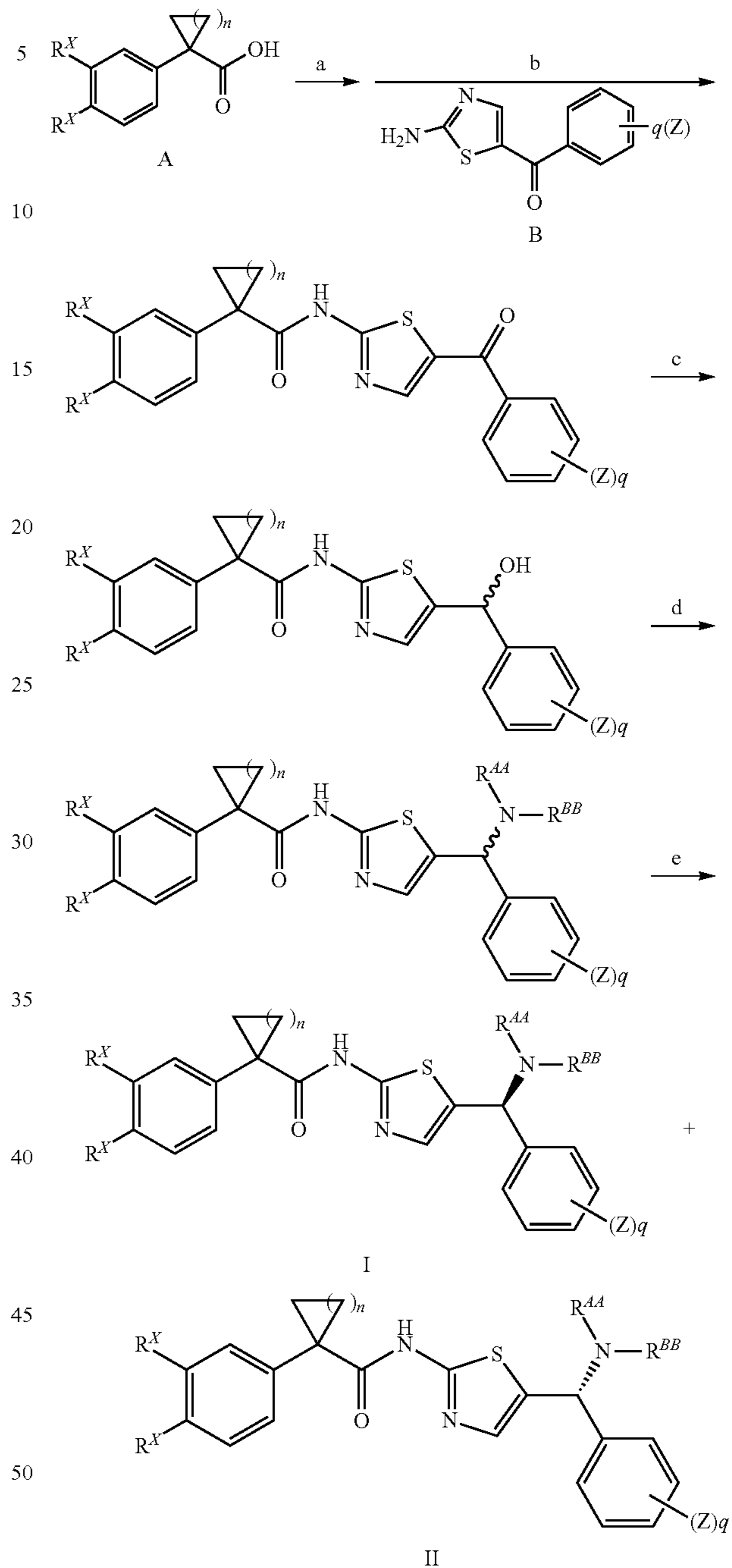
Scheme I-C:
