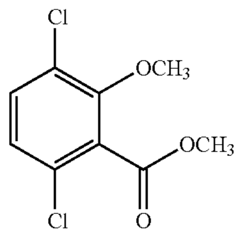
Methyl 3,6-dichloro-2-methoxybenzoate
