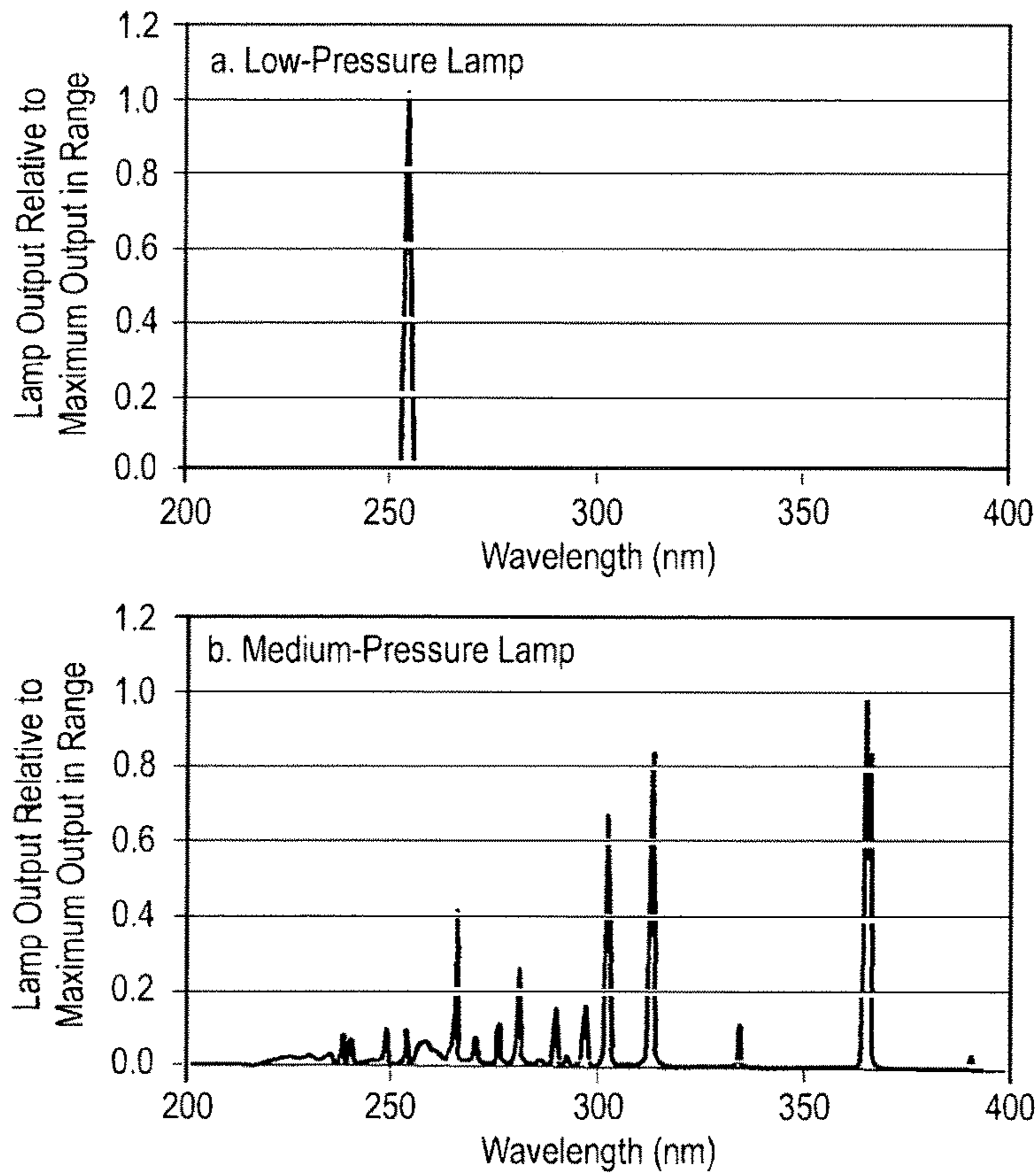
Fig. 1 Prior Art
