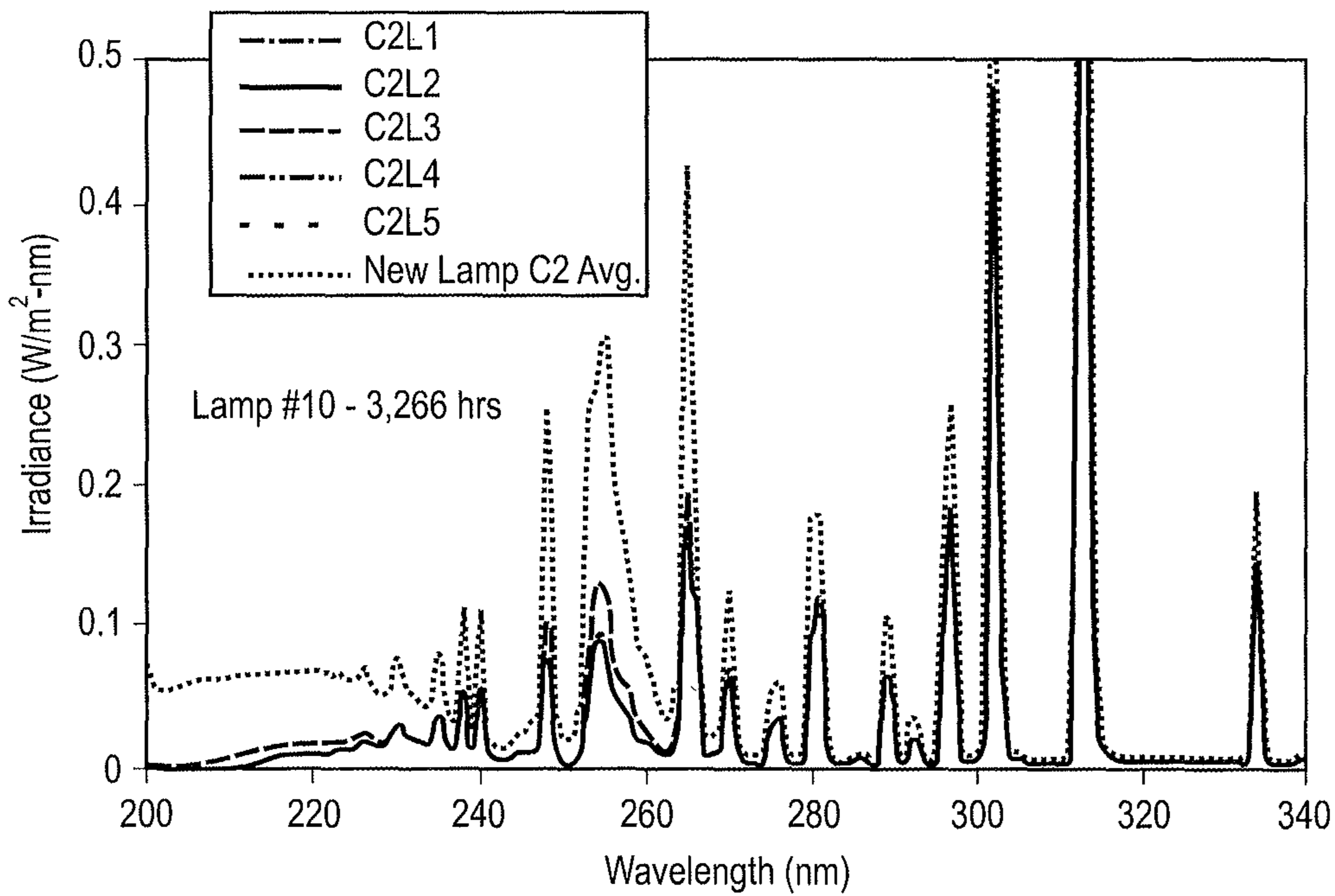
Figure 4.40 Spectral irradiance of Type 1MP lamp #10 as a function of location along the lamp length and around the circumference (C1 - top, C2 - bottom)
