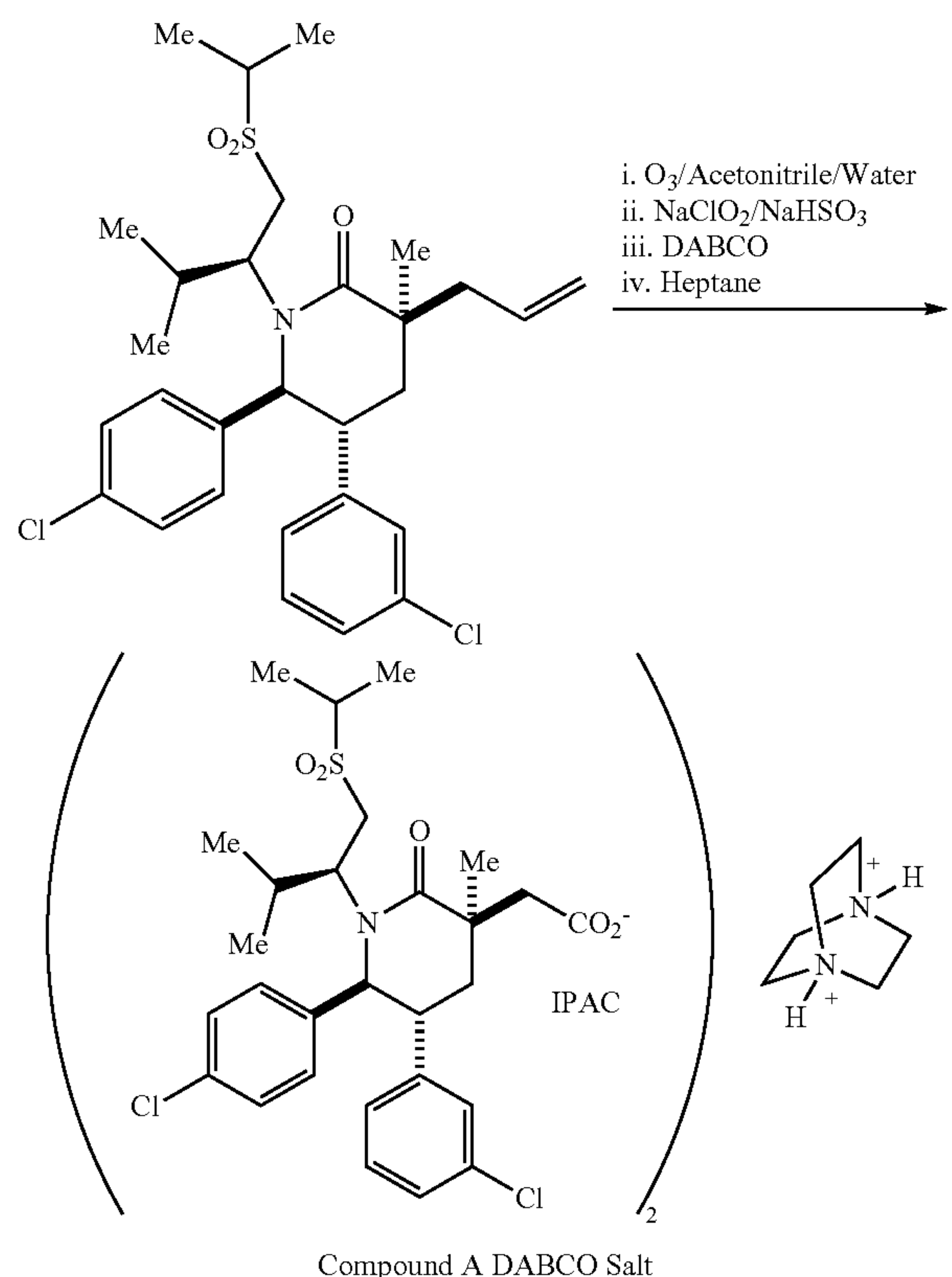
Scheme 3 - DABCO Salt Process
