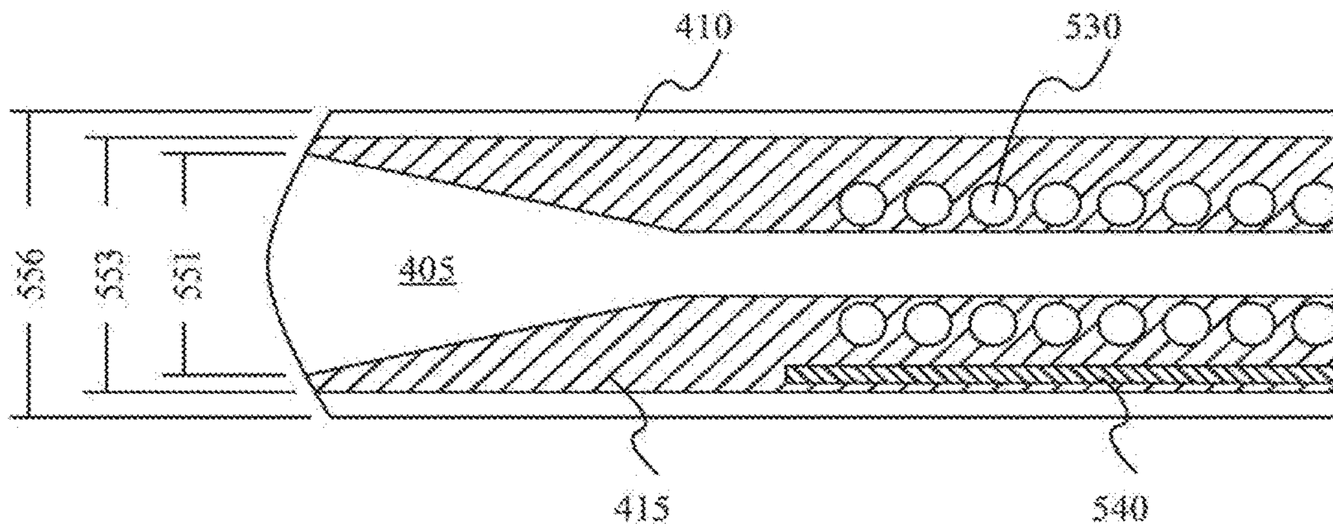
SECTION B-B FIG 5
