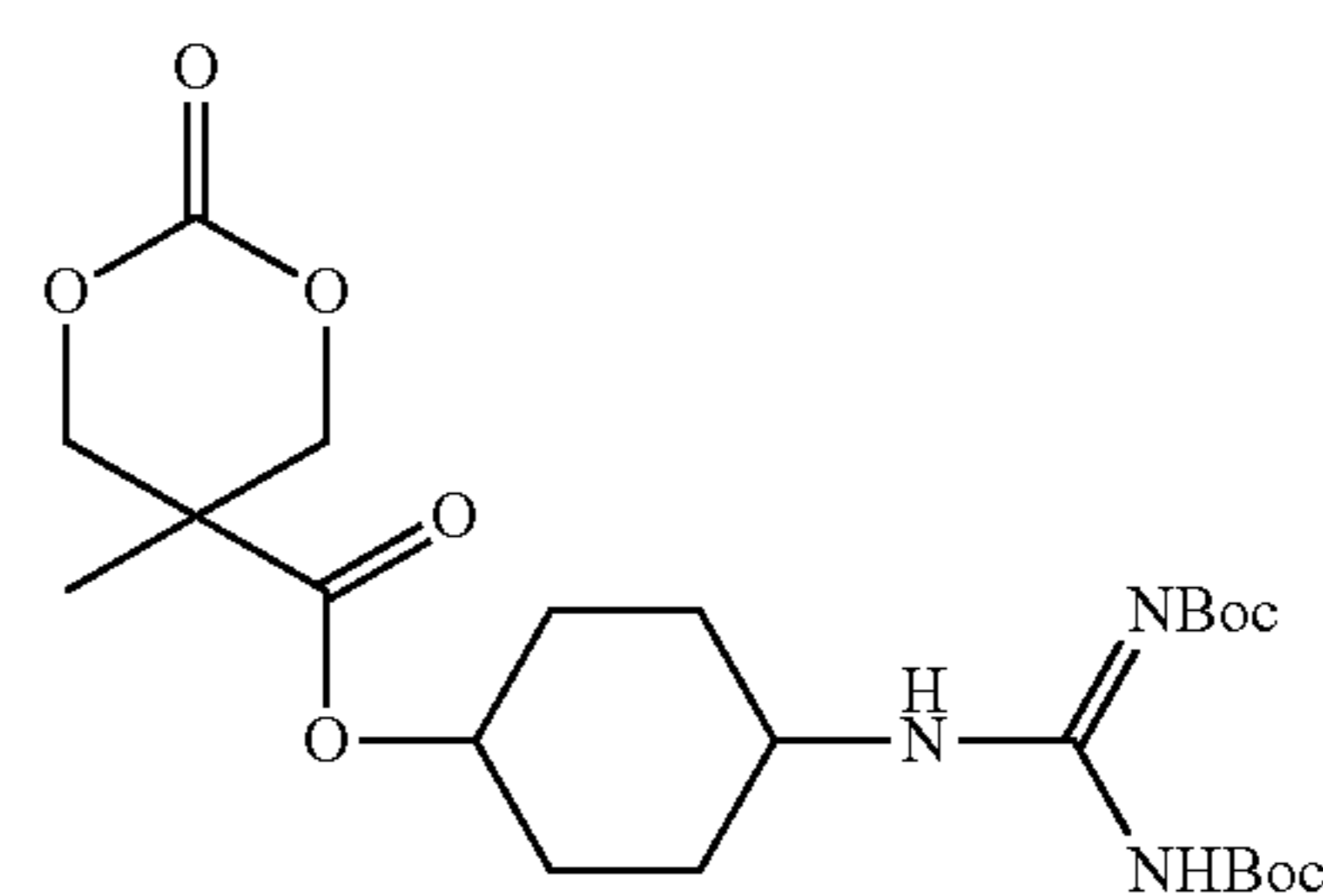
MTC-CyG1
