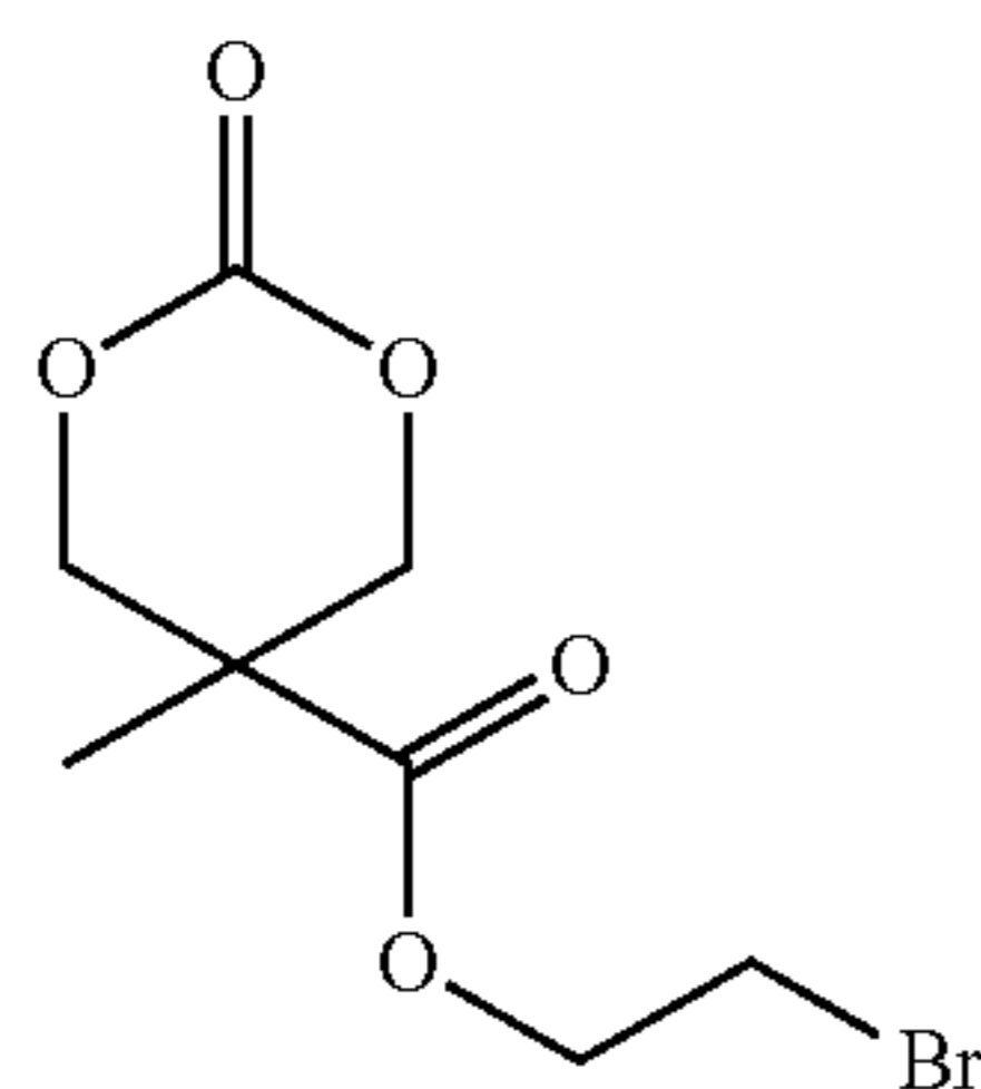
MTC-C2Br MW 267.1
