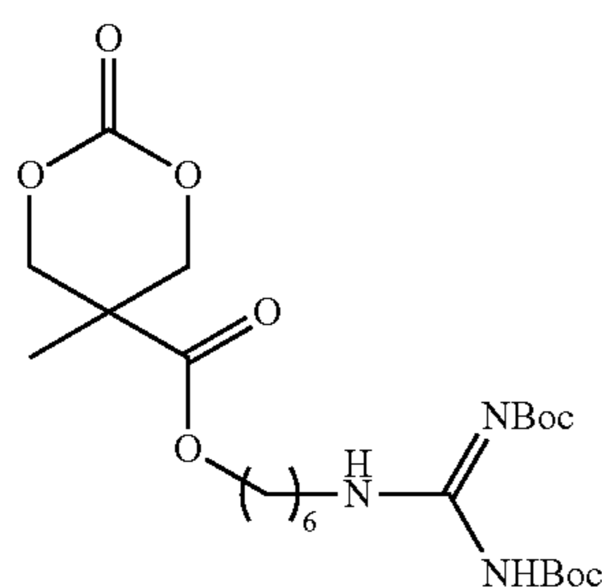
MTC-C6G1
