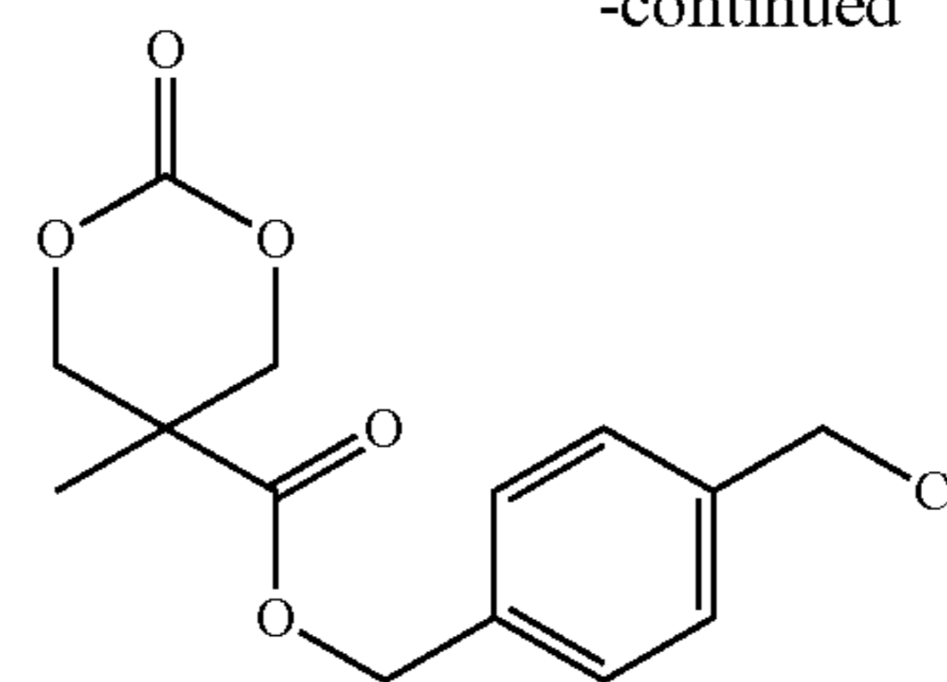
MTC-BnCl MW 298.7
