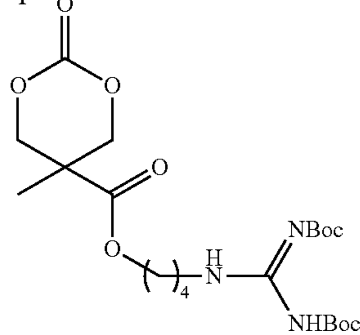
MTC-C4G1
