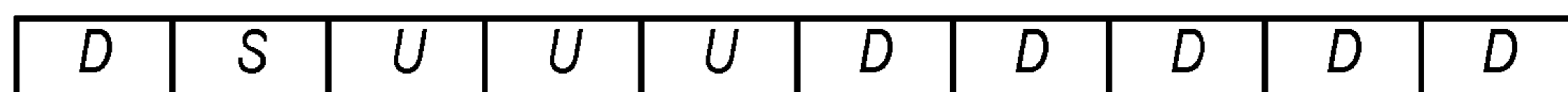
TDD Configuration 3
