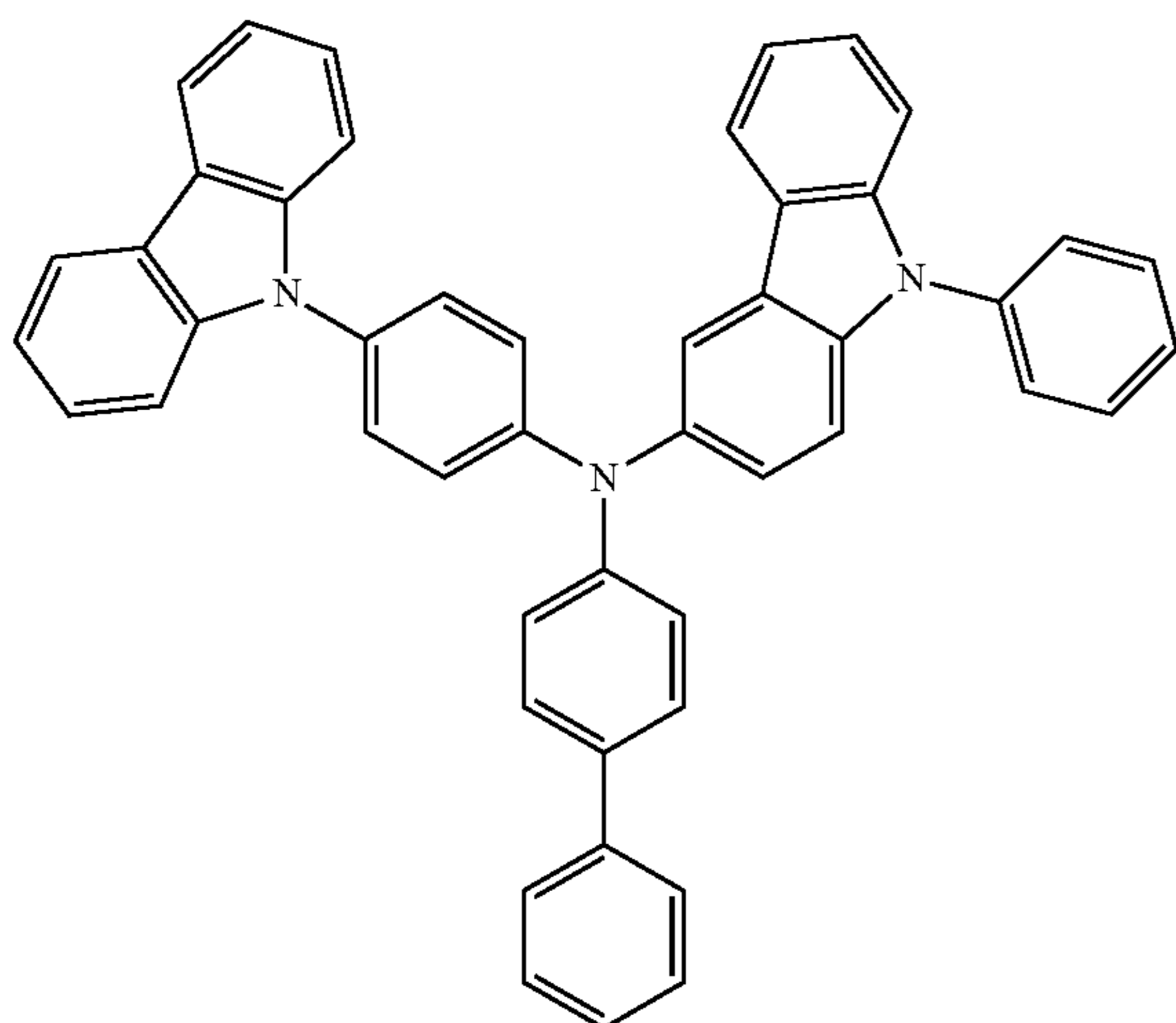
[Chemical Formula 1]
