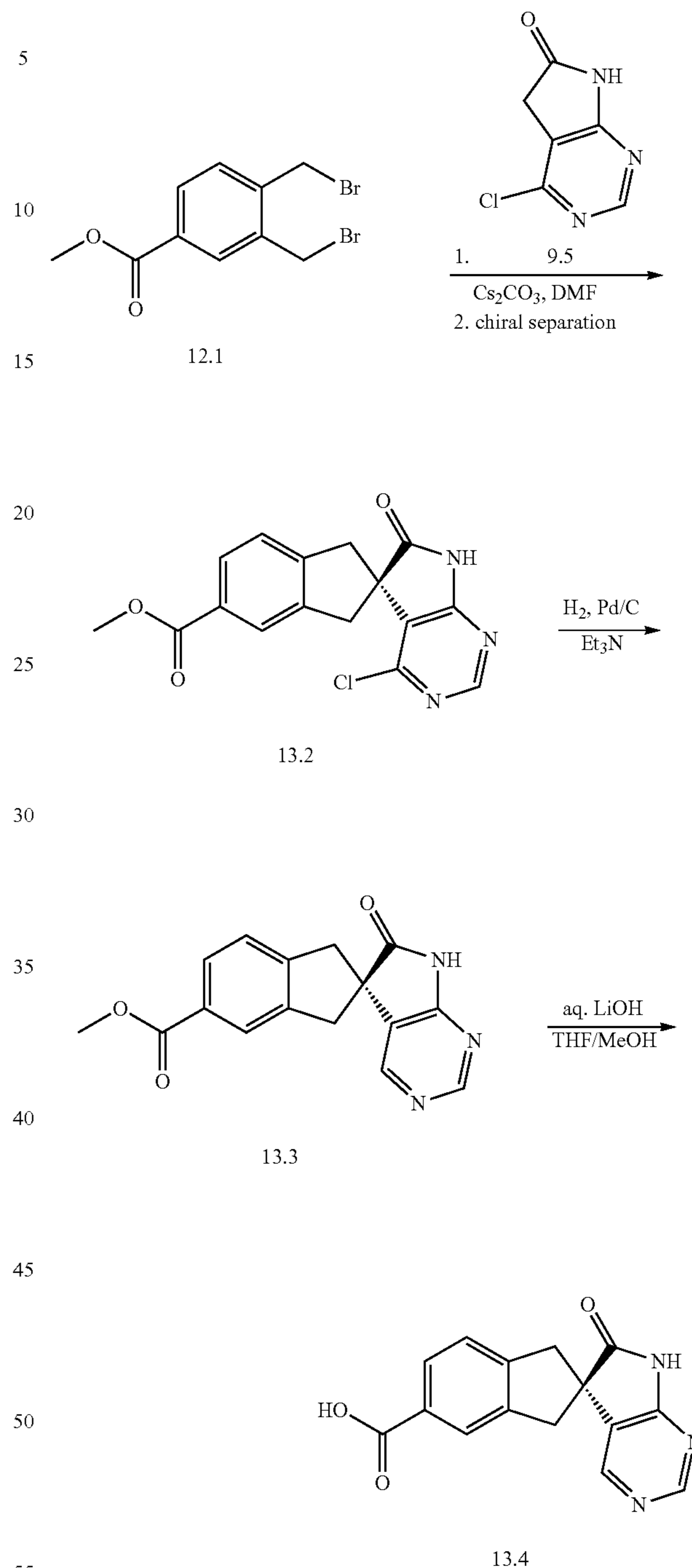
SCHEME 13
