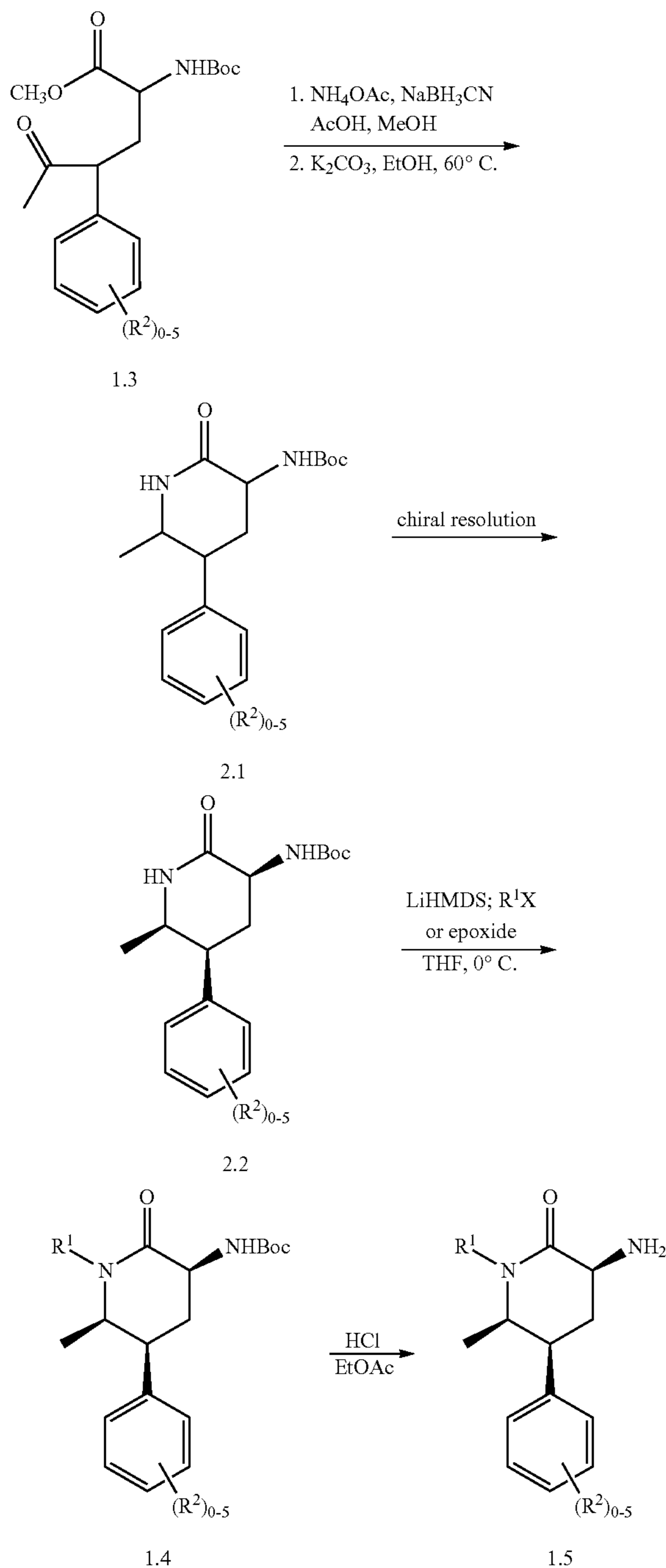
SCHEME 2
