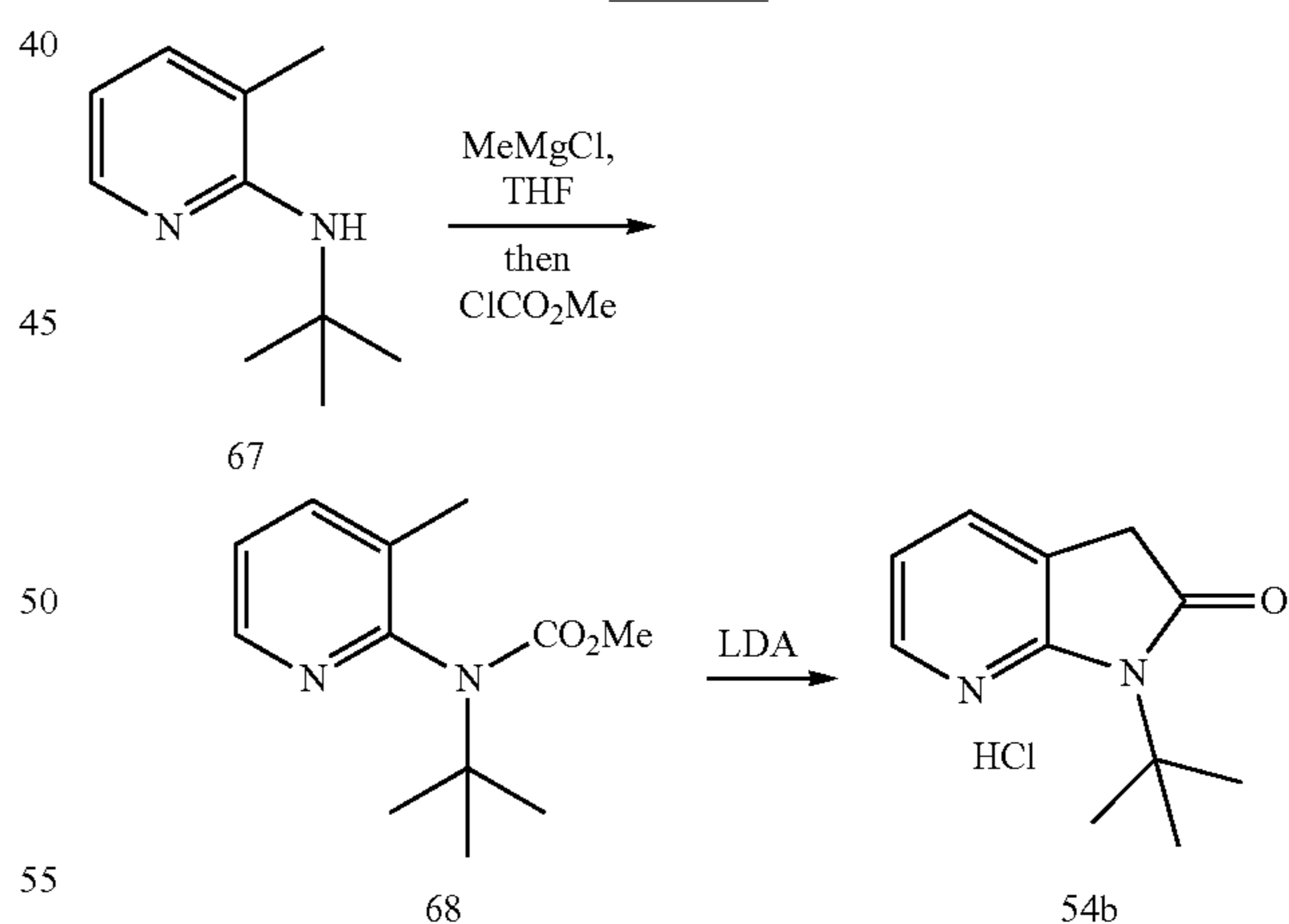
Methyl tert-butyl(3-methylpyridin-2-yl)carbamate (68)
