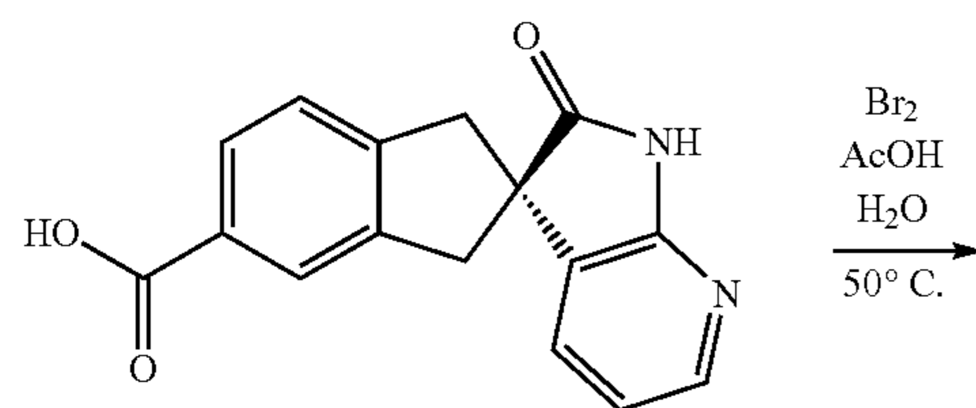
SCHEME 14
