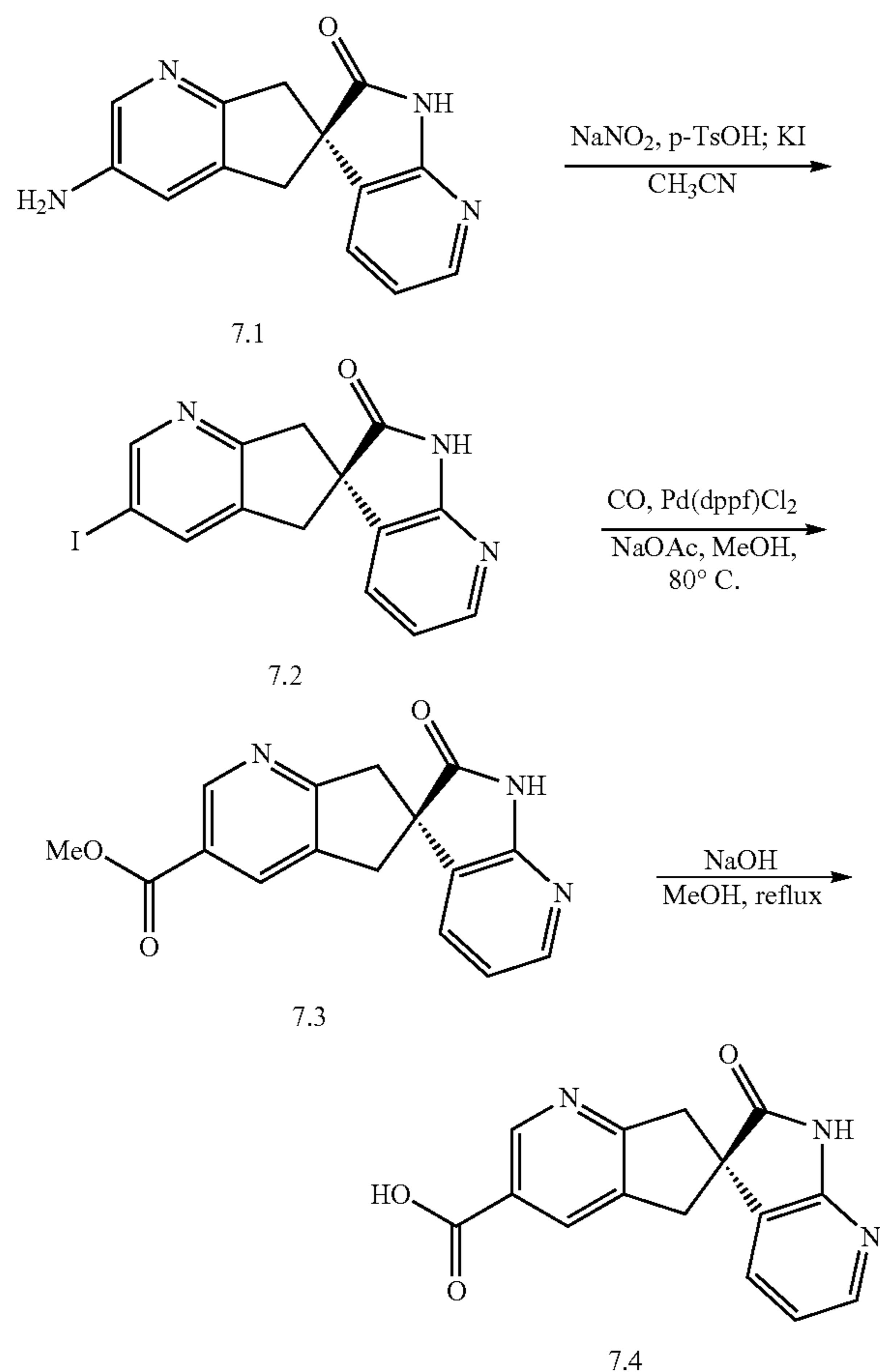
SCHEME 7
