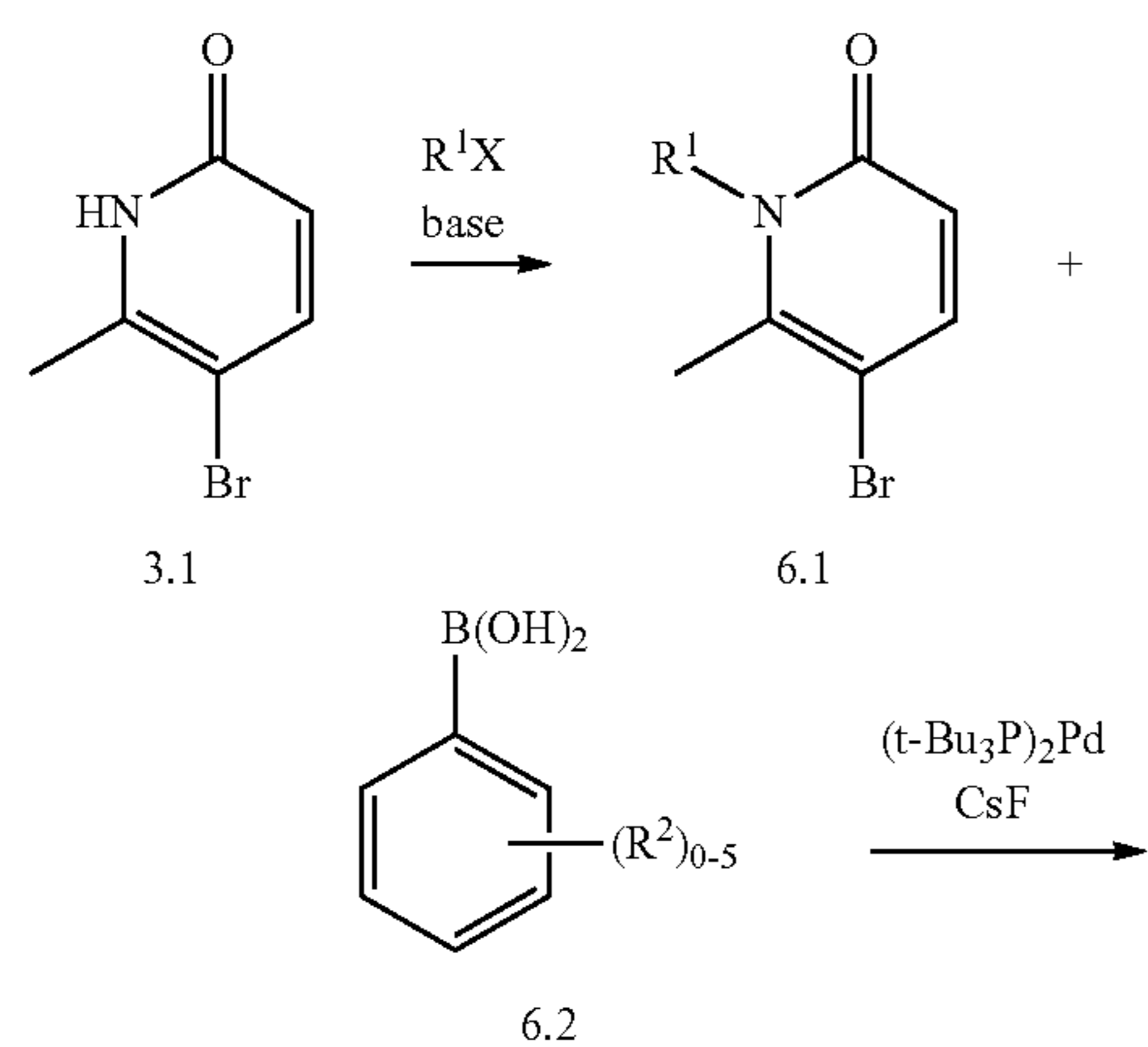
SCHEME 6
