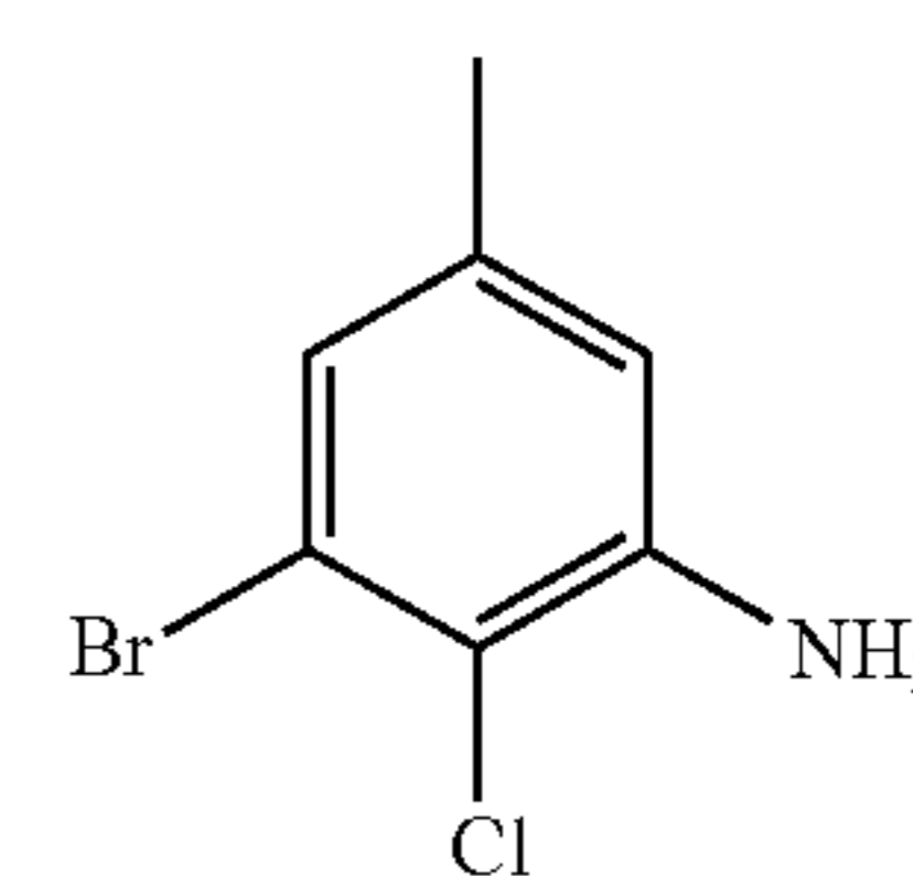
3-bromo-2-chloro-5-methylaniline
