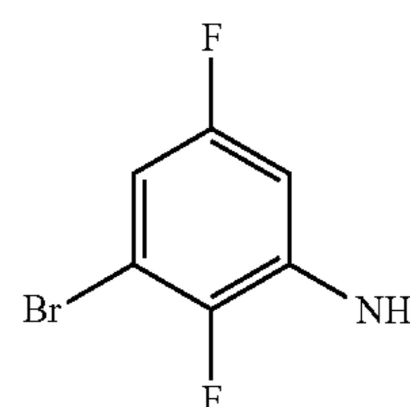
3-bromo-2,5-difluoroaniline
