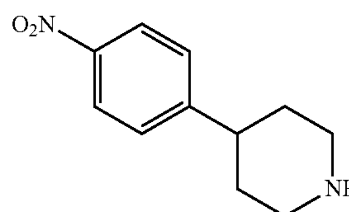
4-(4-Nitrophenyl)piperidine (NT1-001)
