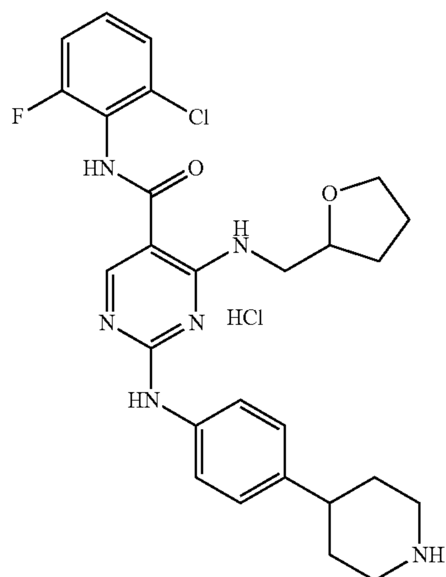
N-(2-chloro-6-fluorophenyl)-2-(4-(piperidin-4-yl)phenylamino)-4-((tetrahydrofuran-2-yl)methylamino)pyrimidine-5-carboxamide (DZ1-089)
