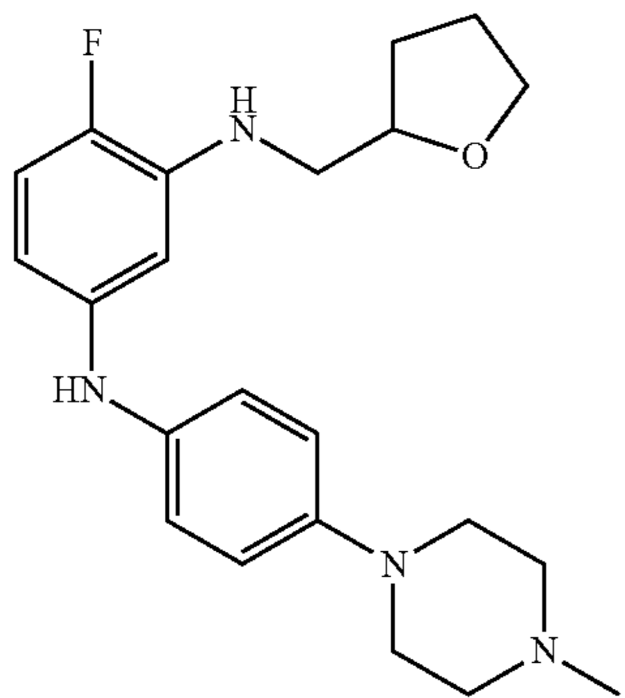
5-fluoro-N2-(4-(4-methylpiperazin-1-yl)phenyl)-N4-((tetrahydrofuran-2-yl)methyl)pyrimidine-2,4-diamine (DZ1-098)
