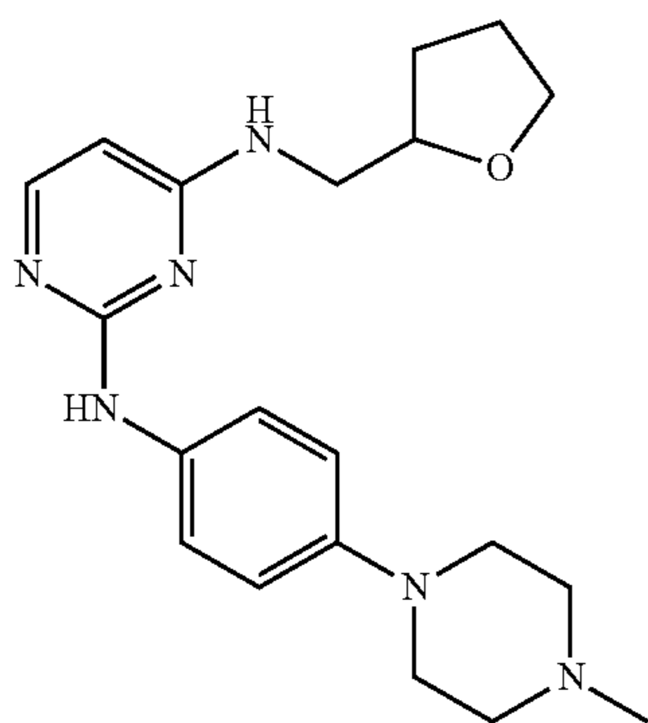
2-(4-(4-methylpiperazin-1-yl)benzyl)-N-((tetrahydrofuran-2-yl)methyl)pyrimidin-4-amine (DZ1-104)
