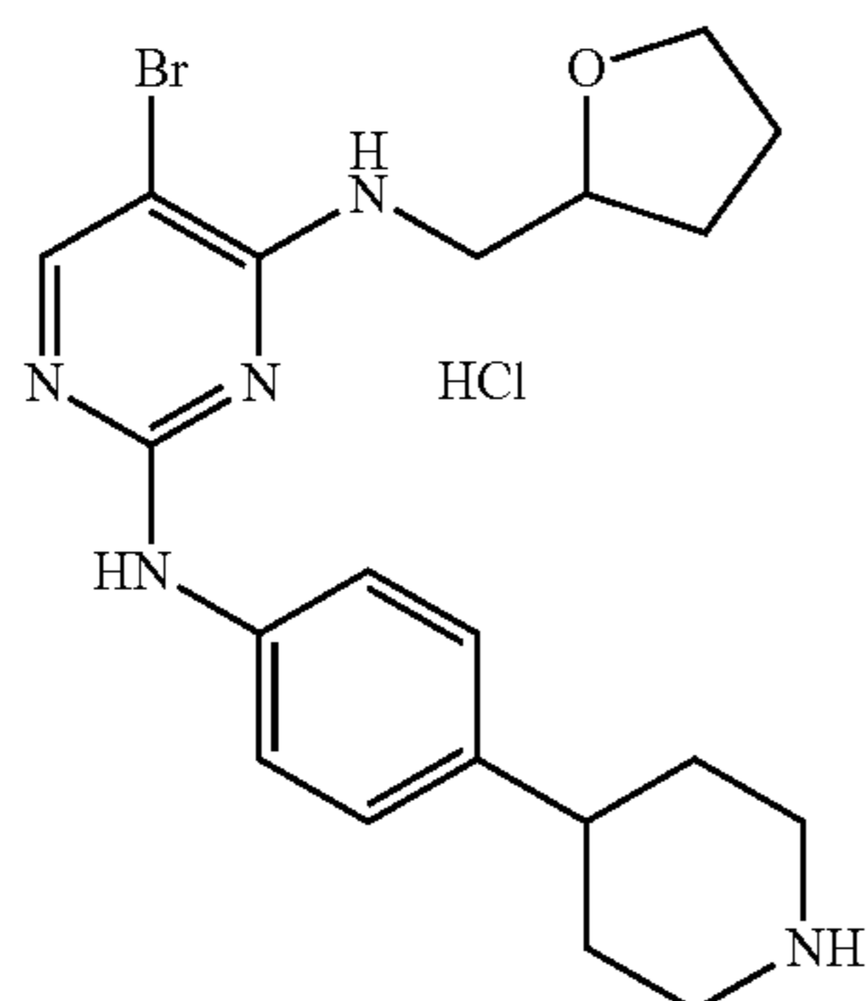
5-bromo-N2-(4-(piperidin-4-yl)phenyl)-N4-((tetrahydrofuran-2-yl)methyl)pyrimidine-2,4-diamine (DZ1-088)
