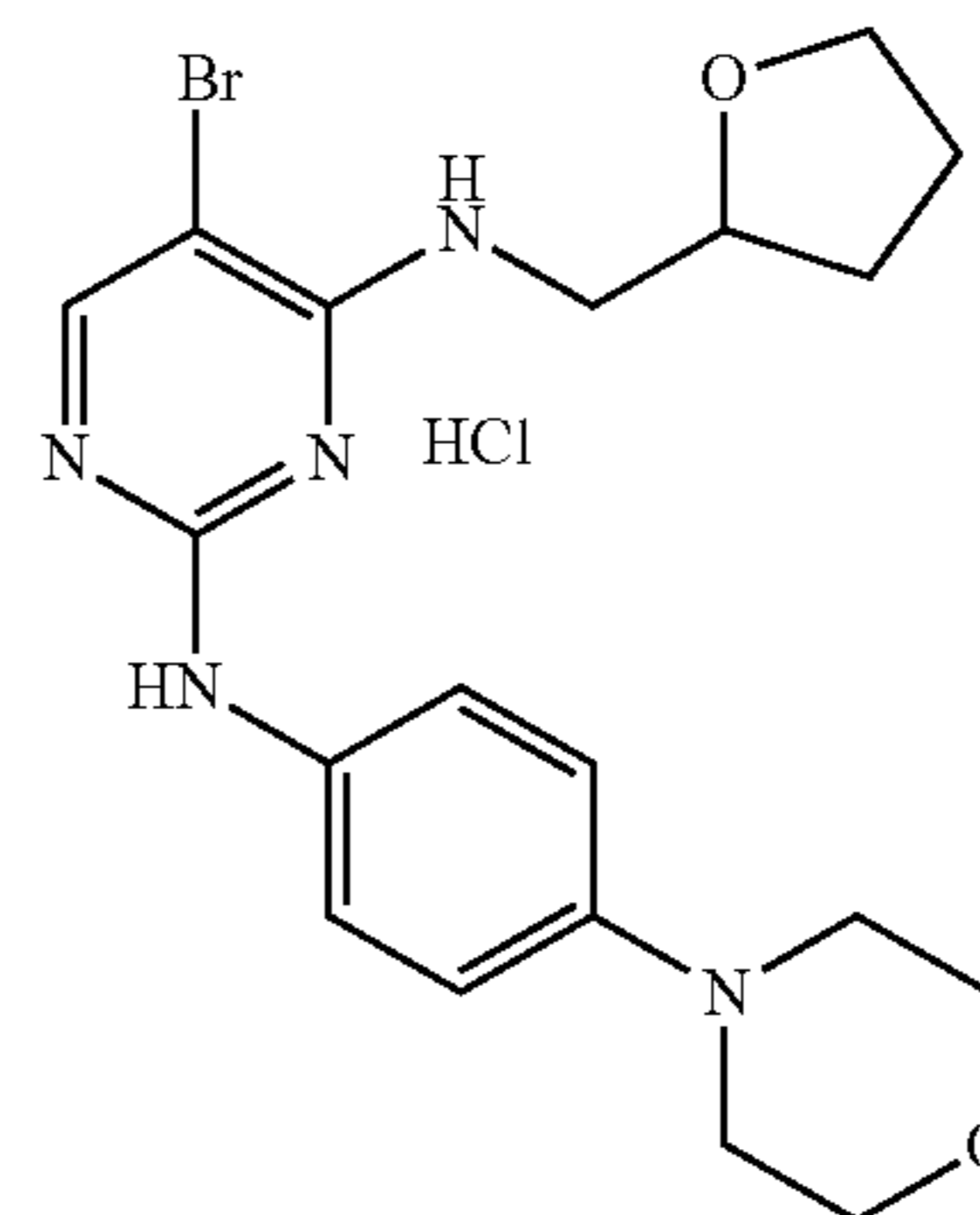
5-bromo-N2-(4-morpholinophenyl)-N4-((tetrahydrofuran-2-yl)methyl)pyrimidine-2,4-diamine (DZ1-091)
