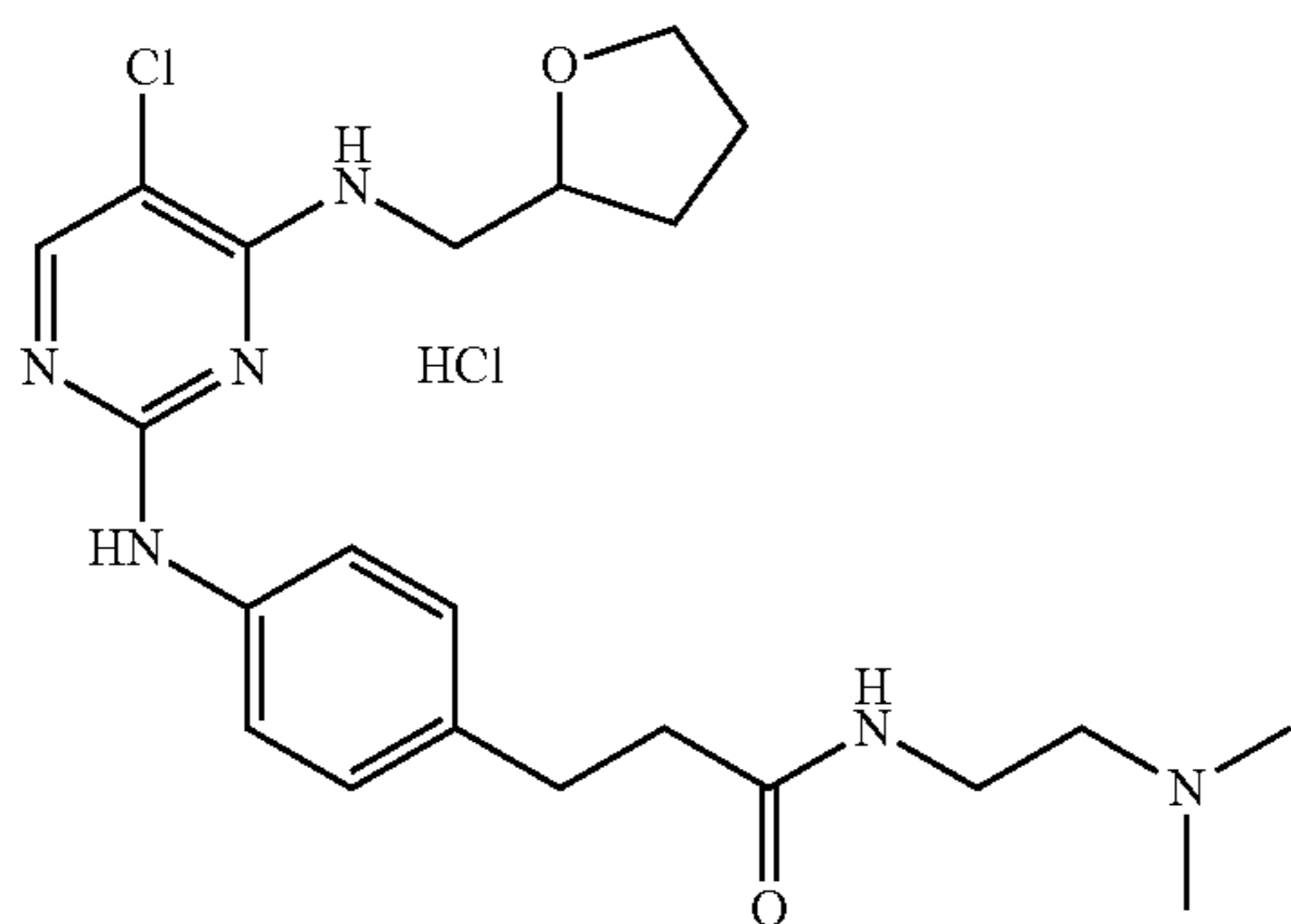
3-(4-(5-Chloro-4-((tetrahydrofuran-2-yl)methylamino)pyrimidin-2-ylamino)phenyl)-N-(2-(dimethylamino)ethyl)propanamide (NT1-028)
