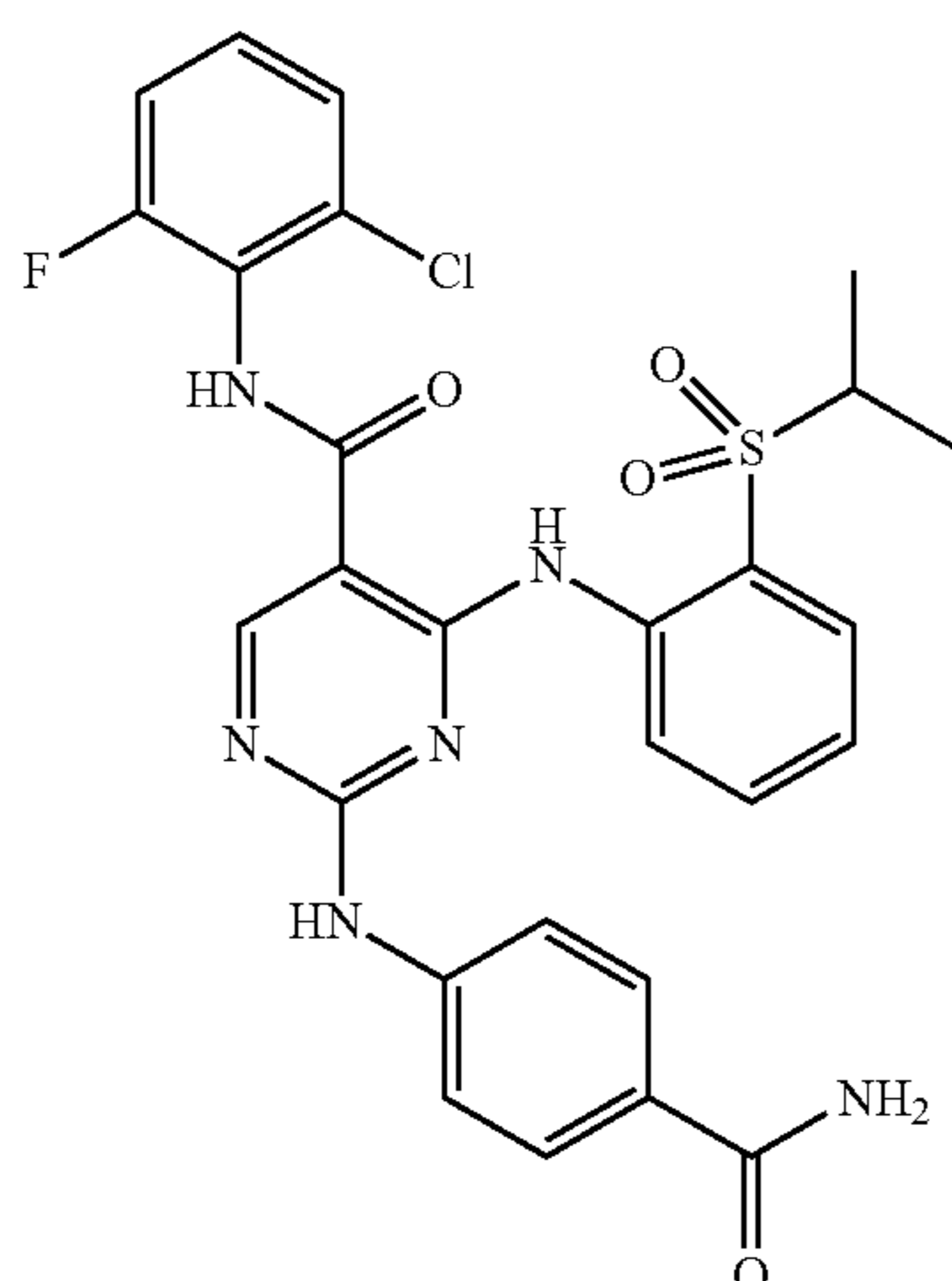
2-(4-Carbamoylphenylamino)-N-(2-chloro-6-fluorophenyl)-4-(2-(isopropylsulfonyl)phenylamino)pyrimidine-5-carboxamide (YL7-106-3)
