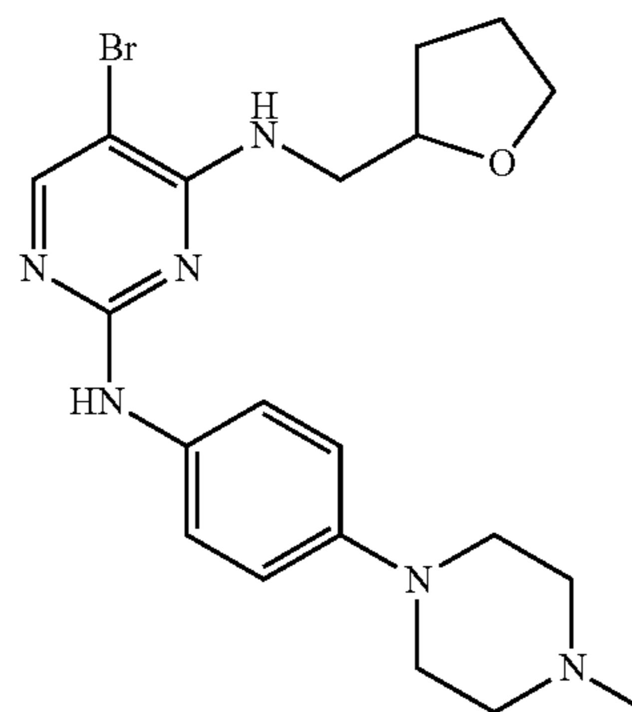
5-bromo-N2-(4-(4-methylpiperazin-1-yl)phenyl)-N4-((tetrahydrofuran-2-yl)methyl)pyrimidine-2,4-diamine (DZ1-122)
