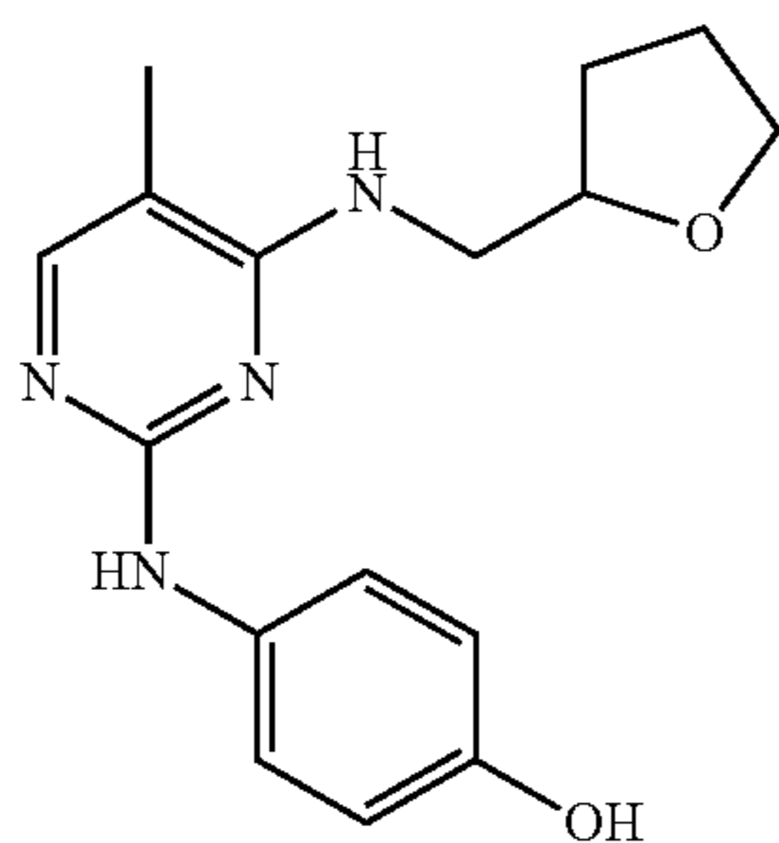
4-(5-methyl-4-((tetrahydrofuran-2-yl)methylamino)pyrimidin-2-ylamino)phenol (DZ1-116)
