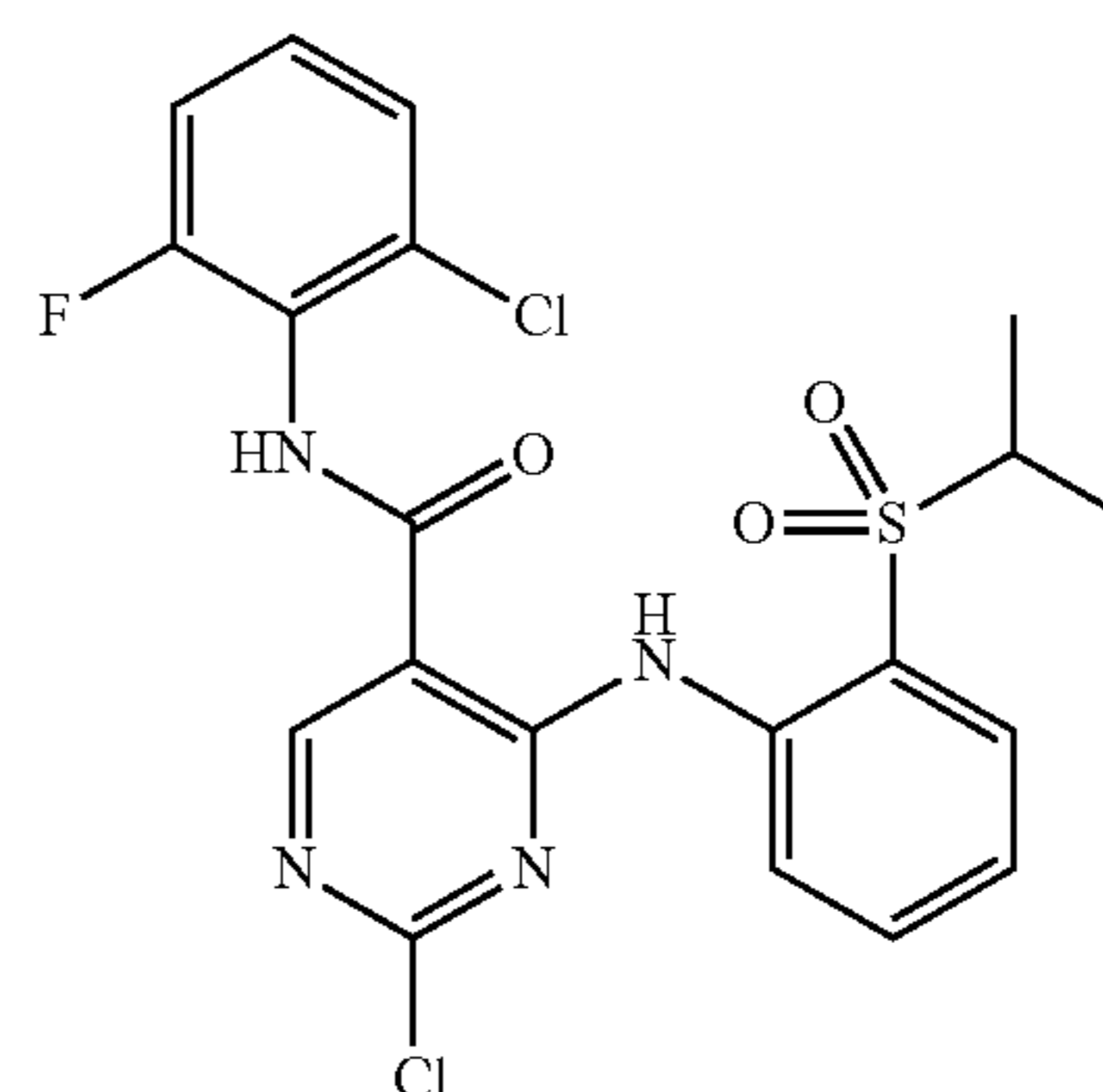
2-Chloro-N-(2-chloro-6-fluorophenyl)-4-(2-(isopropylsulfonyl)phenylamino)pyrimidine-5-carboxamide (YL7-041)
