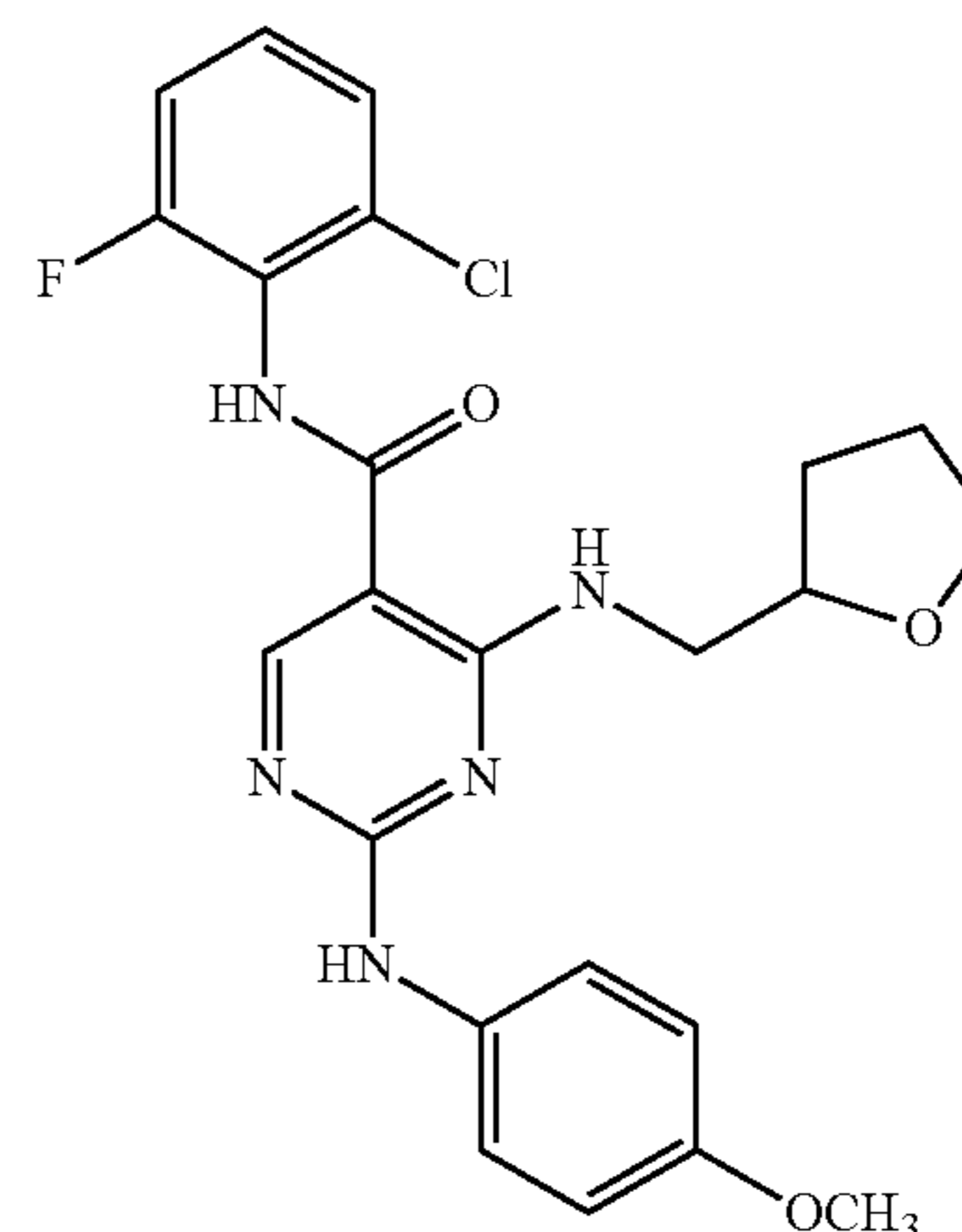
N-(2-chloro-6-fluorophenyl)-2-(4-methoxyphenylamino)-4-((tetrahydrofuran-2-yl)methylamino)pyrimidine-5-carboxamide (YL7-104-1)
