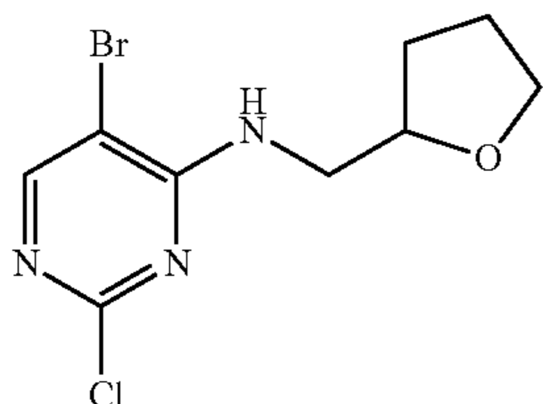
5-Bromo-2-chloro-N-((tetrahydrofuran-2-yl)methyl)pyrimidin-4-amine (SK1-008-B2 8b, Scheme 3)
