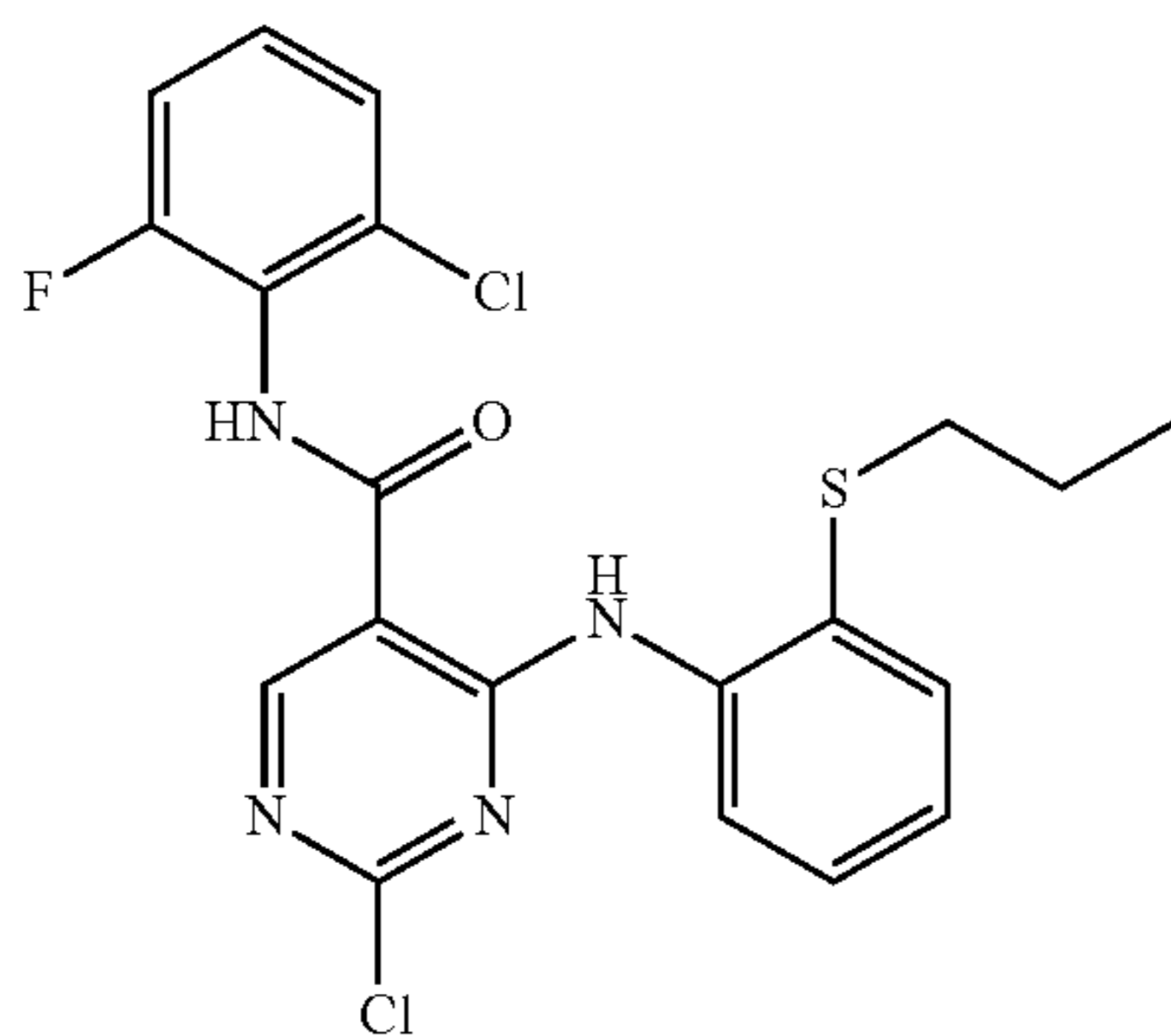
2-Chloro-N-(2-chloro-6-fluorophenyl)-4-(2-(propylthio)phenylamino)pyrimidine-5-carboxamide (YL7-051)
