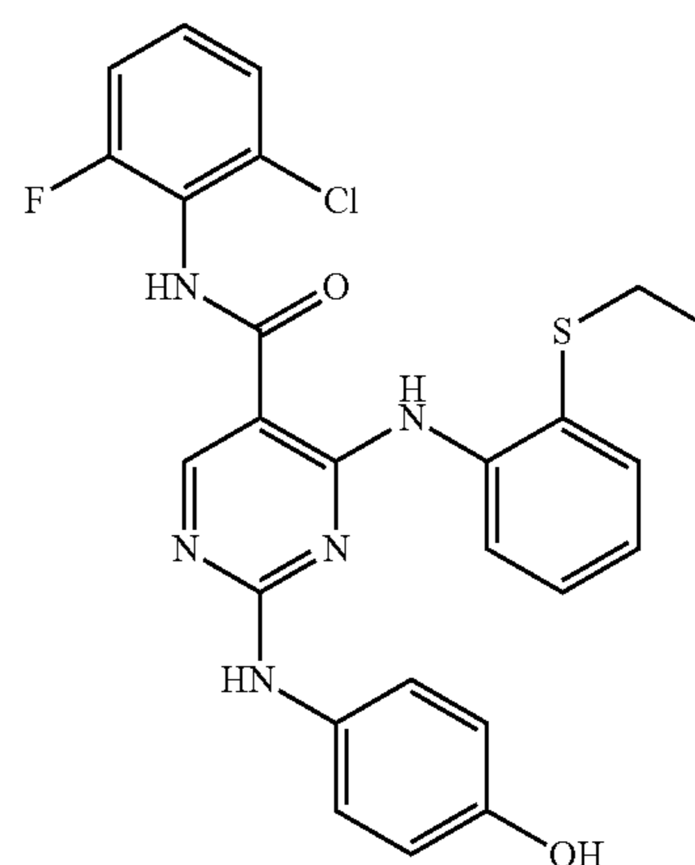
N-(2-chloro-6-fluorophenyl)-4-(2-(ethylthio)phenylamino)-2-(4-hydroxyphenylamino)pyrimidine-5-carboxamide (YL7-058-4)
