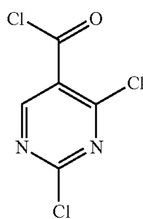
2,4-Dichloropyrimidine-5-carbonyl chloride (PE1-028-B2, Scheme 1)
