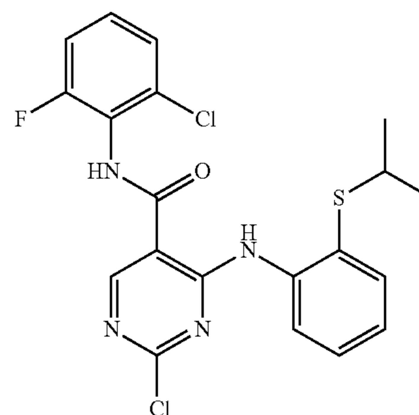
2-Chloro-N-(2-chloro-6-fluorophenyl)-4-(2-(isopropylthio)phenylamino)pyrimidine-5-carboxamide (YL7-040)
