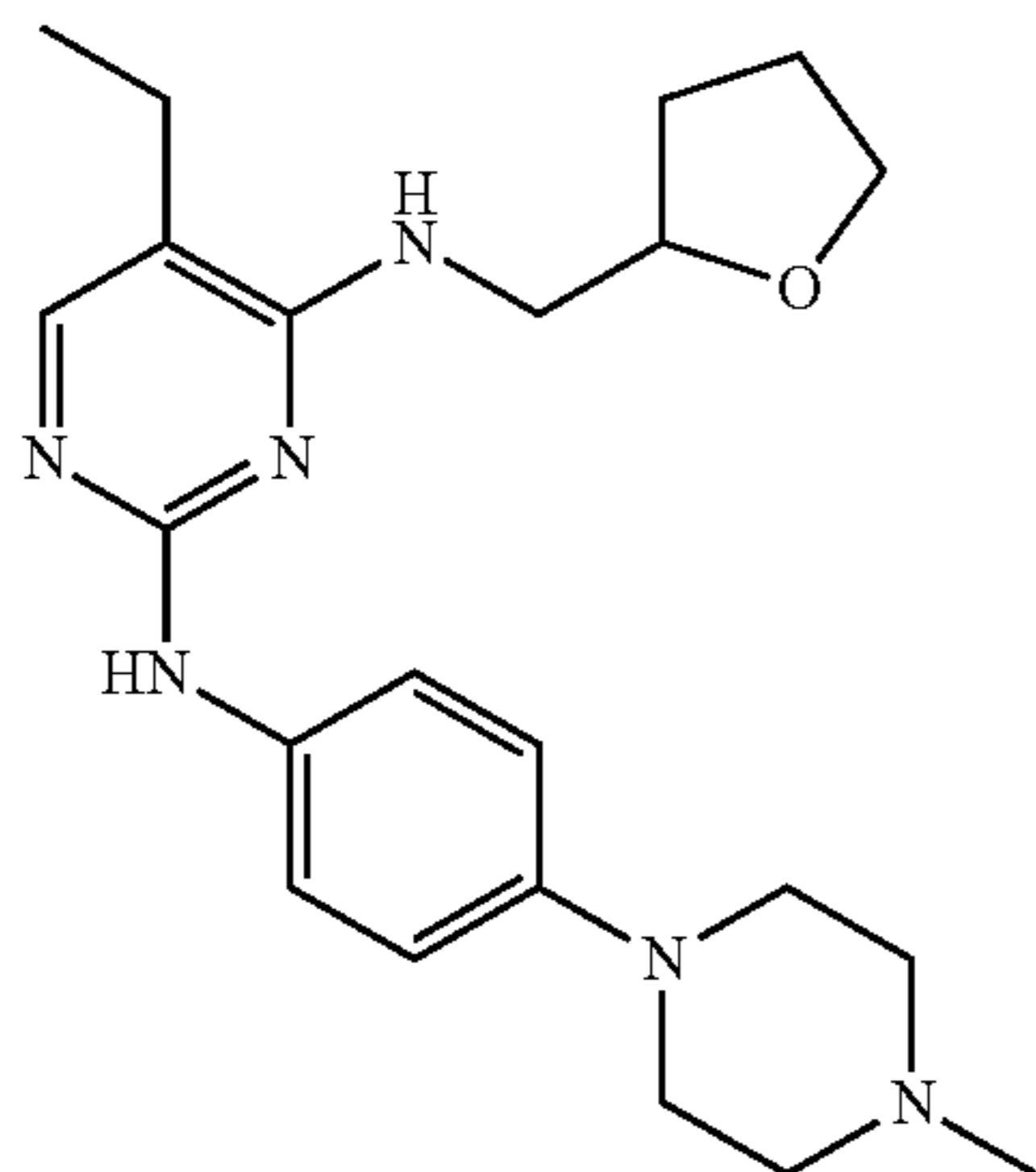
5-ethyl-N2-(4-(4-methylpiperazin-1-yl)phenyl)-N4-((tetrahydrofuran-2-yl)methyl)pyrimidine-2,4-diamine (DZ1-108)
