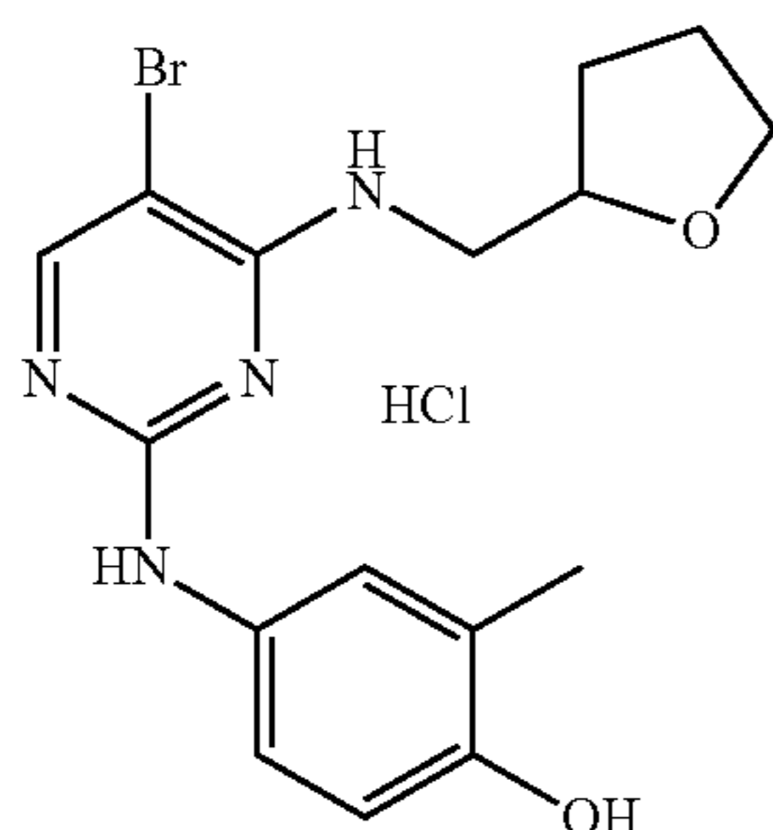
4-(5-bromo-4-((tetrahydrofuran-2-yl)methyl)amino)pyrimidin-2-ylamino)-2-methylphenol (SK1-040)
