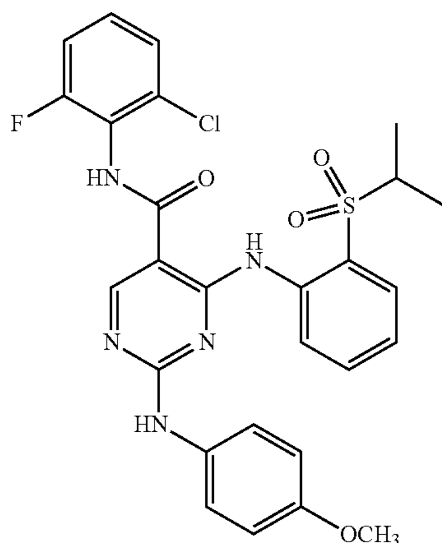
N-(2-chloro-6-fluorophenyl)-4-(2-(isopropylsulfonyl)phenylamino)-2-(4-methoxyphenylamino)pyrimidine-5-carboxamide (YL7-045-1)
