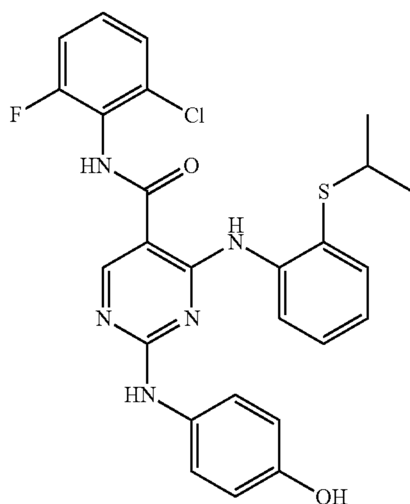
N-(2-chloro-6-fluorophenyl)-2-(4-hydroxyphenylamino)-4-(2-(isopropylthio)phenylamino)pyrimidine-5-carboxamide (YL7-045-4)
