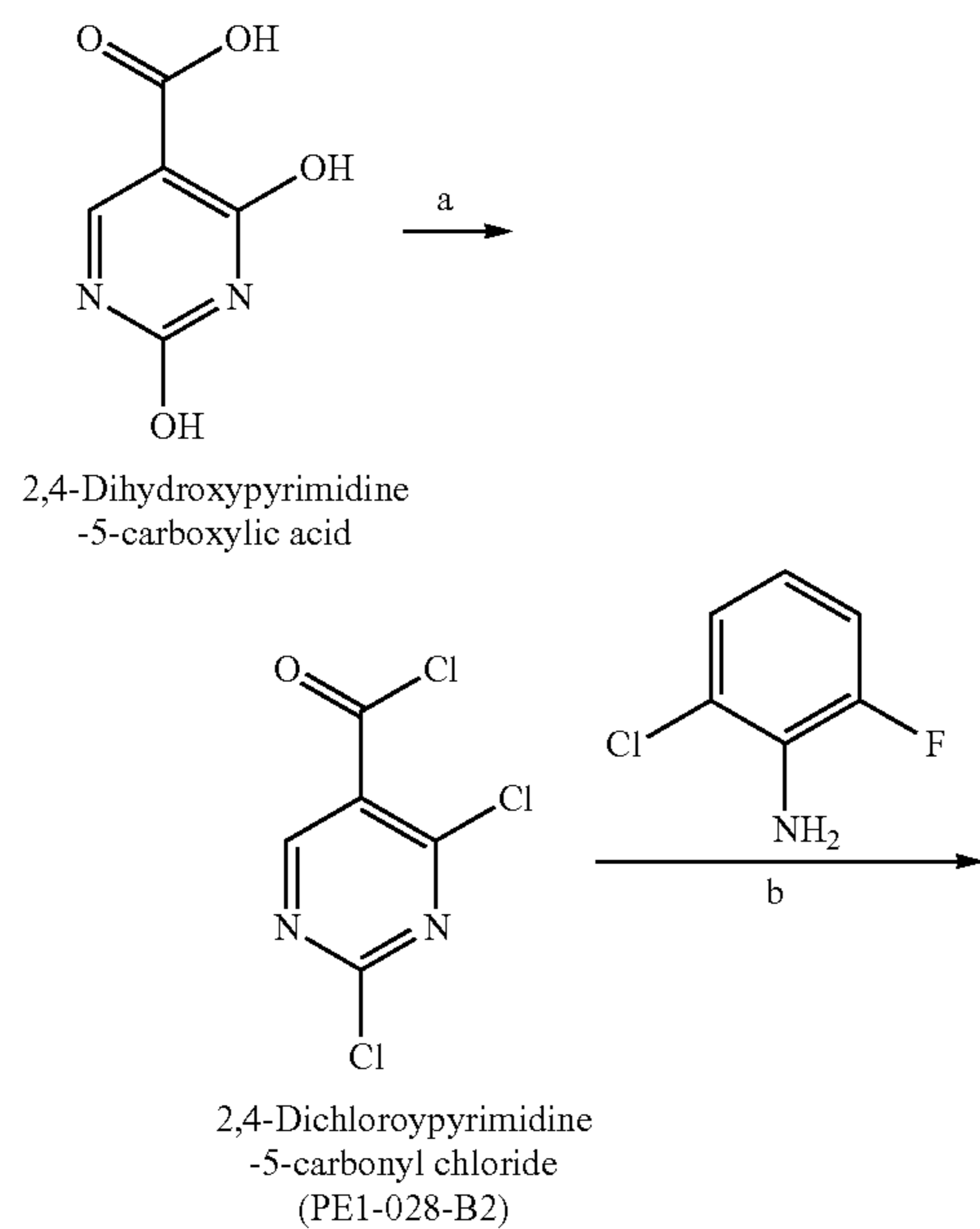
Scheme 1: Synthesis of building block 7c for library synthesis.
