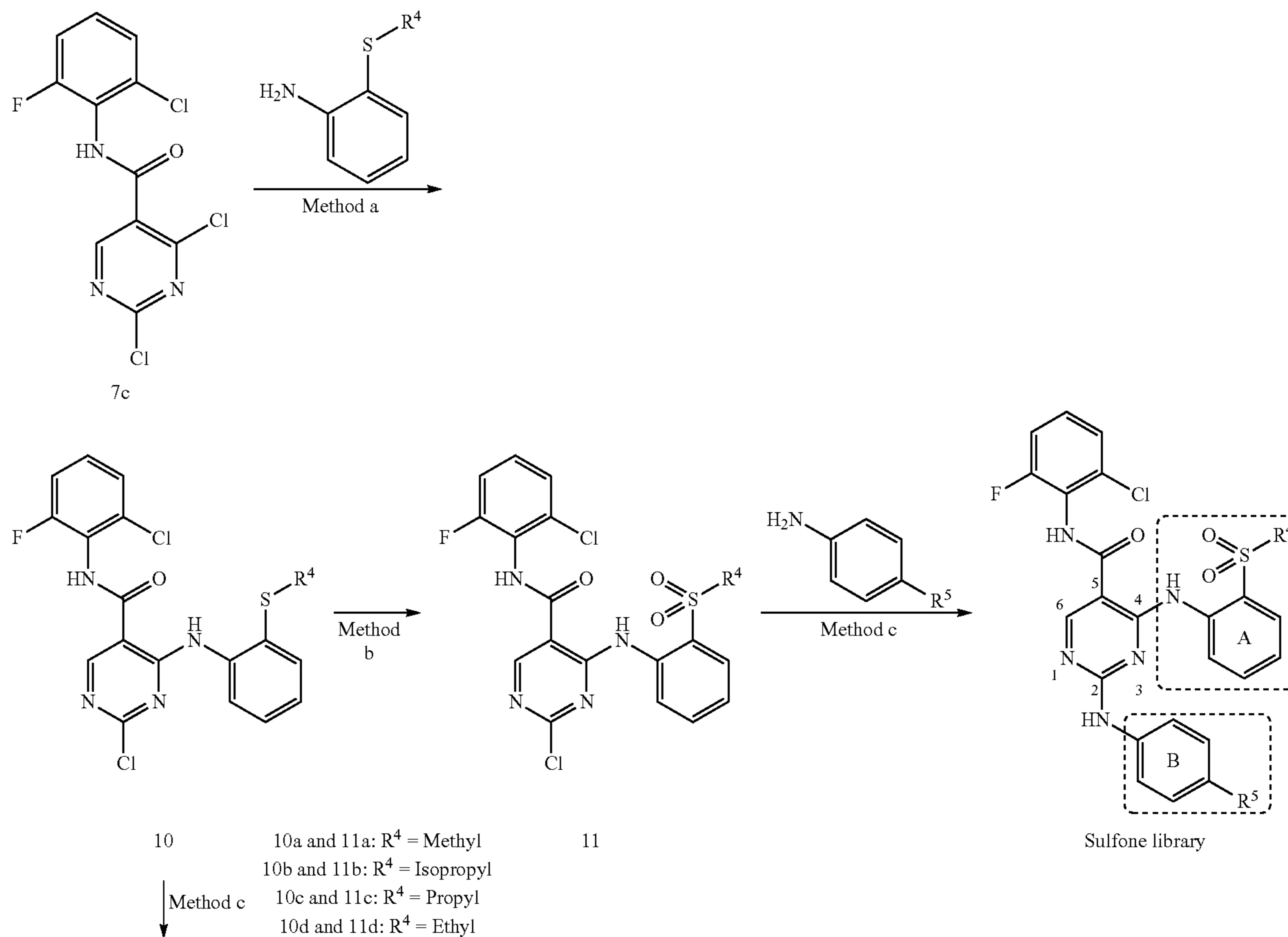
Scheme 2 Synthesis of bisanilinopyrimidine libraries with sulfon-substituted A-ring. And sulfide-substituted A ring
