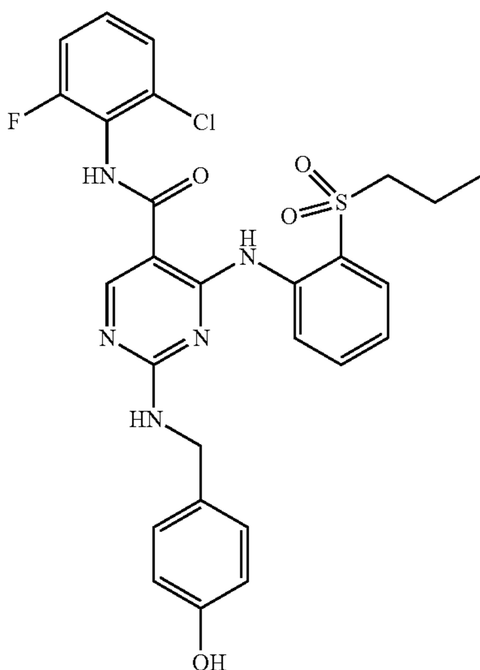
N-(2-chloro-6-fluorophenyl)-4-(2-(isopropylsulfonyl)phenylamino)-2-(4-sulfamoylphenylamino)pyrimidine-5-carboxamide (YL7-109)
