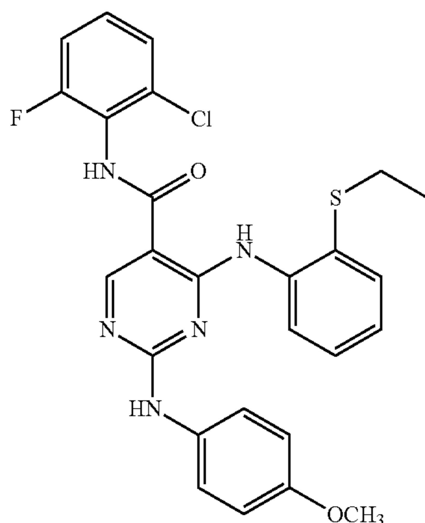
N-(2-chloro-6-fluorophenyl)-4-(2-(ethylthio)phenylamino)-2-(4-methoxyphenylamino)pyrimidine-5-carboxamide (YL7-058-3)
