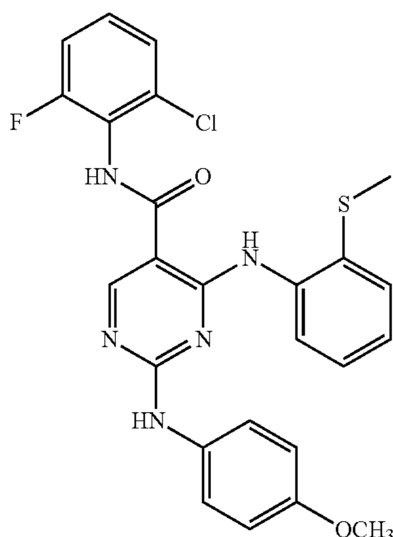
N-(2-chloro-6-fluorophenyl)-2-(4-methoxyphenylamino)-4-(2-(methylthio)phenylamino)pyrimidine-5-carboxamide (YL7-039-1)
