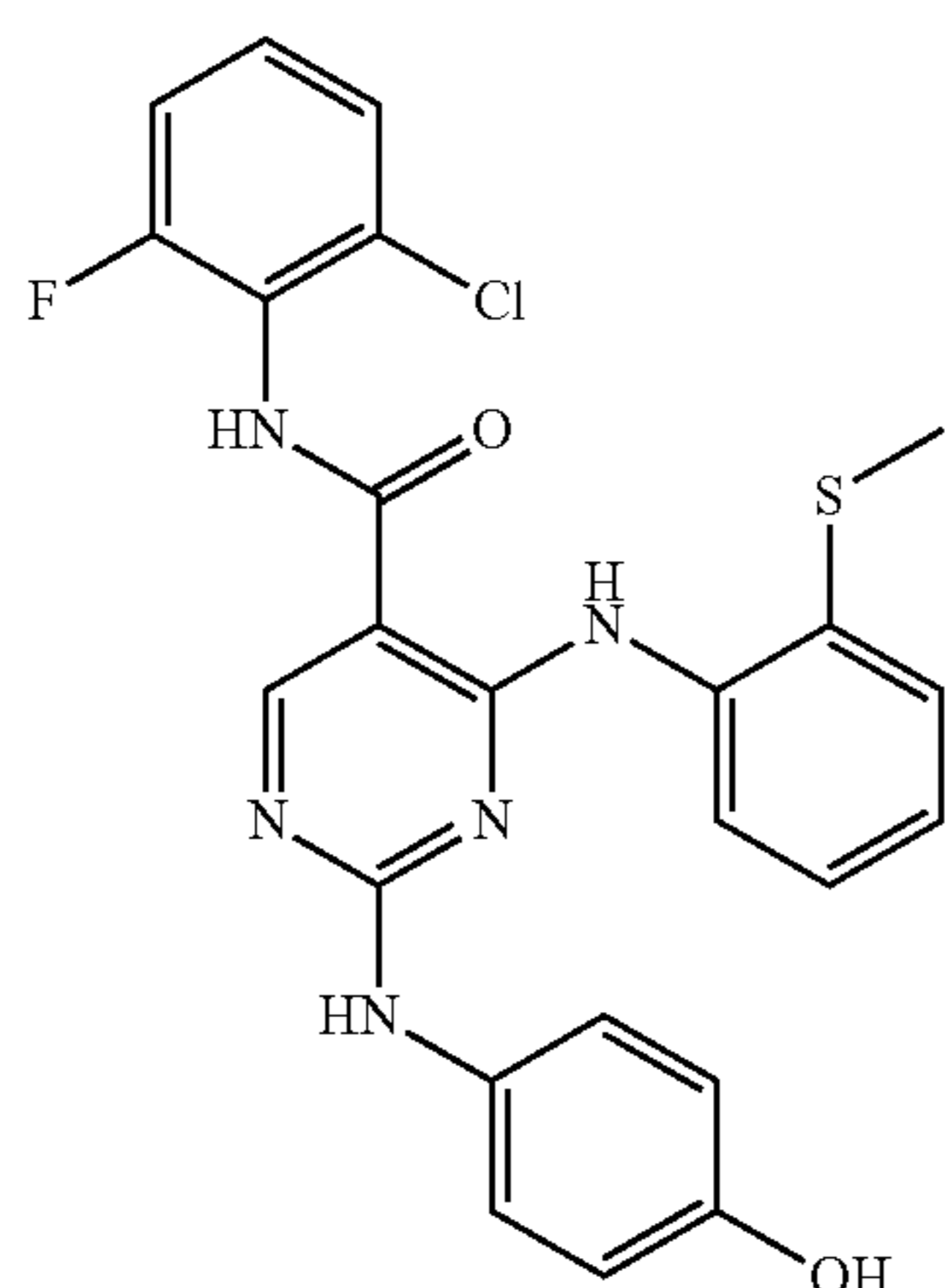
N-(2-chloro-6-fluorophenyl)-2-(4-hydroxyphenylamino)-4-(2-(methylthio)phenylamino)pyrimidine-5-carboxamide (YL7-039-2)
