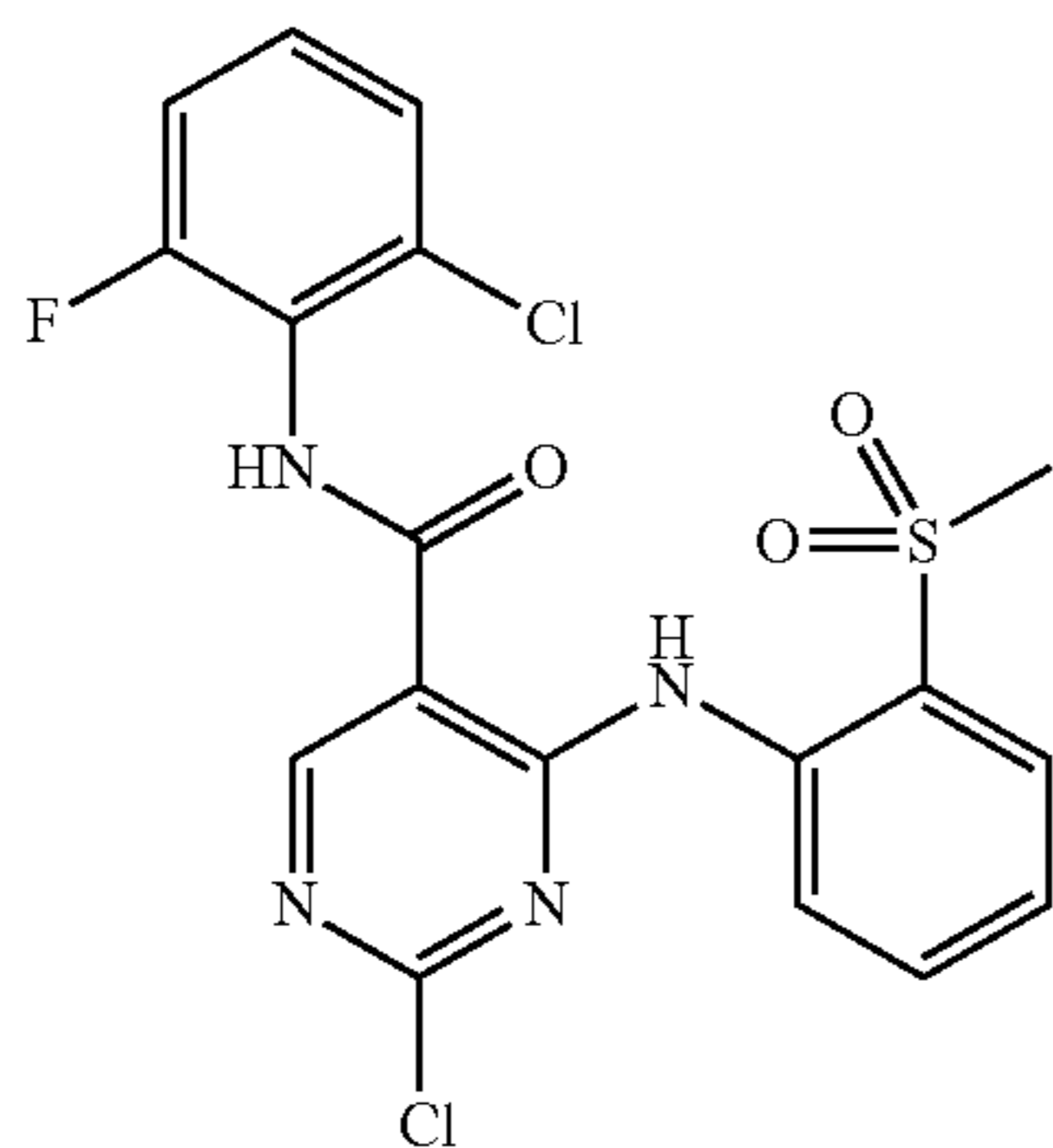
2-Chloro-N-(2-chloro-6-fluorophenyl)-4-(2-(methylsulfonyl)phenylamino)pyrimidine-5-carboxamide (YL7-034)
