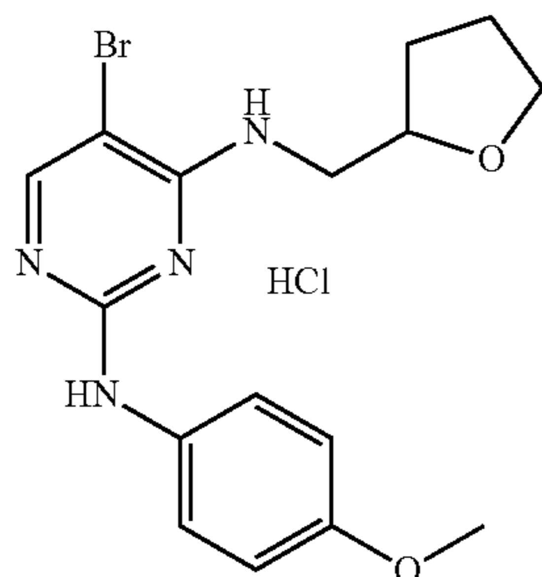
5-Bromo-N2-(4-methoxyphenyl)-N4-((tetrahydrofuran-2-yl)methyl)pyrimidin-2,4-diamine (SK1-022)
