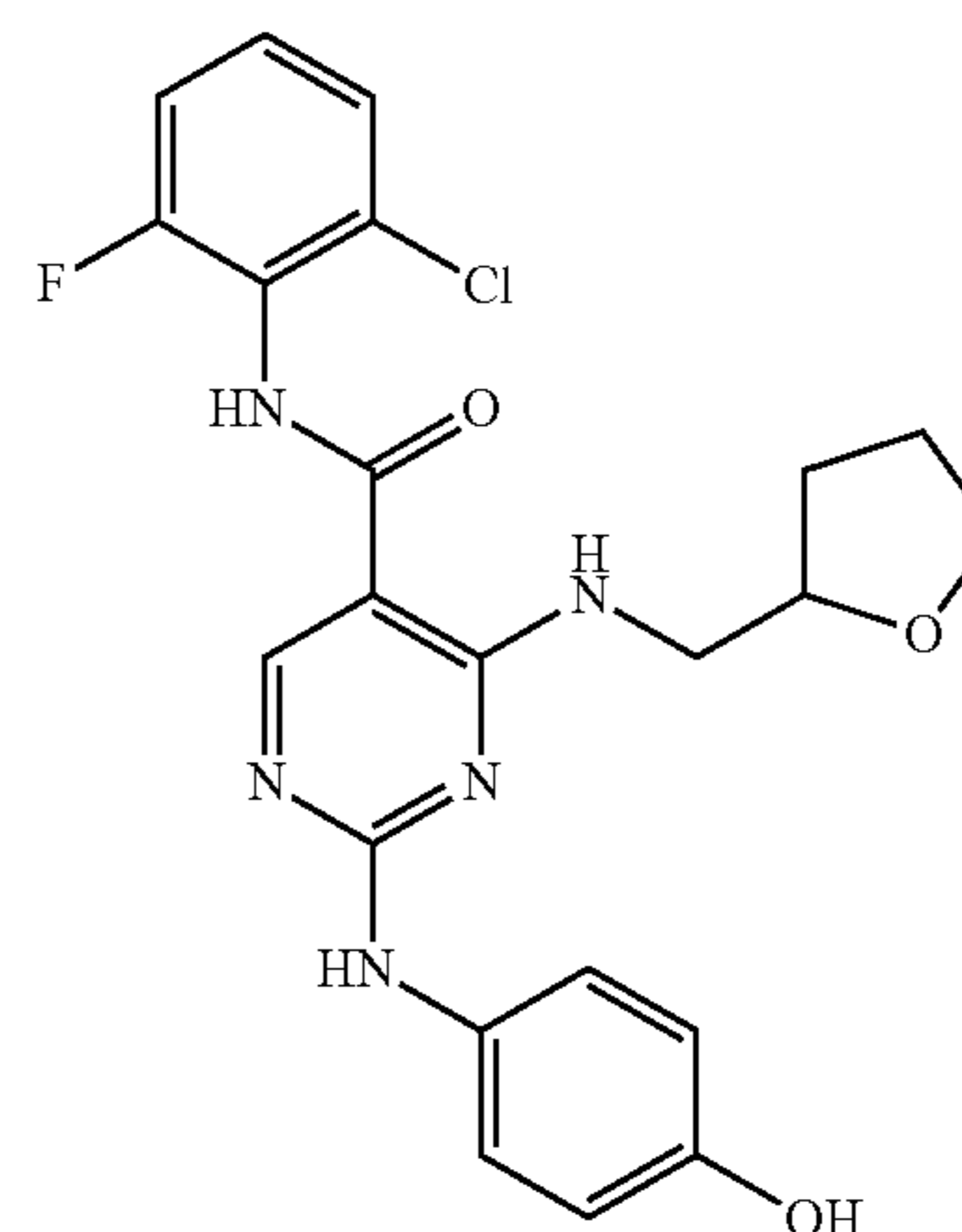
N-(2-chloro-6-fluorophenyl)-2-(4-hydroxyphenylamino)-4-((tetrahydrofuran-2-yl)methylamino)pyrimidine-5-carboxamide (YL7-104-2)
