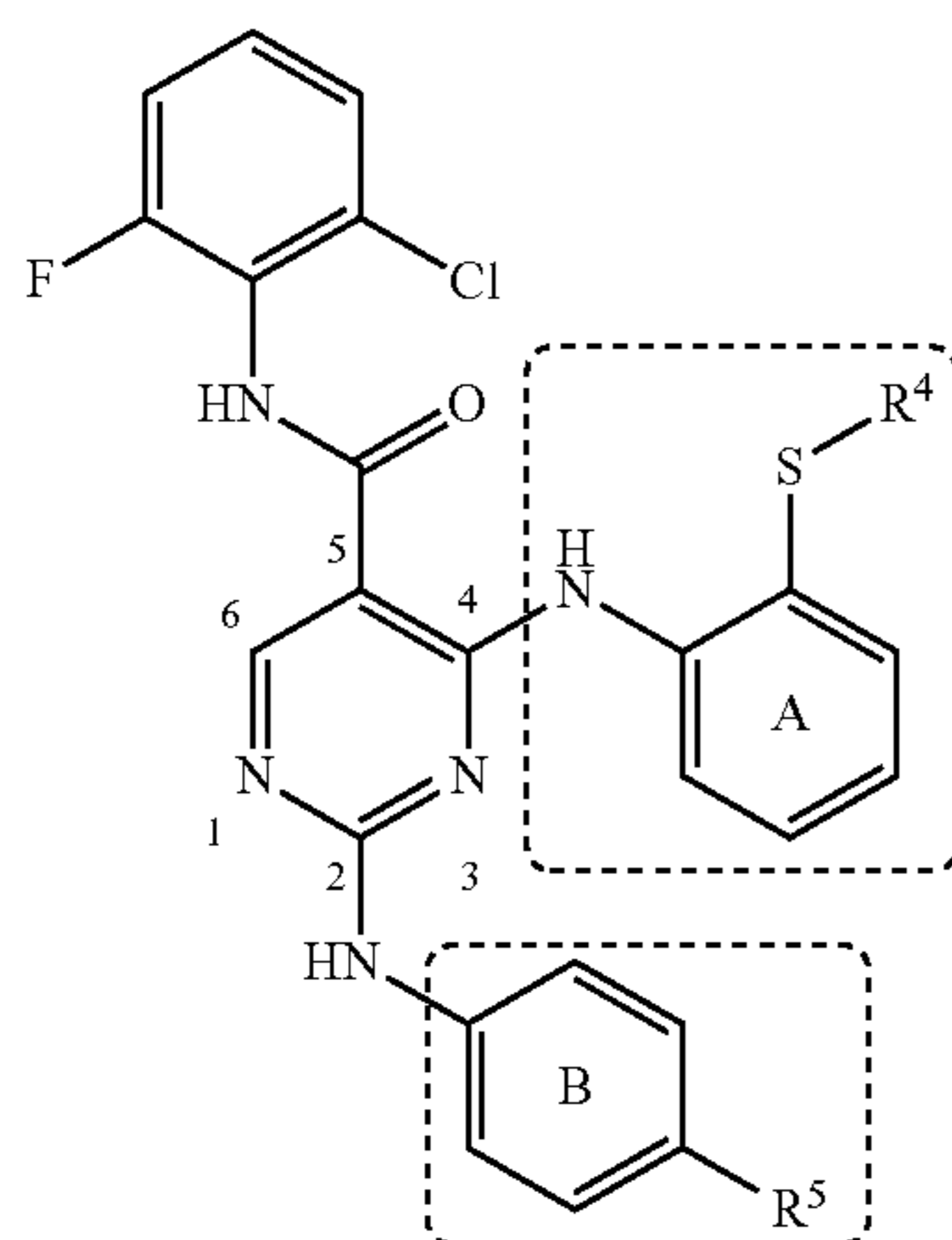
Sulfide library
