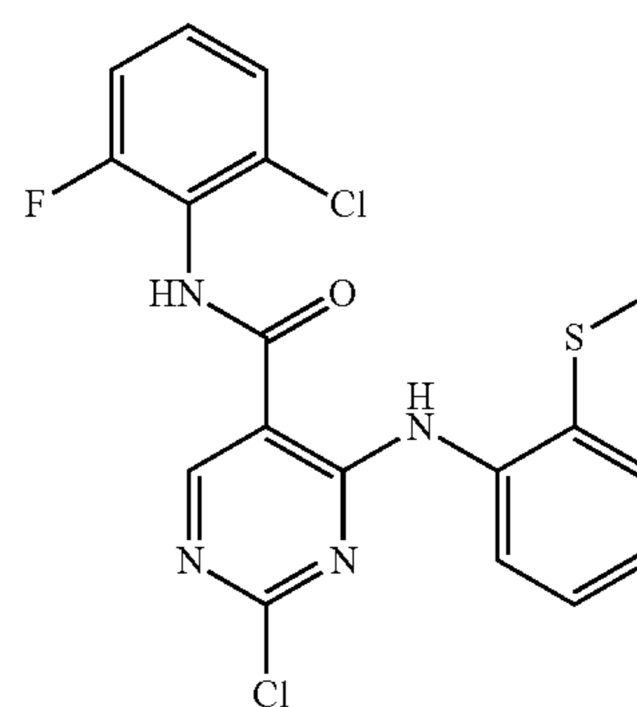
2-Chloro-N-(2-chloro-6-fluorophenyl)-4-(2-(methylthio)phenylamino)pyrimidine-5-carboxamide (YL7-031-B2)
