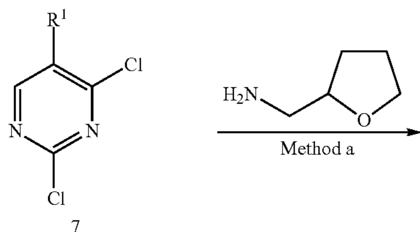
Scheme 5:
