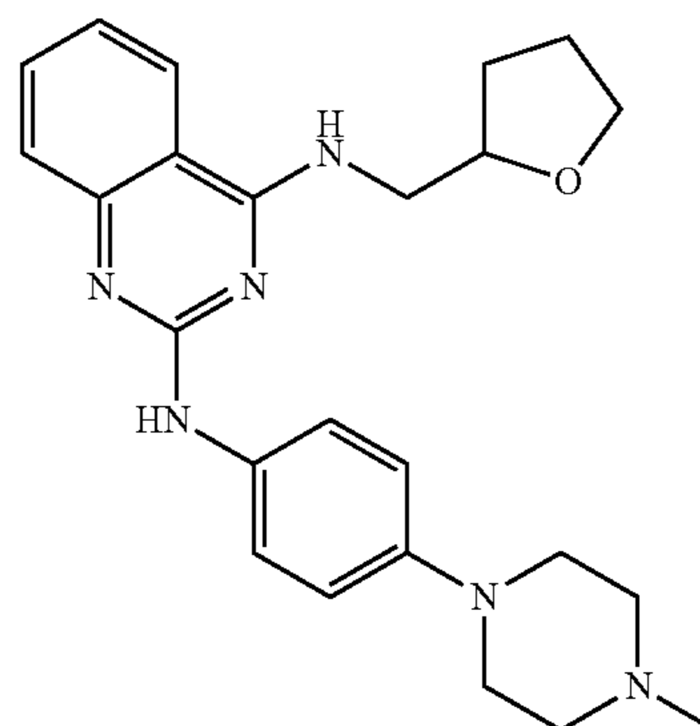
N2-(4-(4-methylpiperazin-1-yl)phenyl)-N4-((tetrahydrofuran-2-yl)methyl)quinazoline-2,4-diamine (DZ1-106)
