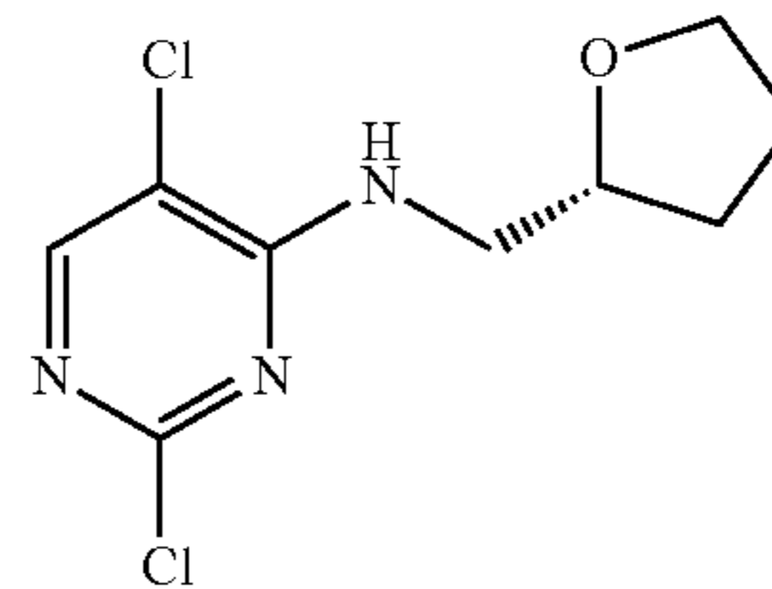
(R)-2,5-dichloro-N-((tetrahydrofuran-2-yl)methyl)pyrimidin-4-amine (DZ1-061, Scheme 4)
