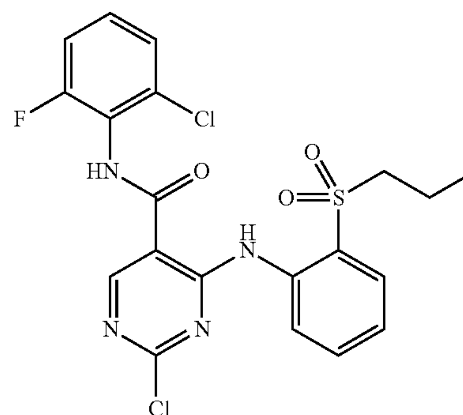
2-Chloro-N-(2-chloro-6-fluorophenyl)-4-(2-(propylsulfonyl)phenylamino)pyrimidine-5-carboxamide (YL7-052)
