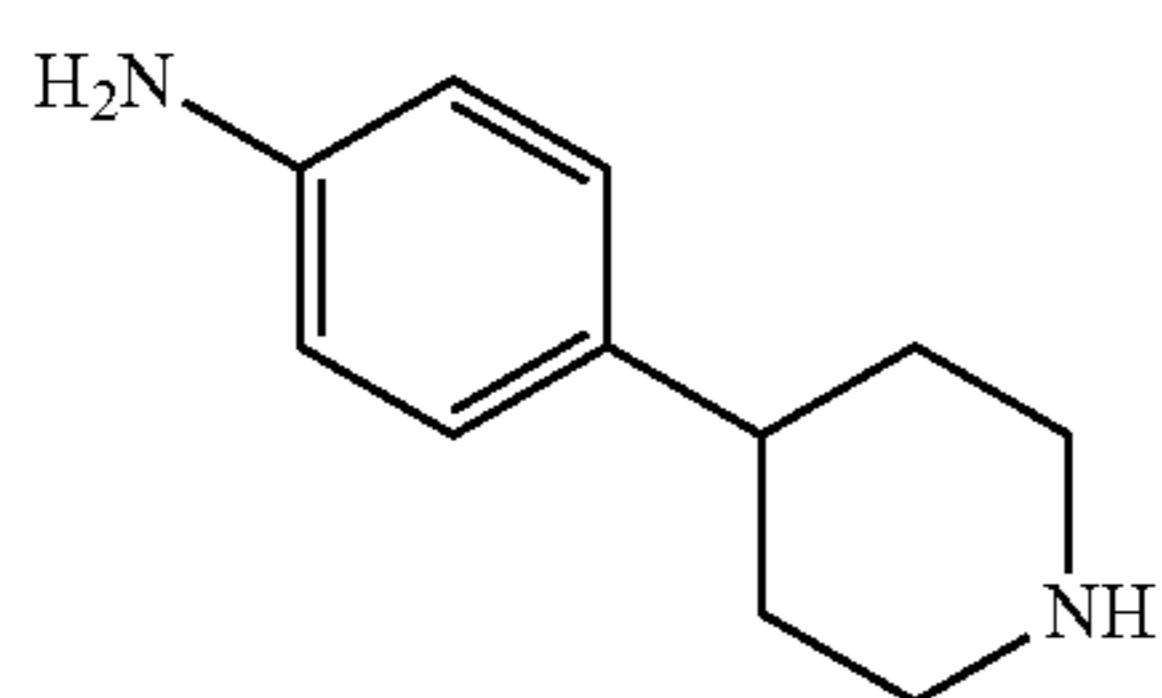
4-(Piperidin-4-yl)aniline (NT1-004)
