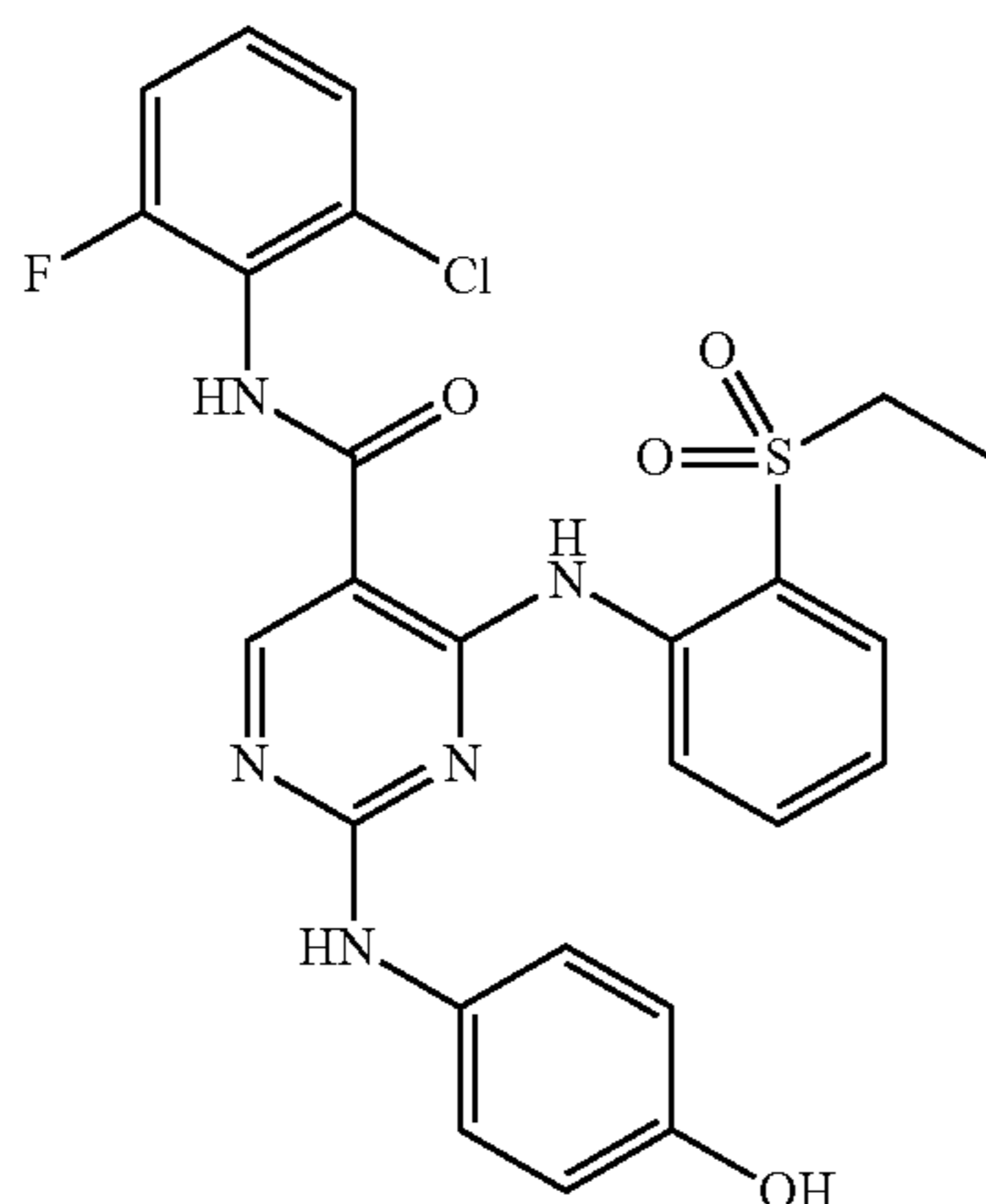
N-(2-chloro-6-fluorophenyl)-4-(2-(ethylsulfonyl)phenylamino)-2-(4-hydroxyphenylamino)pyrimidine-5-carboxamide (YL7-058-2)
