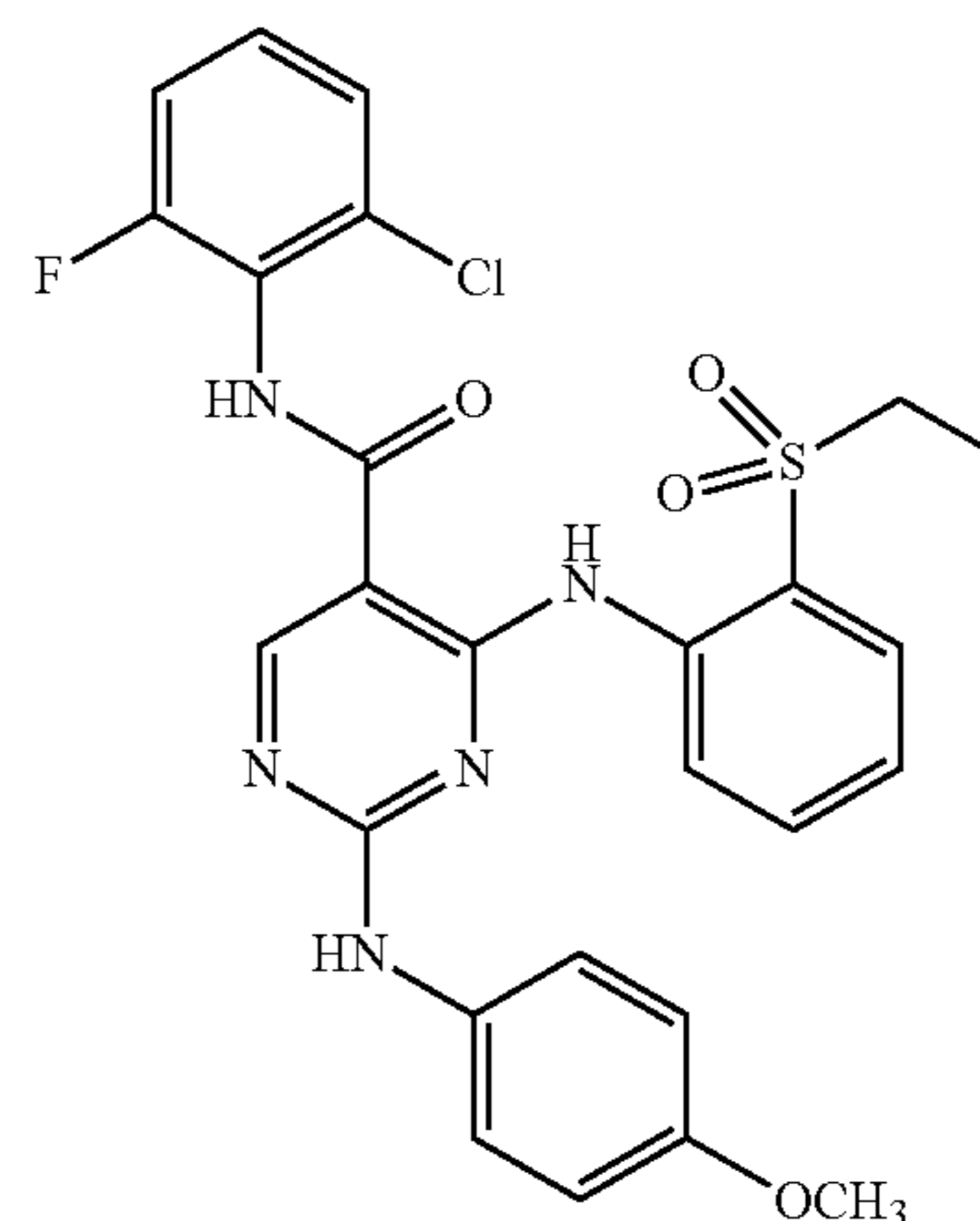
N-(2-chloro-6-fluorophenyl)-4-(2-(ethylsulfonyl)phenylamino)-2-(4-methoxyphenylamino)pyrimidine-5-carboxamide (YL7-058-1)
