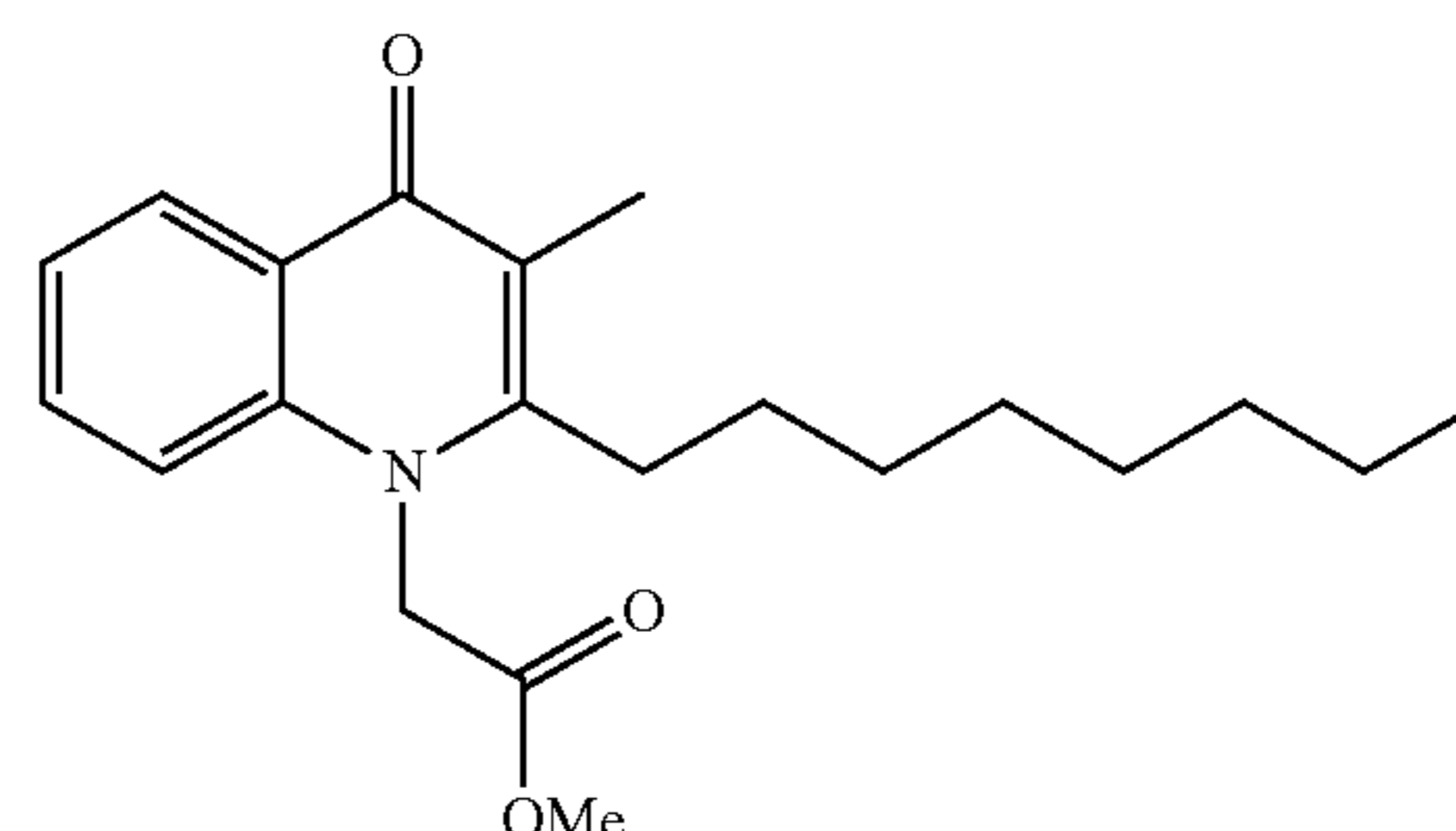
Structural Formula (5)
