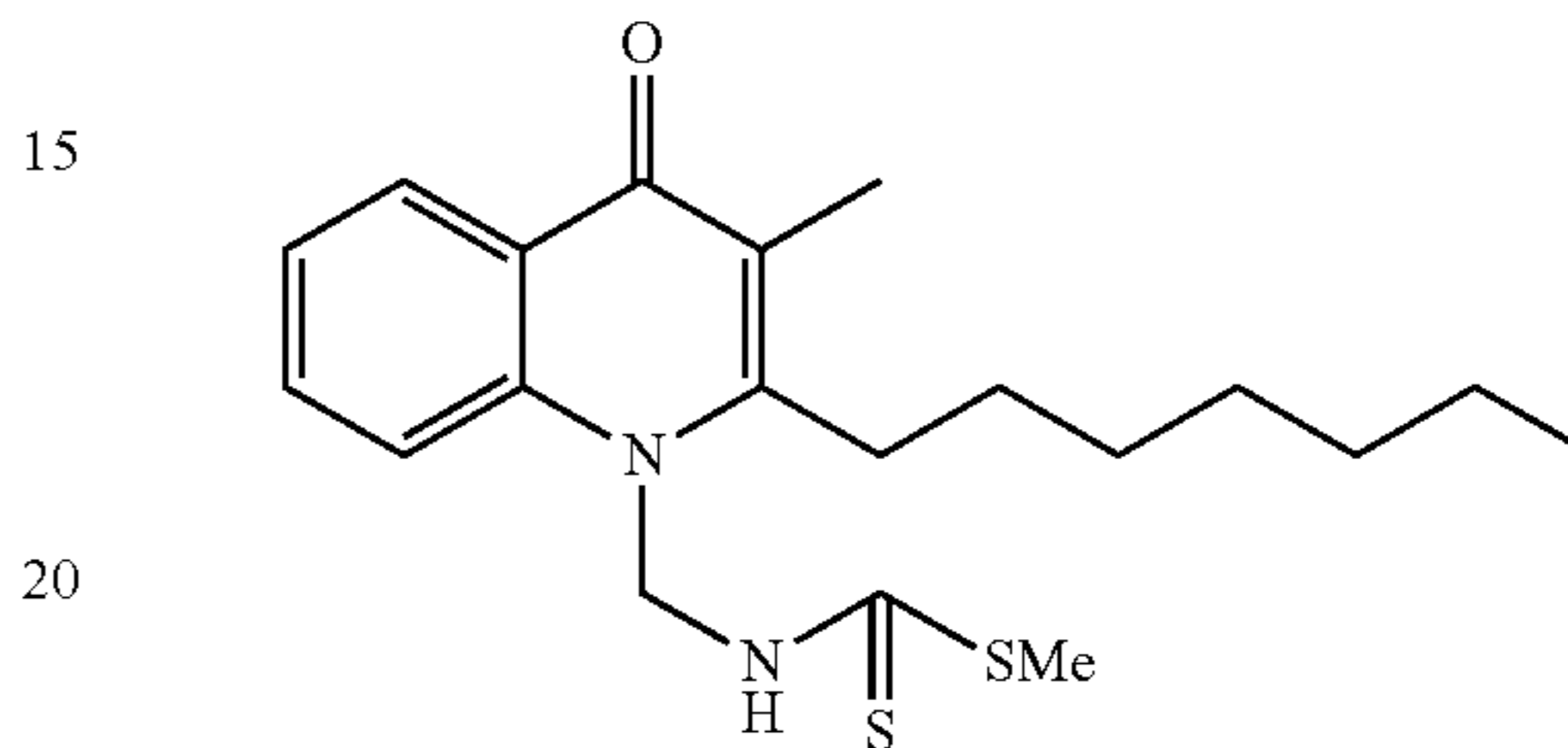
Structural Formula (13)
