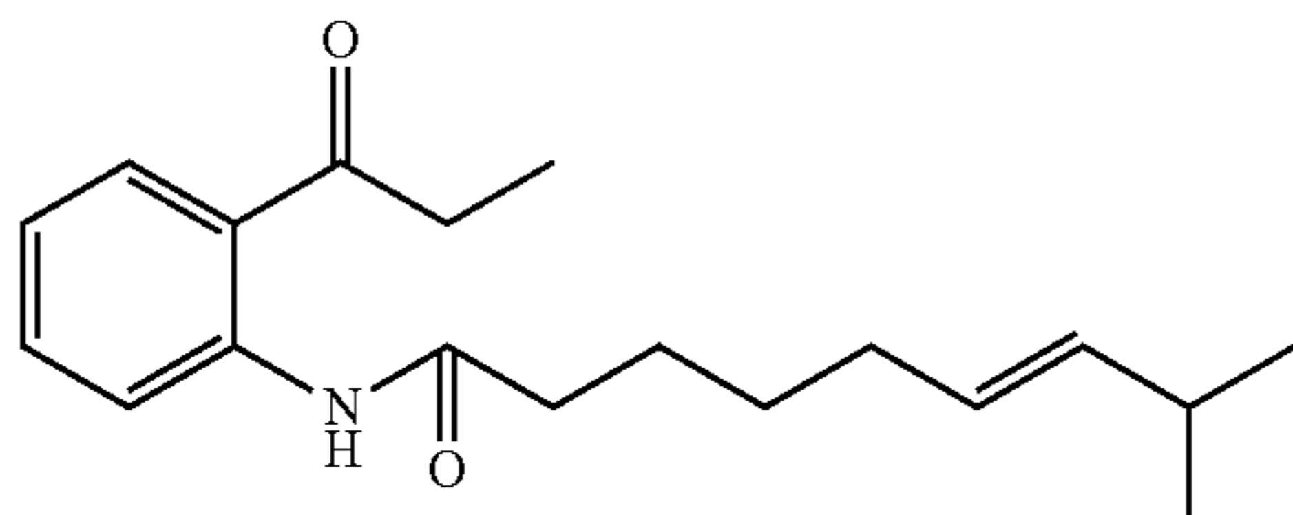
Structural Formula (3)
