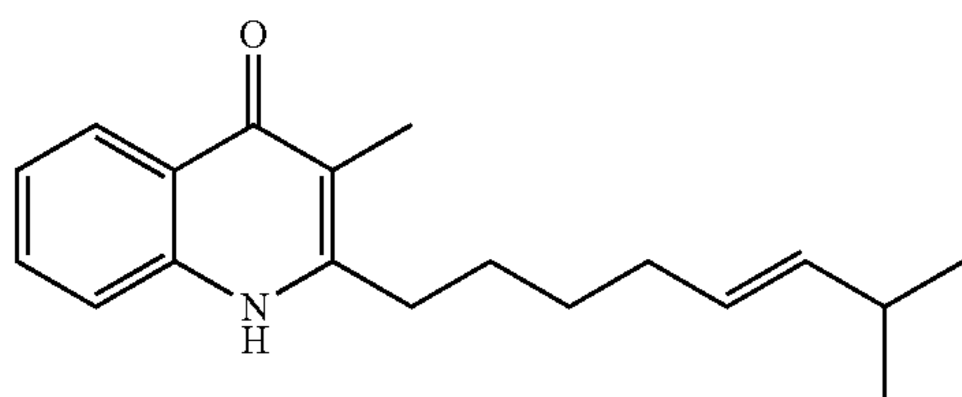
Structural Formula (3)
