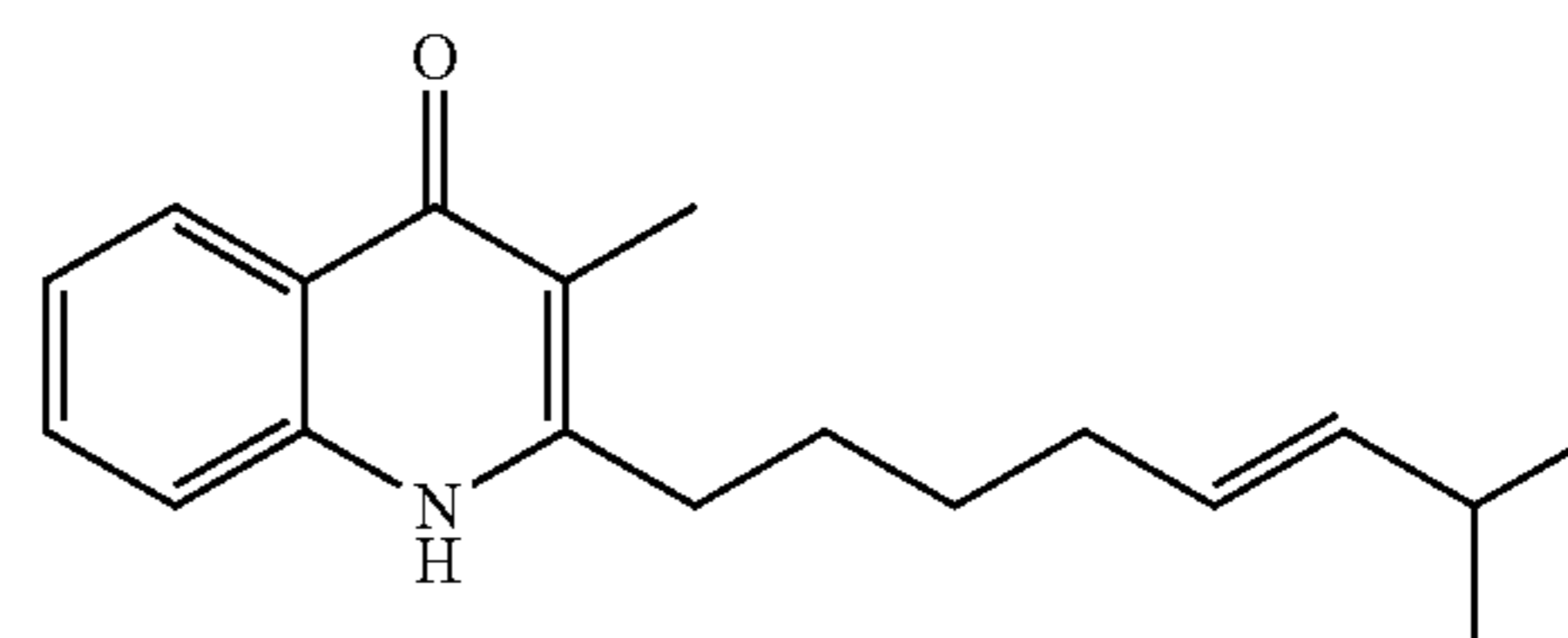
Structural Formula (3)
