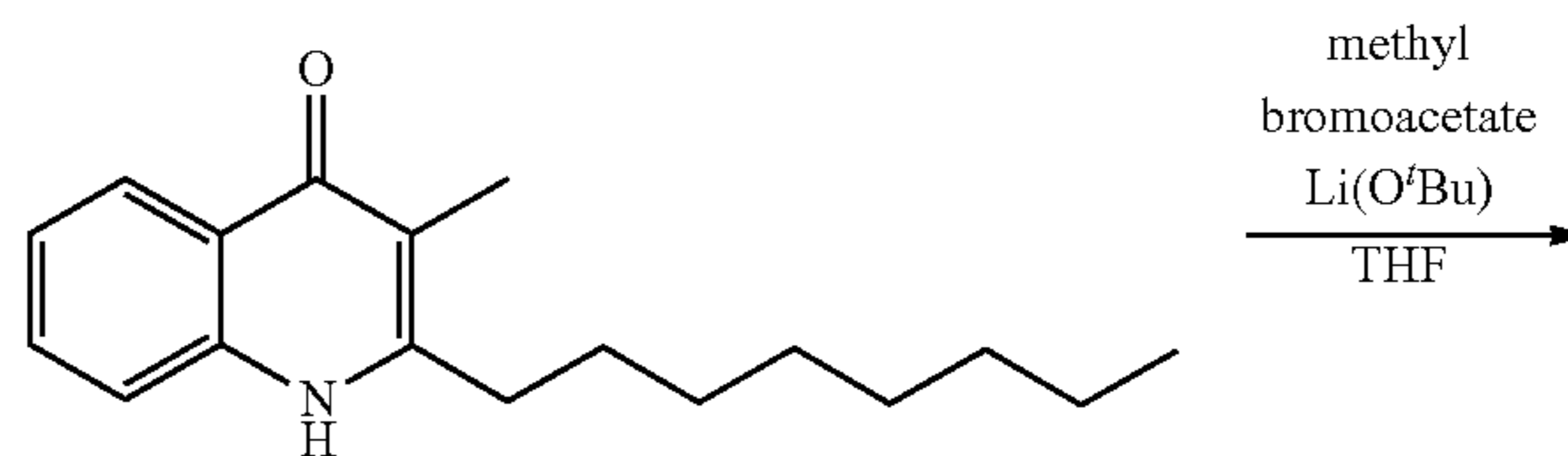
Structural Formula (21)
