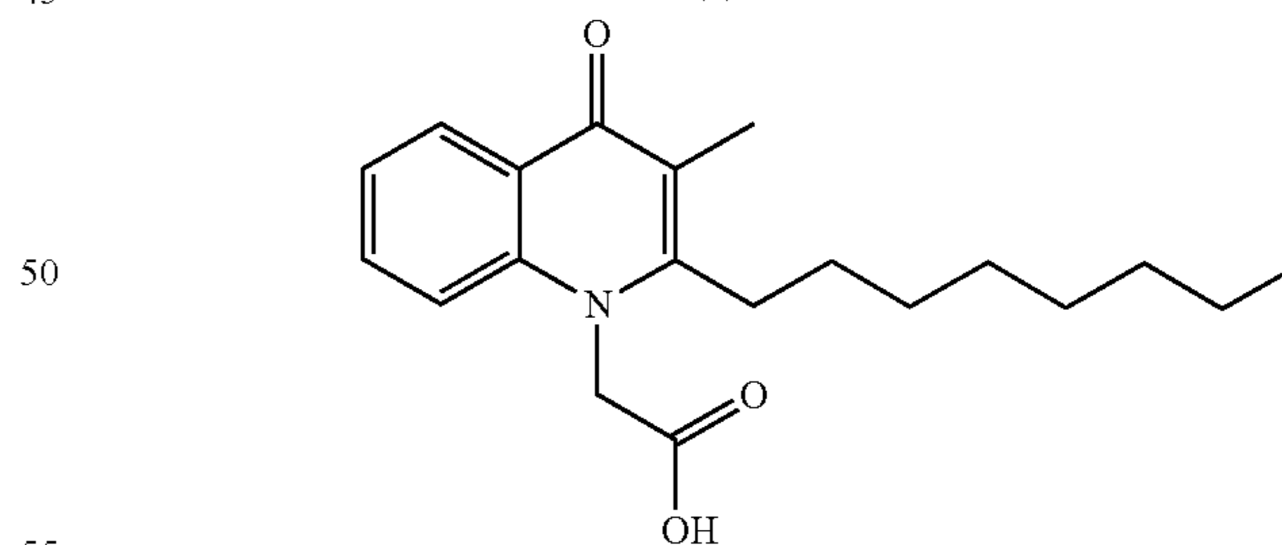
Structural Formula (6)
