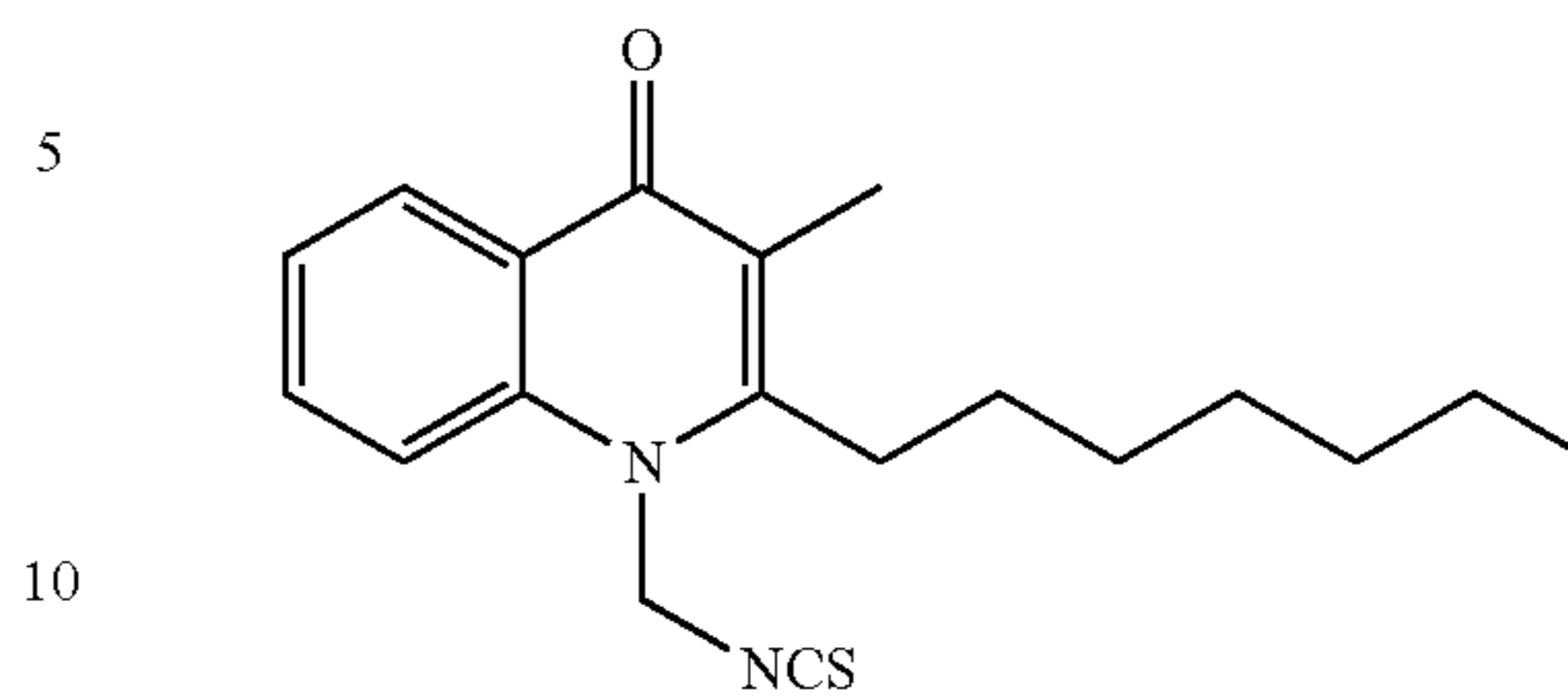
Structural Formula (12)
