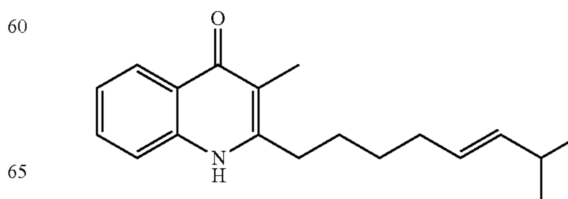
Structural Formula (3)
