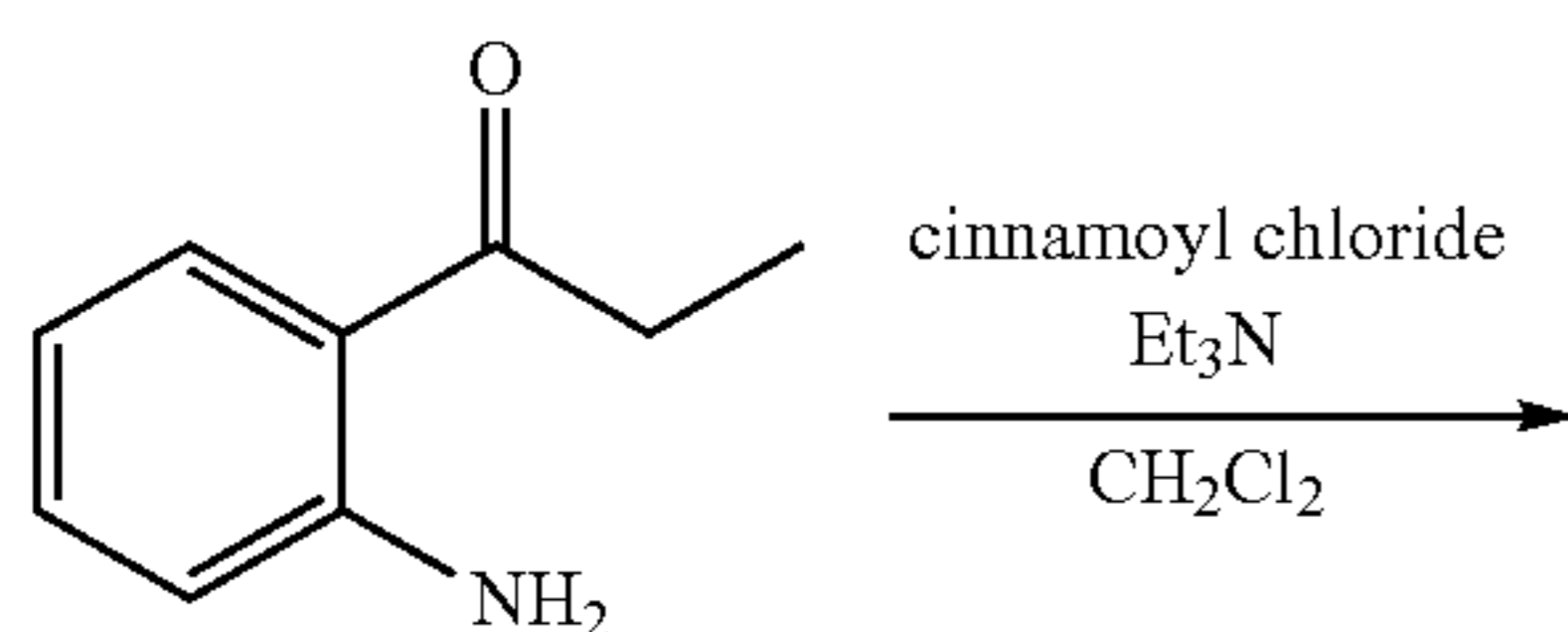
Structural Formula (14)
