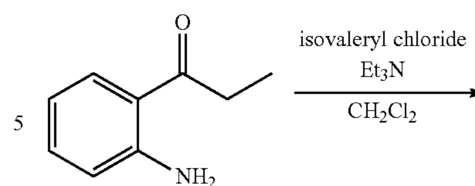
Structural Formula (14)
