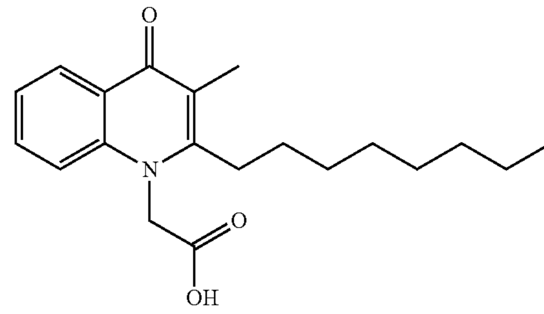
Structural Formula (7)
