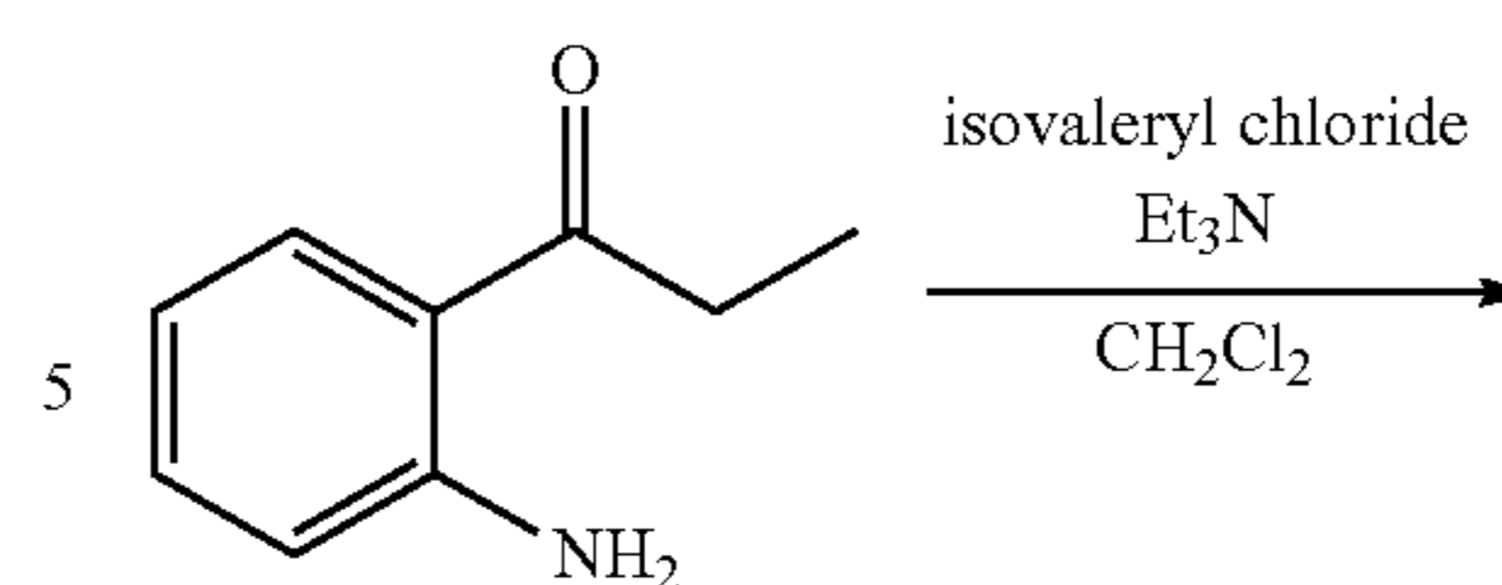
Structural Formula (14)
