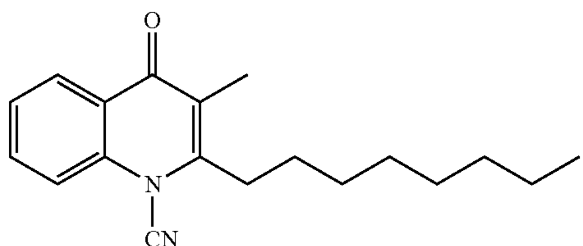
Structural Formula (7)
