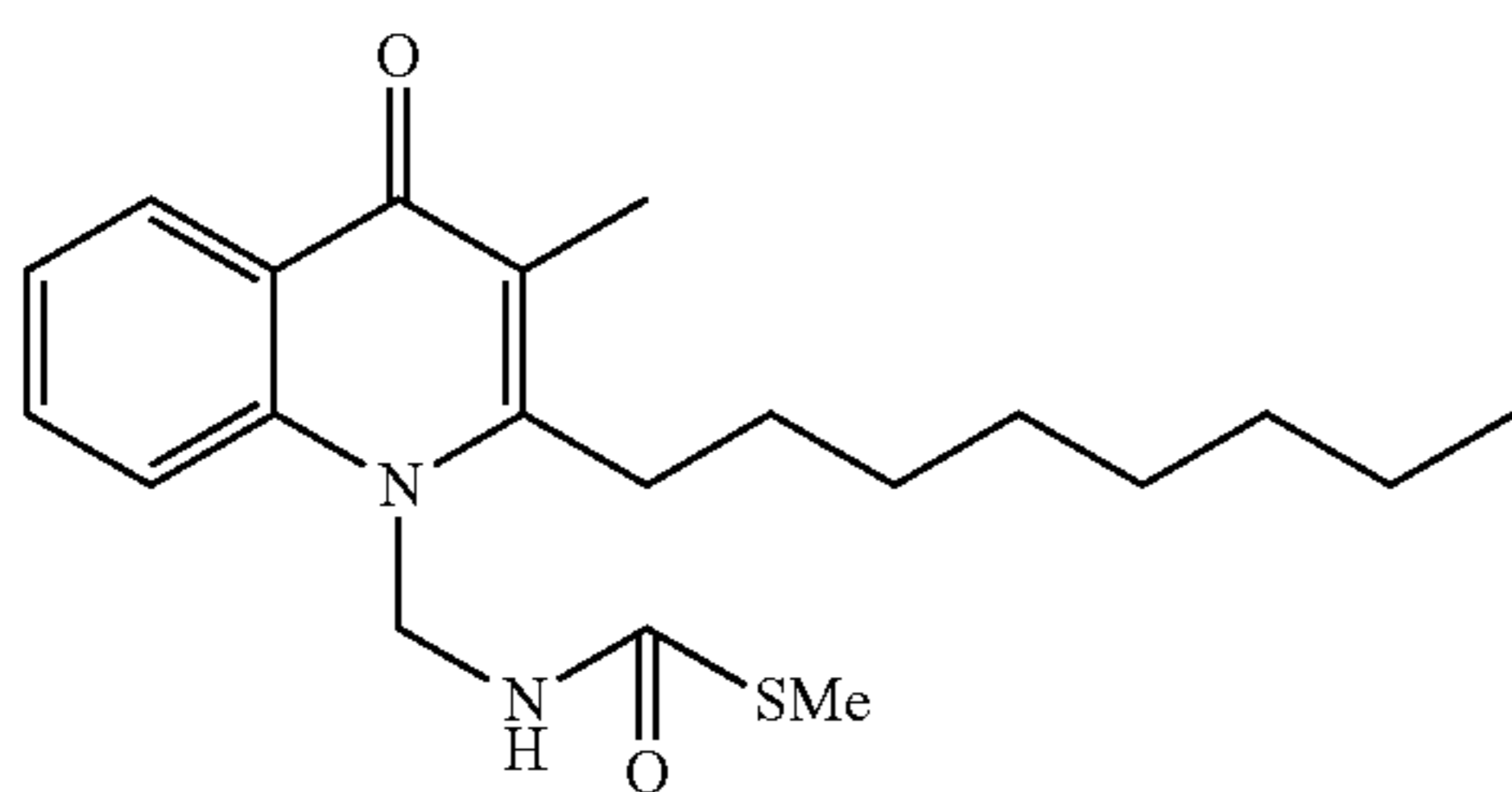
Structural Formula (10)
