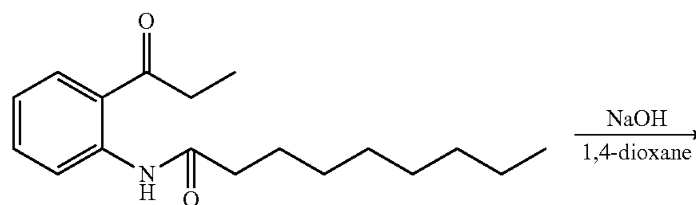
Structural Formula (16)
