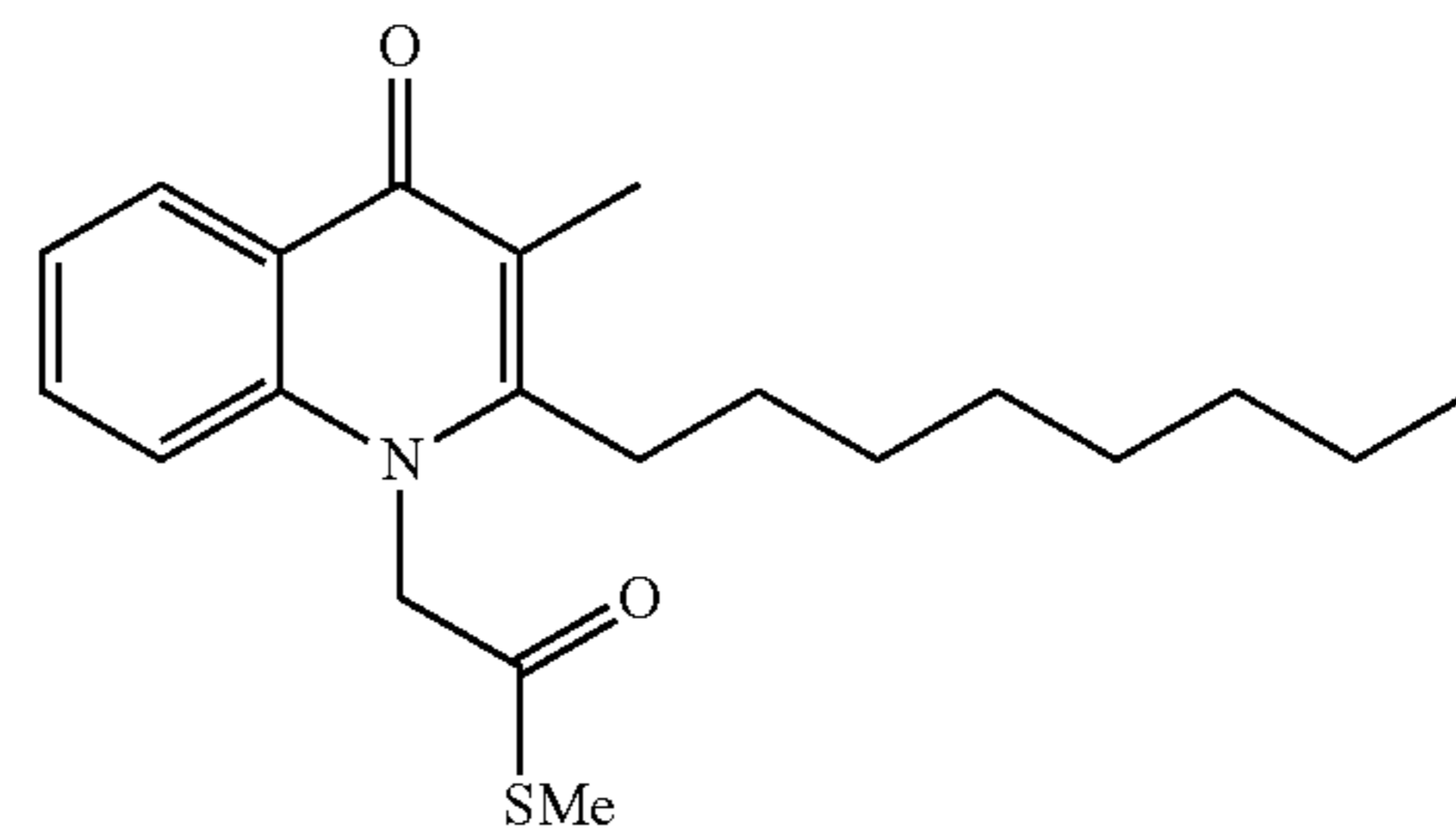
Structural Formula (10)
