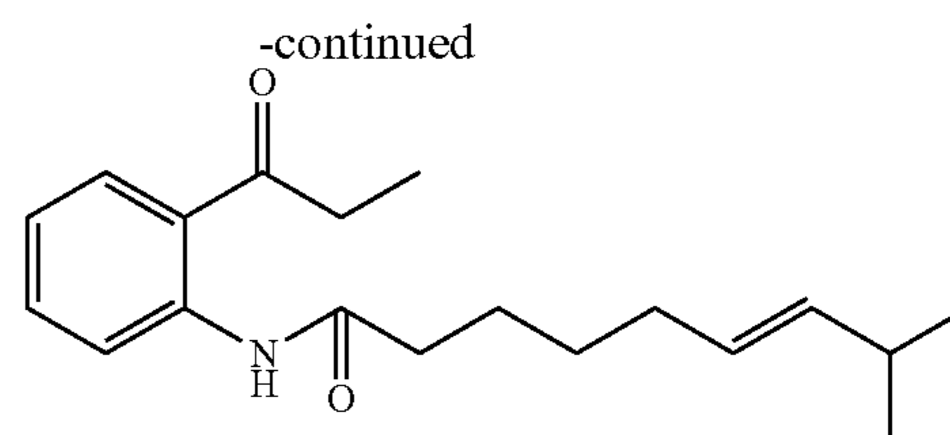
Structural Formula (17)
