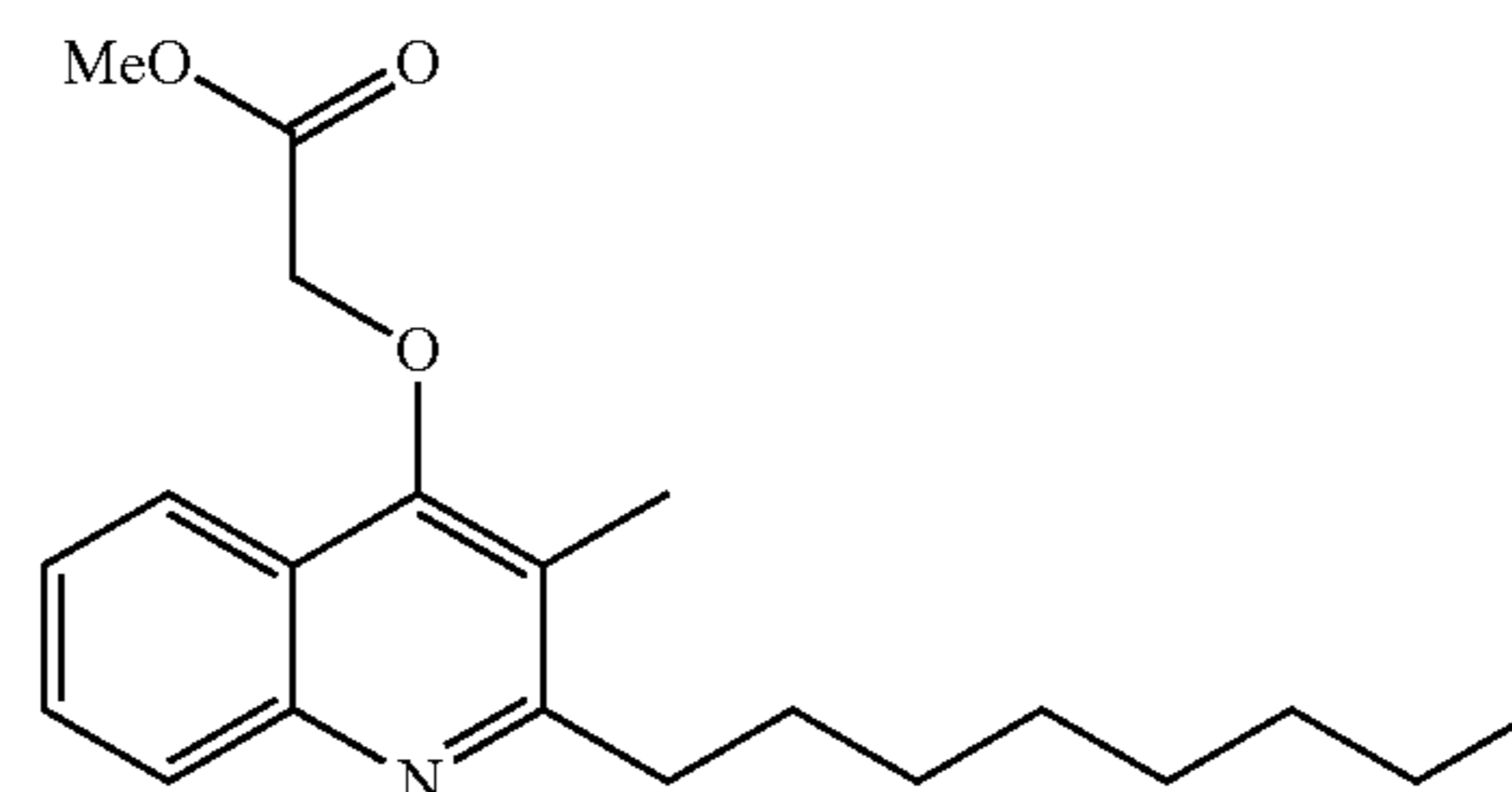
Structural Formula (1)
