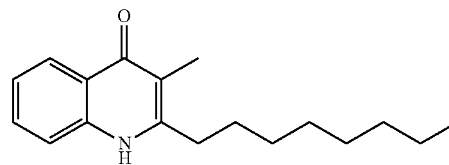
Structural Formula (1)
