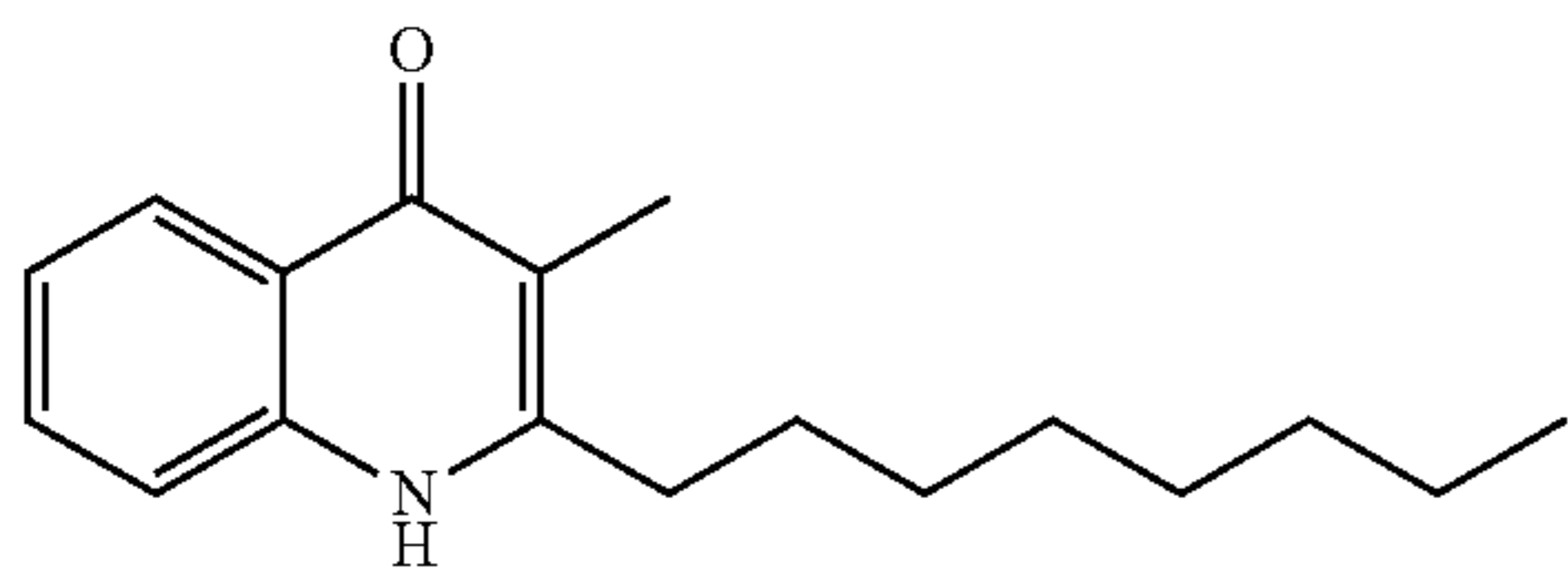
Structural Formula (1)
