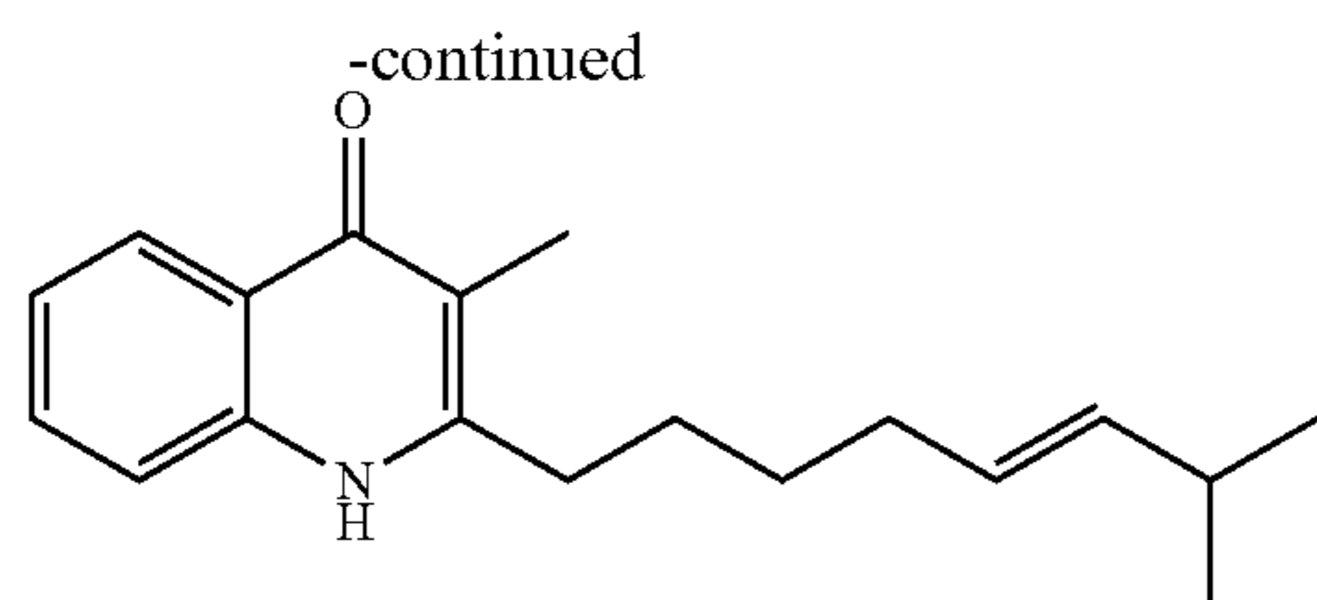
Structural Formula (3)
