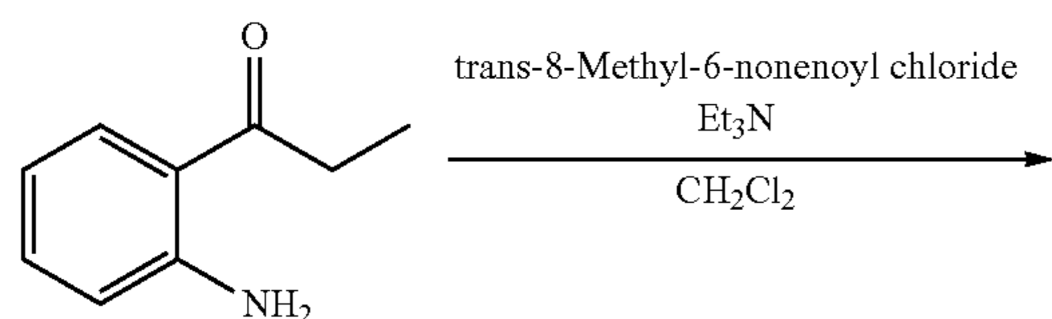
Structural Formula (14)
