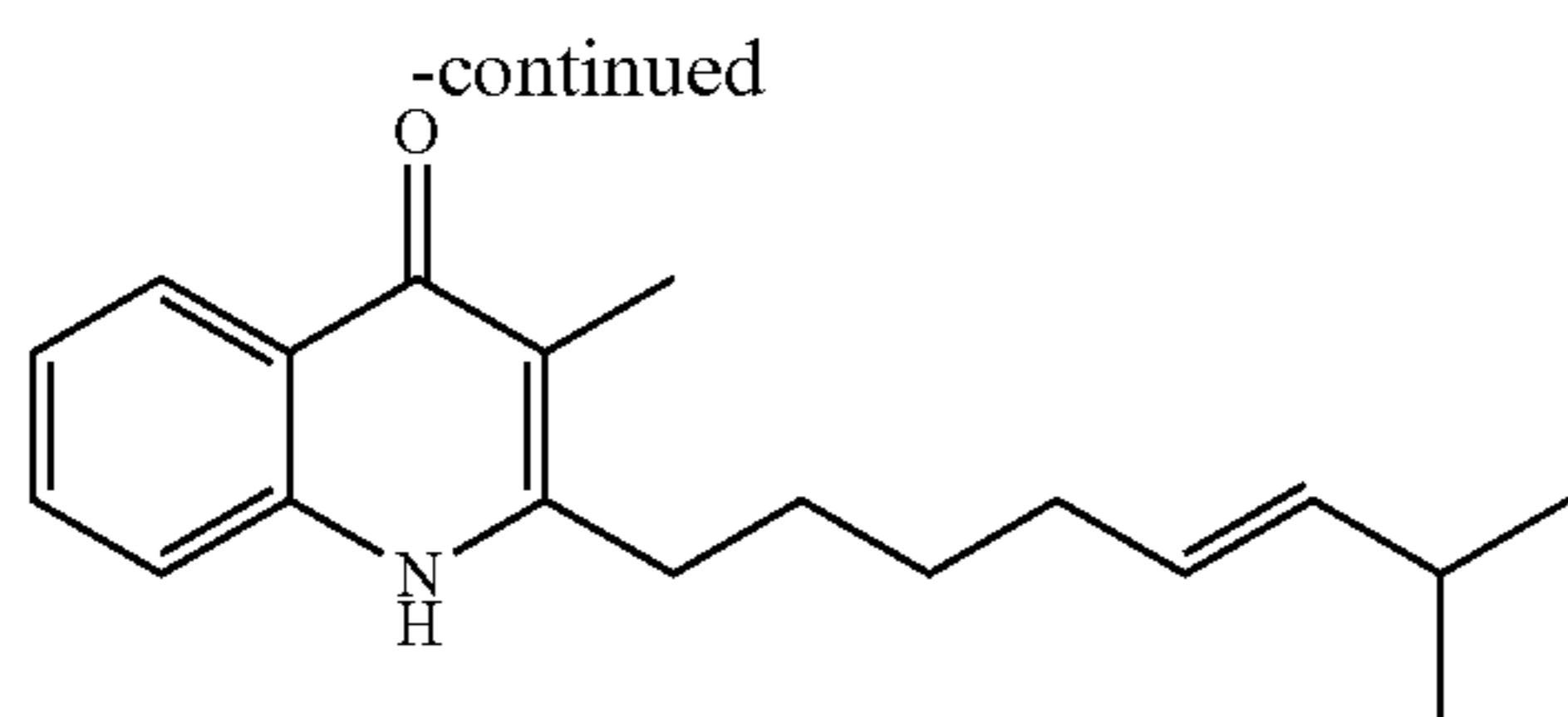
Structural Formula (3)
