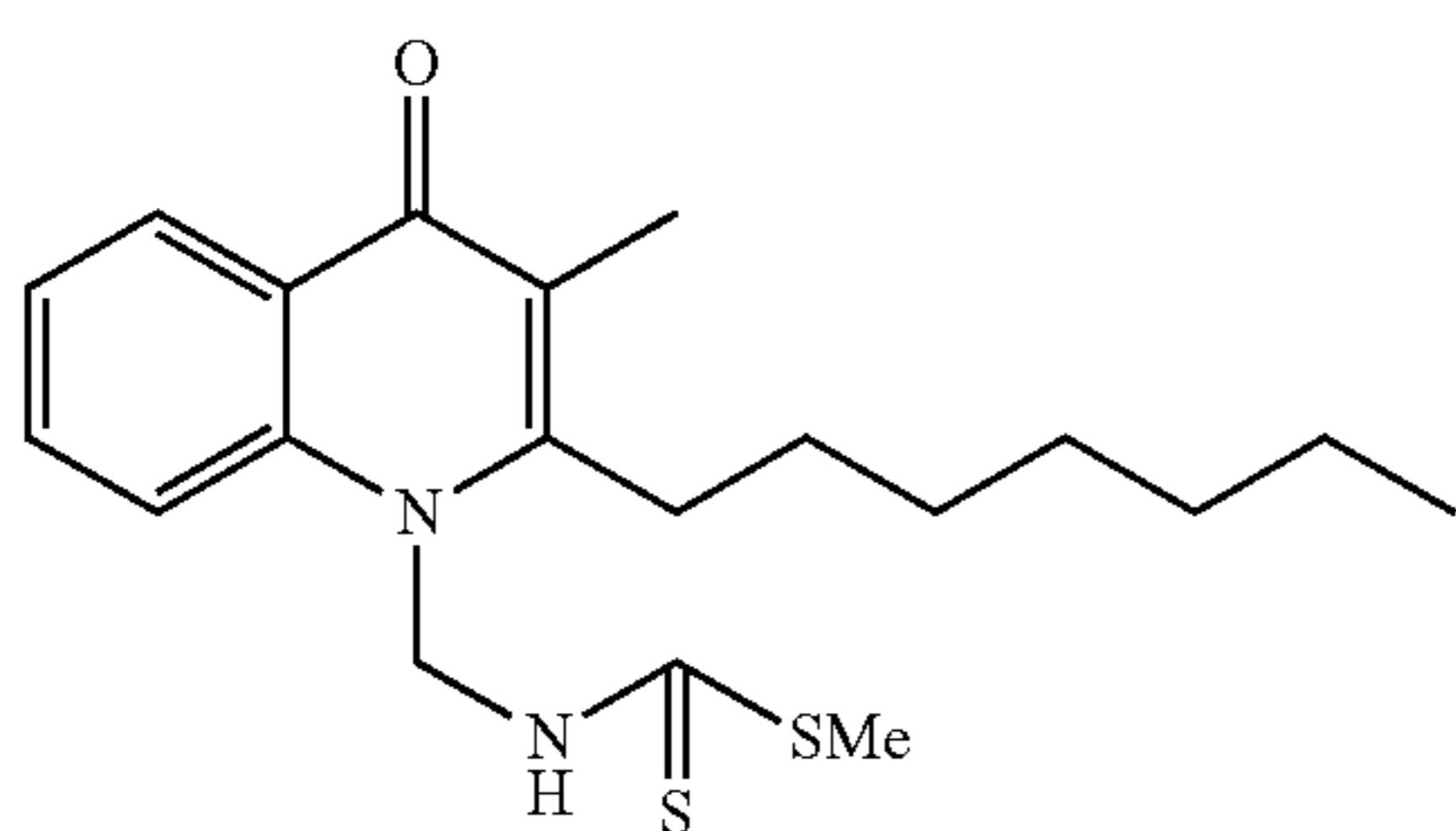
Structural Formula (12)
