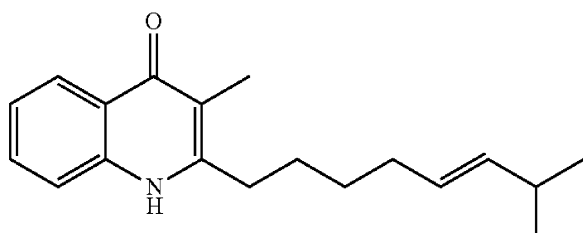
Structural Formula (18)
