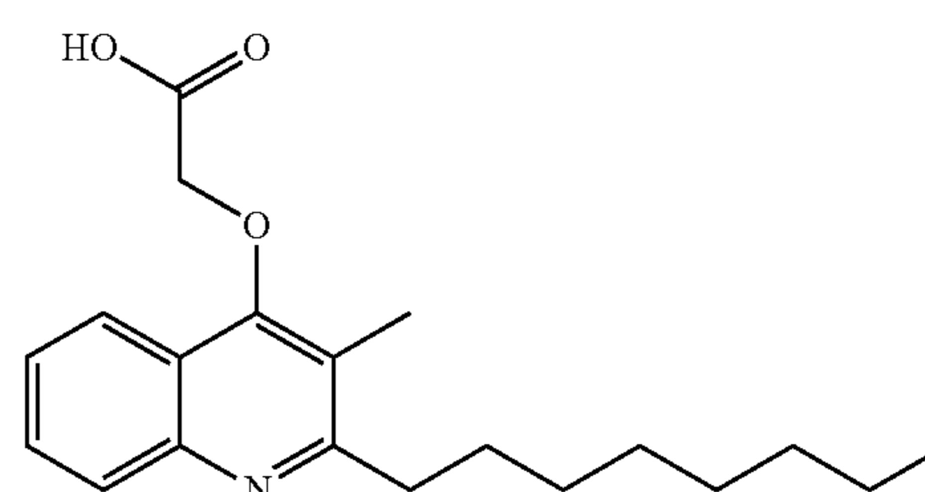
Structural Formula (2)
