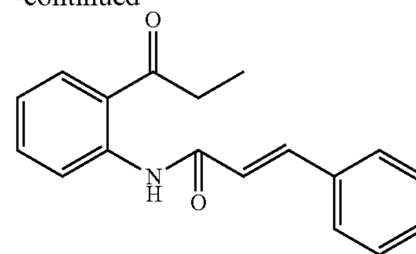
Structural Formula (19)
