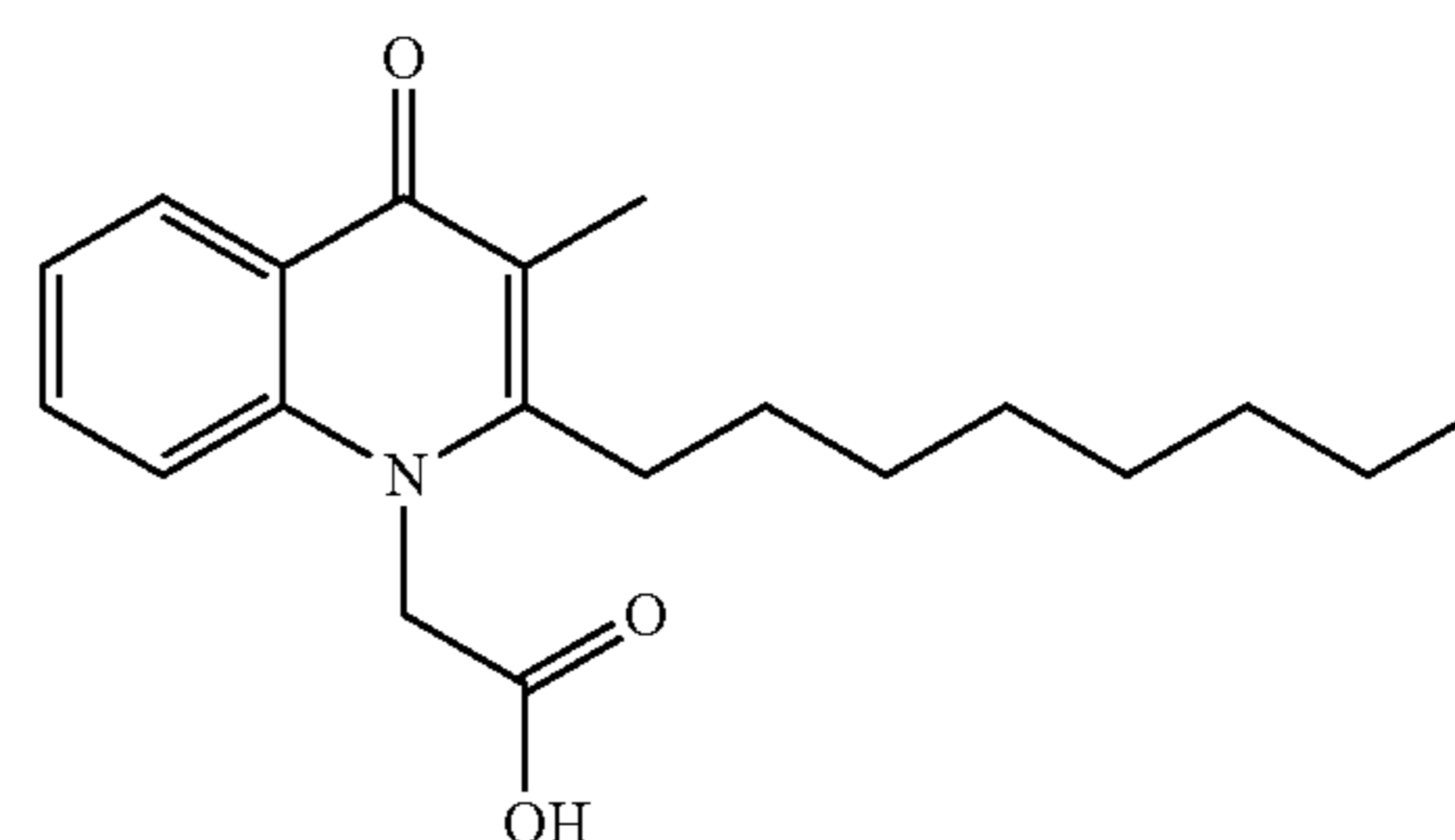
Structural Formula (10)
