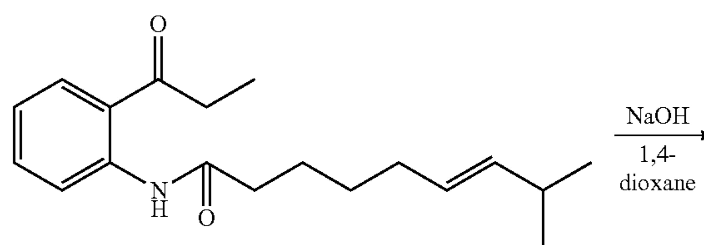
Structural Formula (17)
