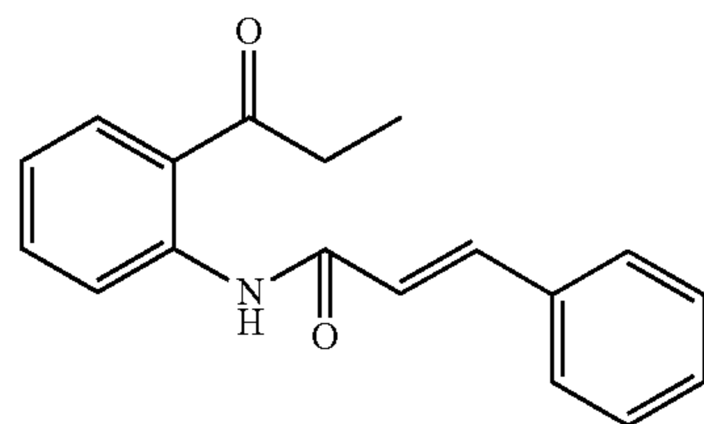
Structural Formula (19)
