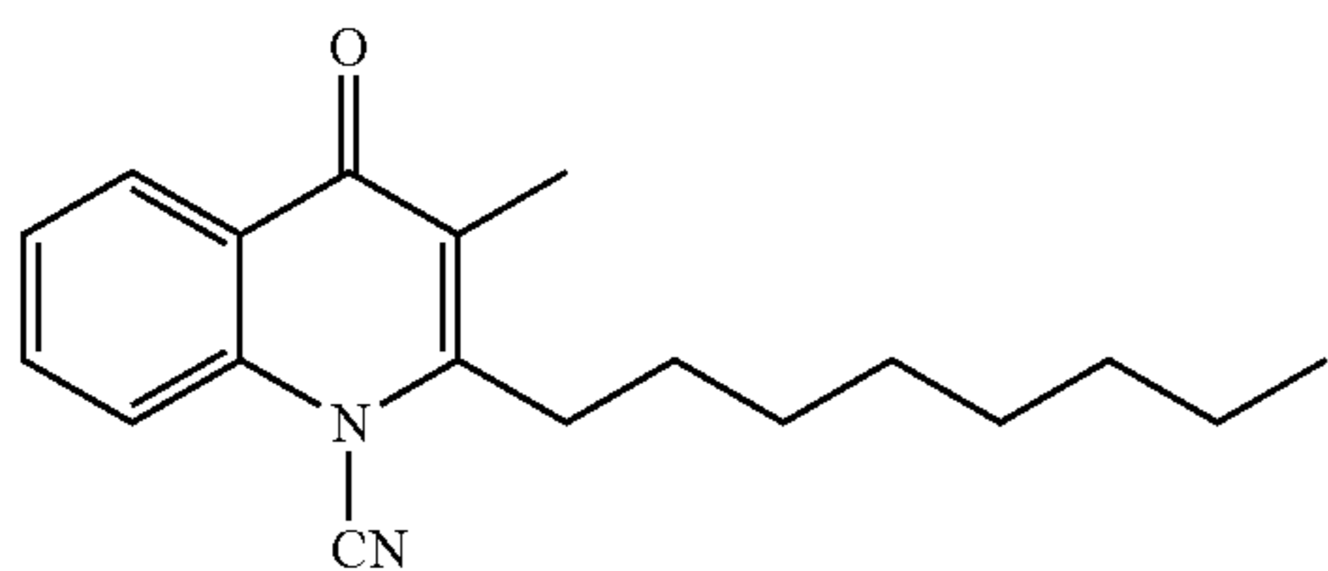
Structural Formula (8)
