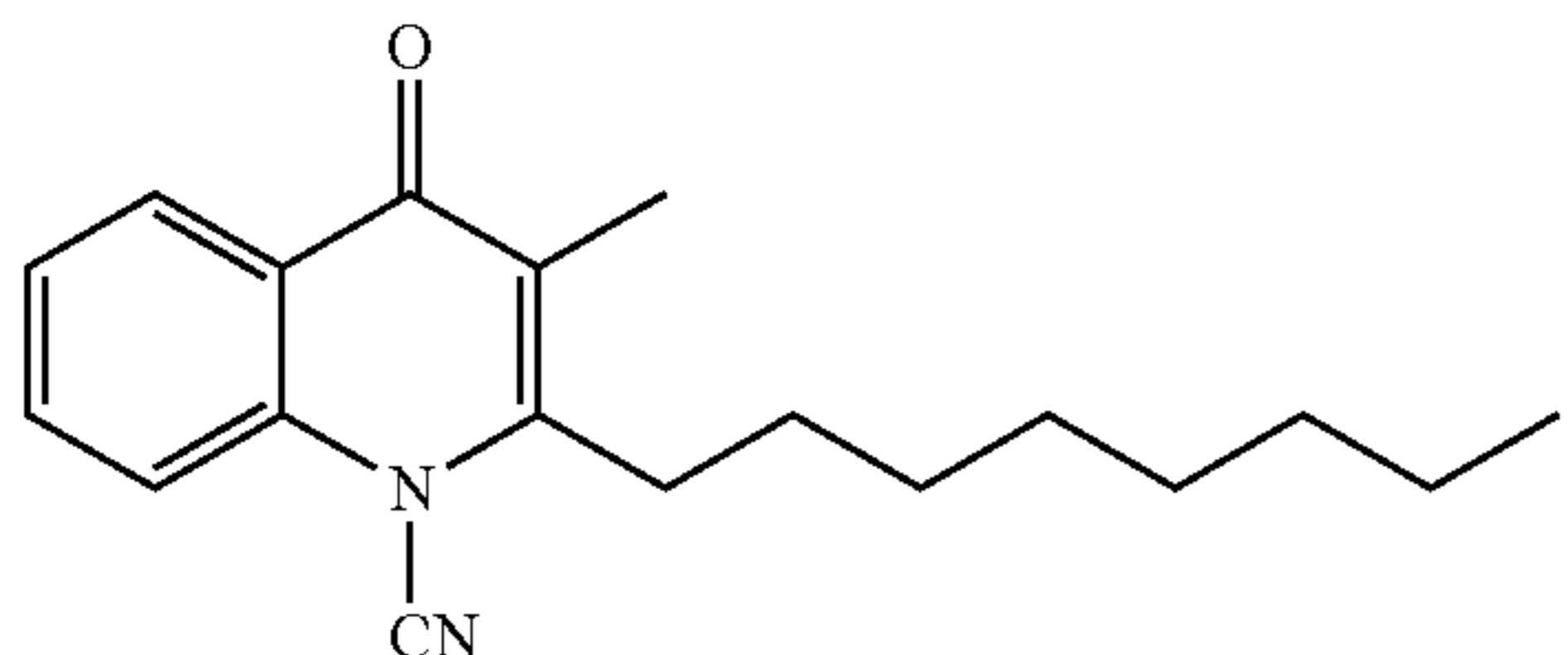
Structural Formula (7)
