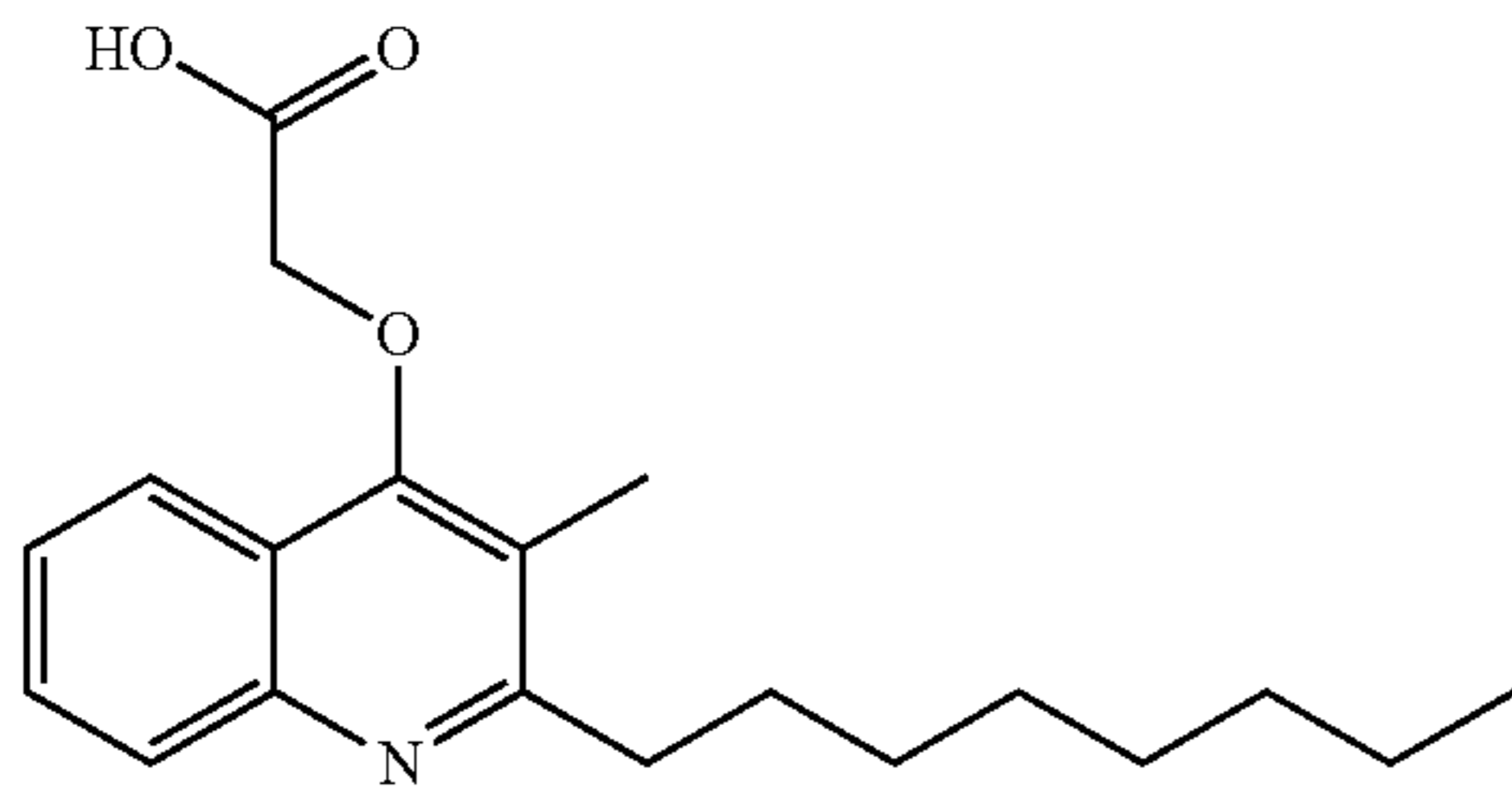
Structural Formula (3)
