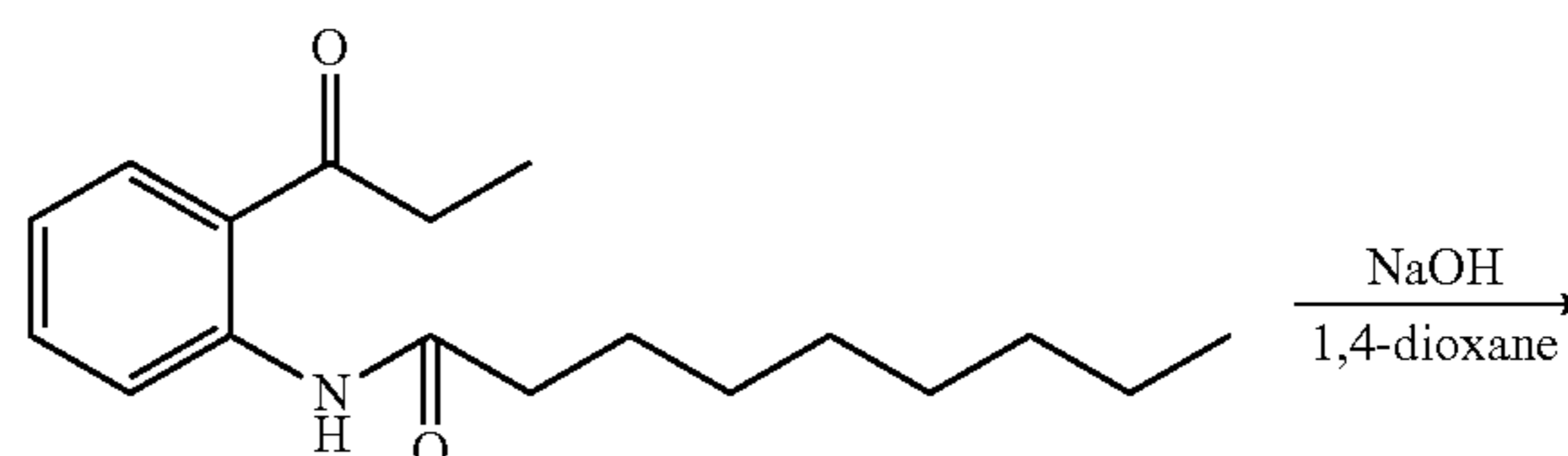
Structural Formula (16)
