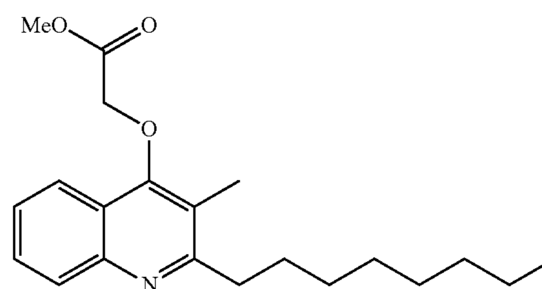
Structural Formula (2)
