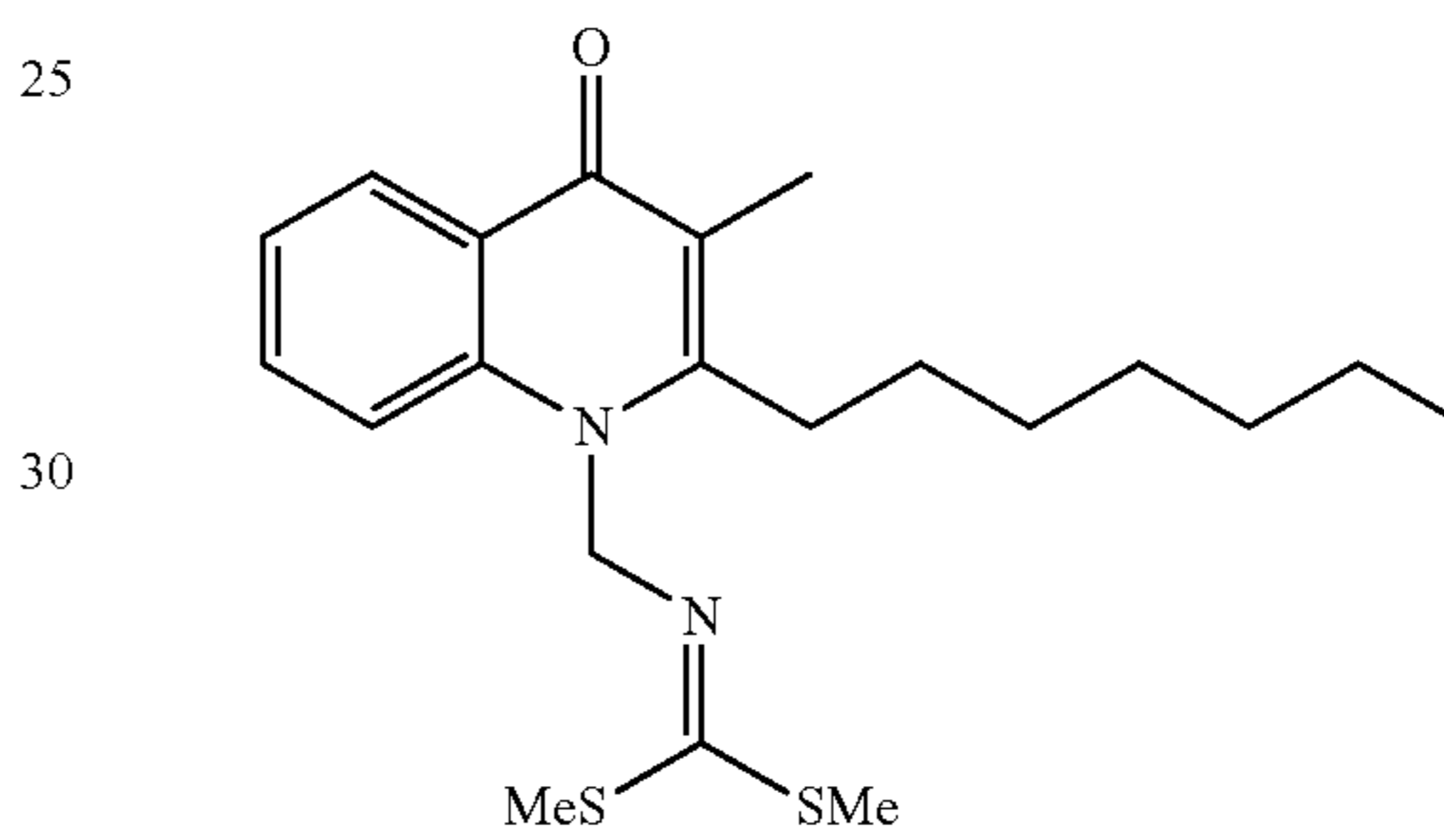
Structural Formula (13)
