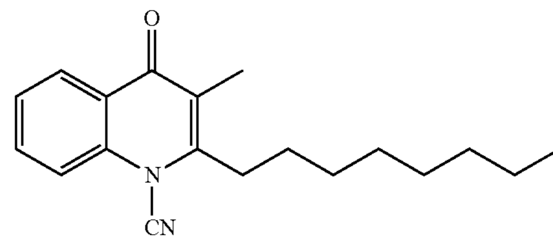
Structural Formula (8)
