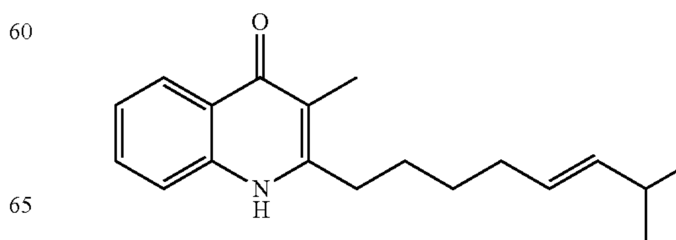
Structural Formula (3)
