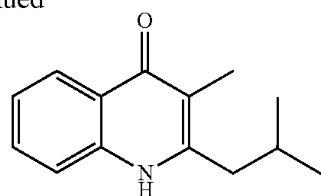
Structural Formula (4)
