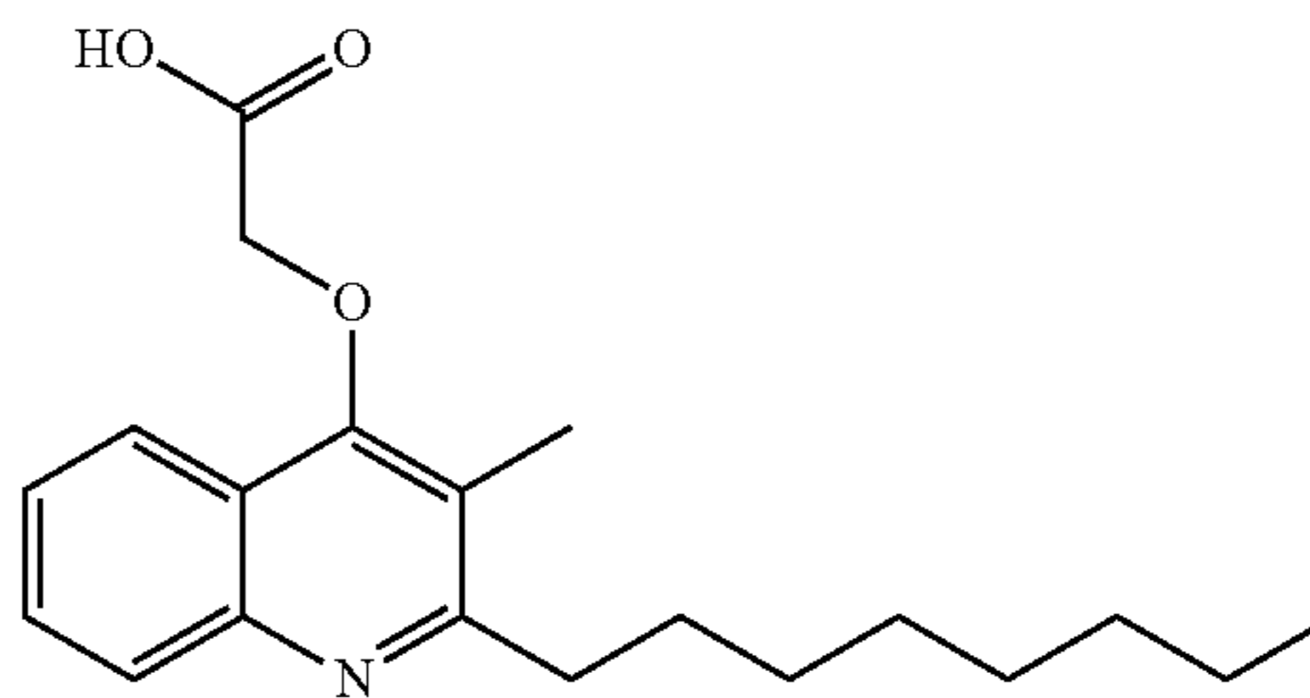
Structural Formula (2)
