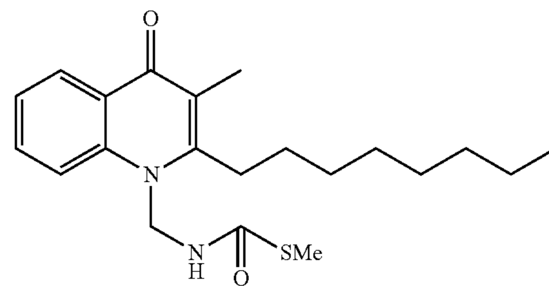
Structural Formula (10)
