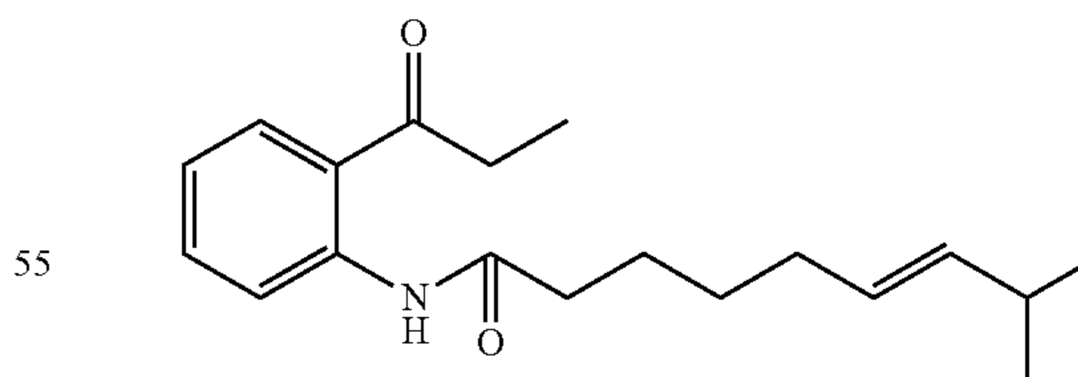
Structural Formula (3)
