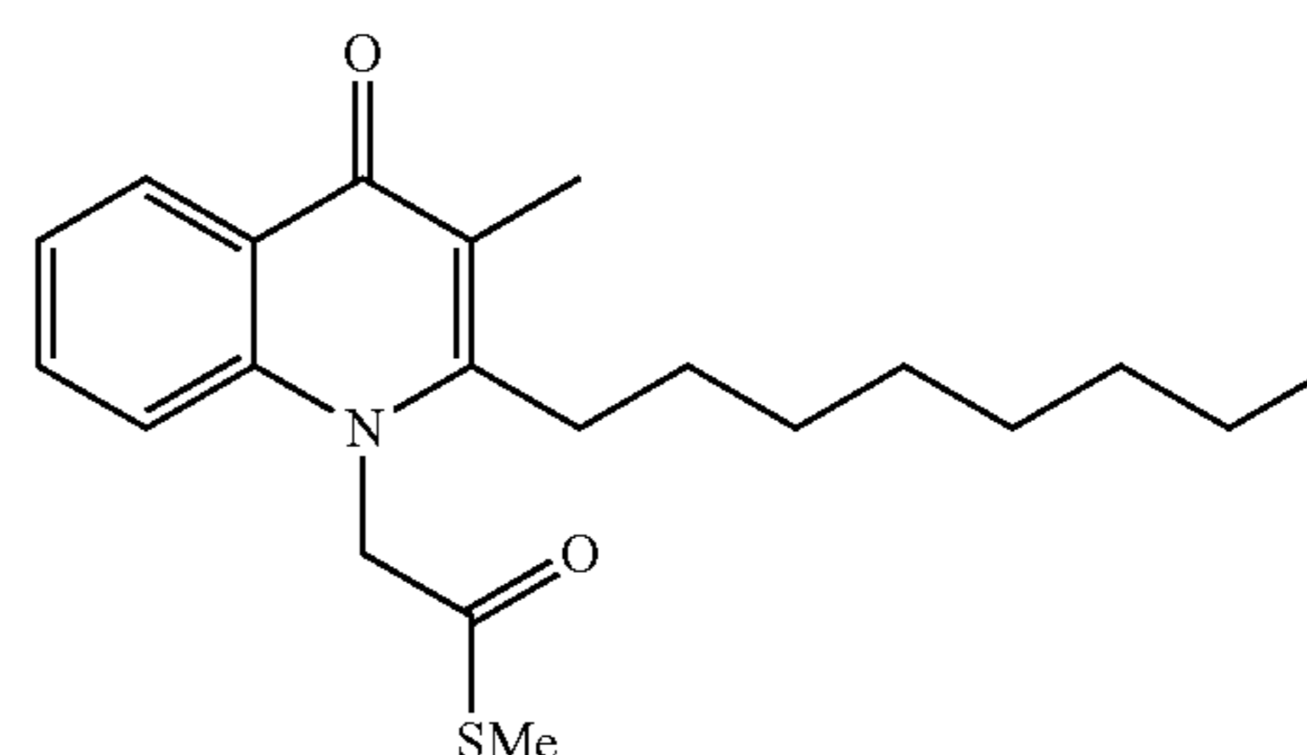
Structural Formula (9)
