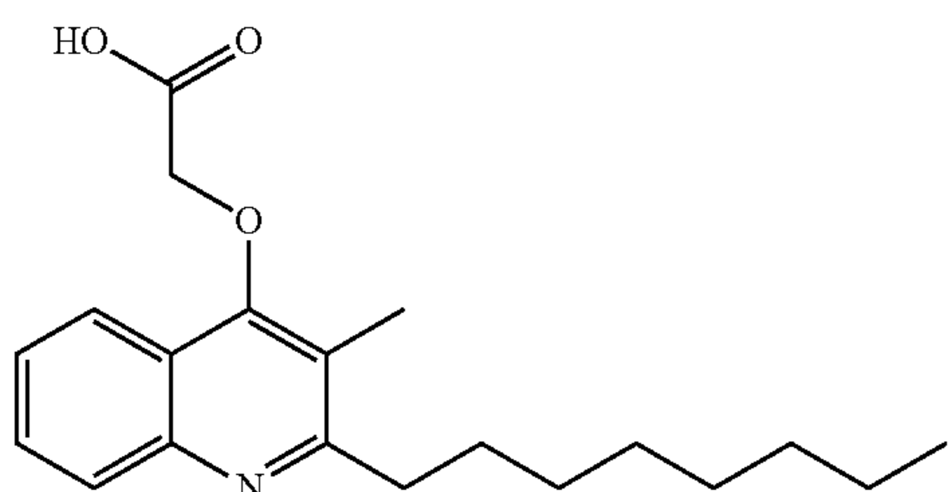
Structural Formula (2)
