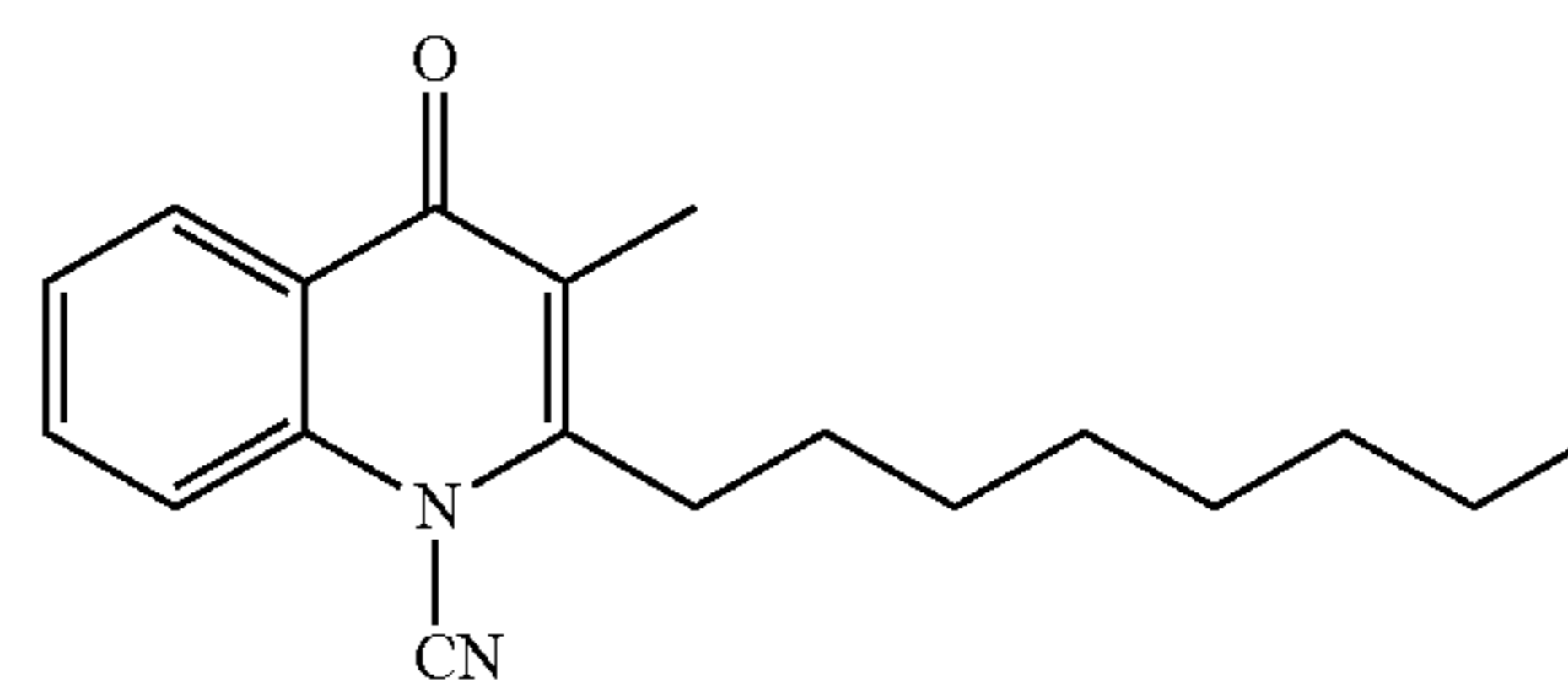
Structural Formula (7)
