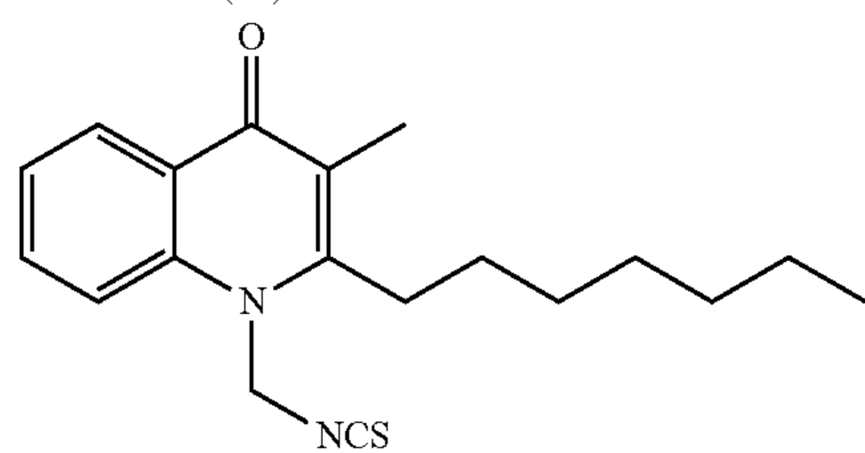
Structural Formula (11)
