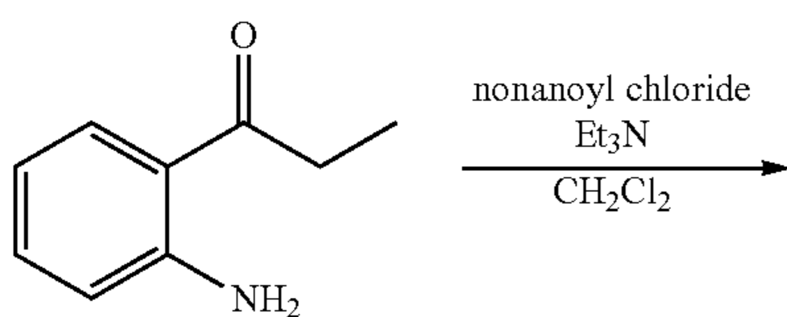
Structural Formula (14)
