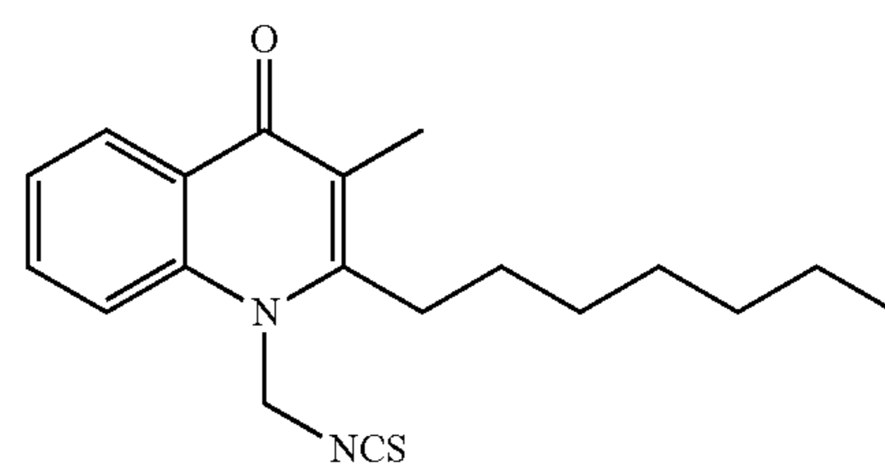
Structural Formula (11)
