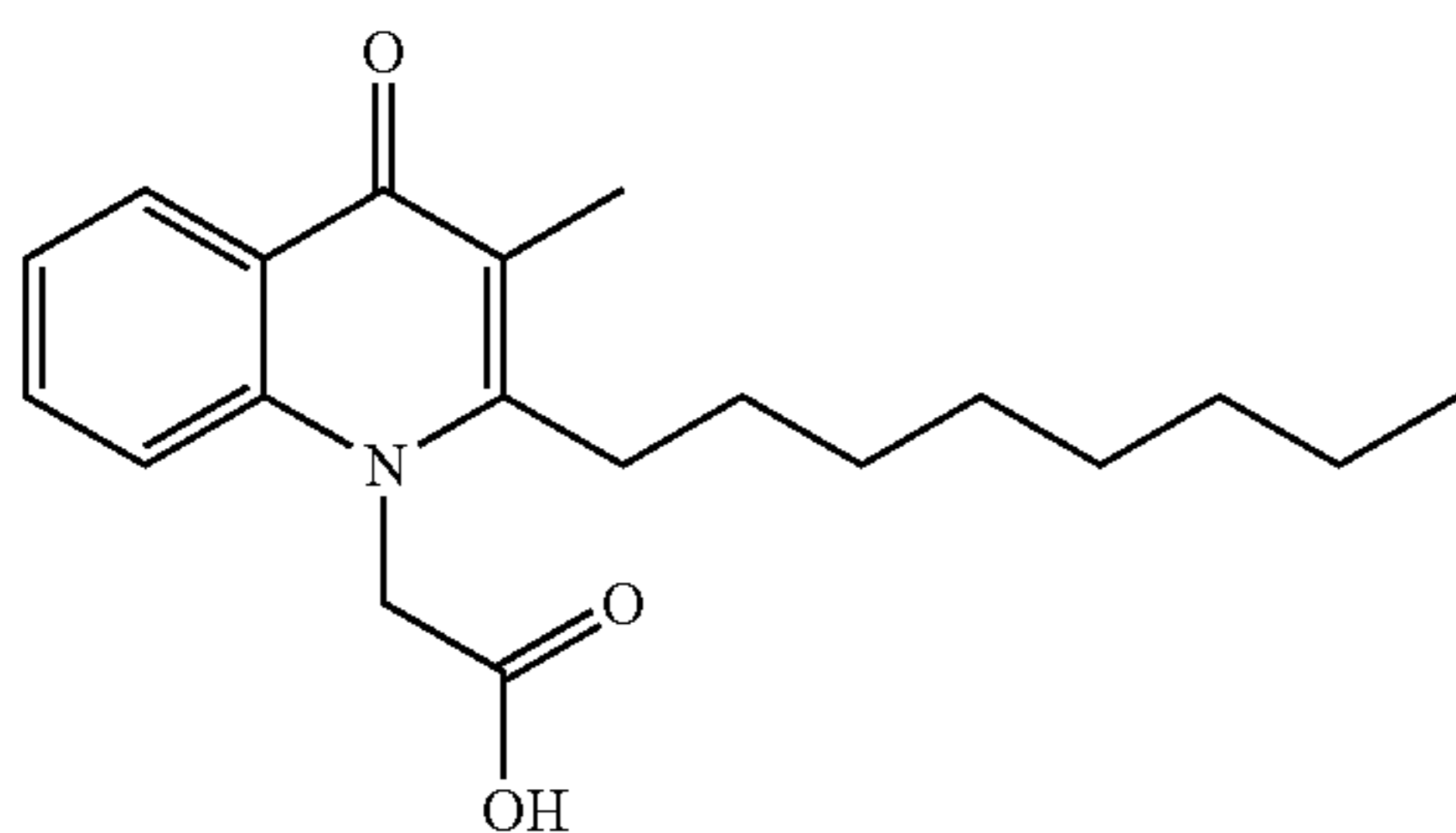
Structural Formula (10)
