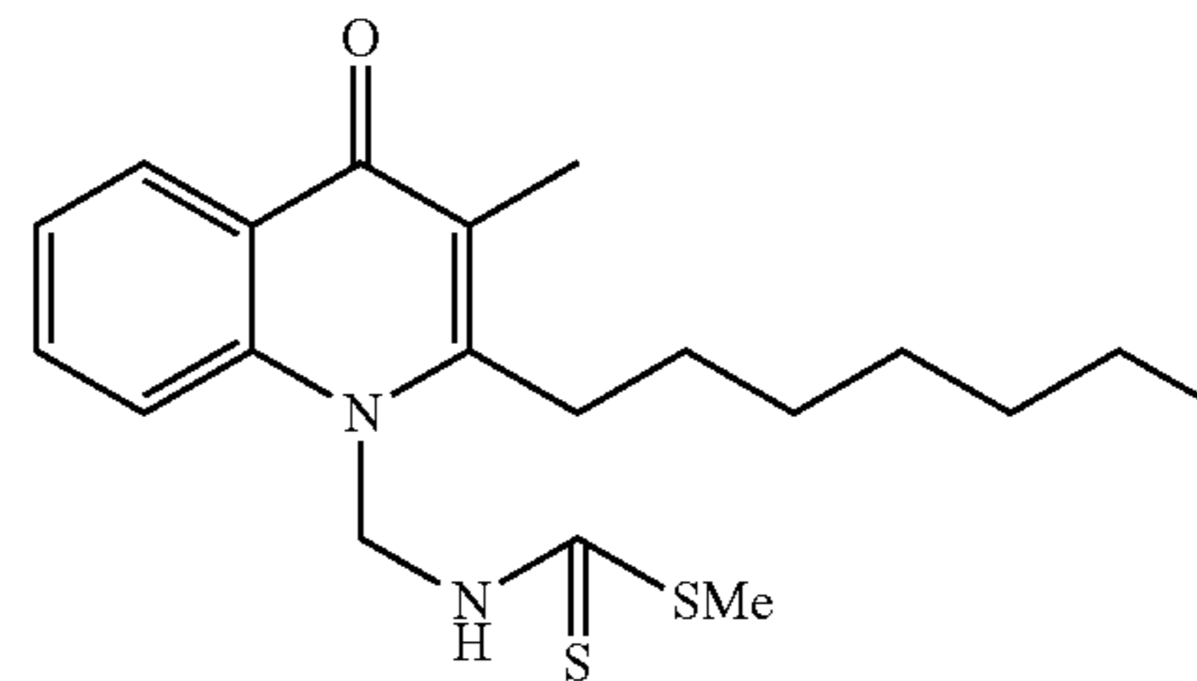
Structural Formula (12)
