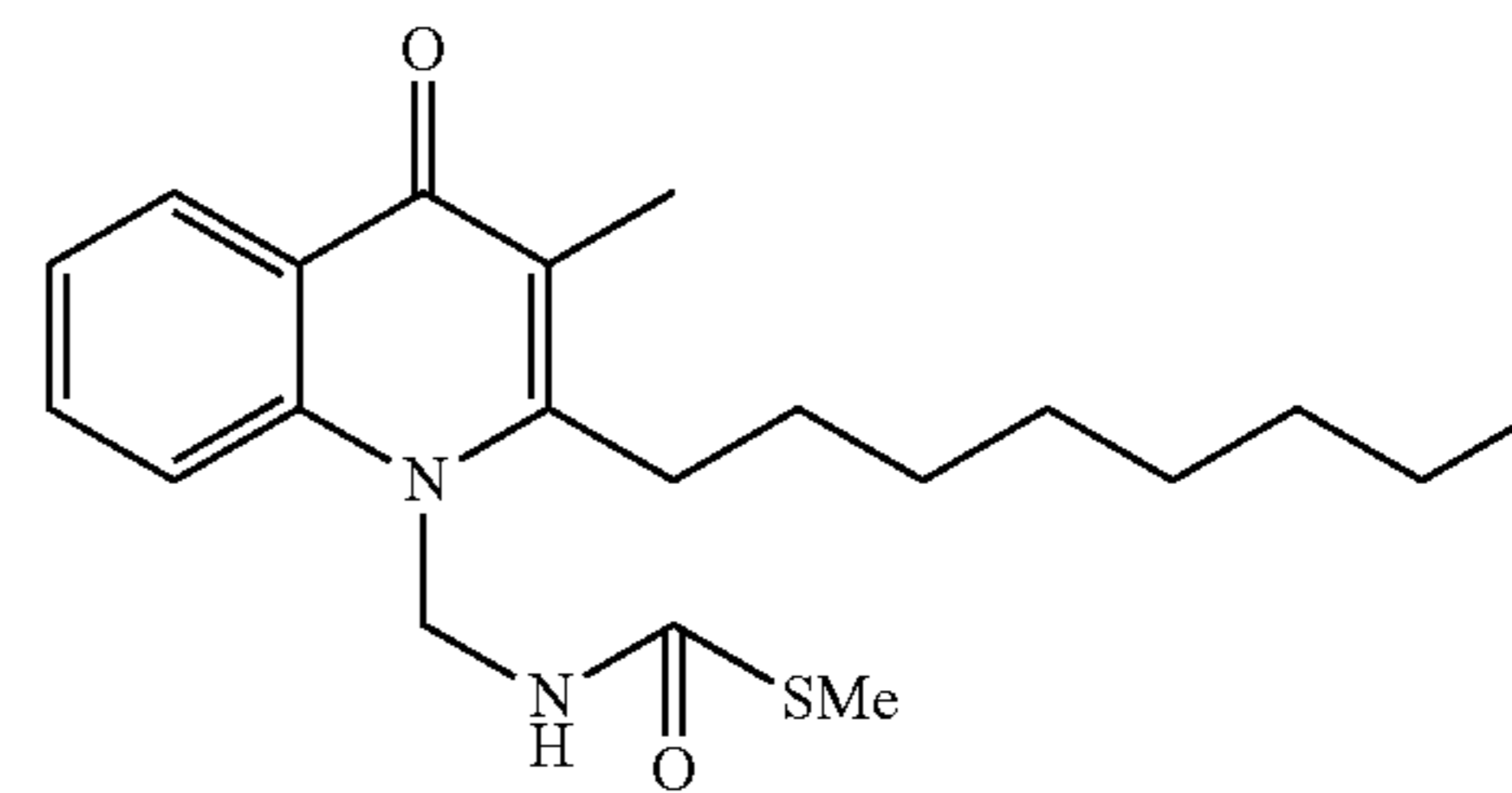
Structural Formula (10)
