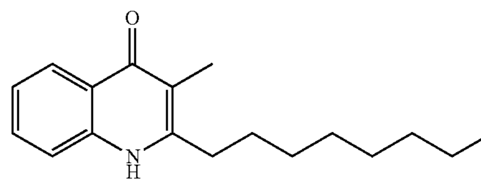
Structural Formula (7)
