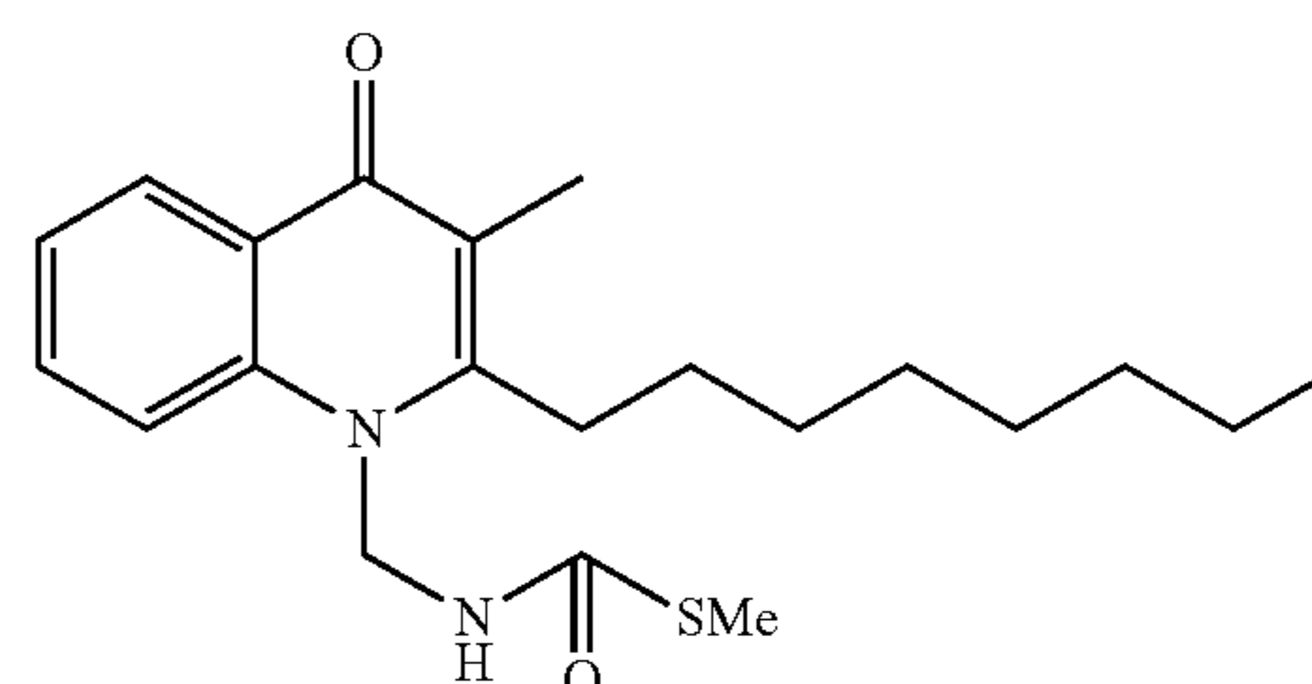
Structural Formula (10)
