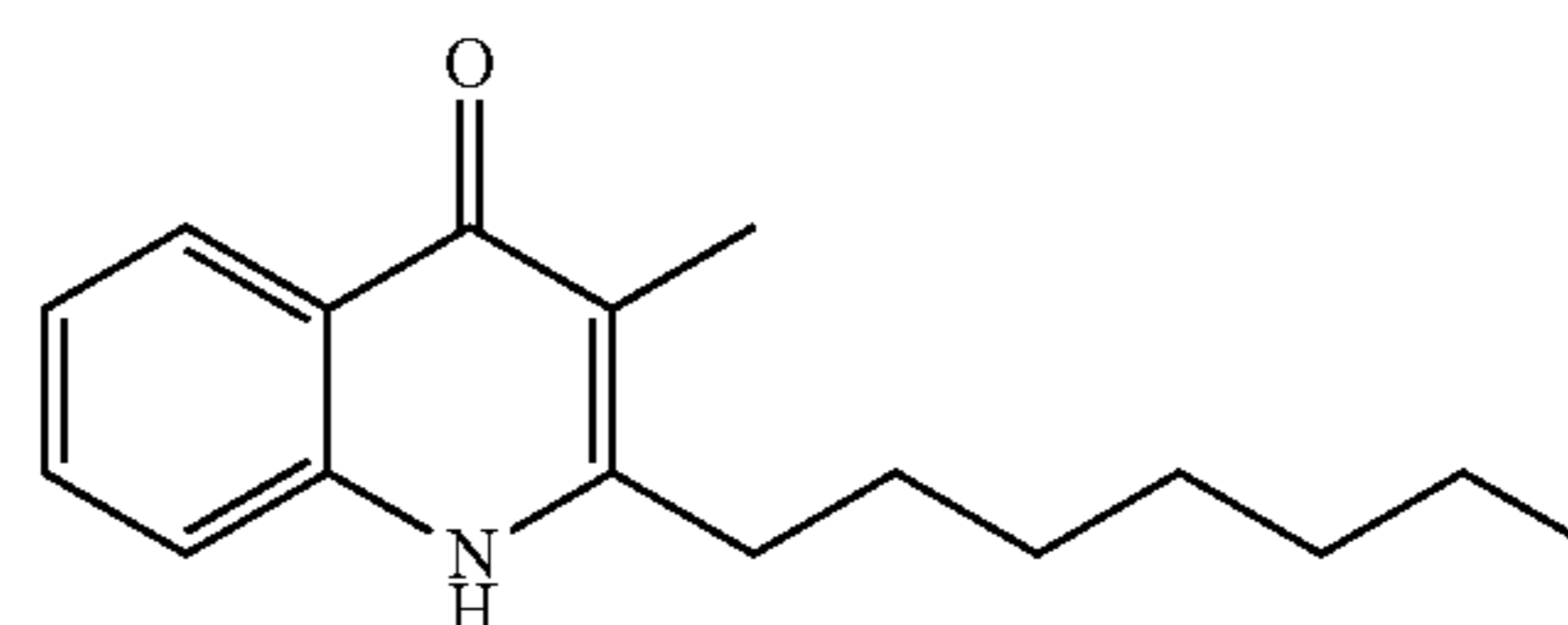
Structural Formula (20)
