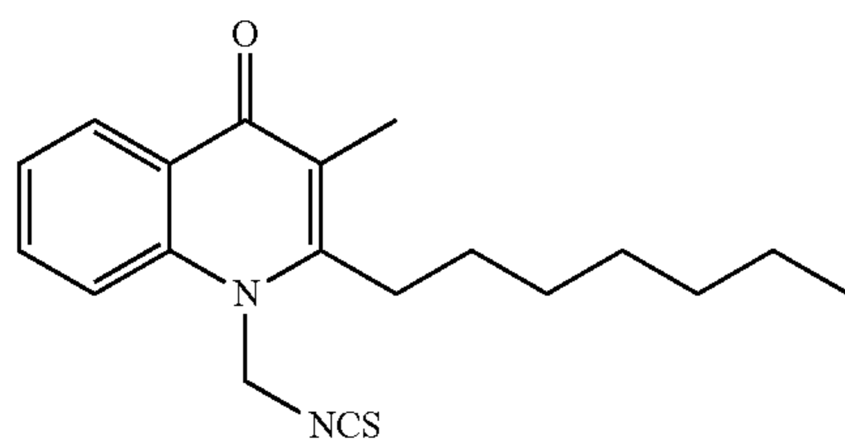
Structural Formula (12)
