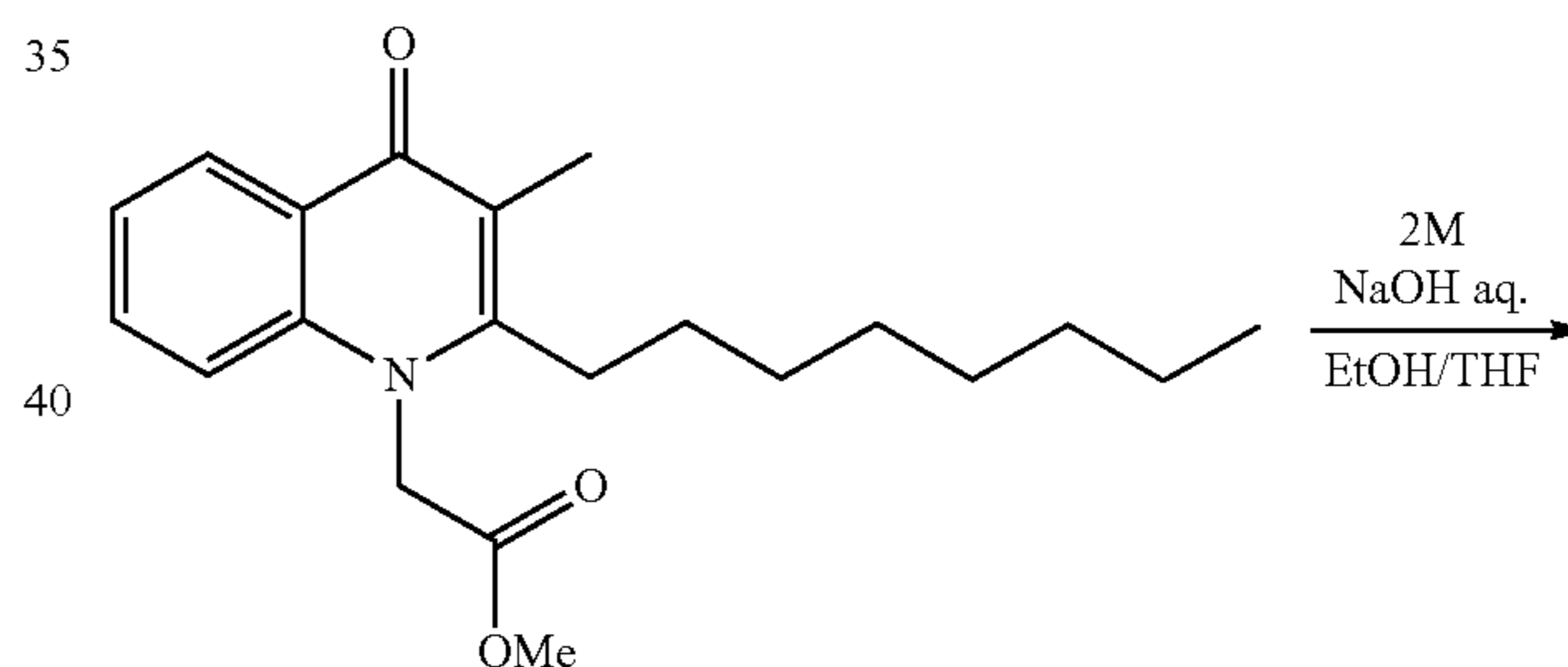
Structural Formula (5)
