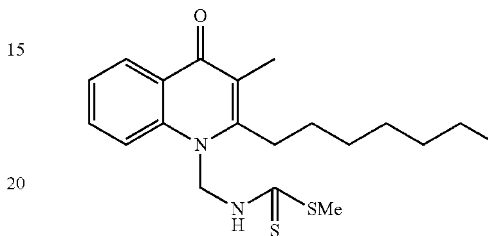
Structural Formula (13)
