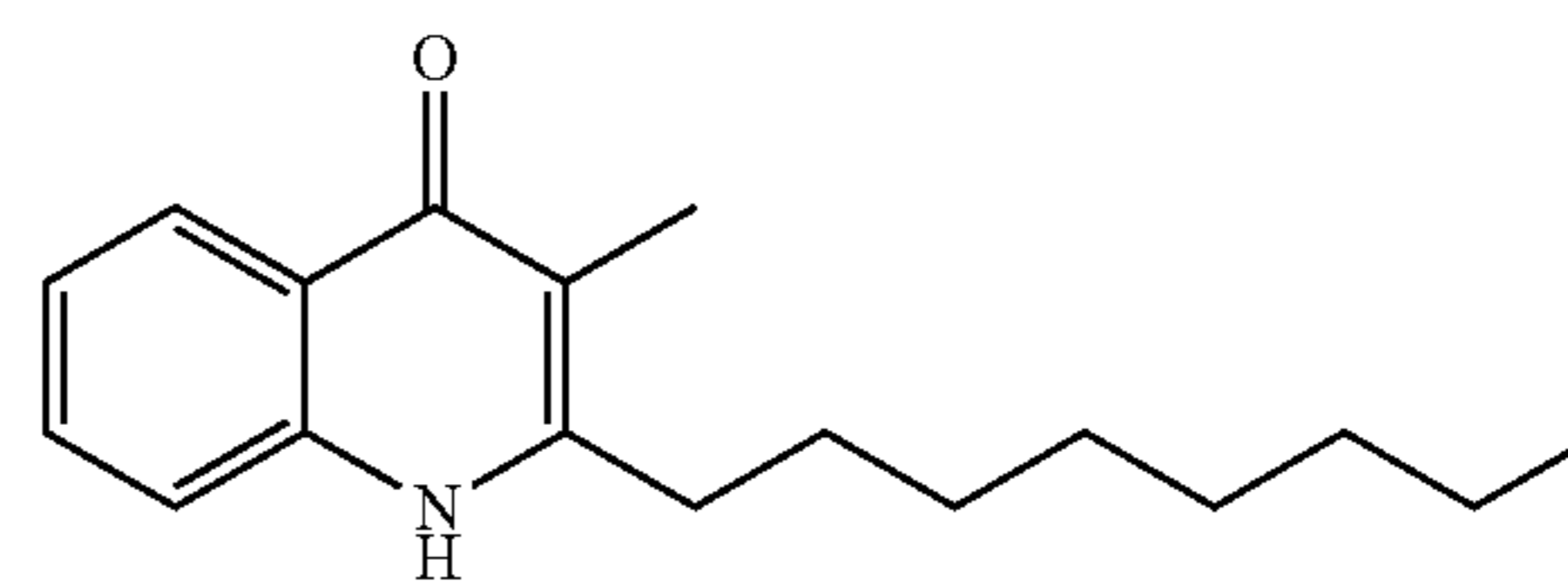
Structural Formula (7)
