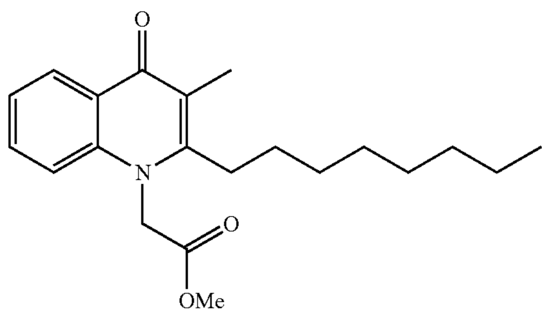
Structural Formula (6)
