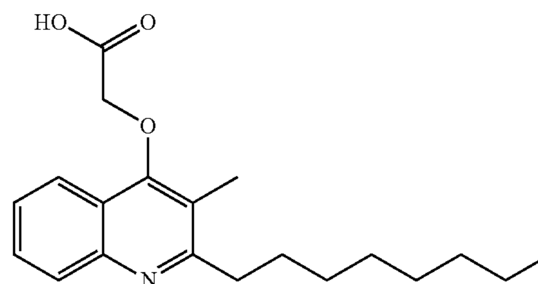
Structural Formula (2)
