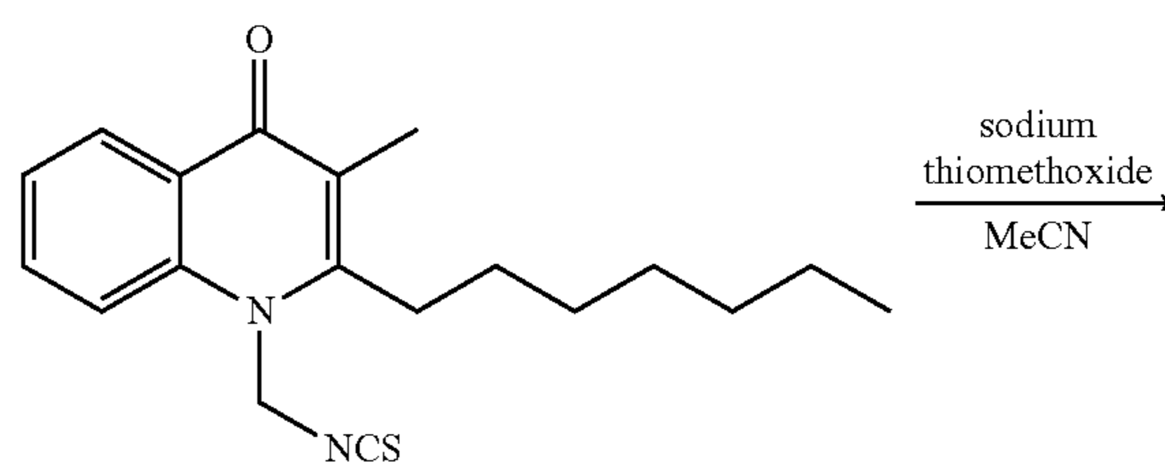
Structural Formula (11)
