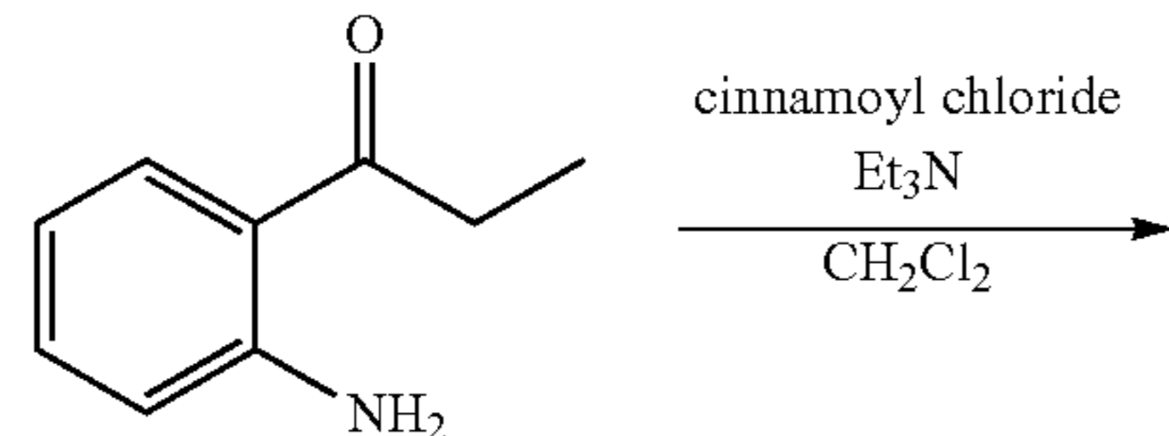
Structural Formula (14)
