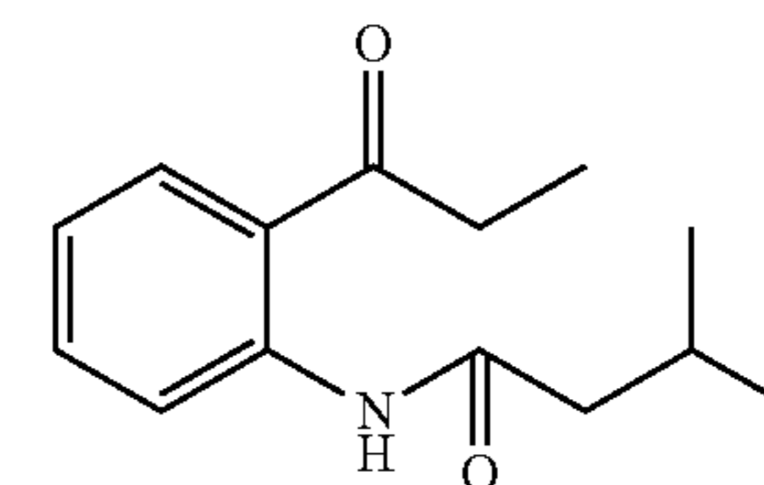
Structural Formula (18)
