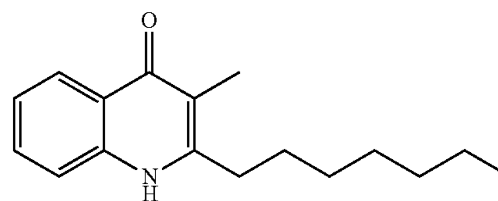
Structural Formula (20)
