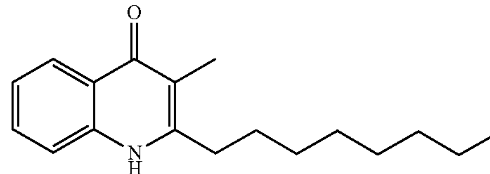
Structural Formula (21)
