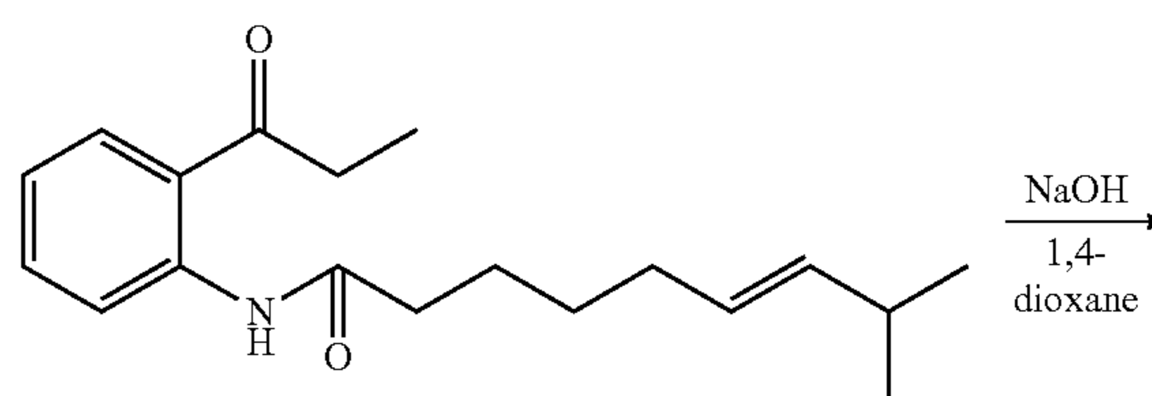
Structural Formula (17)
