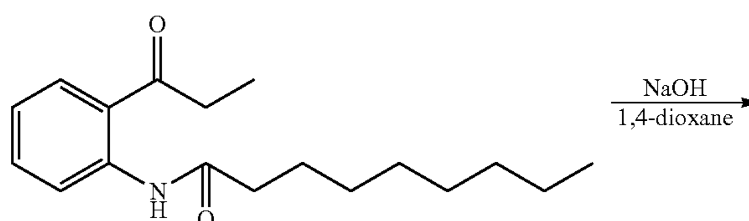
Structural Formula (16)
