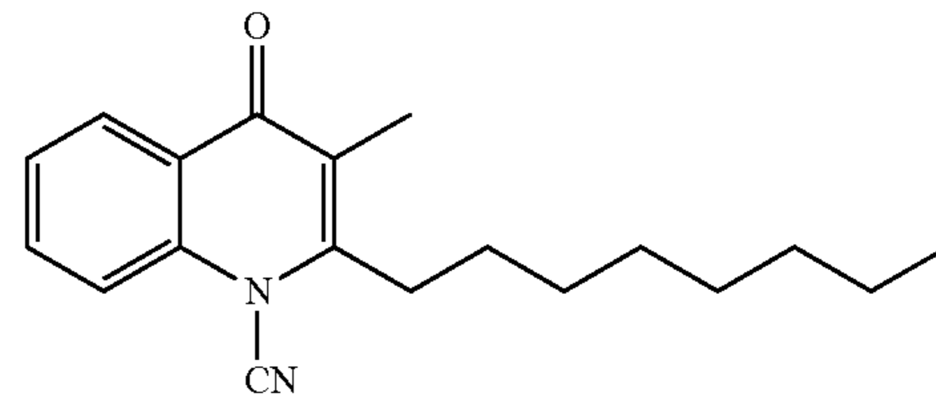
Structural Formula (8)
