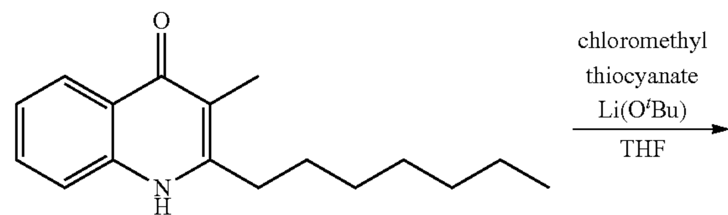
Structural Formula (20)
