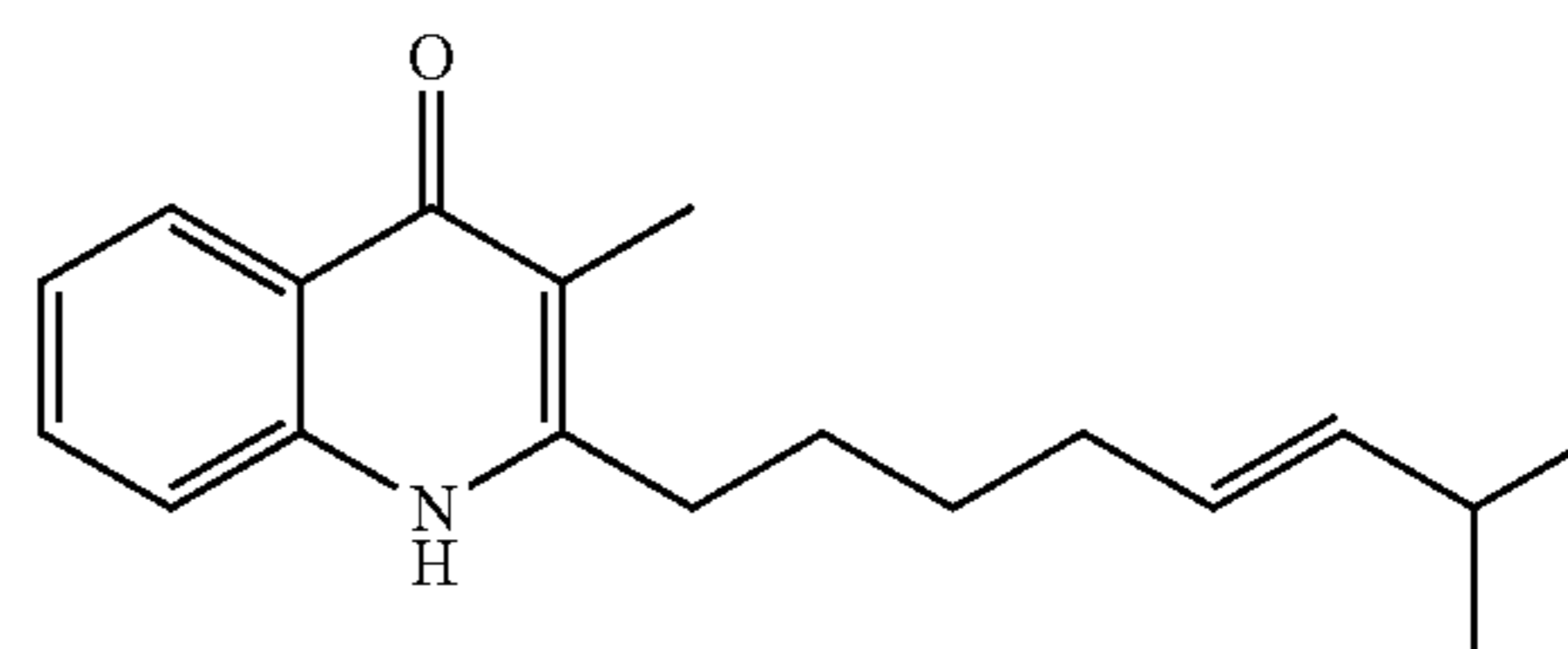
Structural Formula (3)
