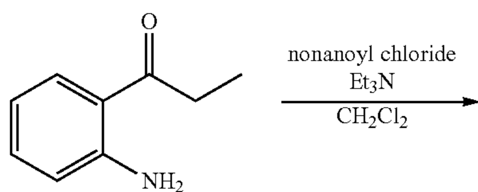
Structural Formula (14)
