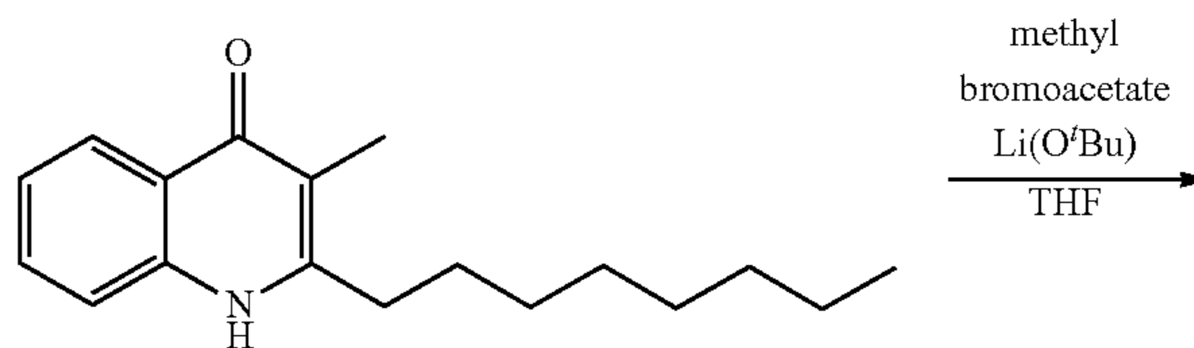
Structural Formula (21)
