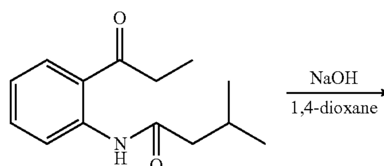
Structural Formula (18)
