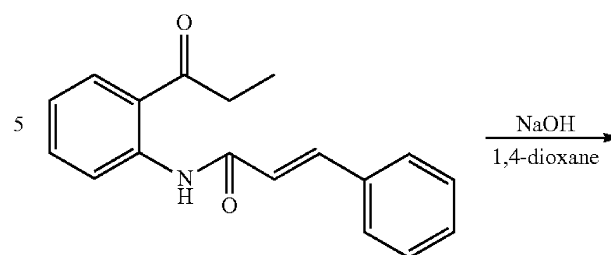
Structural Formula (19)
