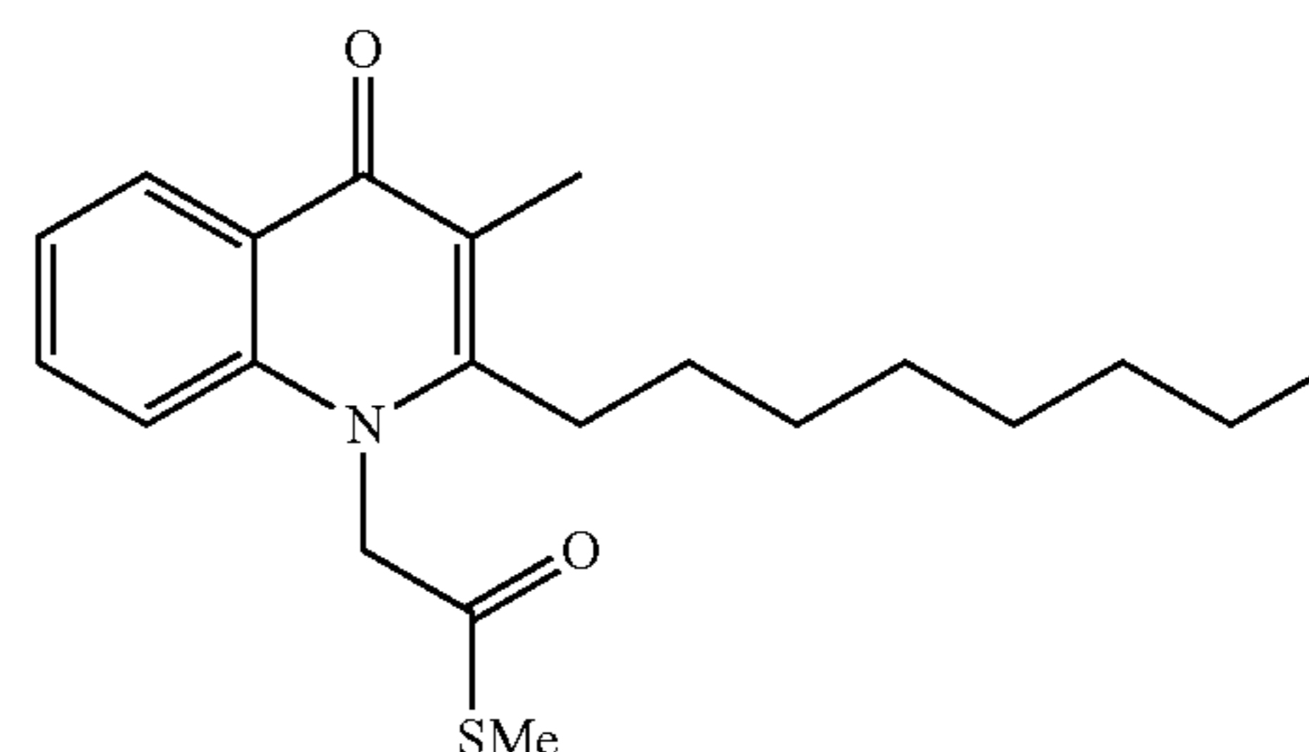
Structural Formula (9)
