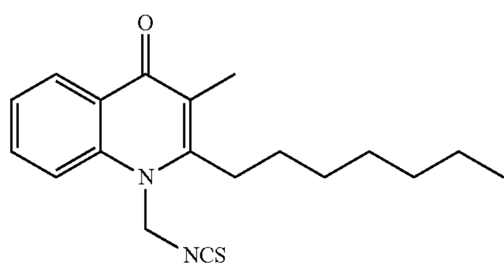
Structural Formula (12)
