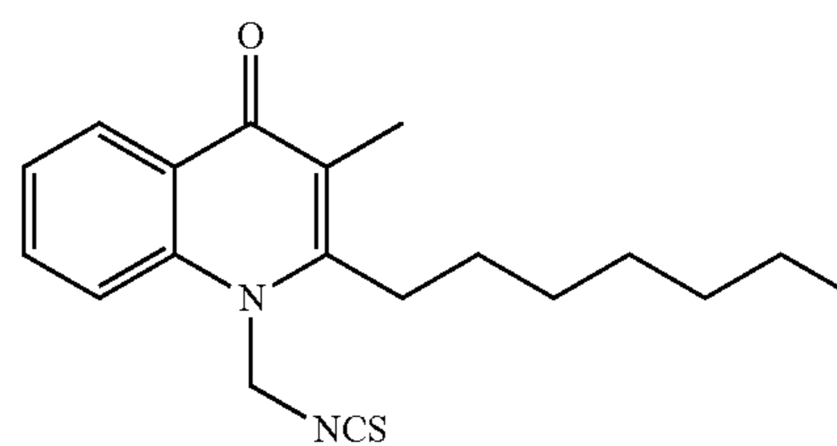
Structural Formula (11)
