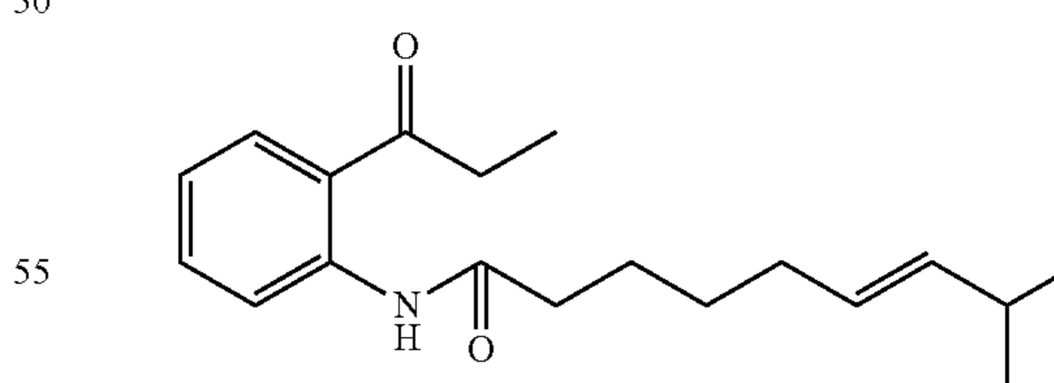
Structural Formula (3)
