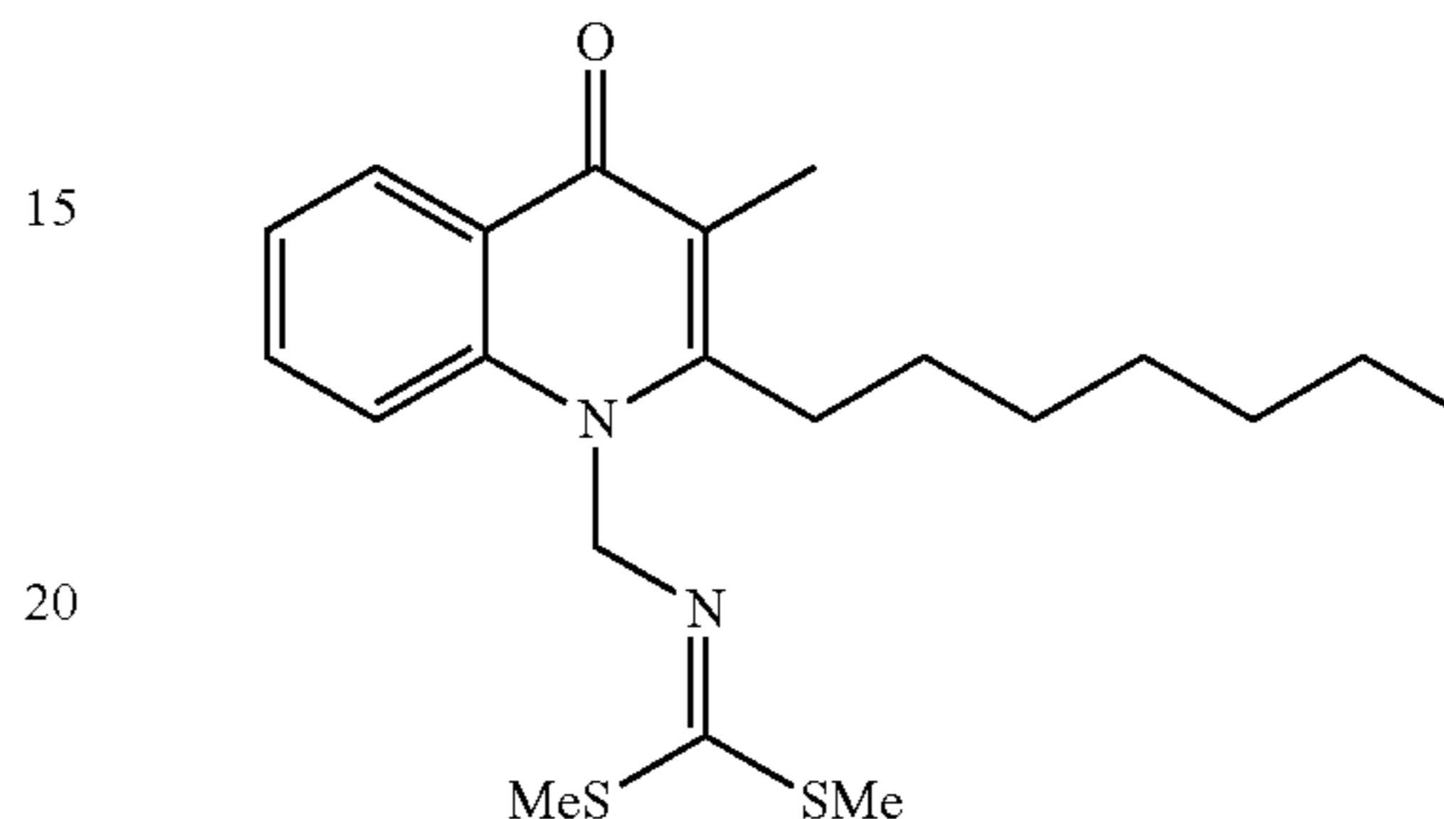
Structural Formula (13)
