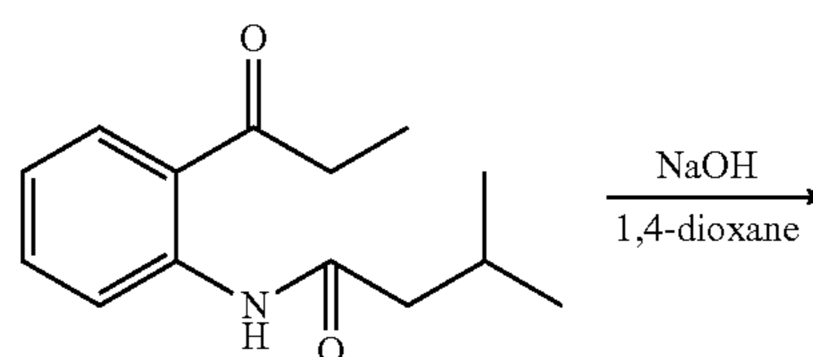
Structural Formula (18)
