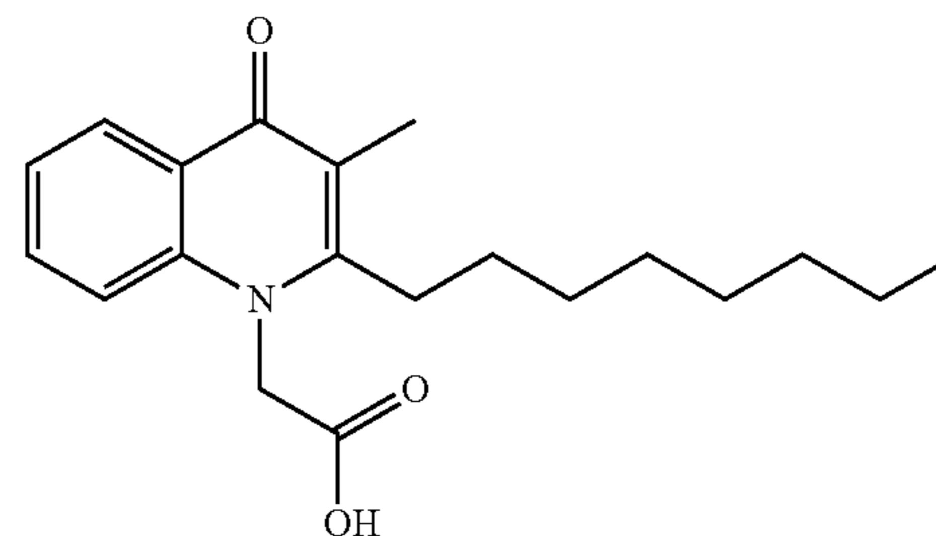
Structural Formula (9)
