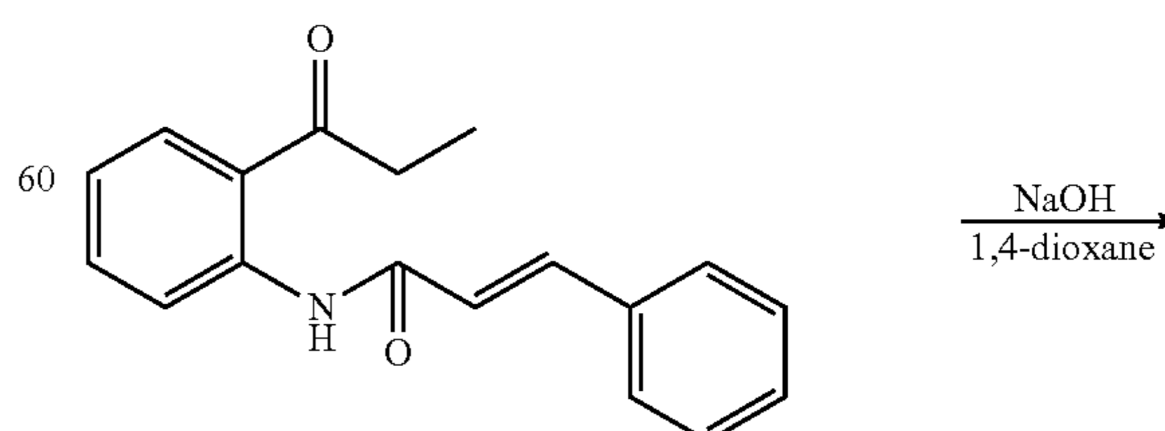
Structural Formula (19)
