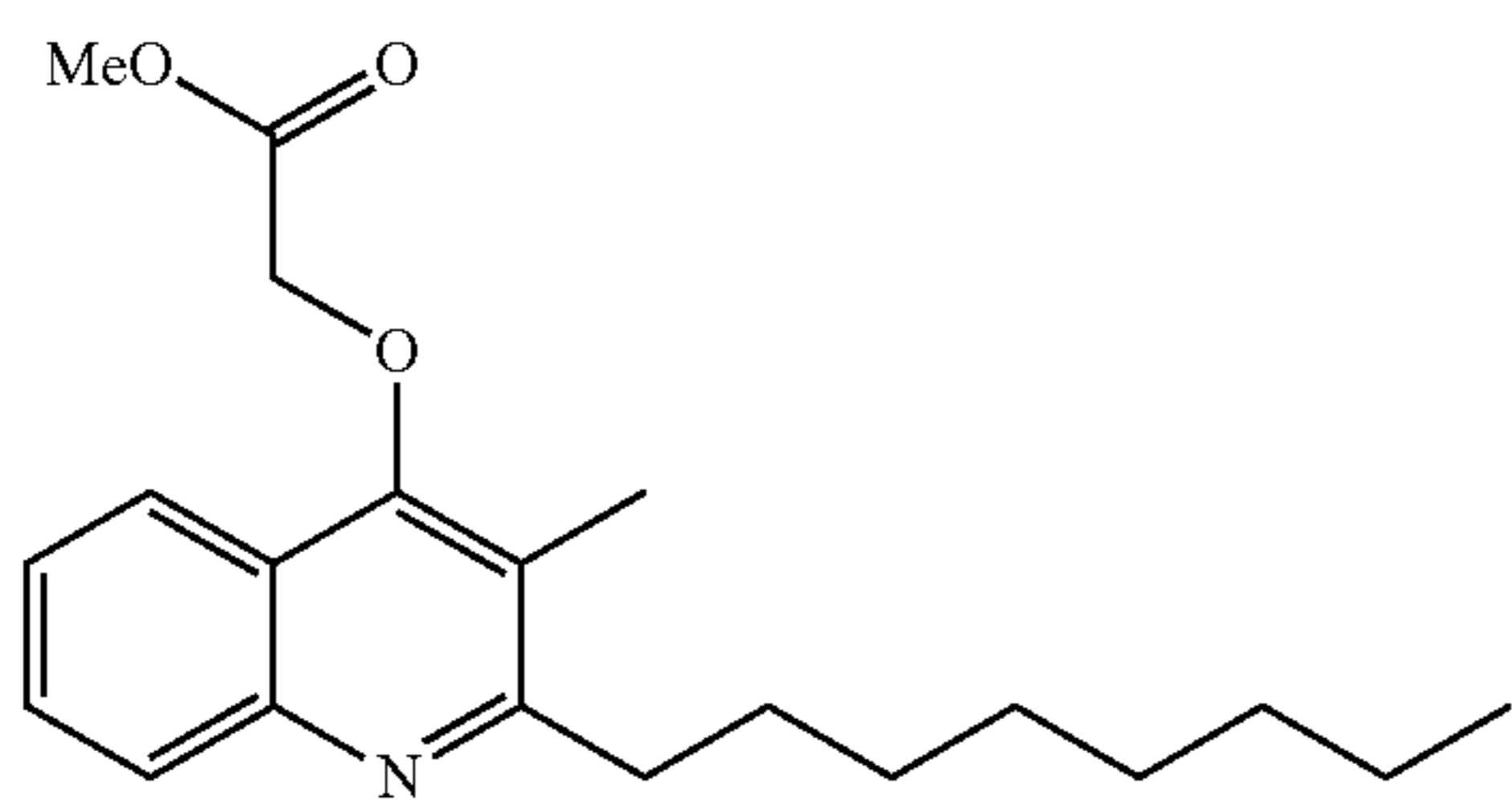
Structural Formula (1)
