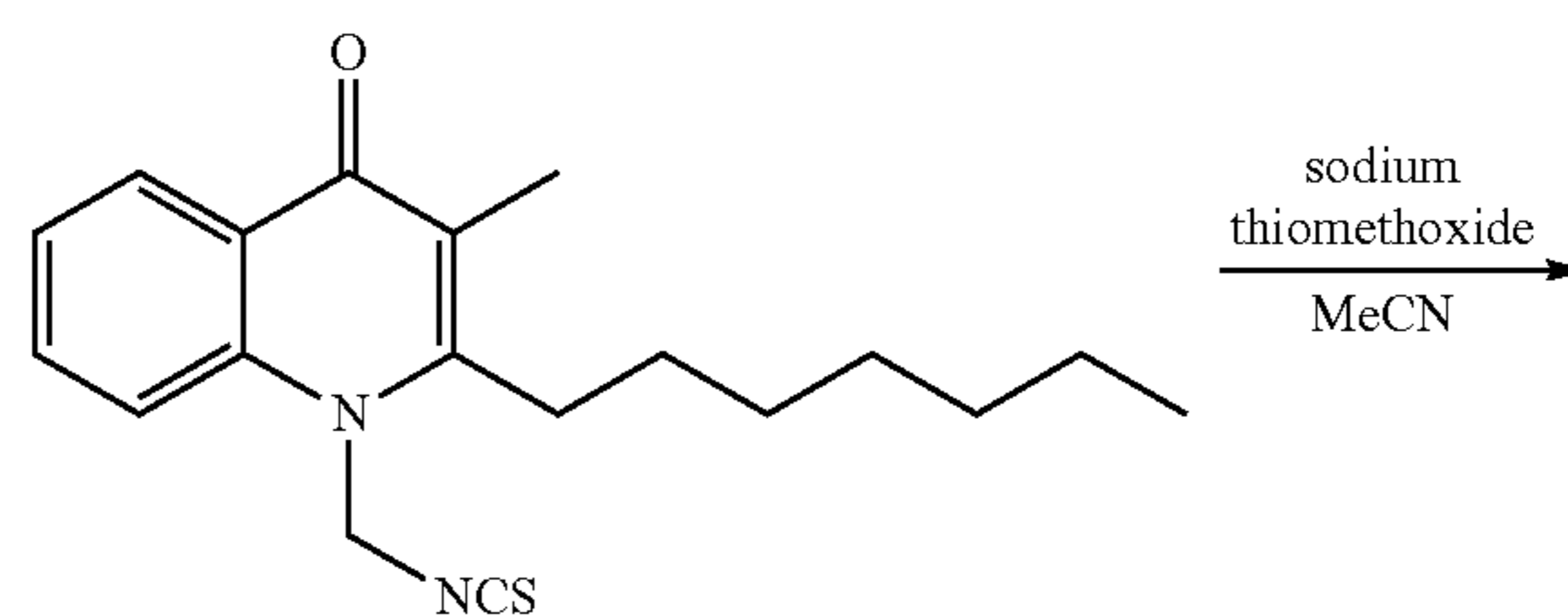
Structural Formula (11)
