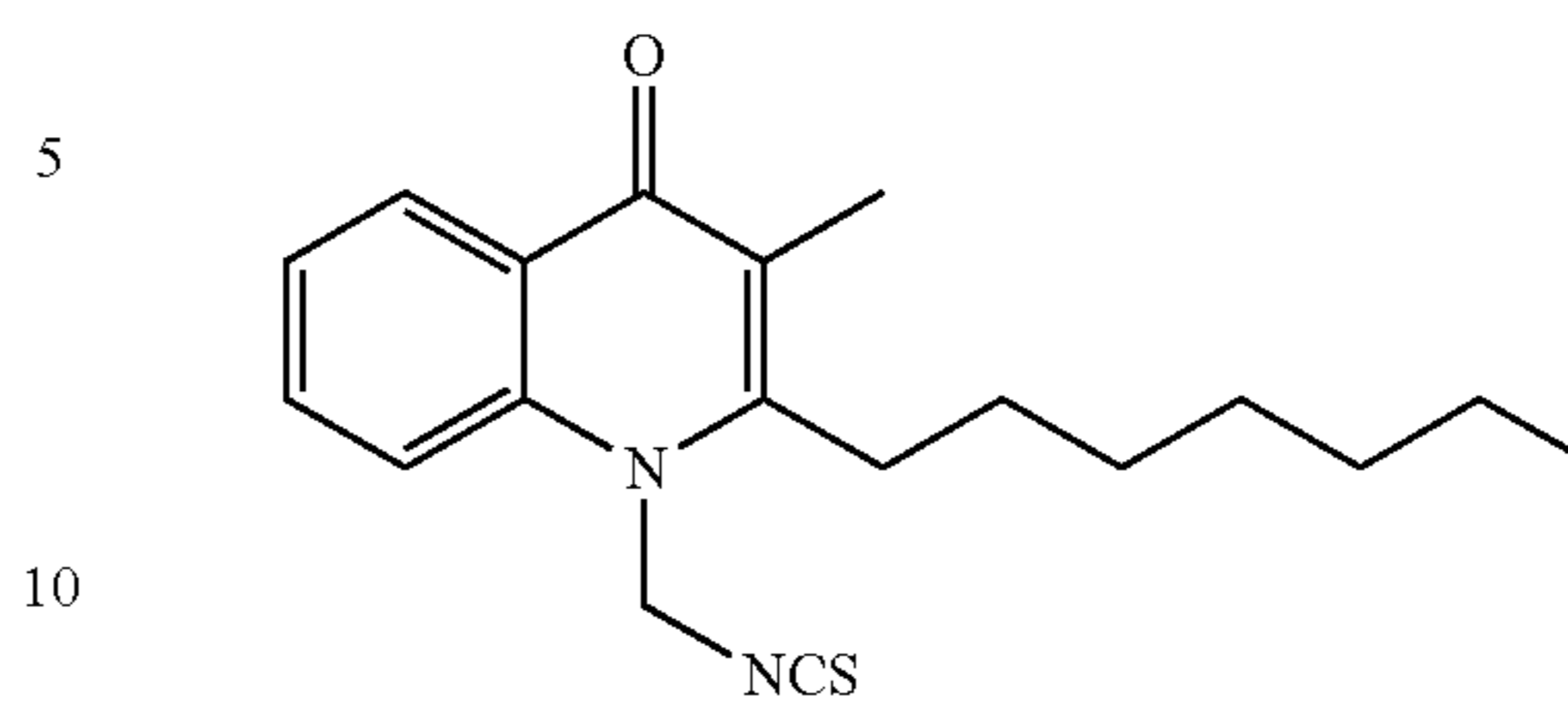
Structural Formula (12)
