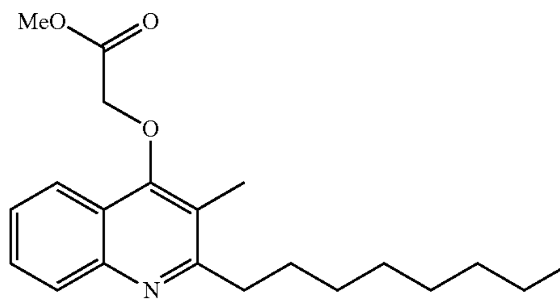
Structural Formula (1)
