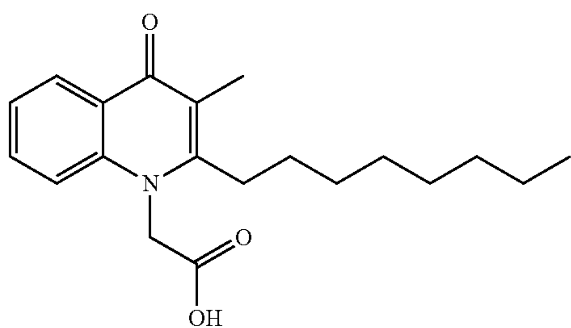
Structural Formula (7)
