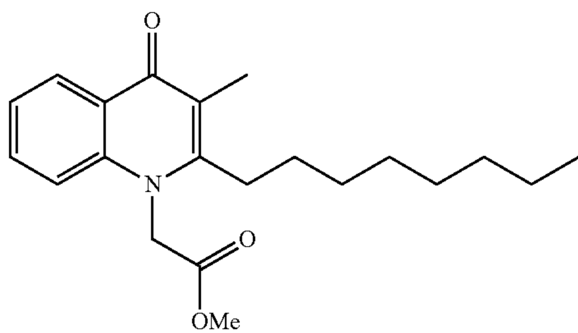
Structural Formula (5)
