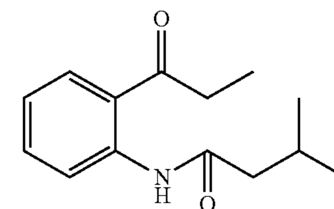
Structural Formula (18)
