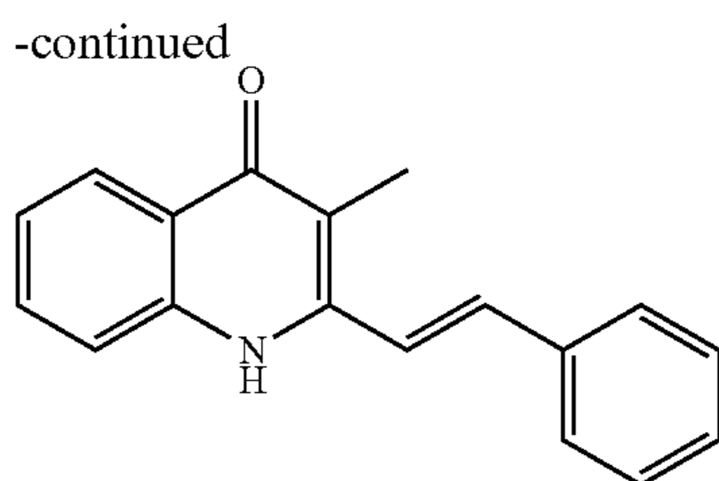
Structural Formula (8)
