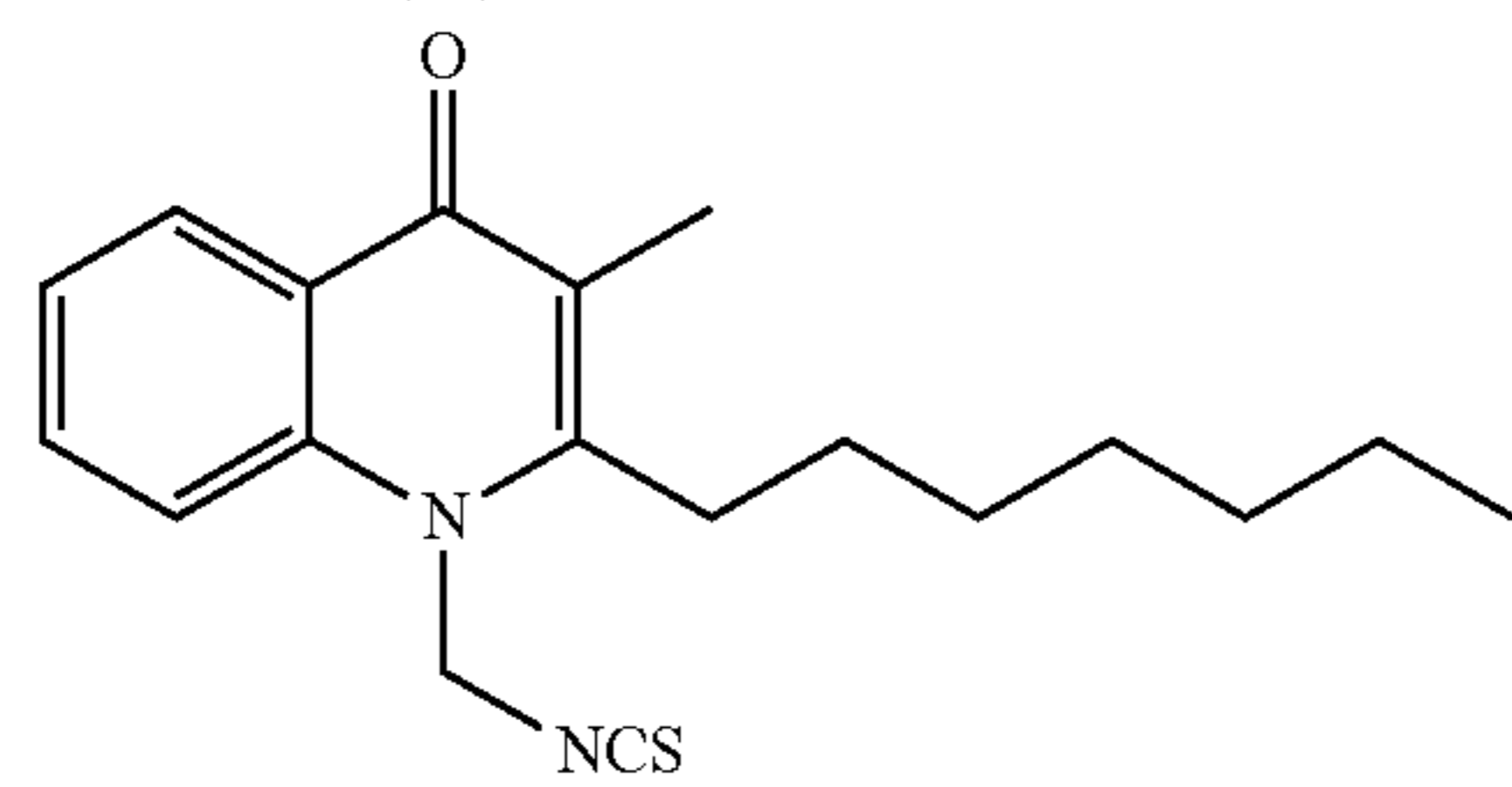
Structural Formula (11)
