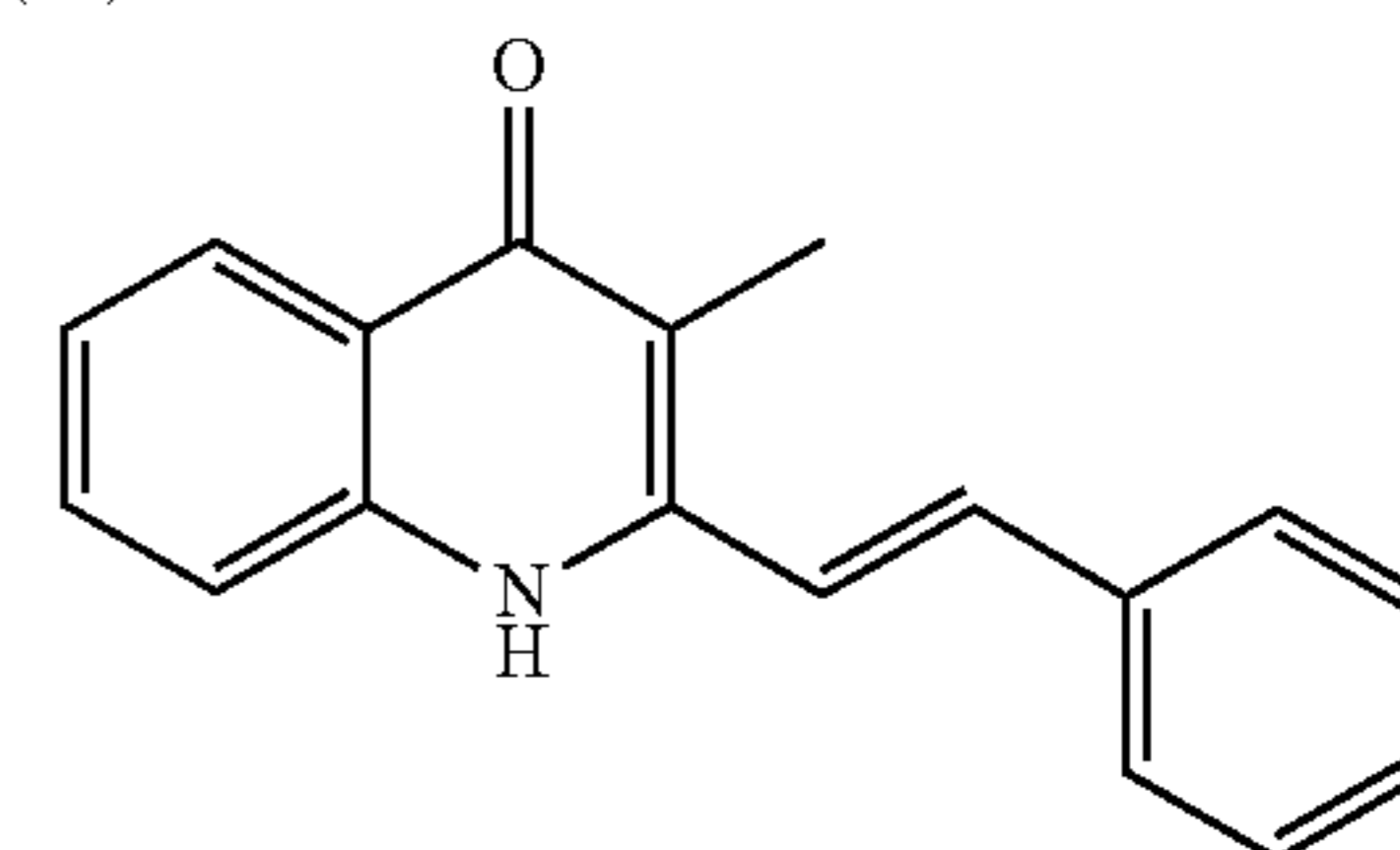
Structural Formula (8)
