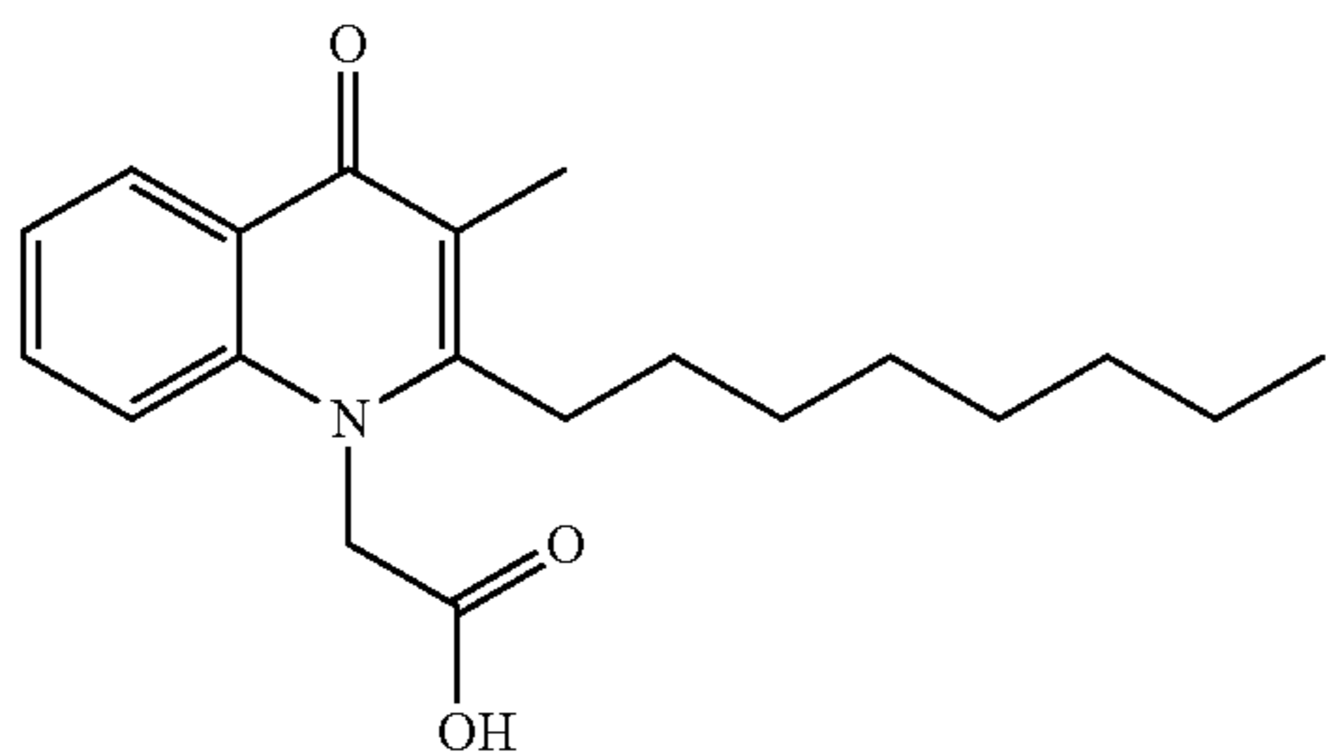
Structural Formula (7)
