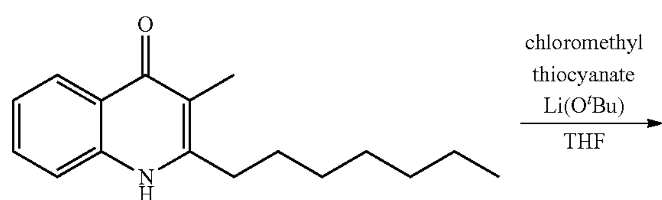
Structural Formula (20)
