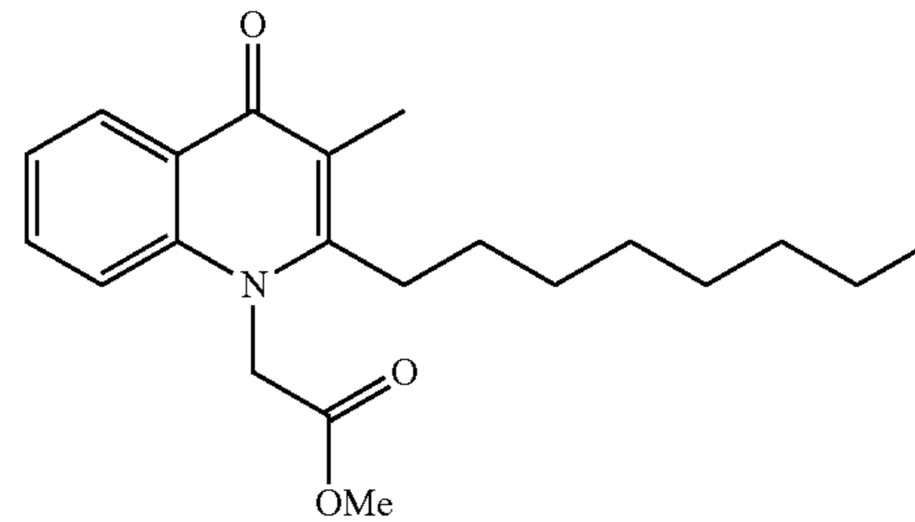
Structural Formula (6)
