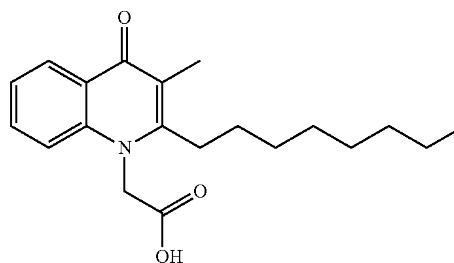
Structural Formula (6)
