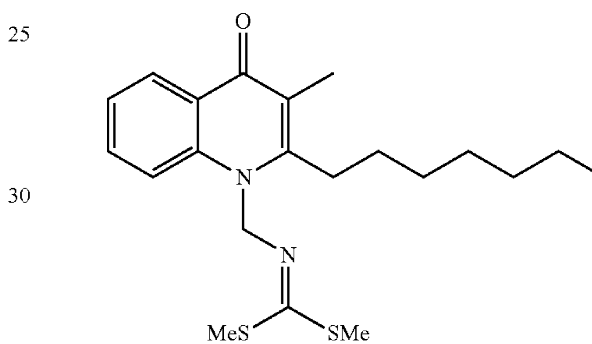
Structural Formula (13)
