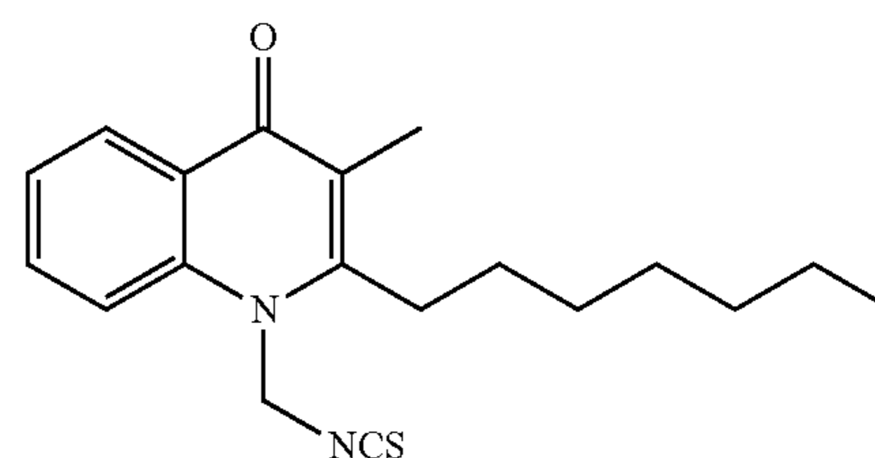
Structural Formula (11)
