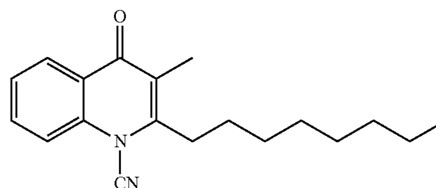
Structural Formula (7)
