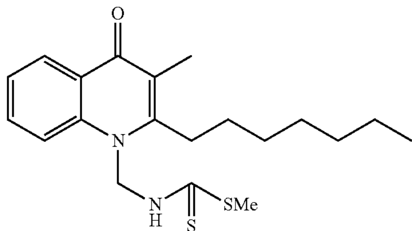
Structural Formula (12)
