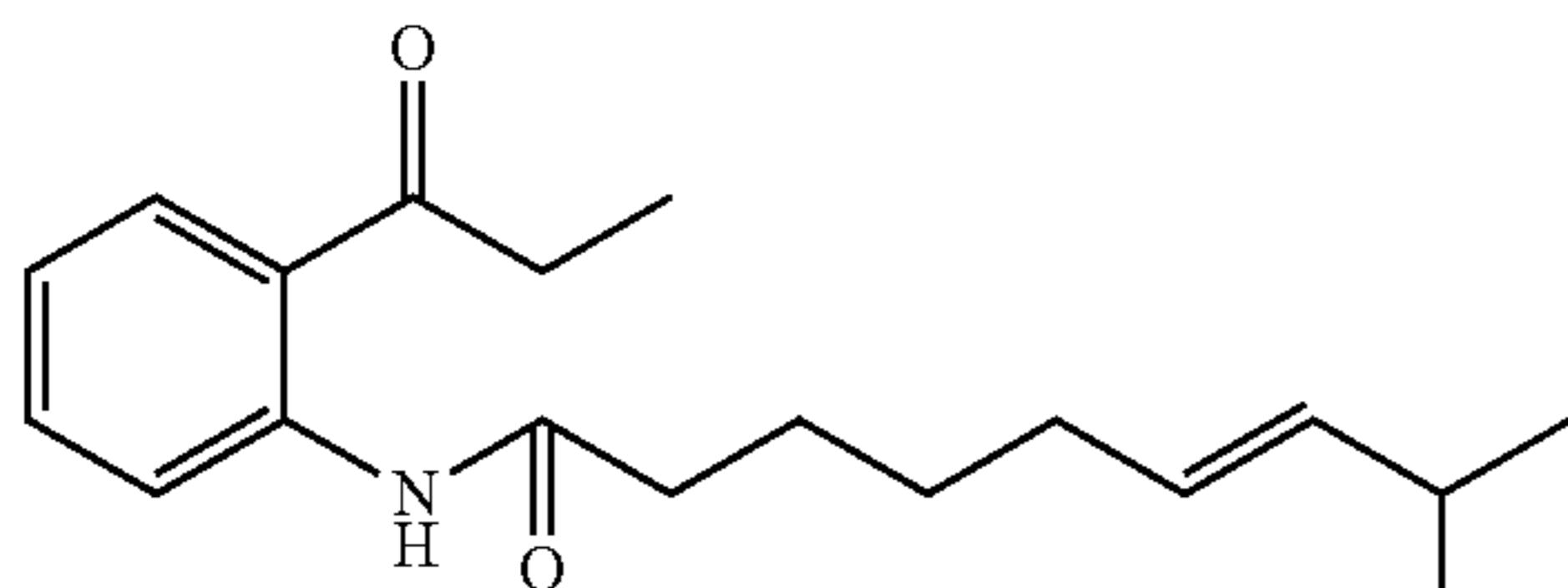
Structural Formula (3)
