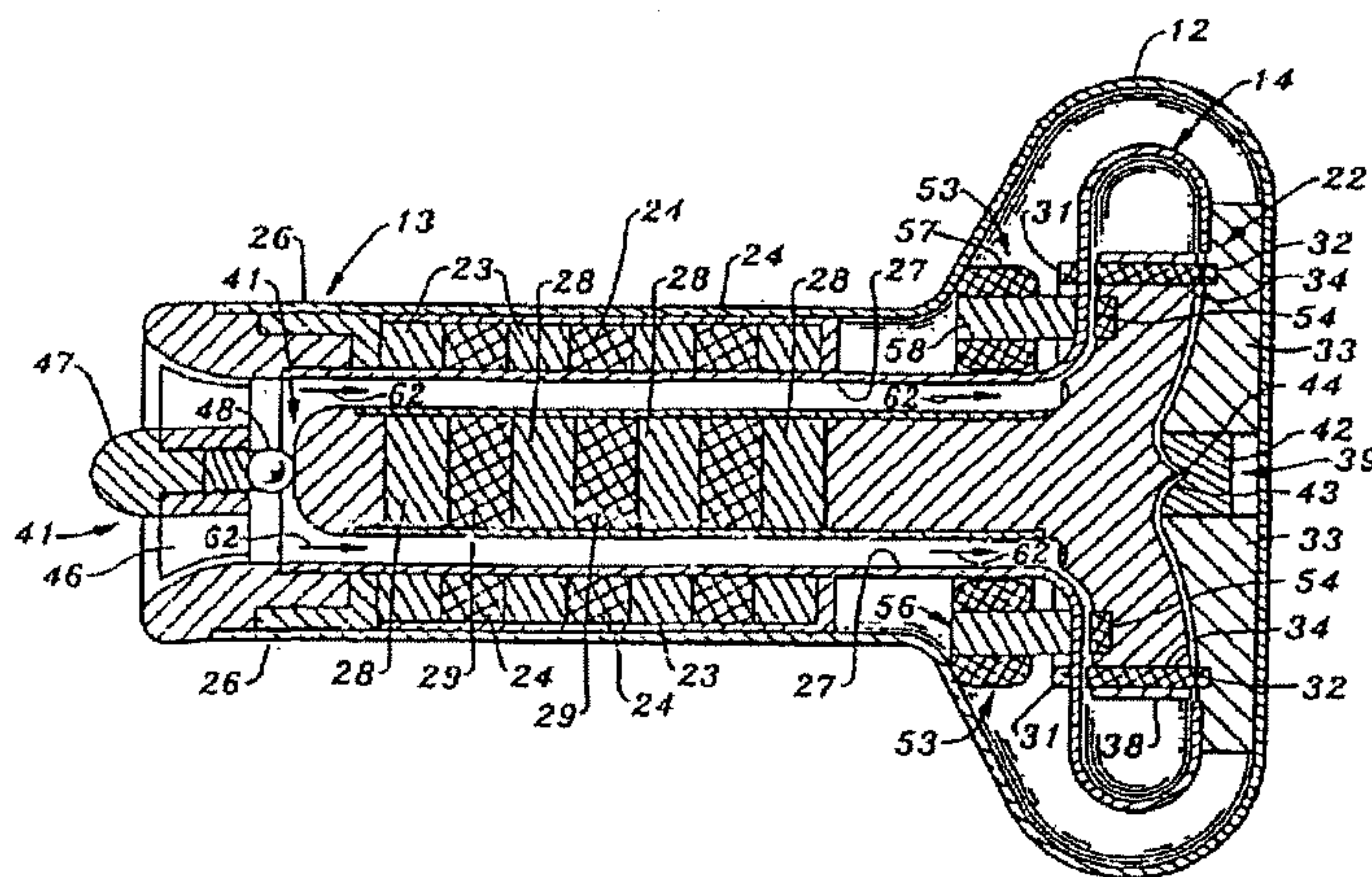
FIG. 2 (Prior Art)
