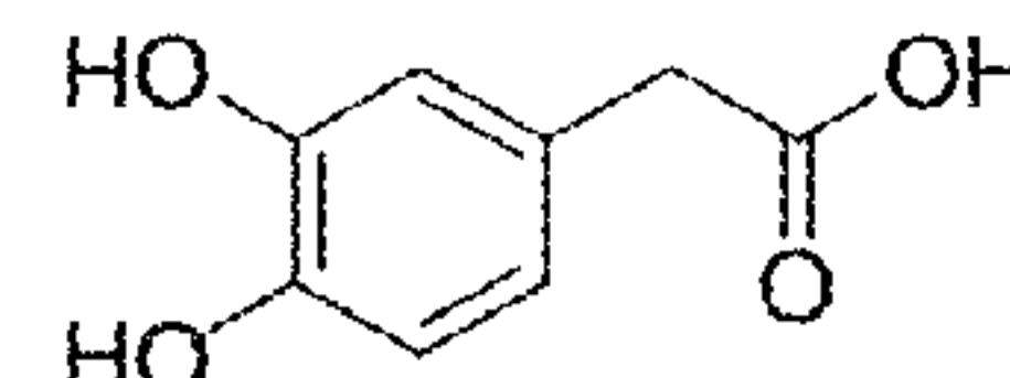
homoprotocatechuic acid
