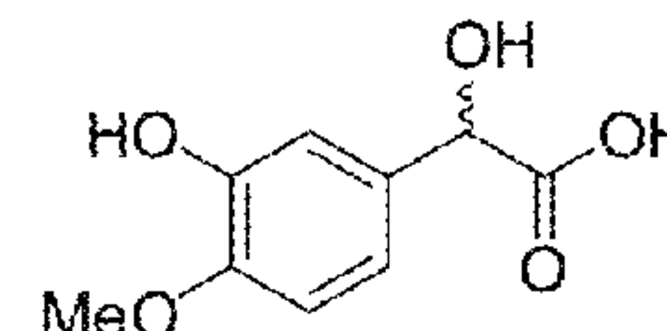
isovanillylmandelic acid
