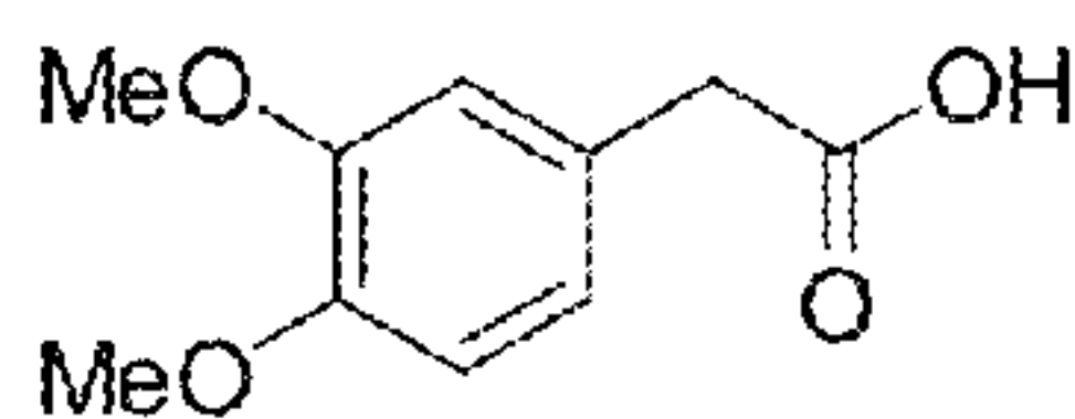
homoveratric acid
