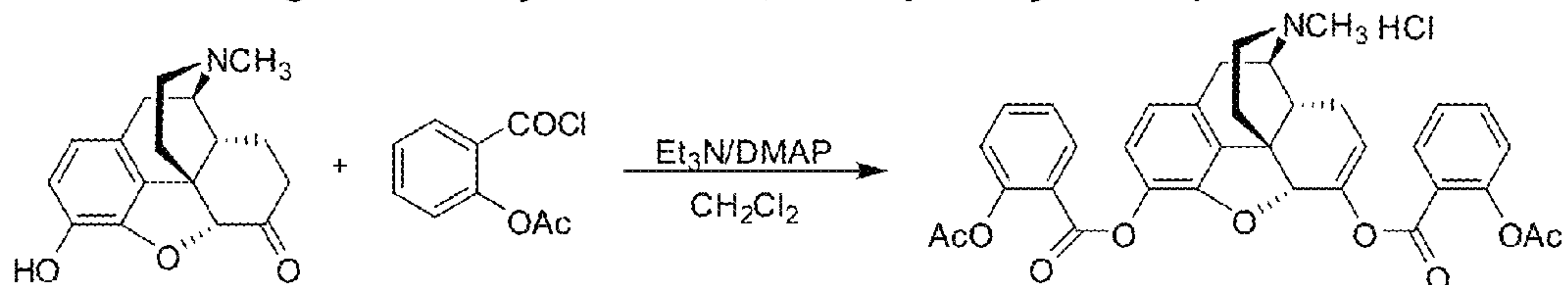
Figure 21D: Synthesis of 3,6-di-aspirin-hydromorphone:
