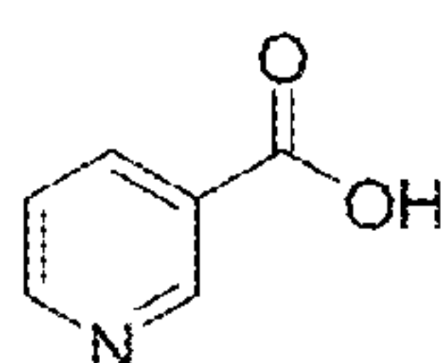
nicotinic acid
