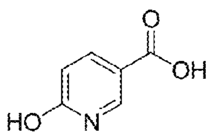
6-hydroxynicotinic acid
