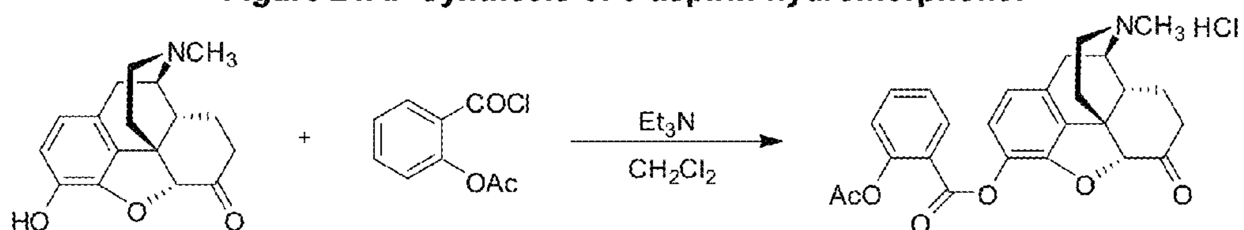
Figure 21A: Synthesis of 3-aspirin-hydromorphone:
