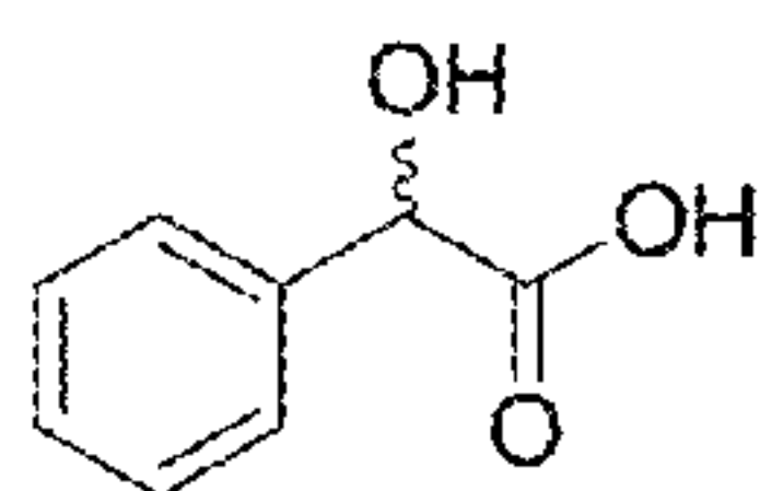
mandelic acid
