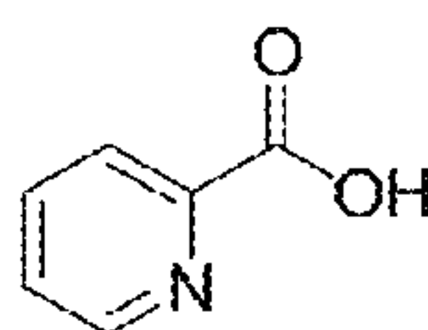
picolinic acid
