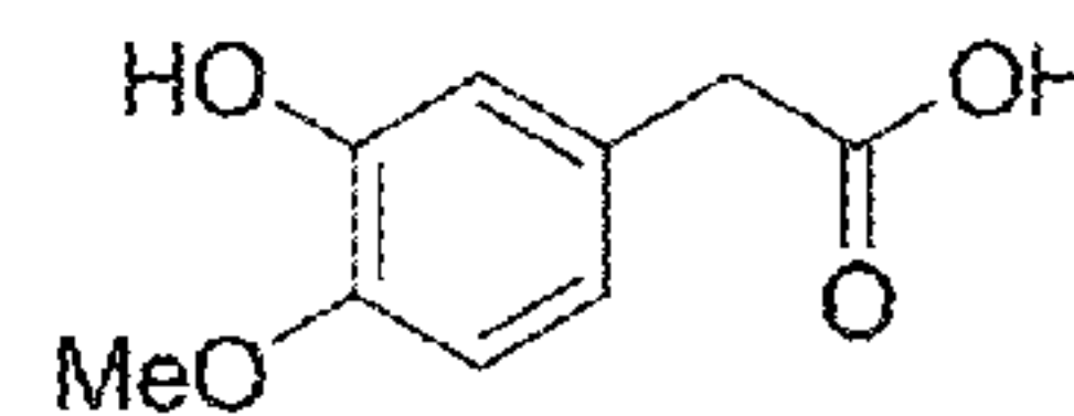
homoisovanillic acid
