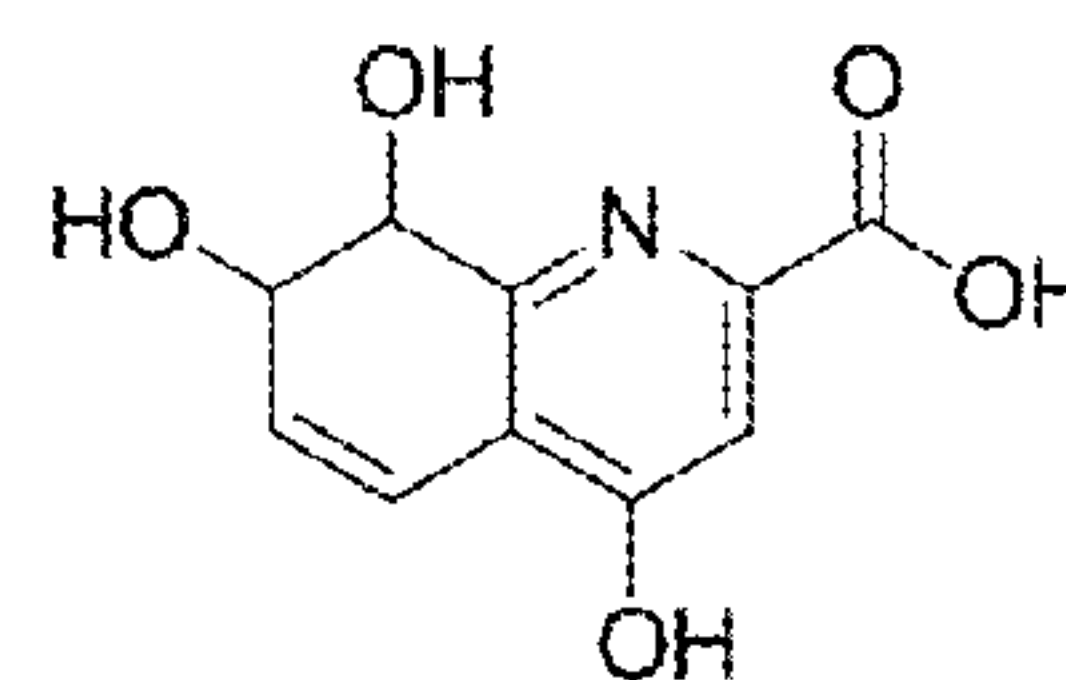
7,8-dihydro-7,8-dihydroxykynurenic acid
