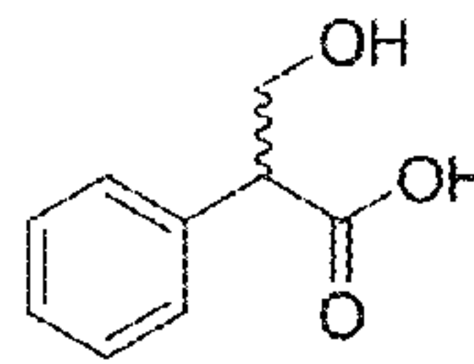
tropic acid
