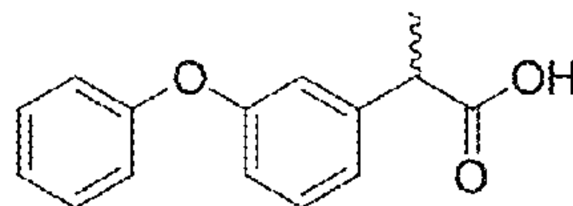
fenoprofen
