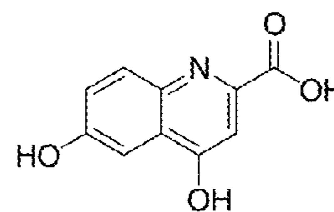
6-hydroxykynurenic acid
