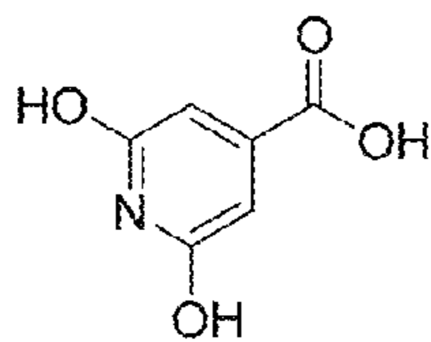
citrazinic acid
