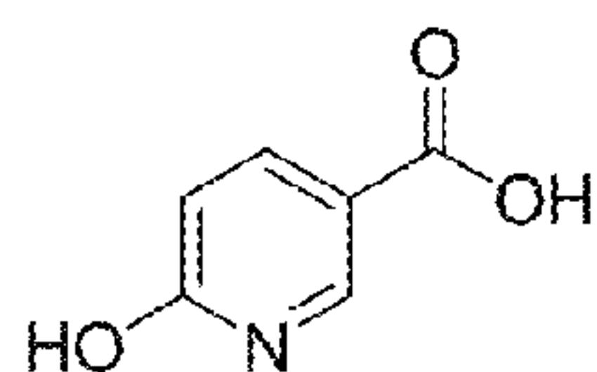
6-hydroxynicotinic acid
