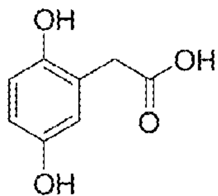
homogentisic acid
