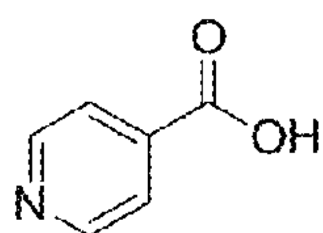
isonicotinic acid
