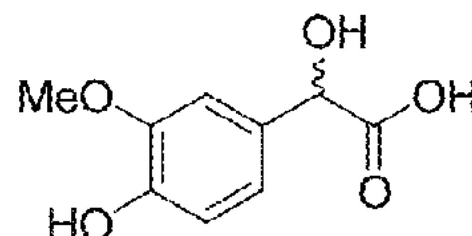
vanillylmandelic acid
