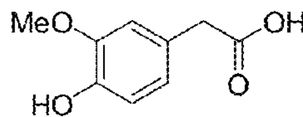
homovanillic acid
