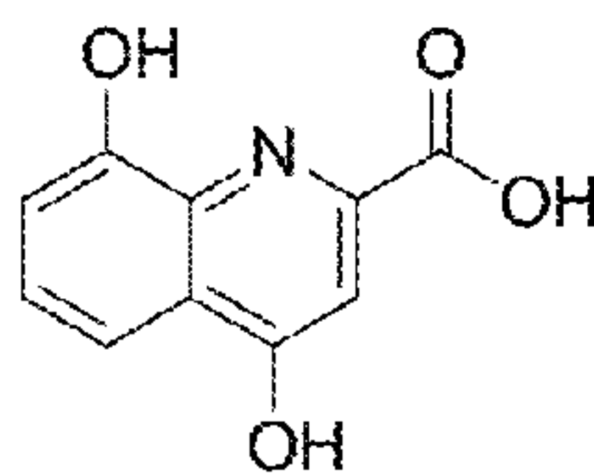
xanthurenic acid
