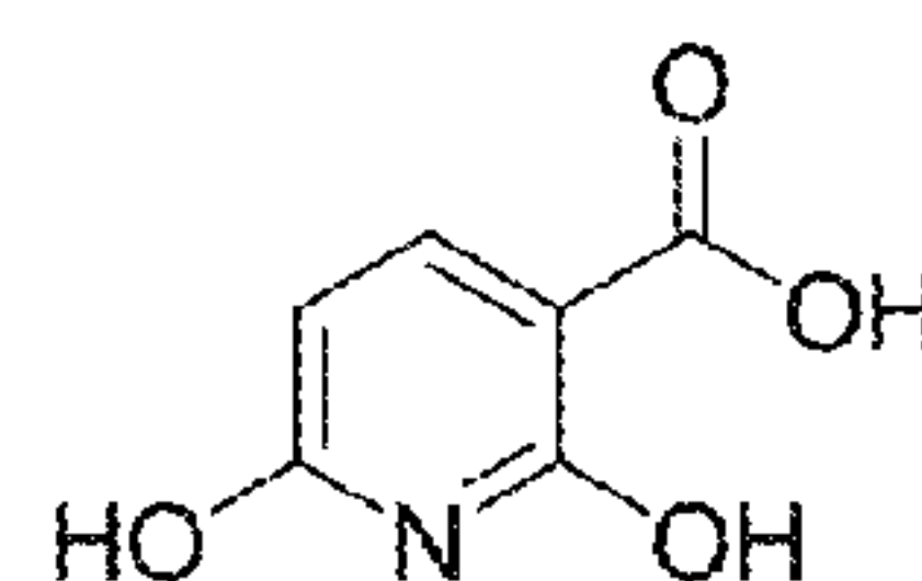
2,6-dihydroxynicotinic acid
