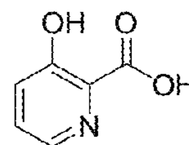
3-hydroxypicolinic acid
