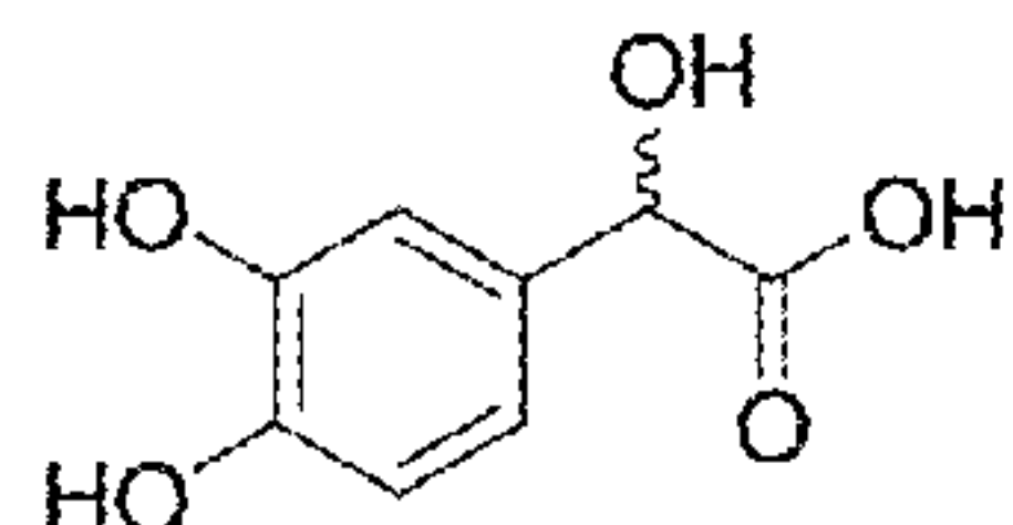
3,4-dihydroxymandelic acid
