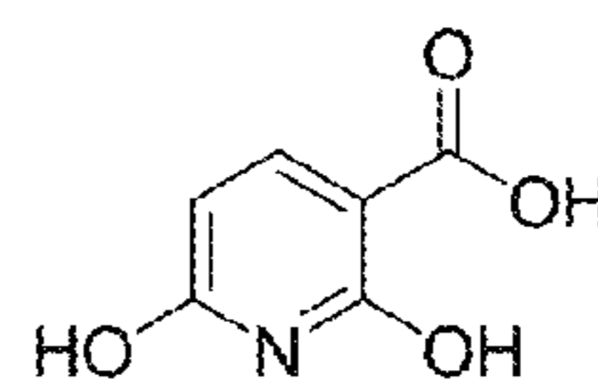
2,6-dihydroxynicotinic acid
