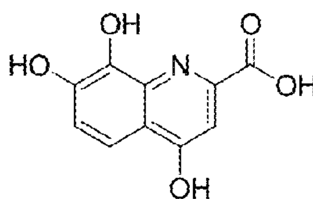
7,8-dihydroxykynurenic acid
