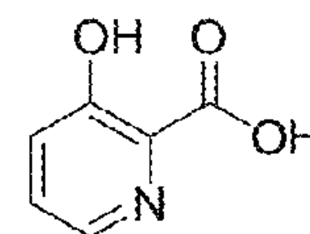
3-hydroxypicolinic acid
