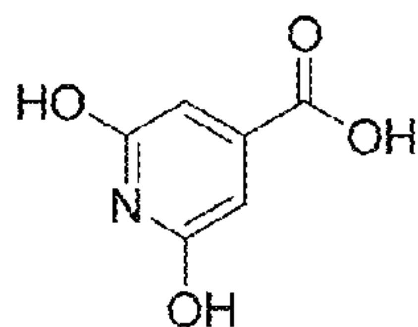
citrazinic acid
