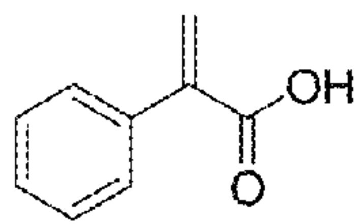
atropic acid
