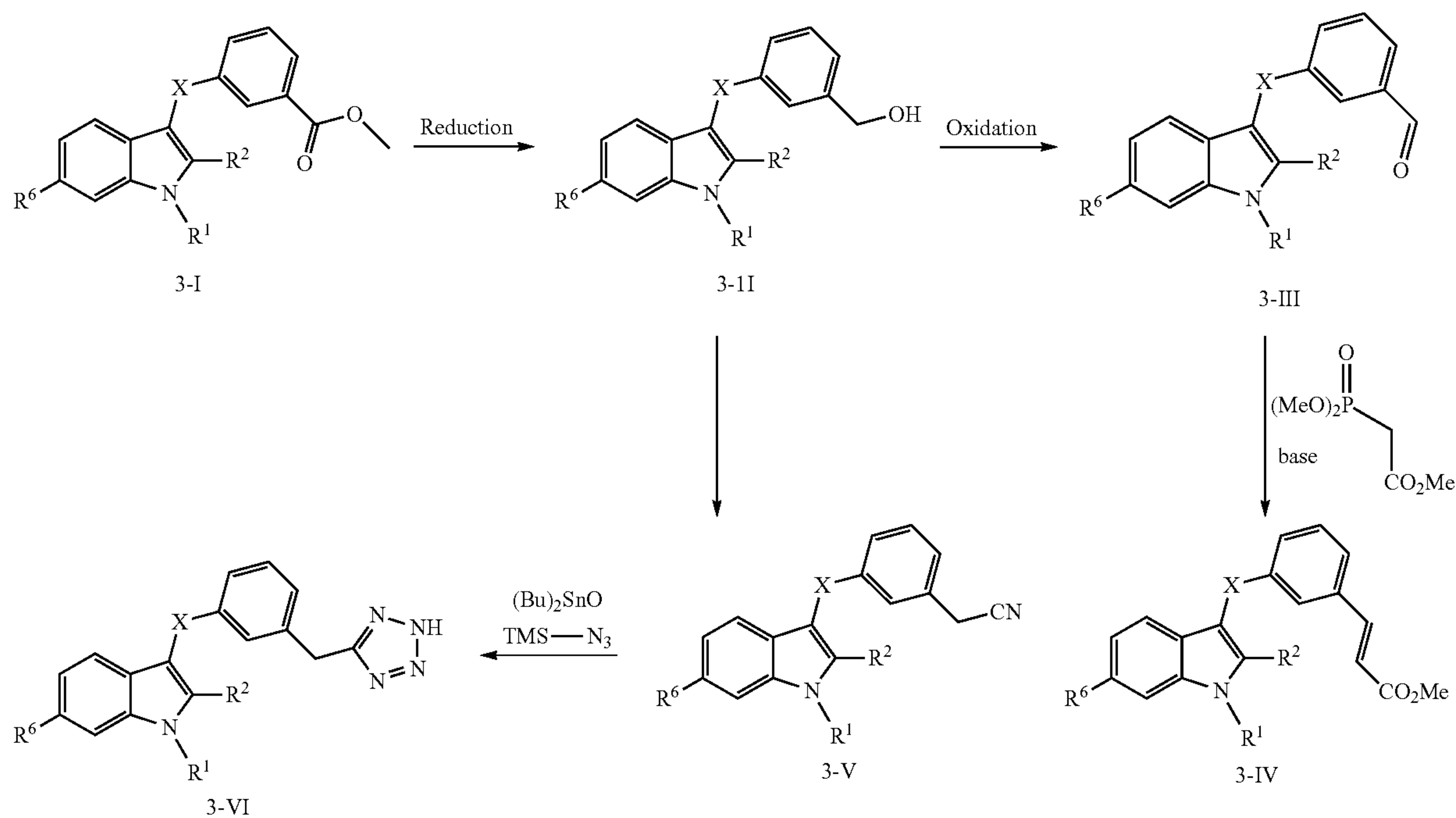
Scheme 3.
