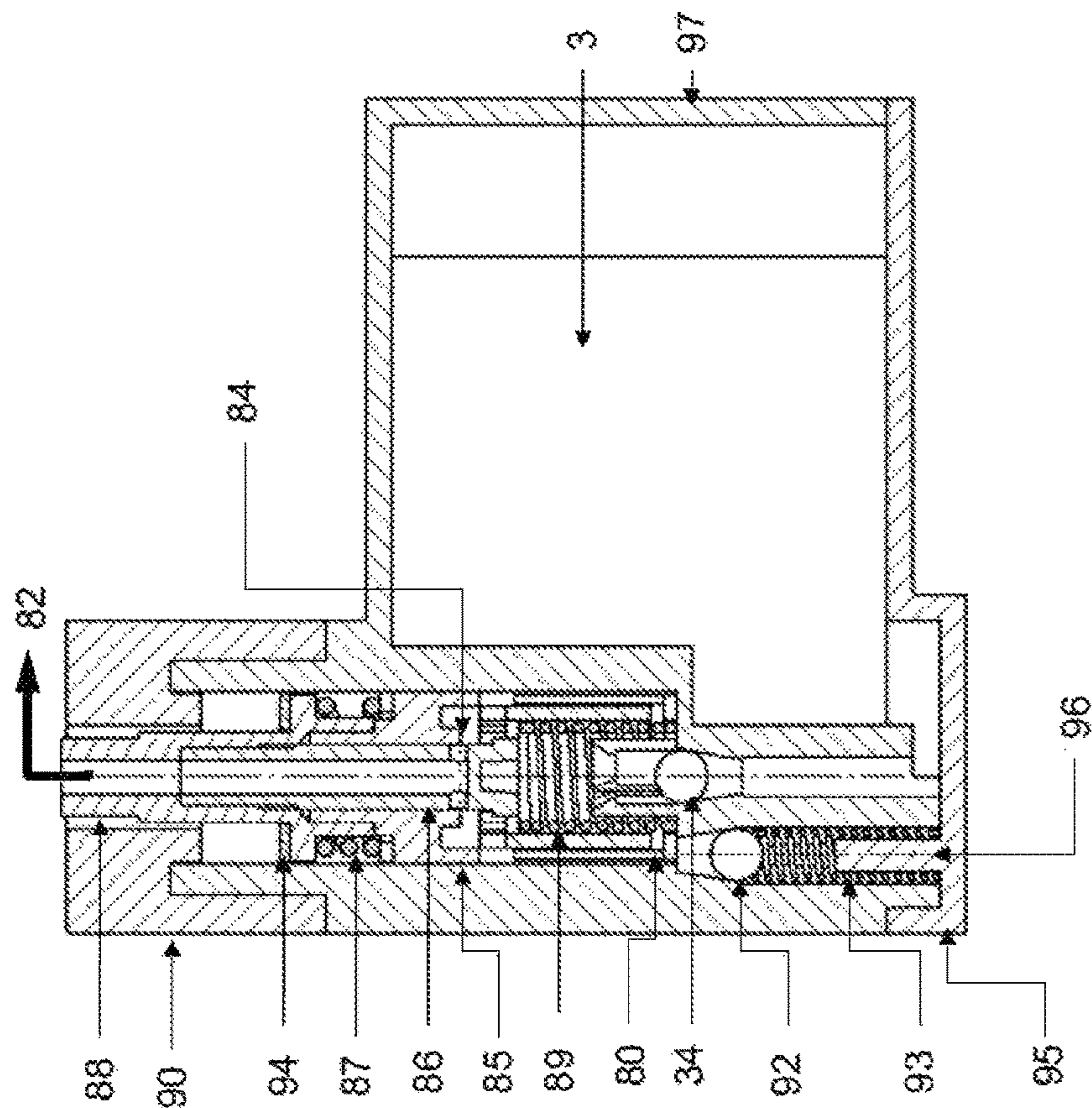
INTEGRATED PUMP / RESERVOIR / OVERFLOW VALVE IN "OPEN" POSITION
