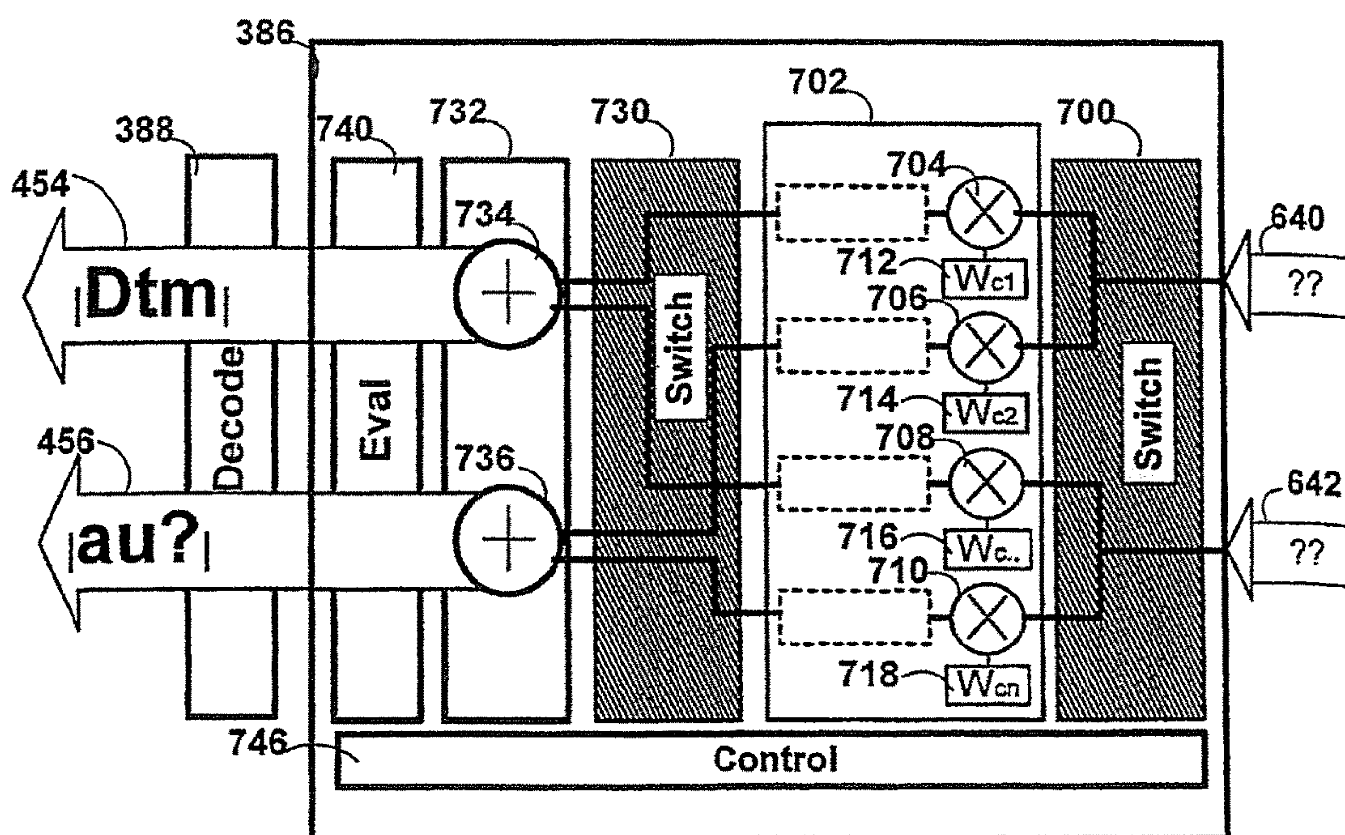
Spatial Processor
