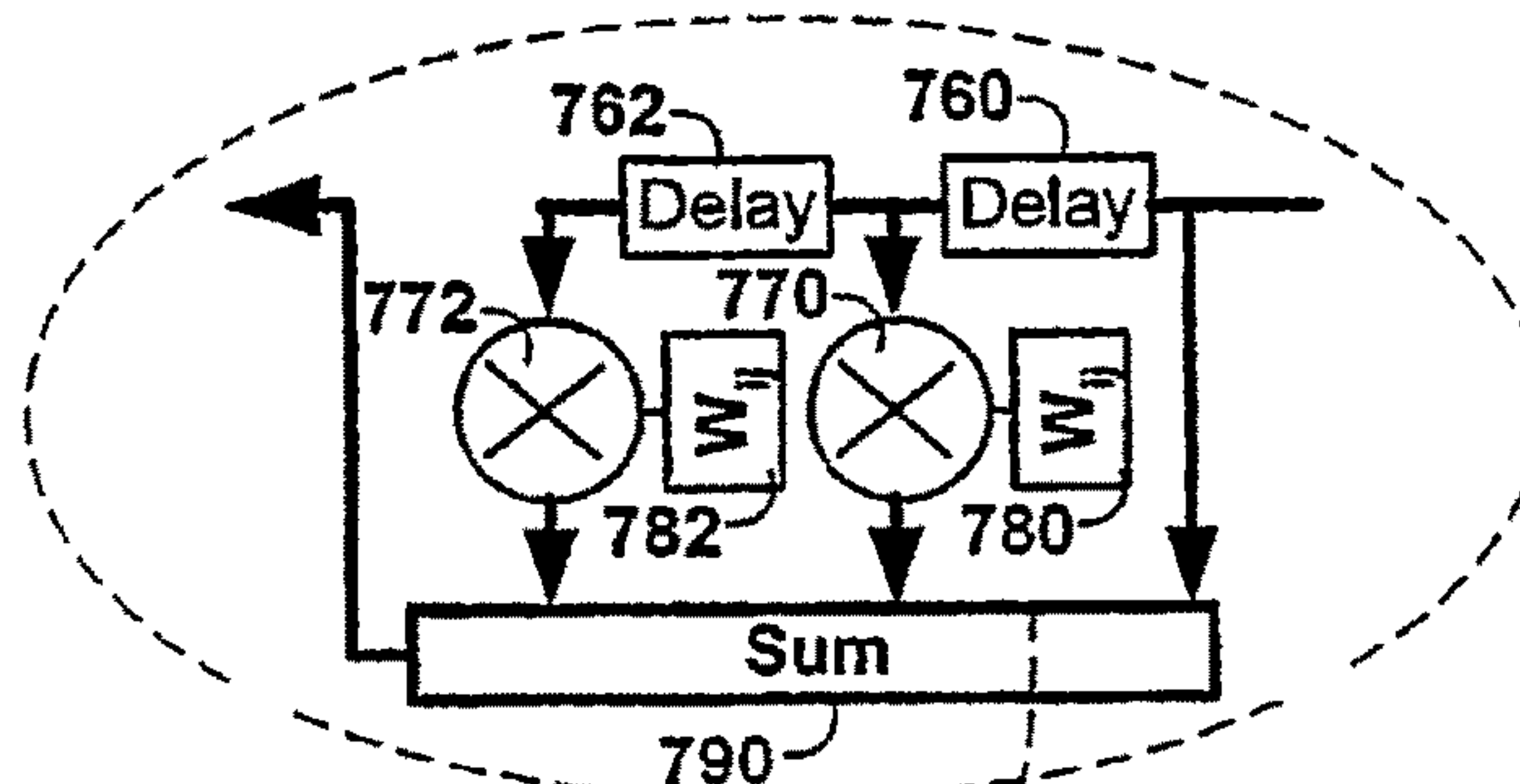
Space-Time Processor FIG. 7C
