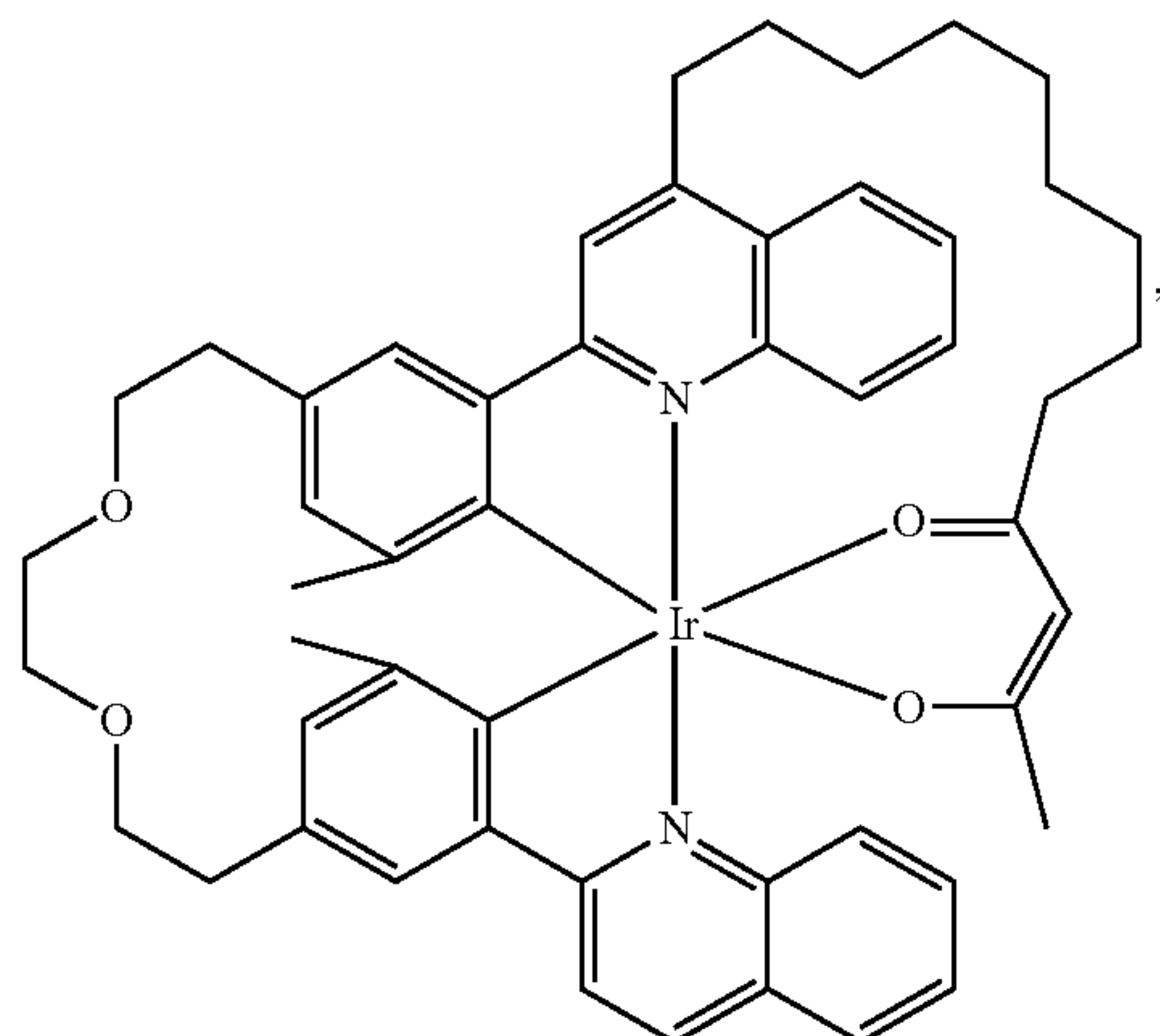
Compound 64
