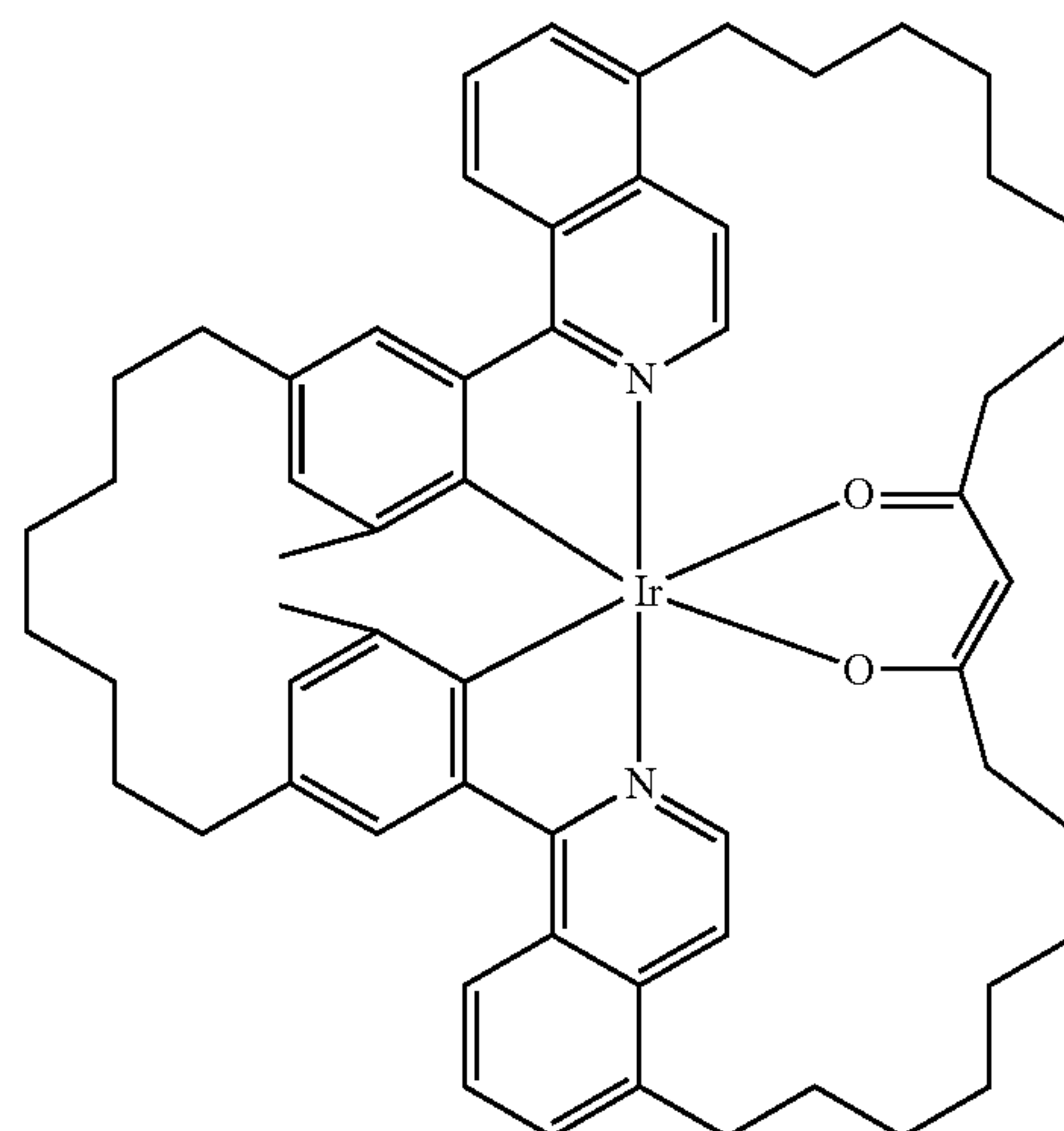
Compound 94
