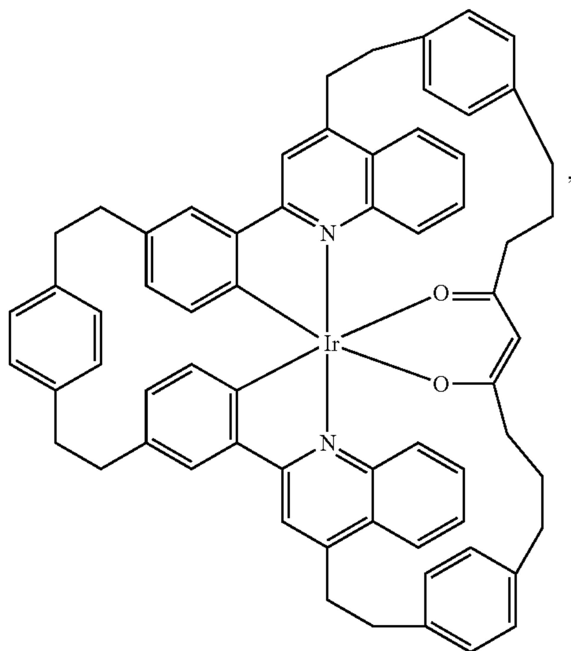
Compound 35
