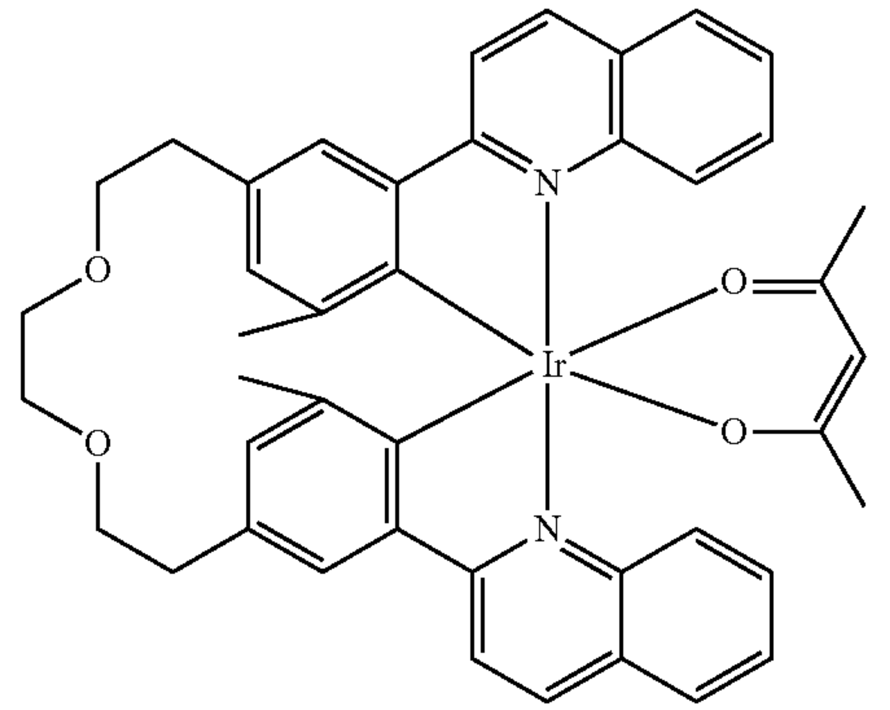
Compound 76
