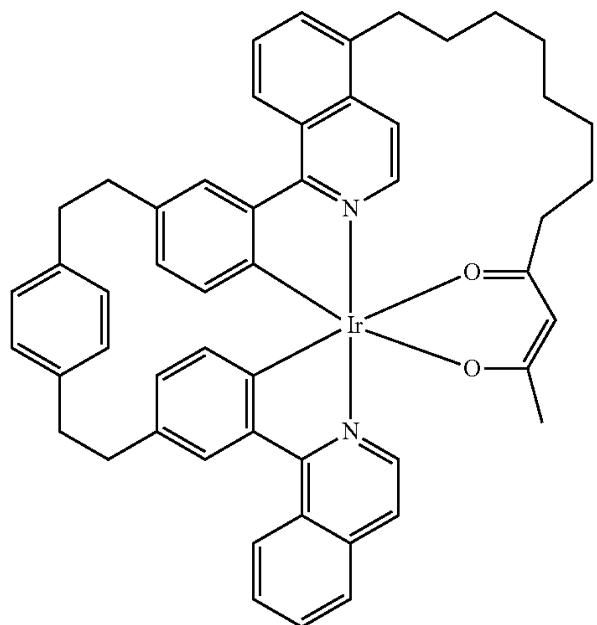
Compound 105
