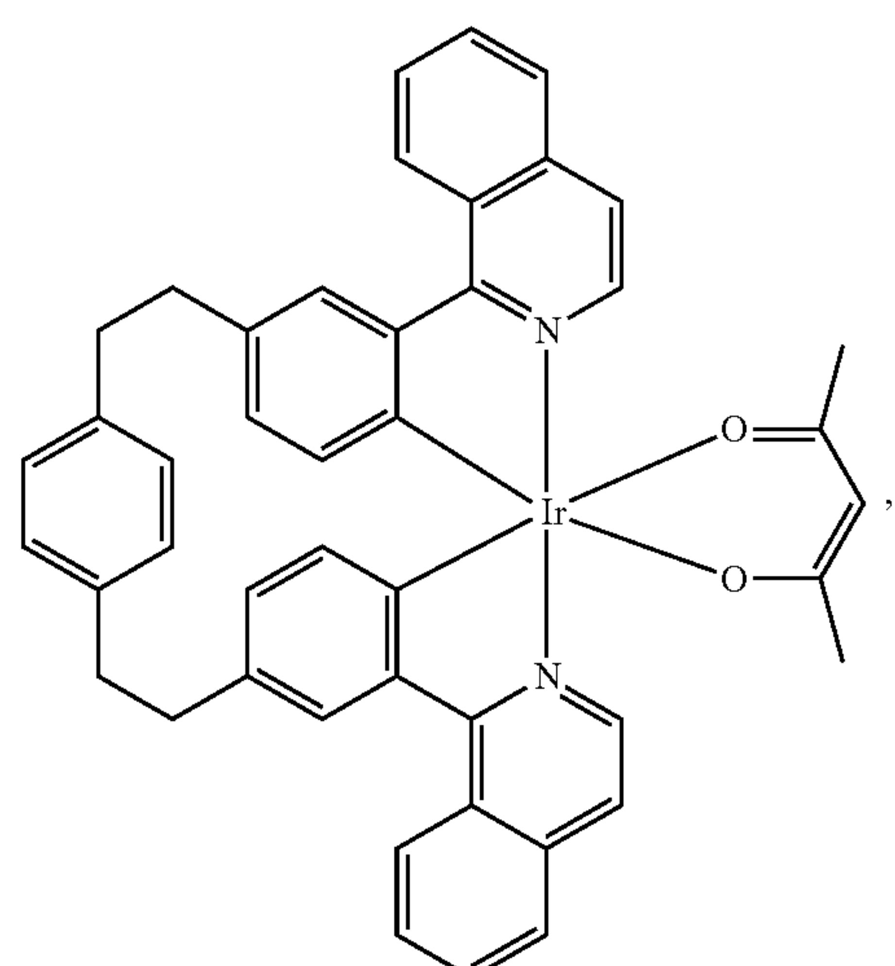
Compound 113
