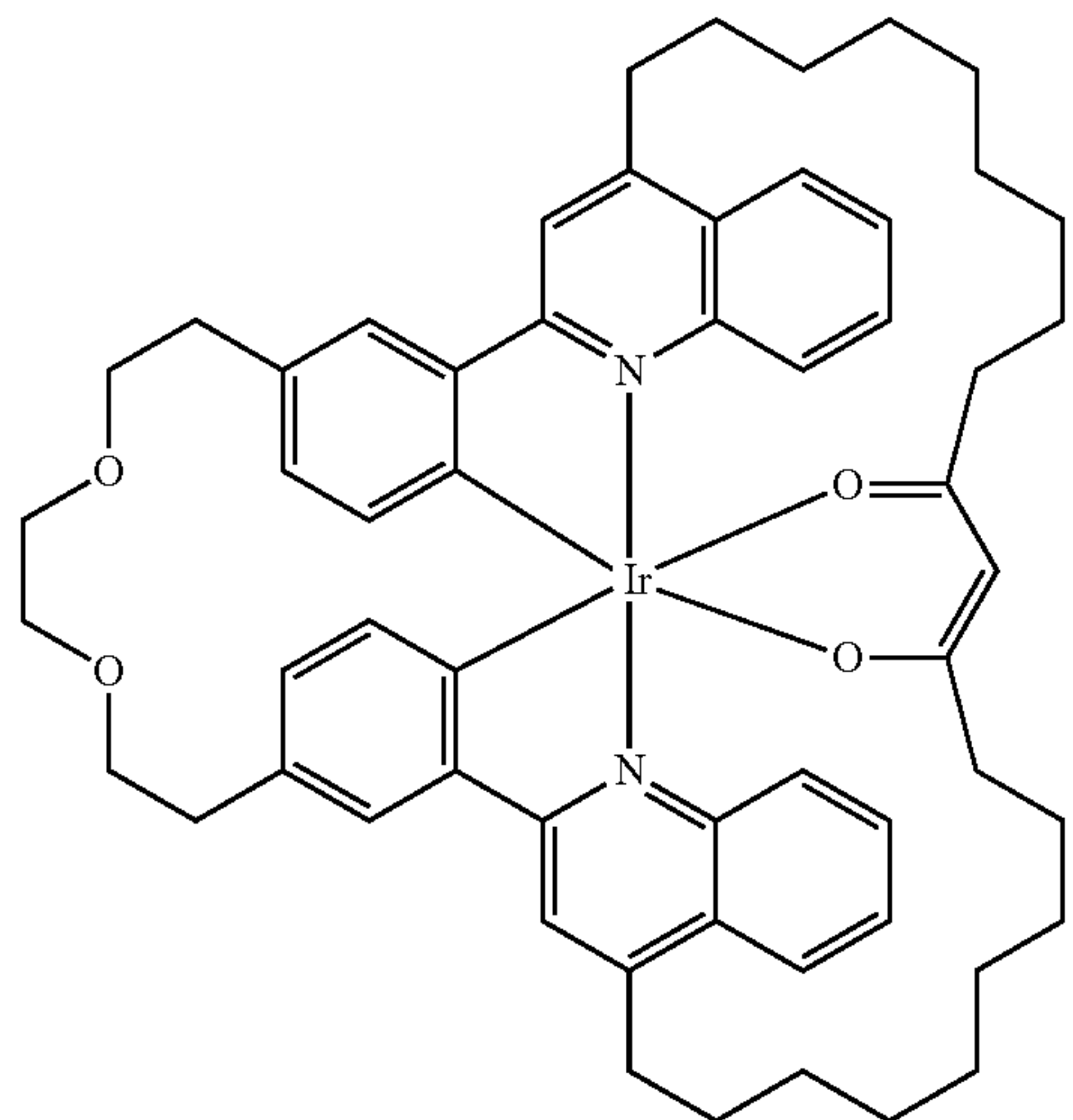
Compound 39
