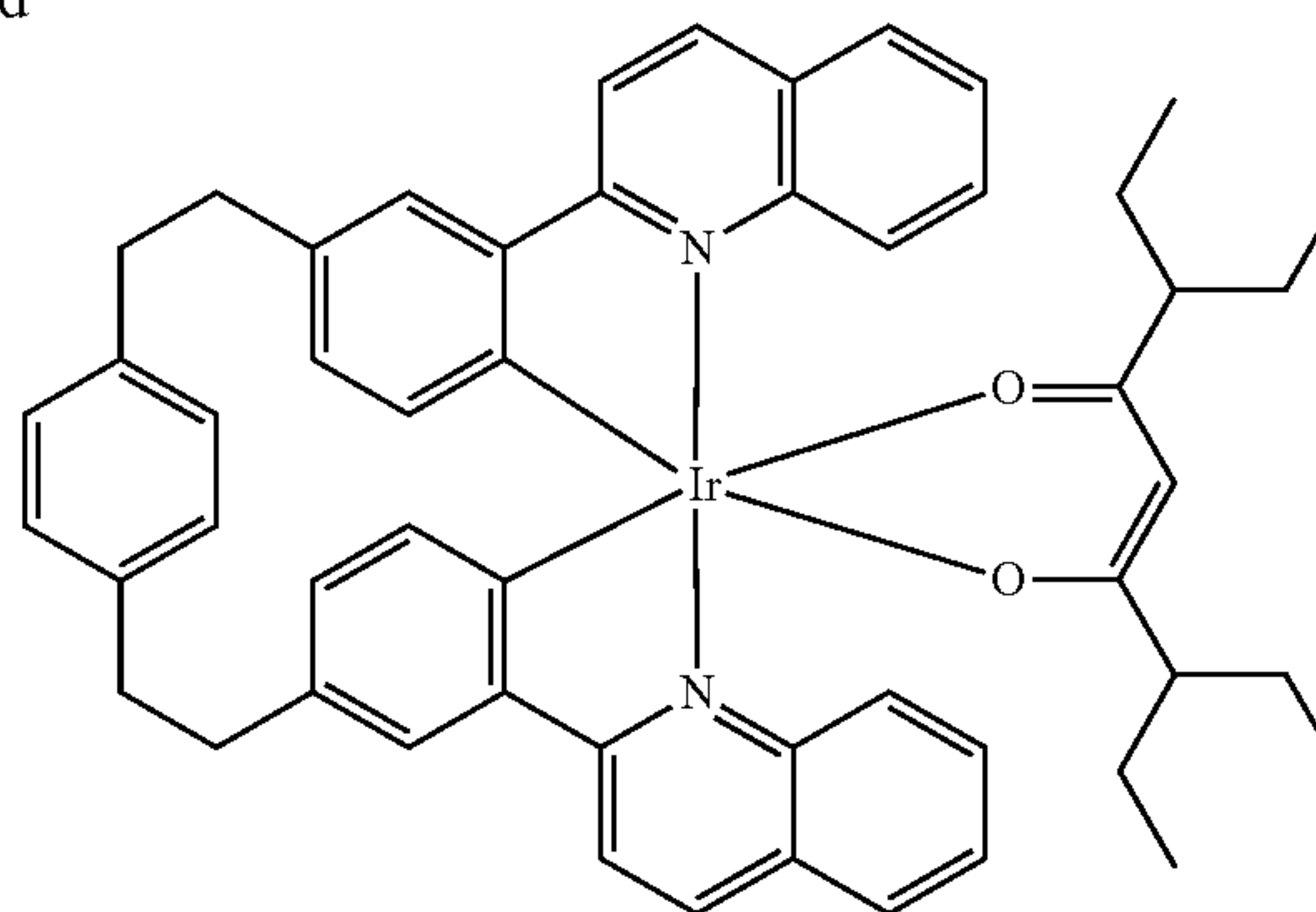
Compound 66
