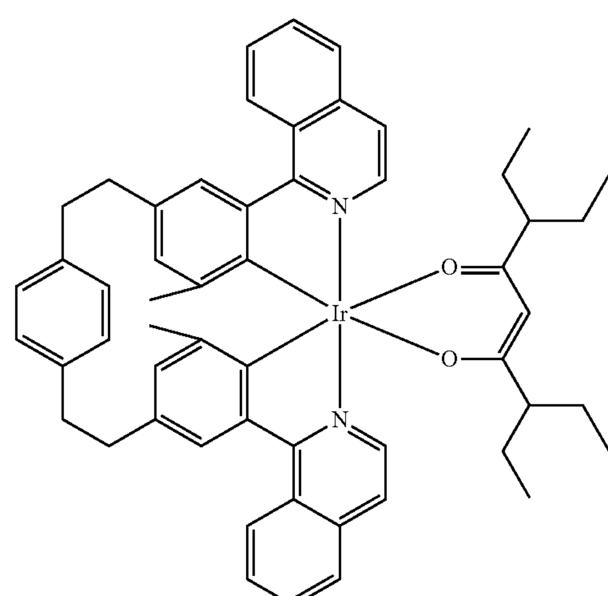
Compound 120
