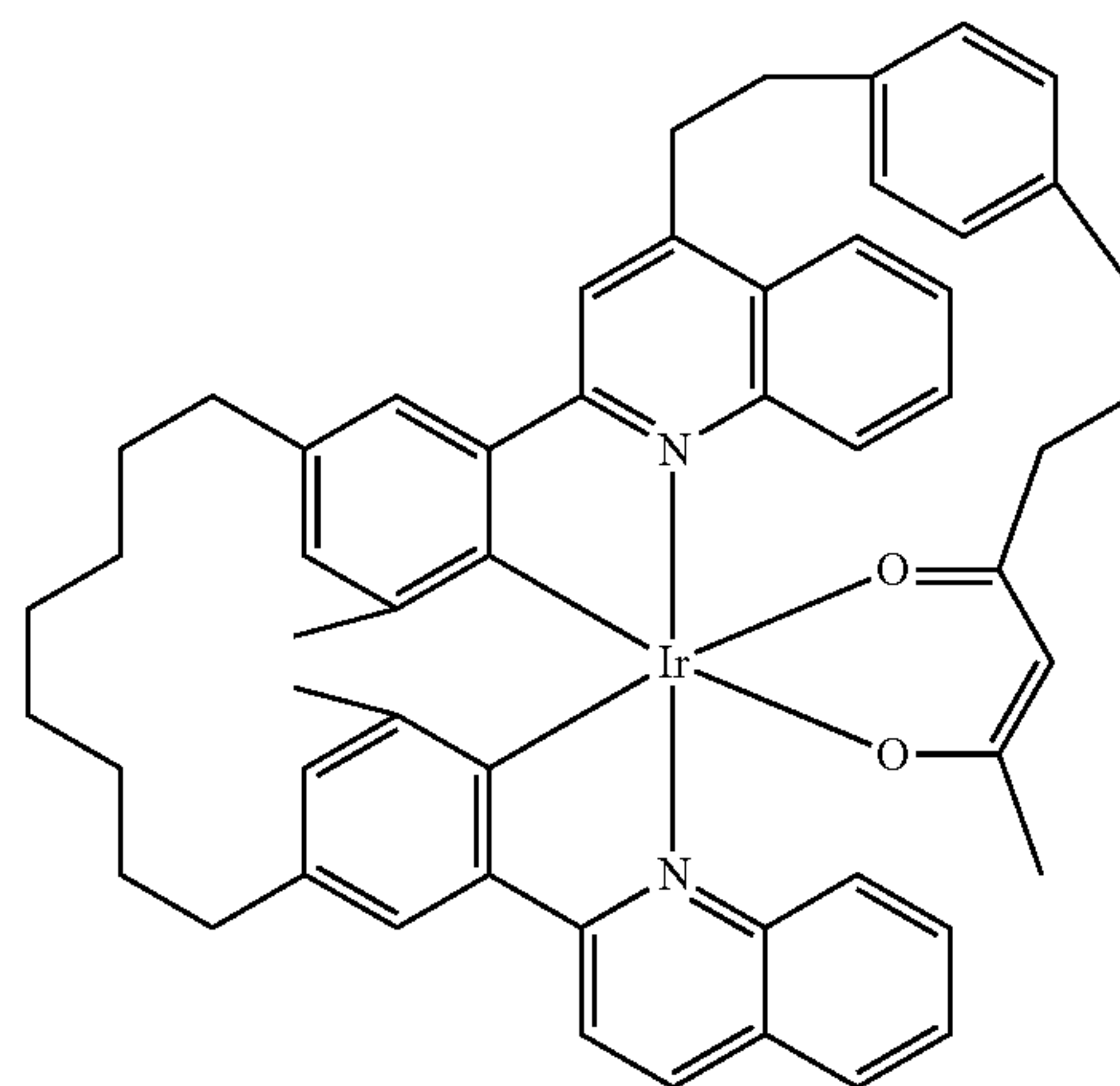
Compound 56
