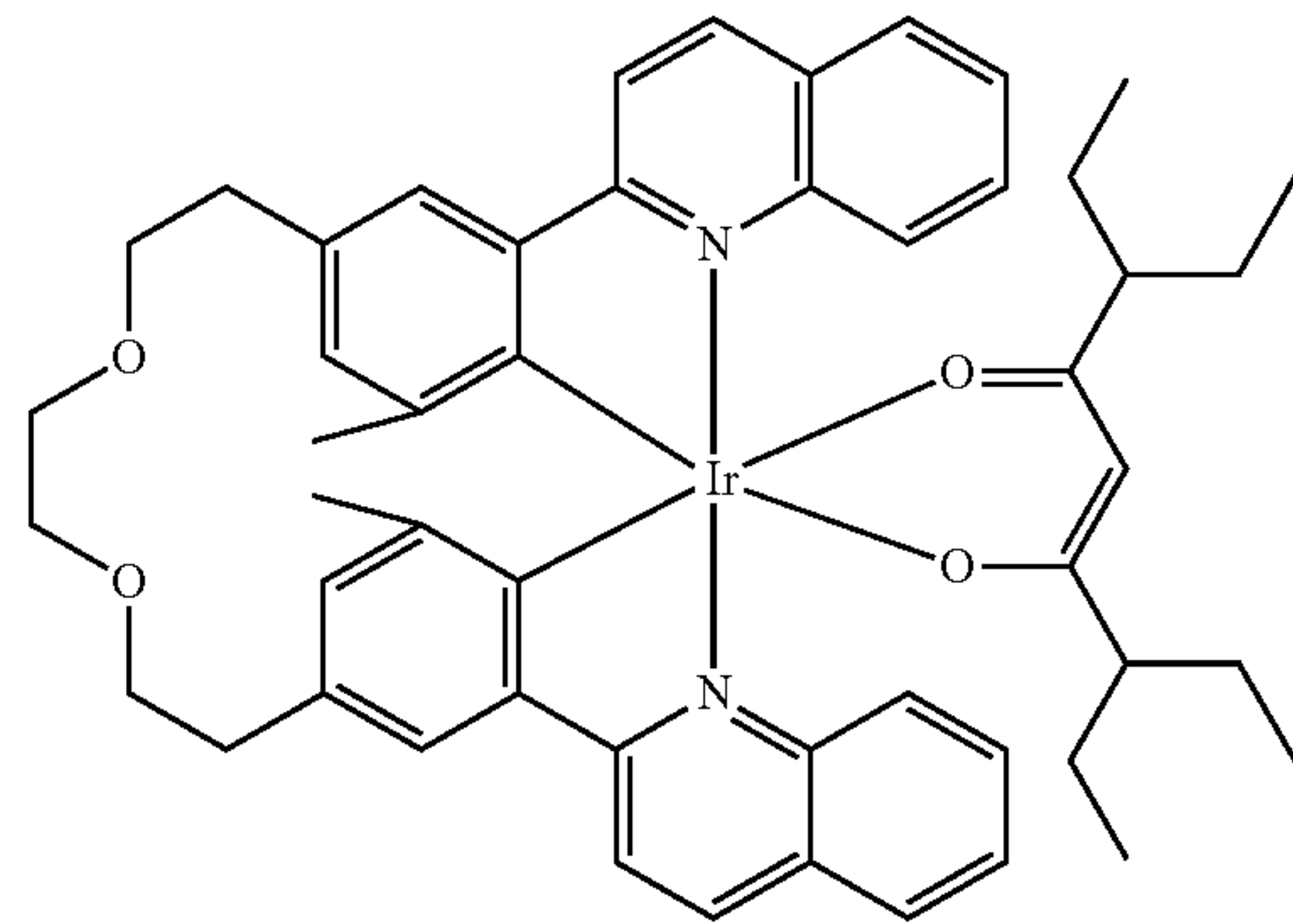
Compound 77
