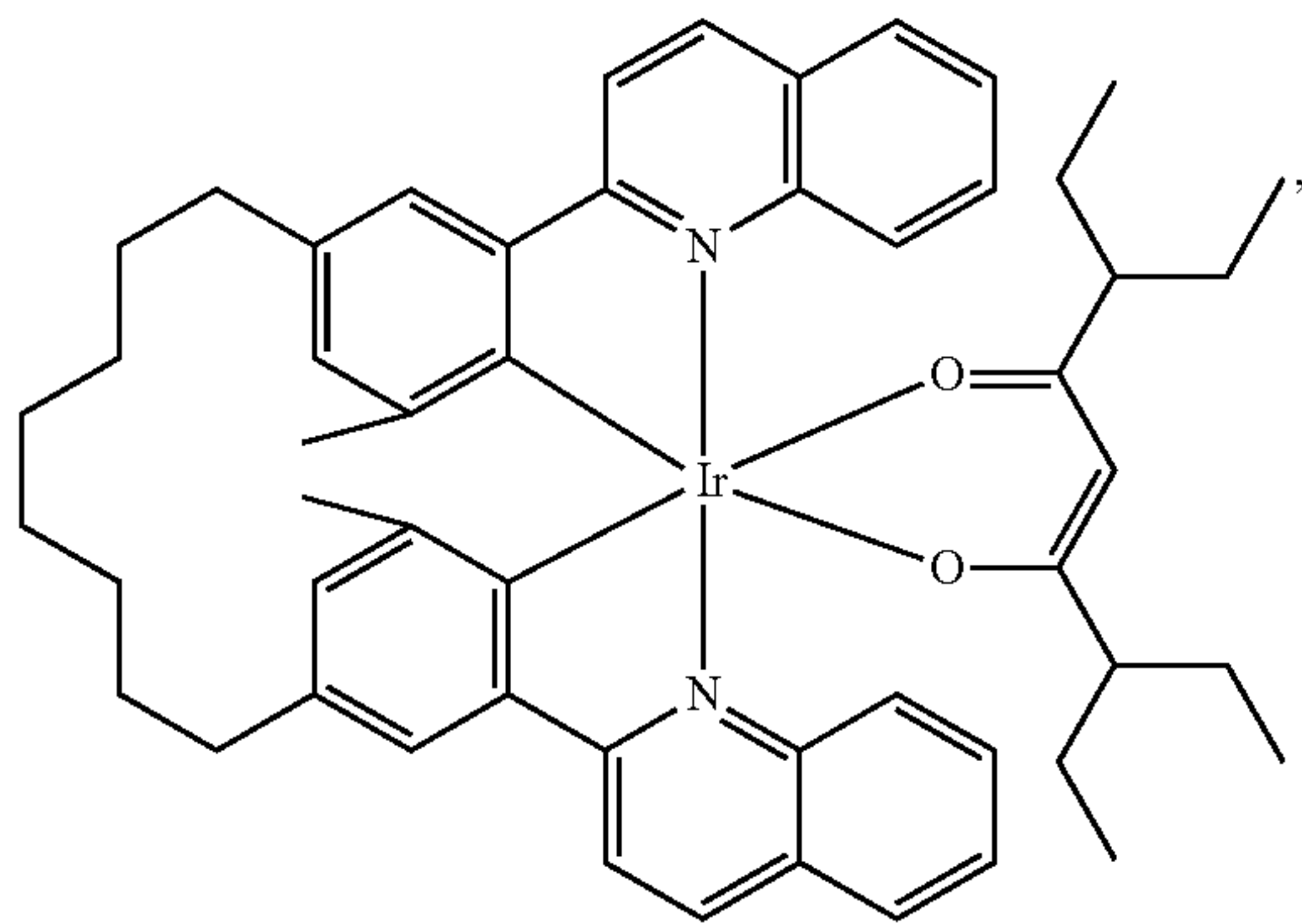
Compound 74
