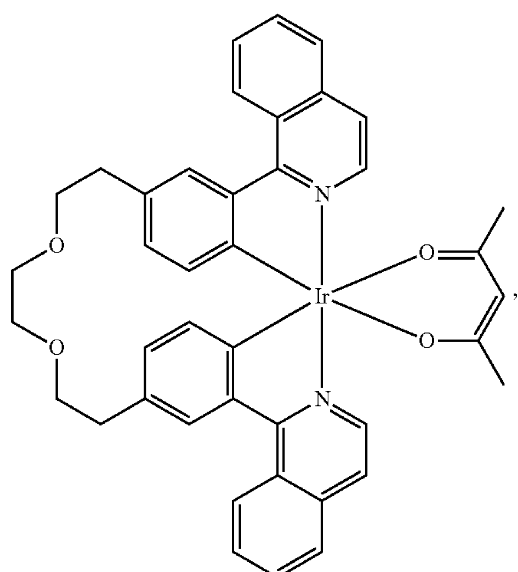
Compound 117
