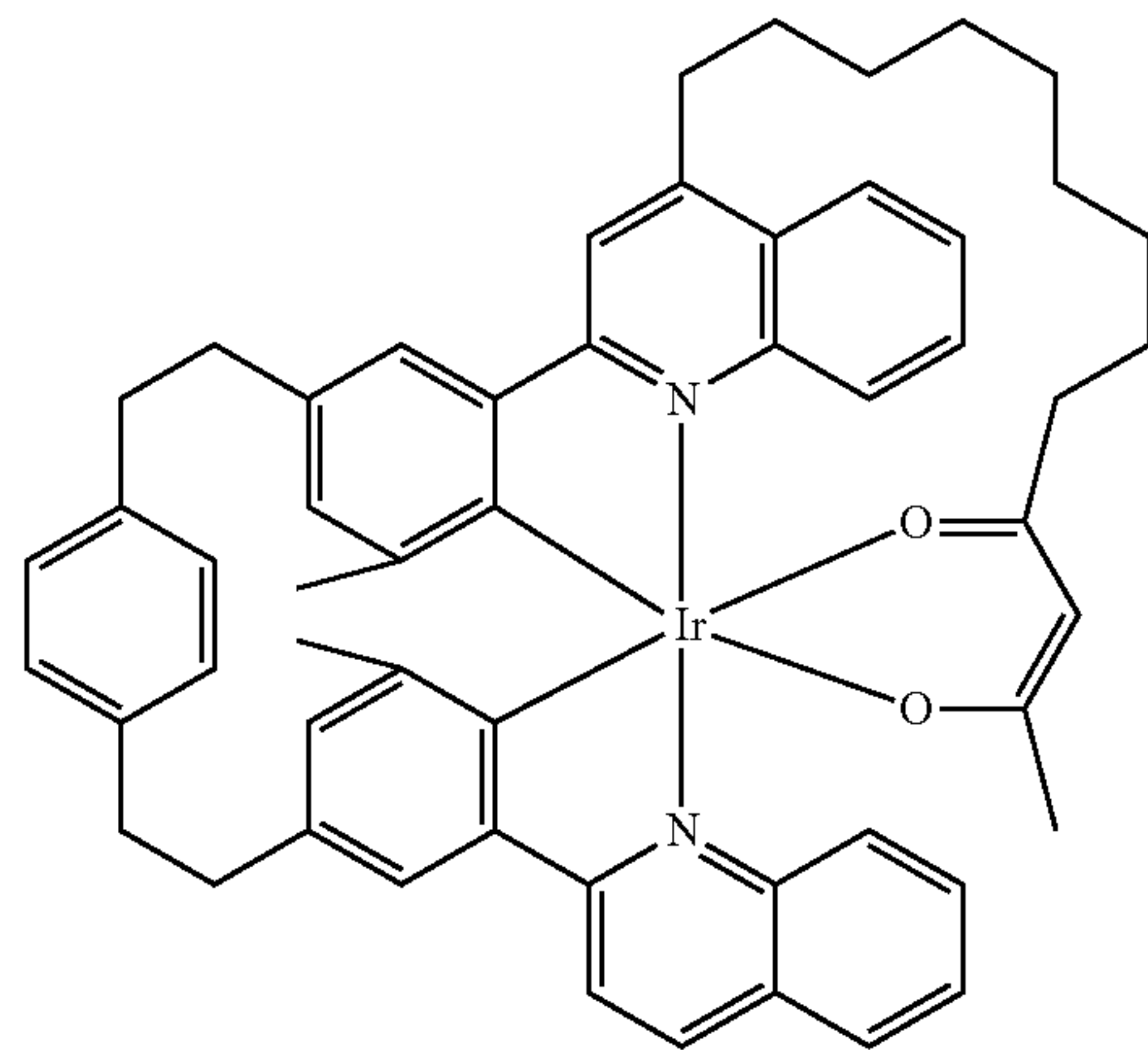
Compound 61
