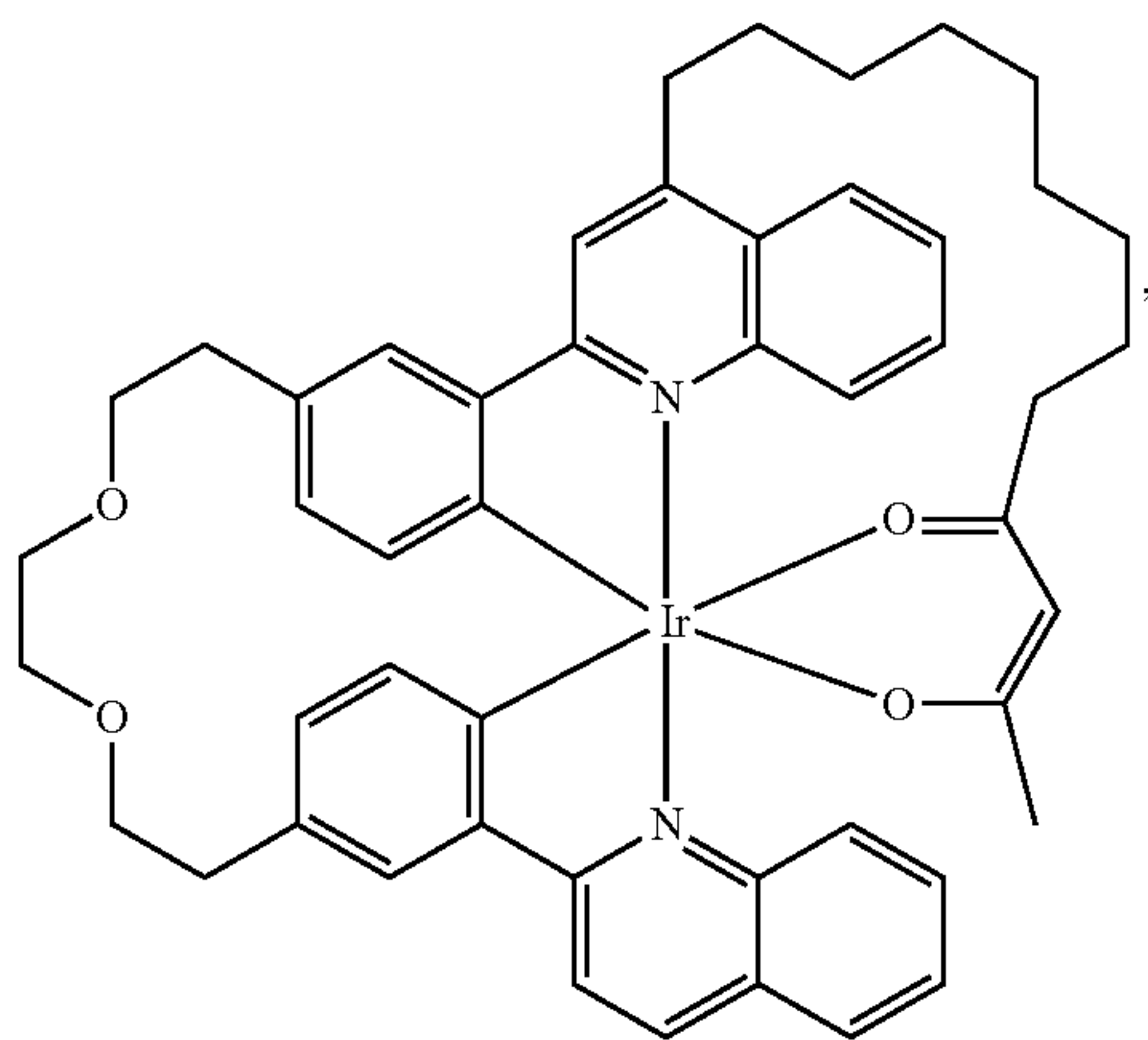
Compound 59
