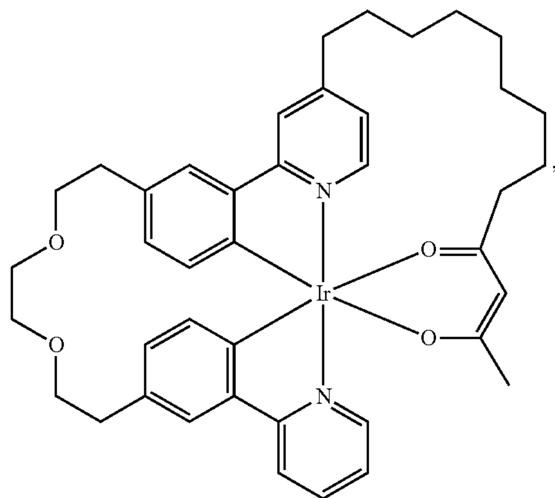
Compound 14
