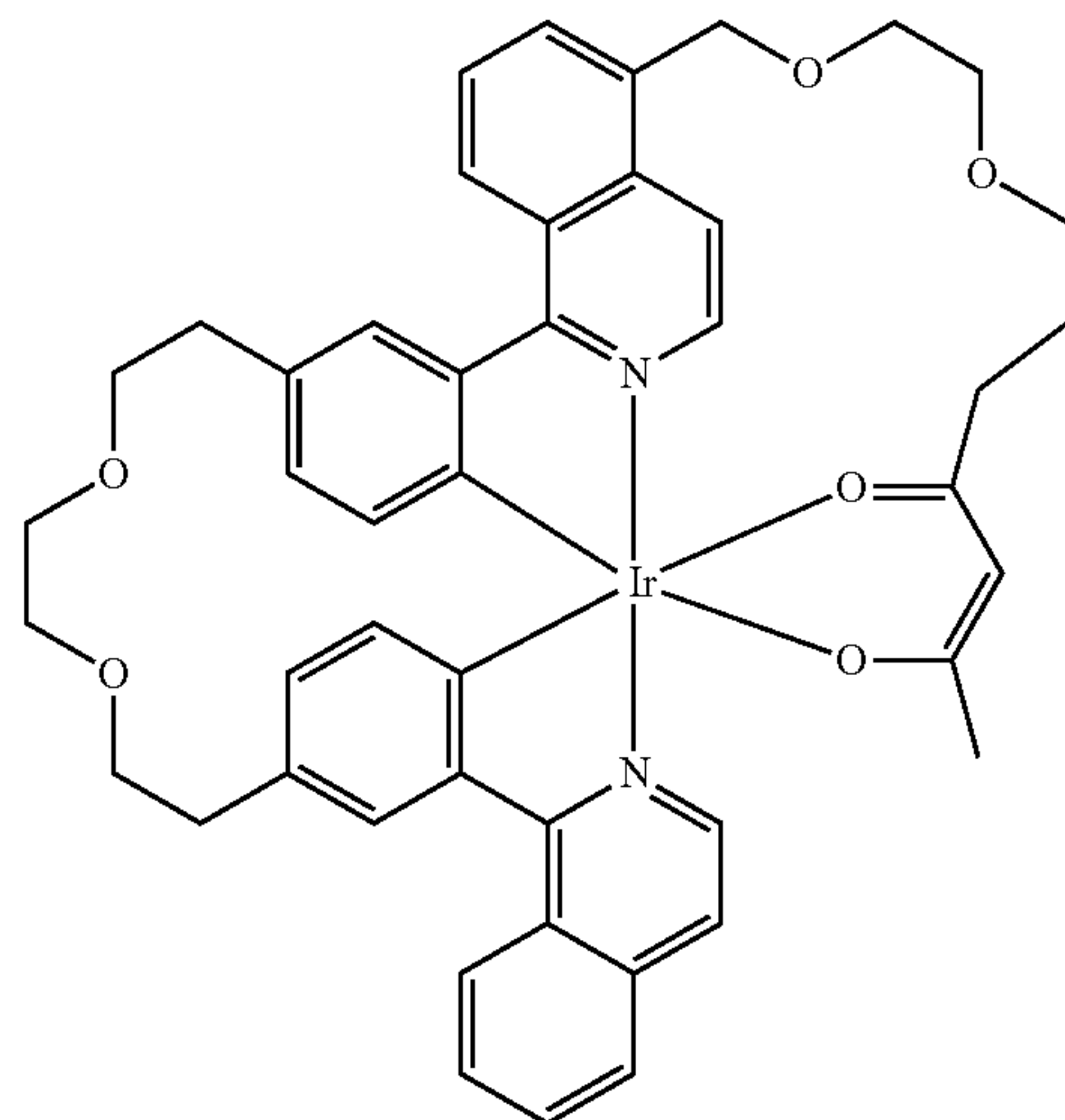
Compound 108
