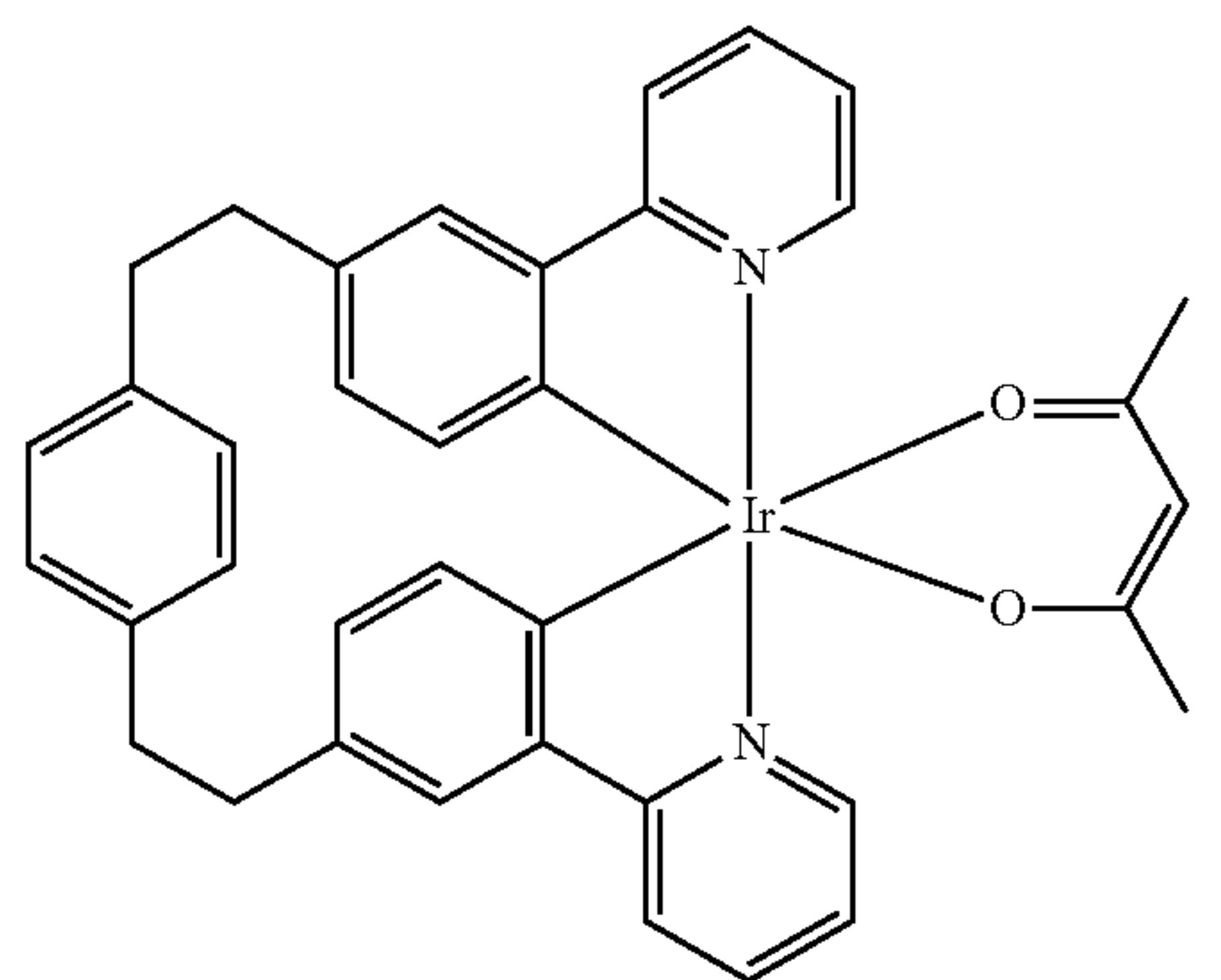
Compound 16
