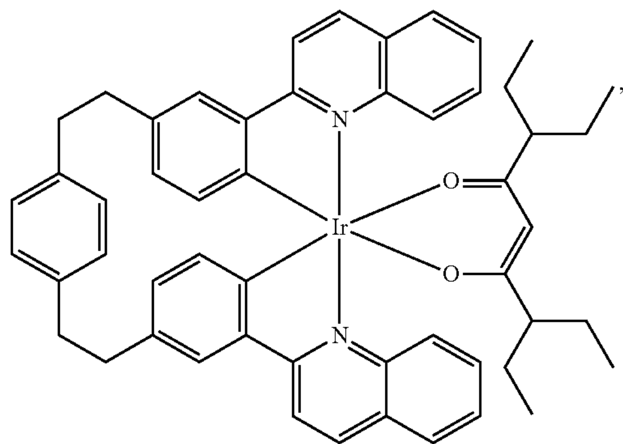
Compound 66
