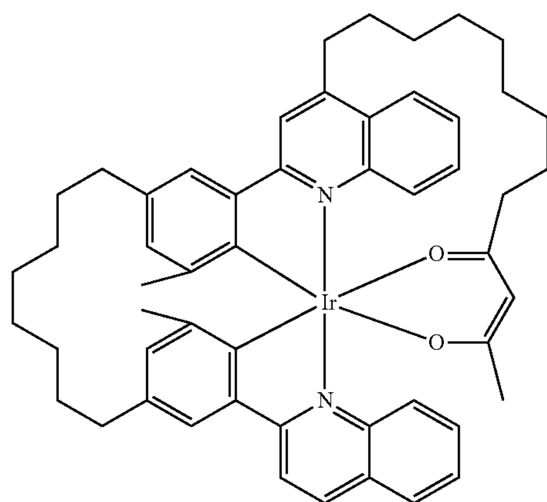
Compound 62
