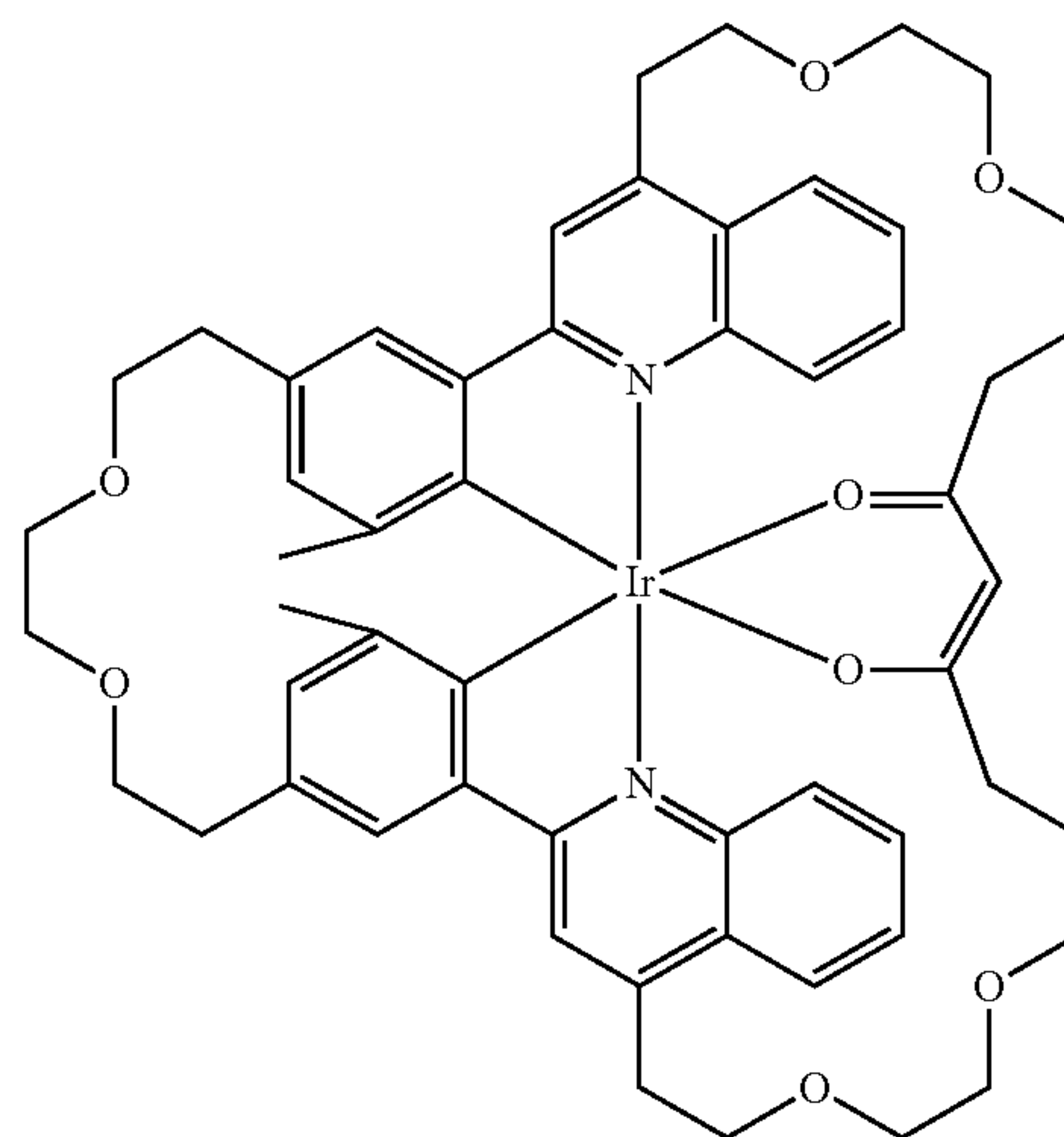
Compound 42
