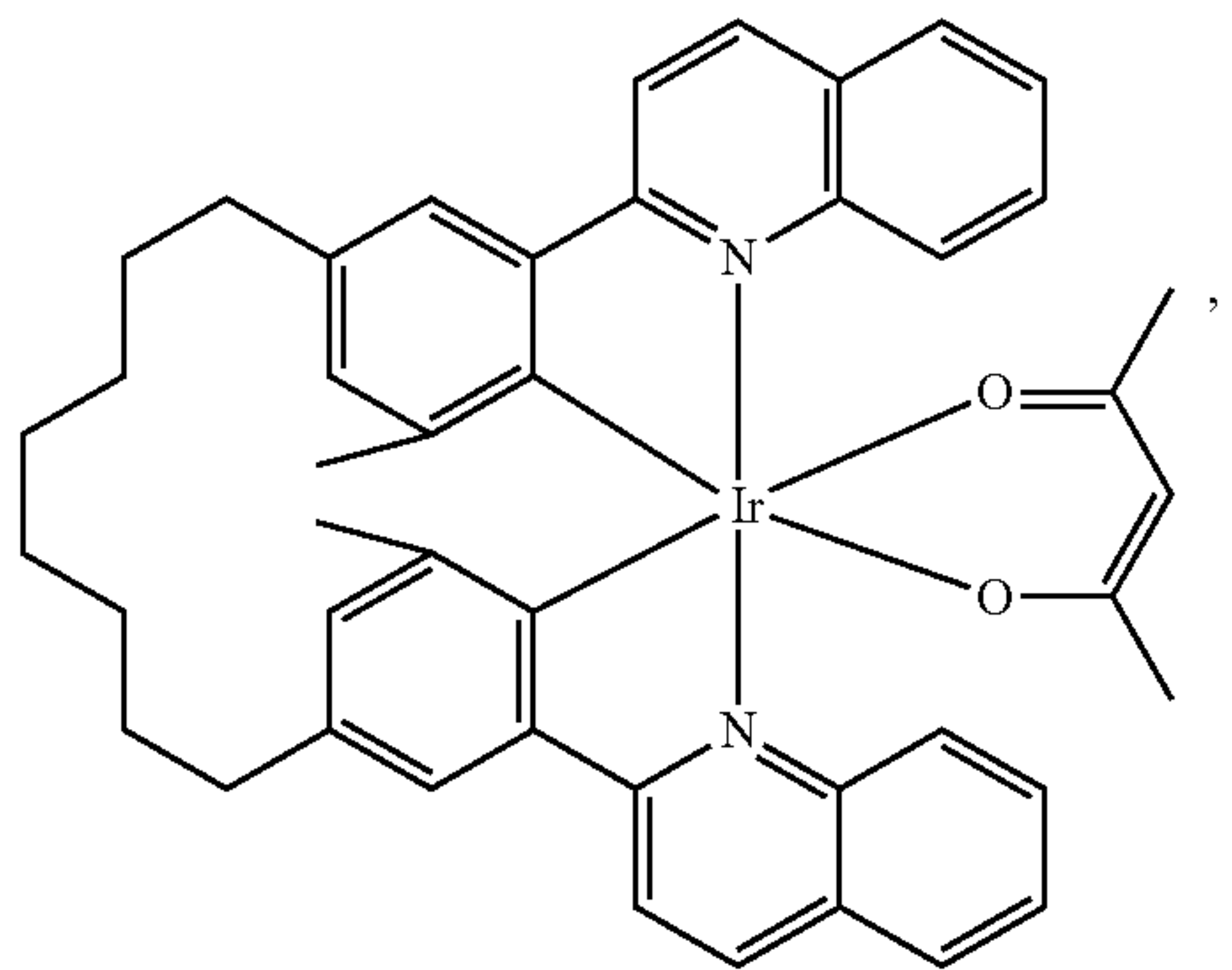
Compound 74
