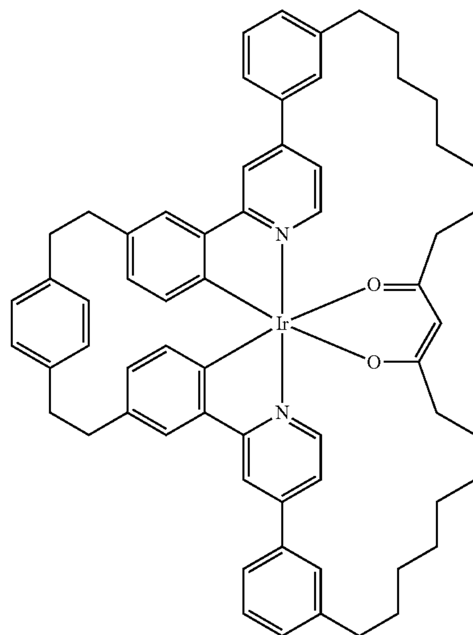
Compound 25
