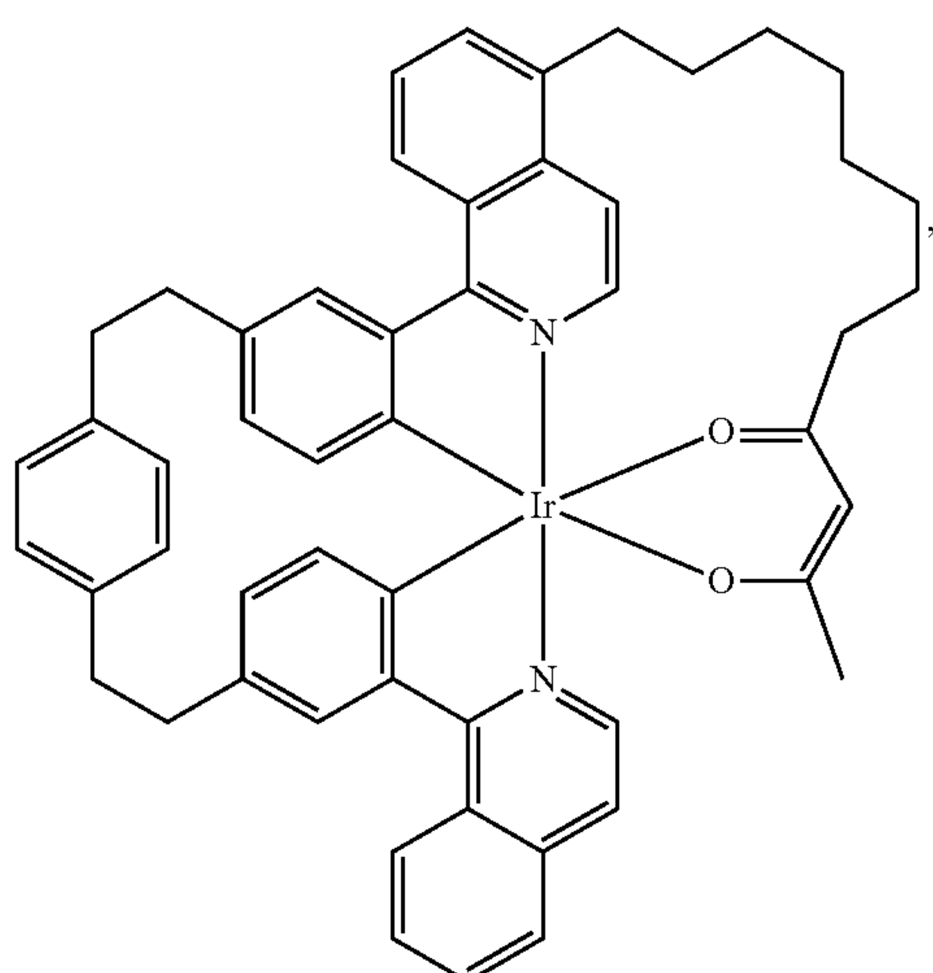
Compound 105
