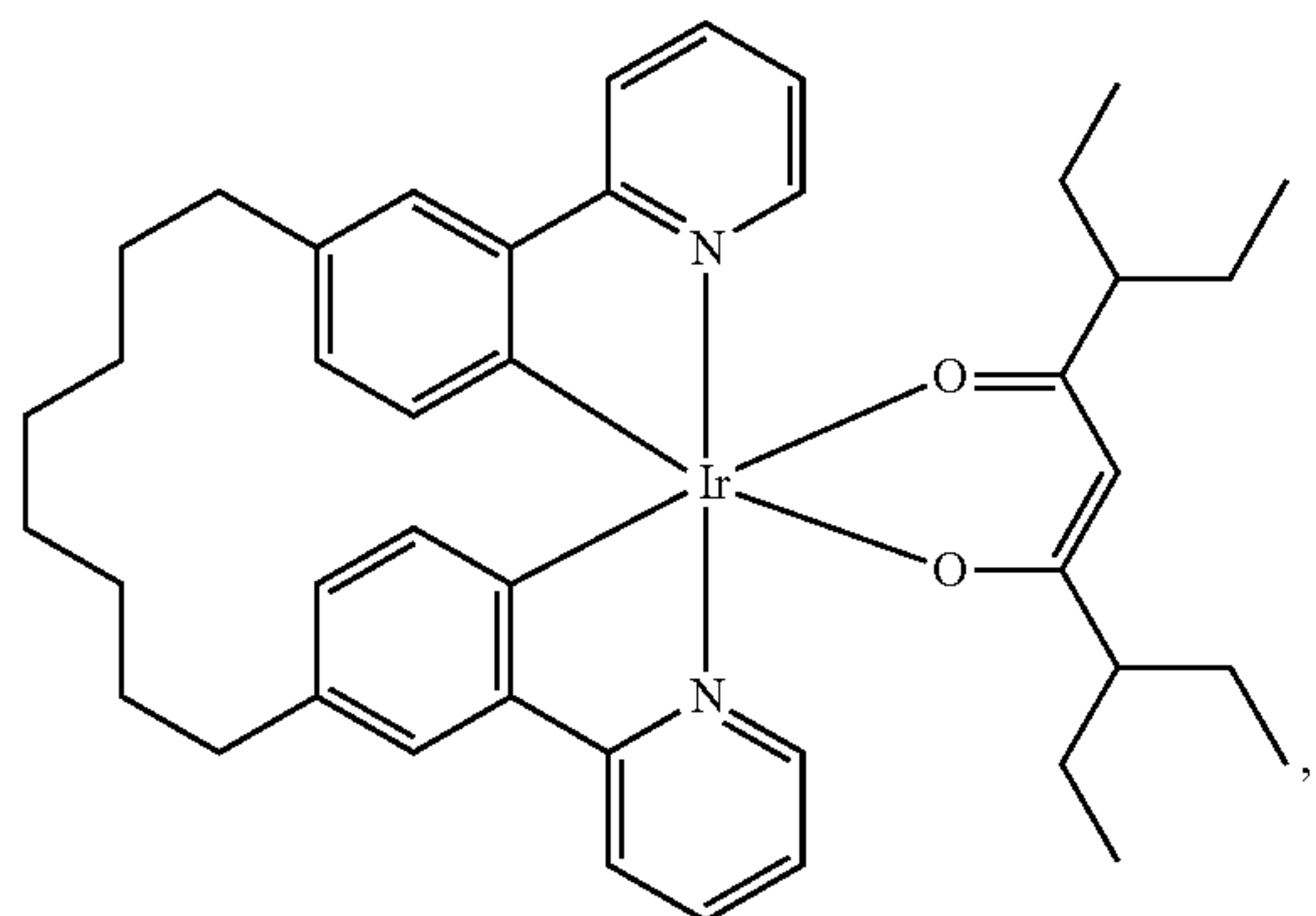
Compound 19
