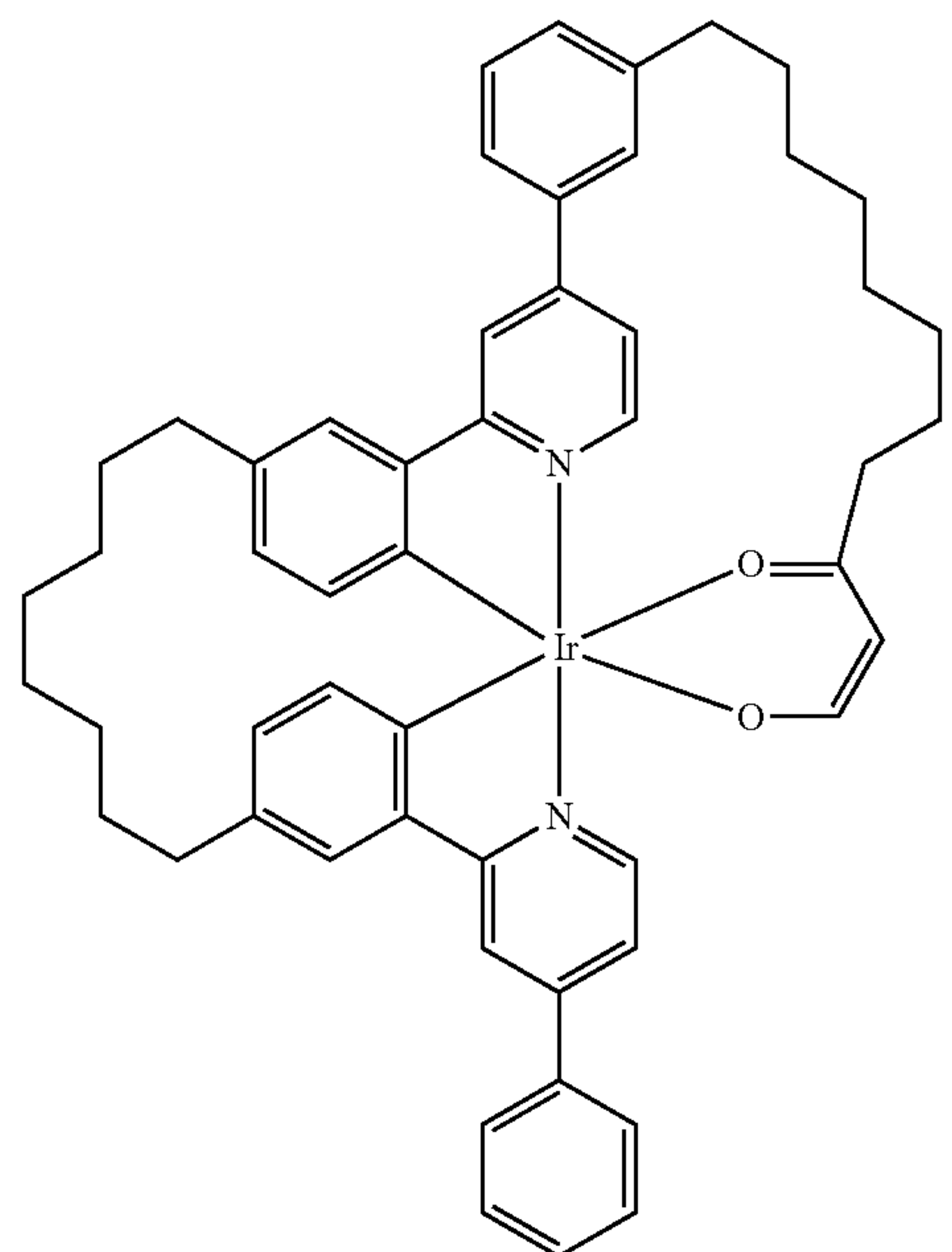
Compound 28
