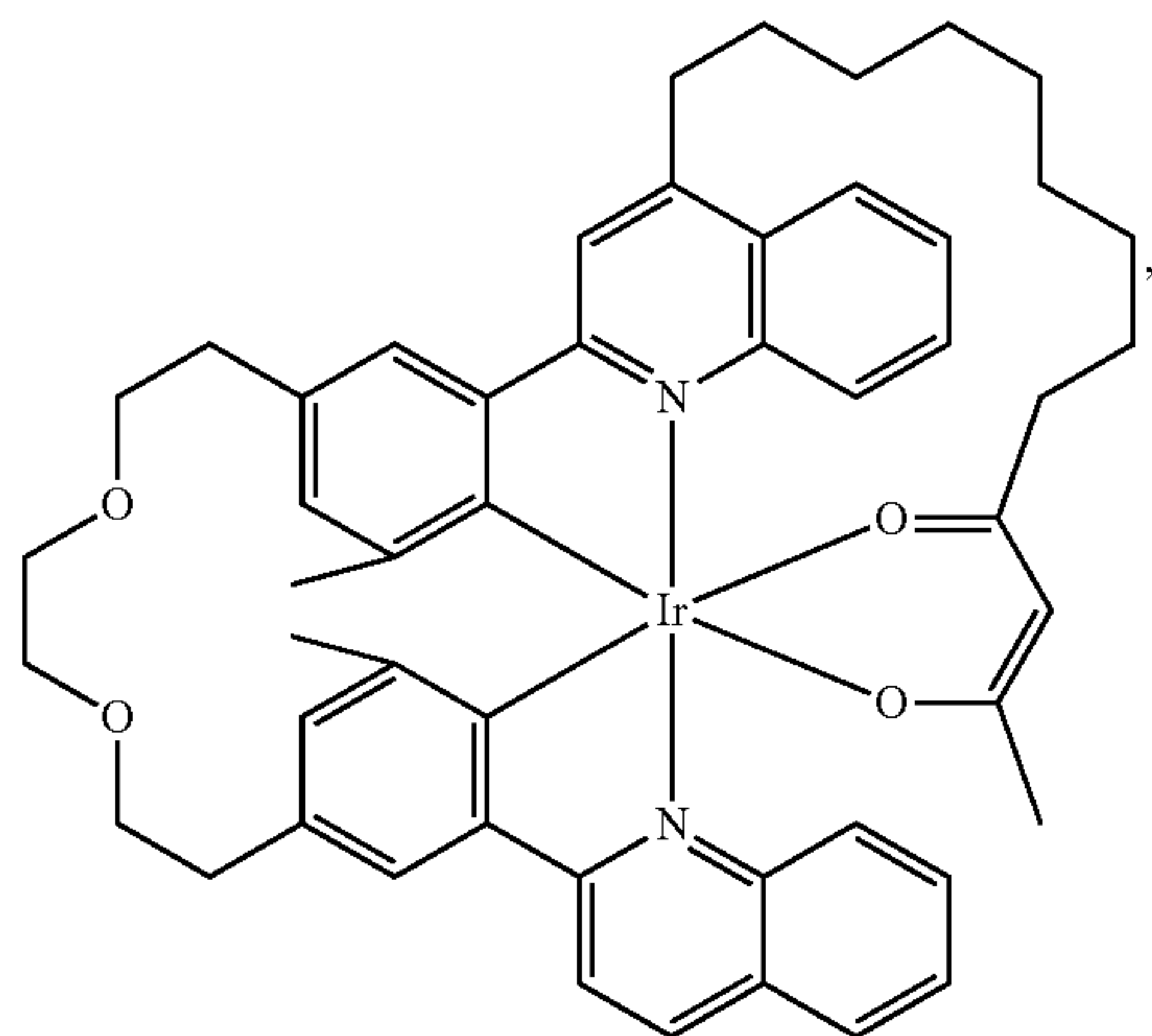
Compound 64
