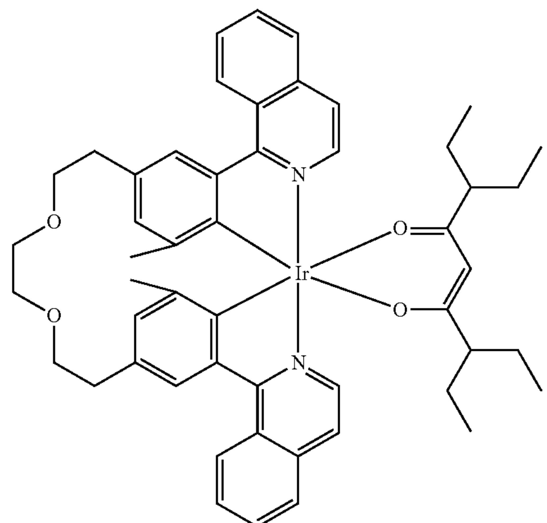
Compound 124
