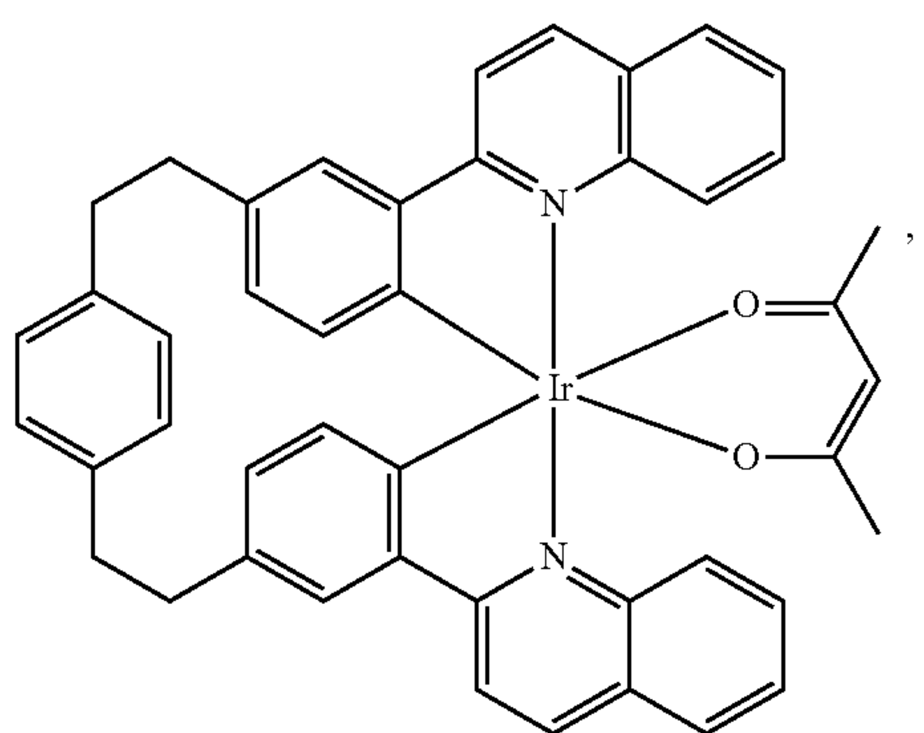
Compound 66
