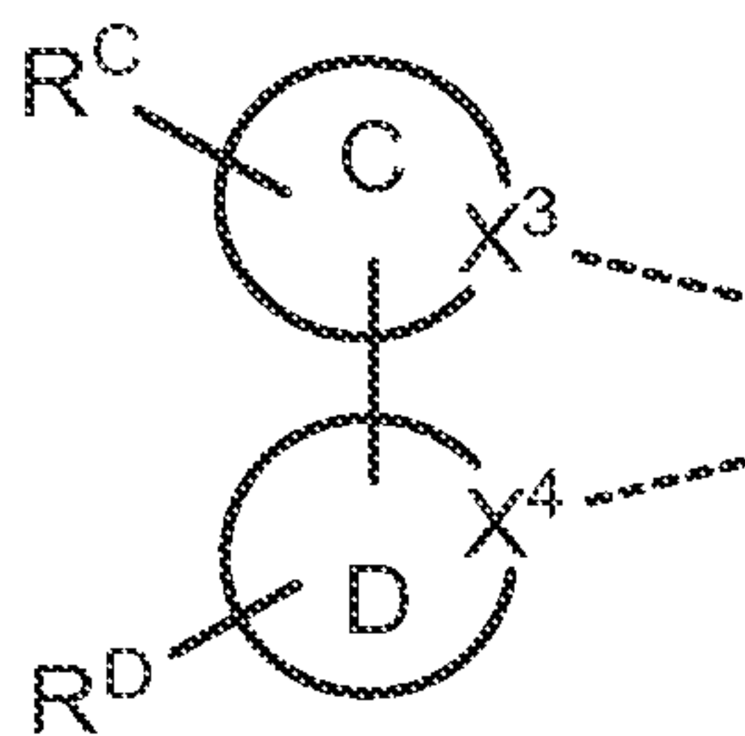
FORMULA II
