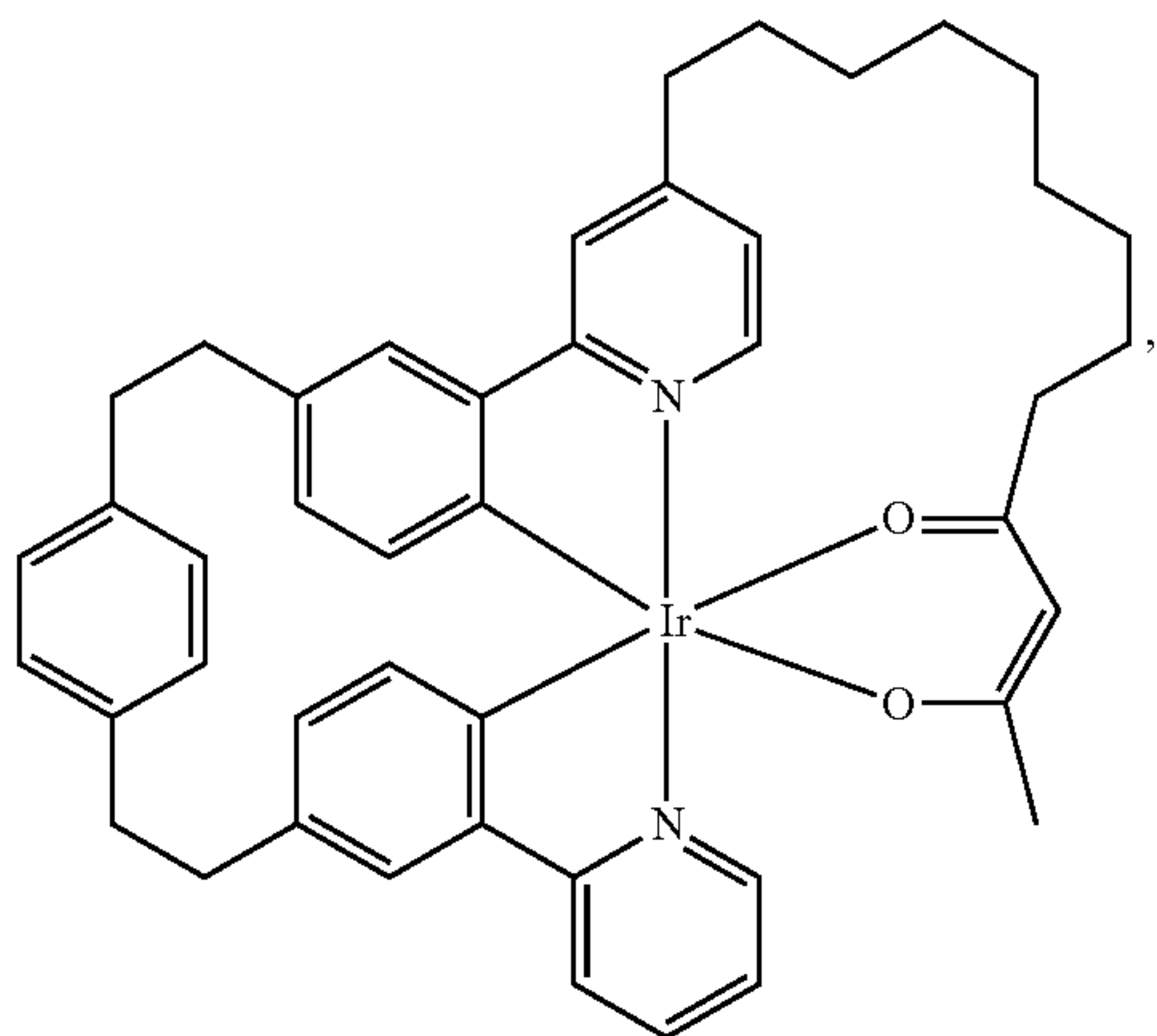
Compound 12
