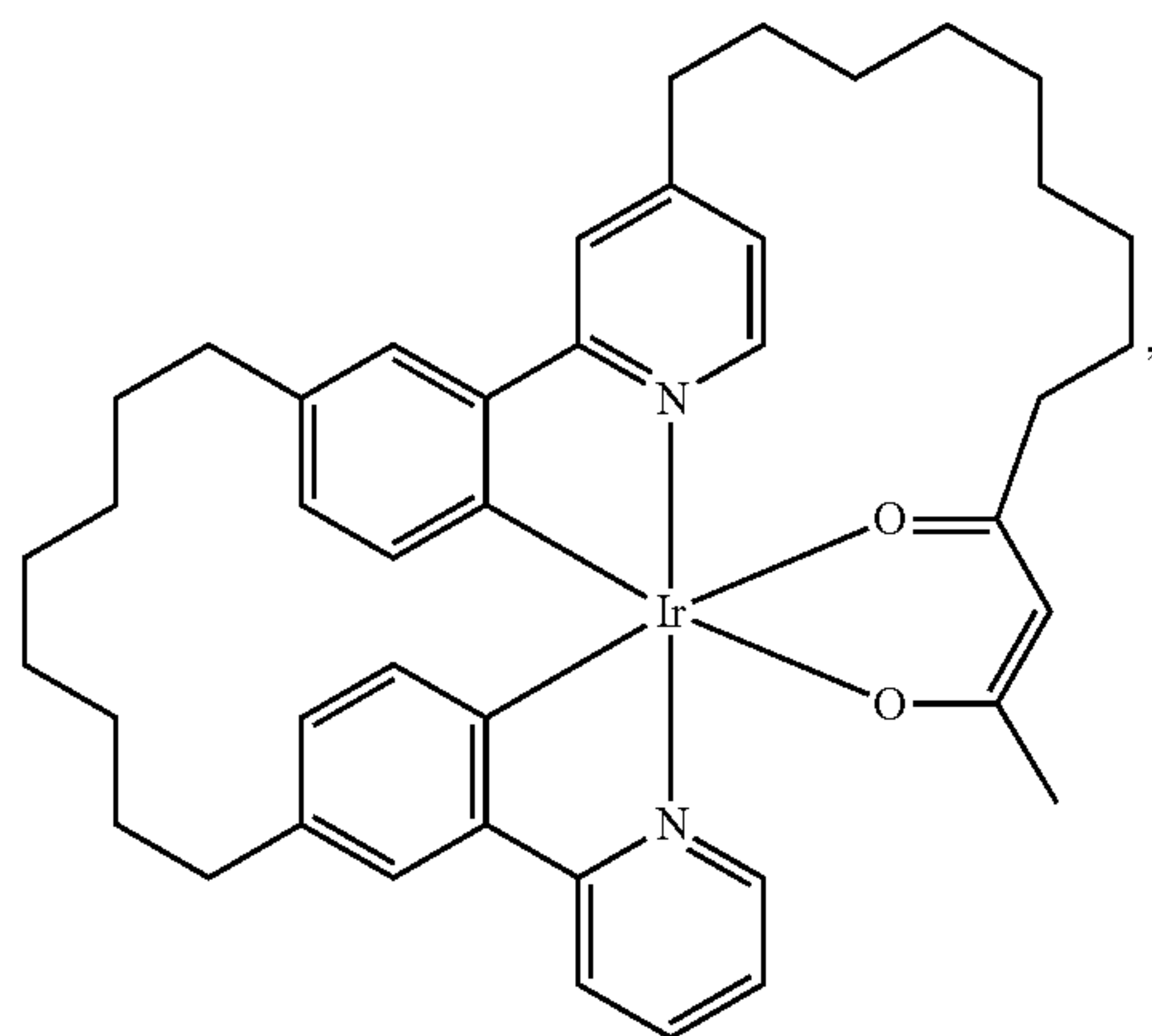
Compound 13
