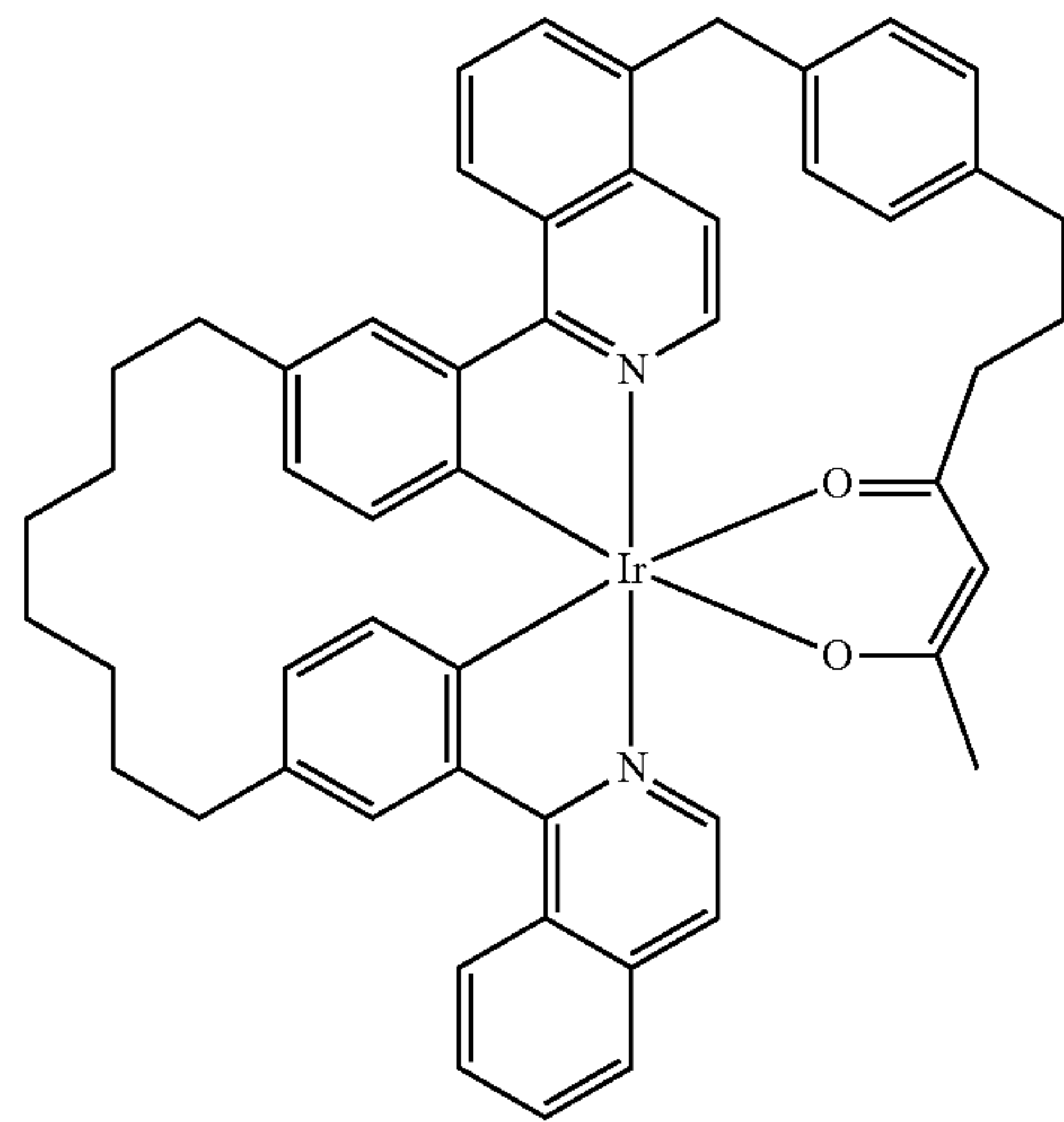
Compound 101
