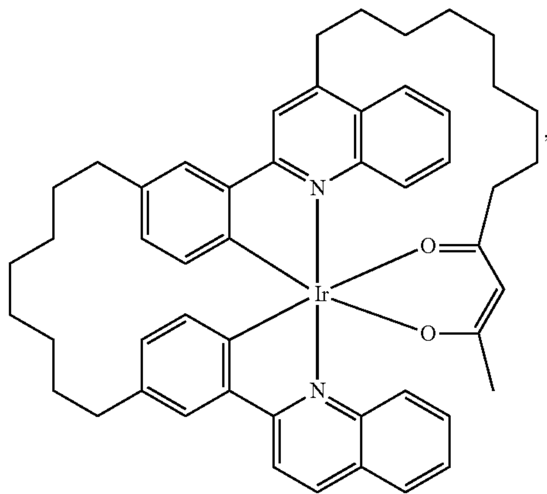
Compound 58
