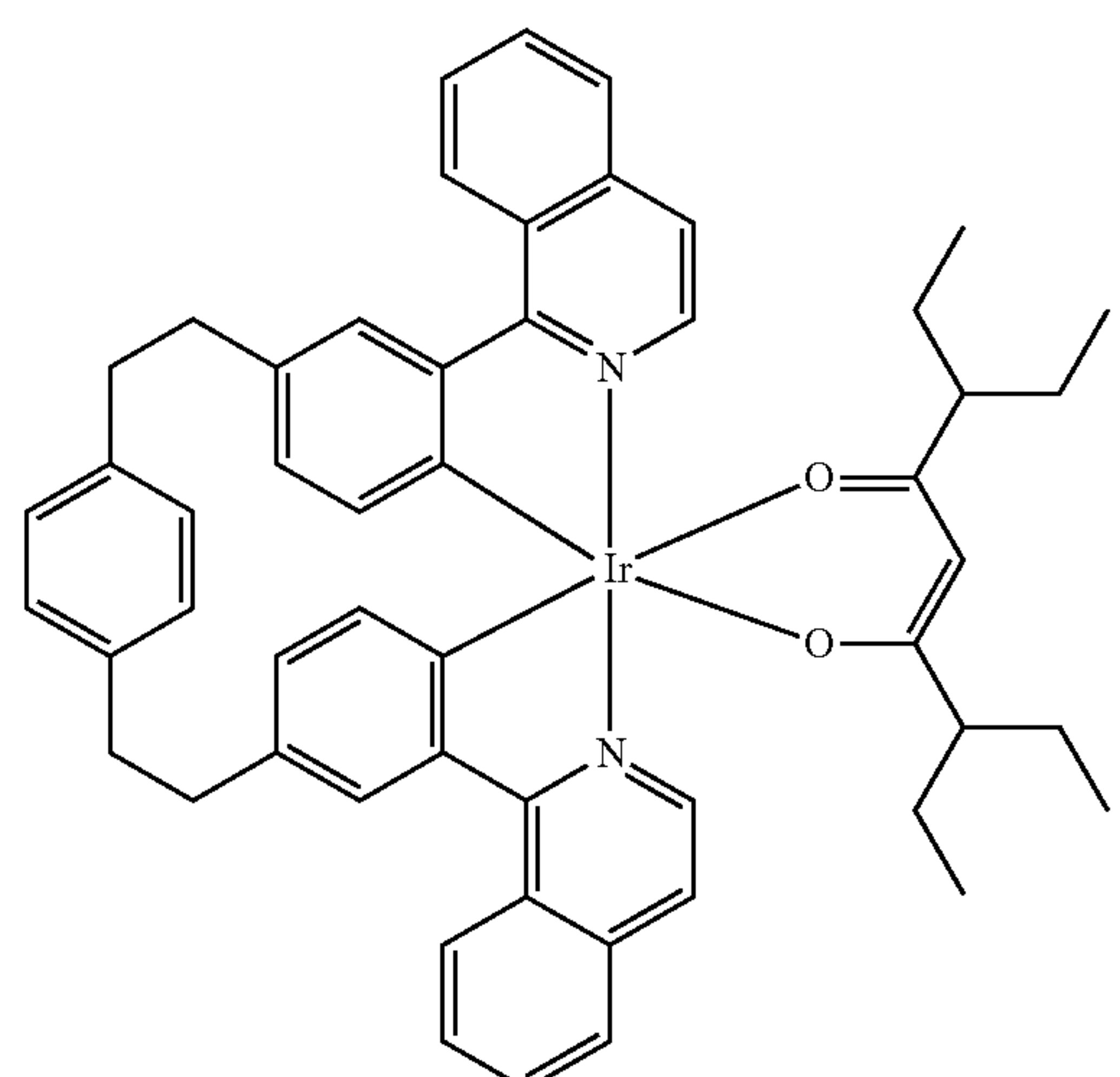
Compound 114
