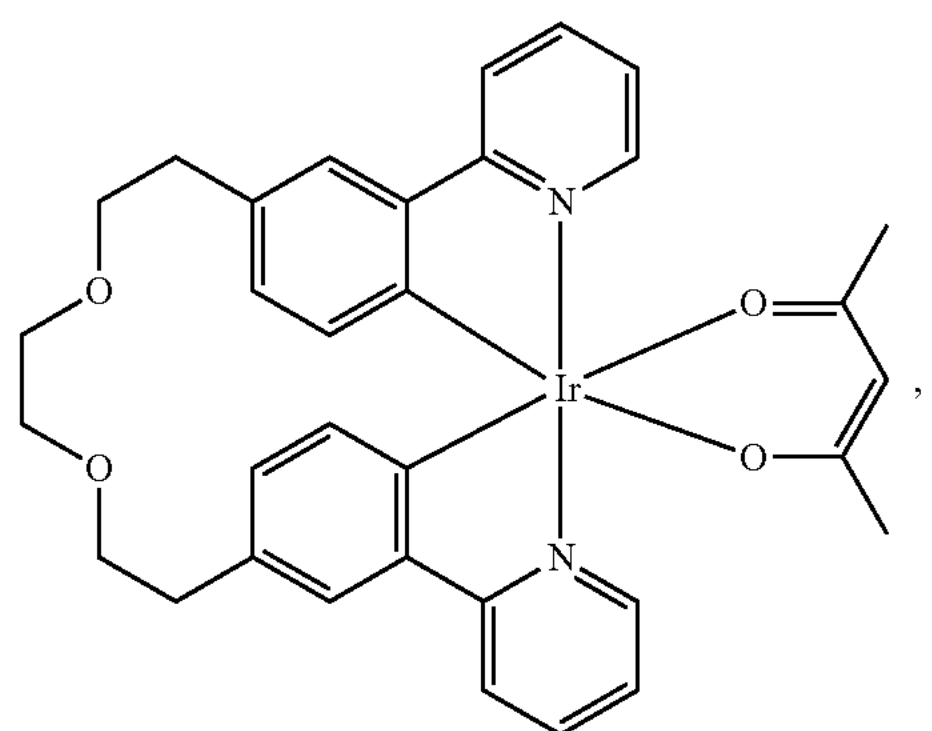
Compound 20
