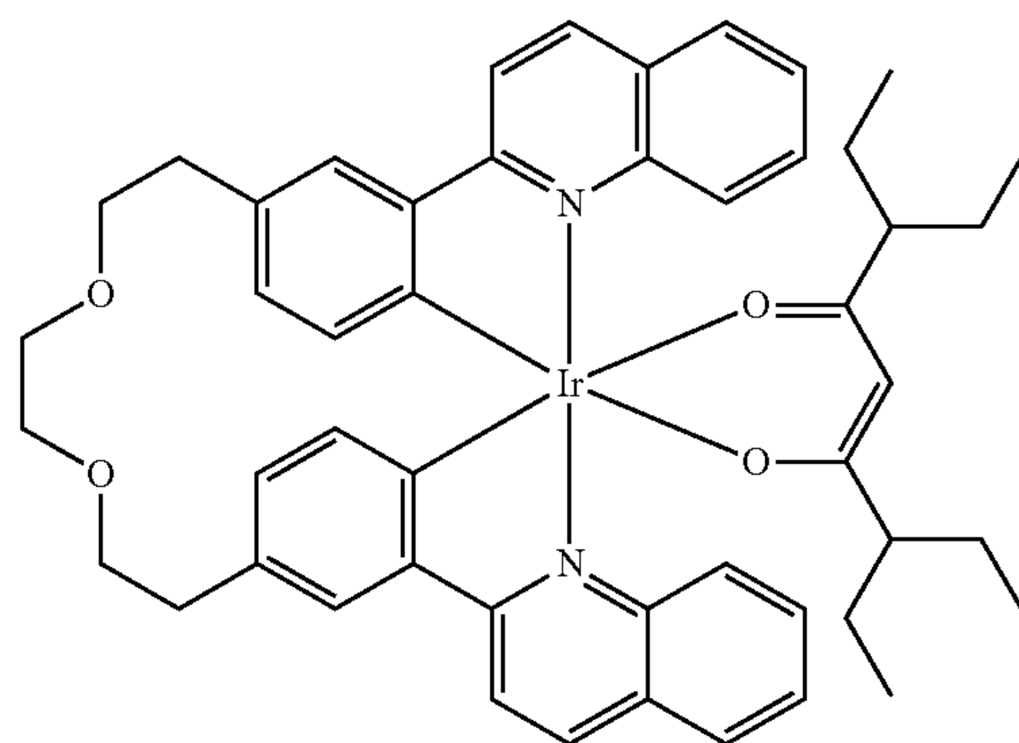
Compound 70
