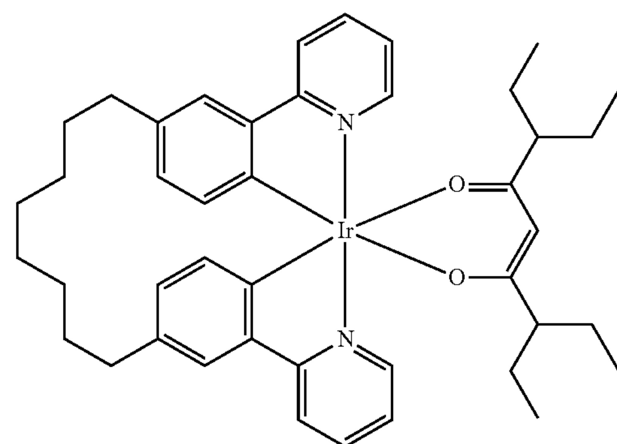
Compound 19
