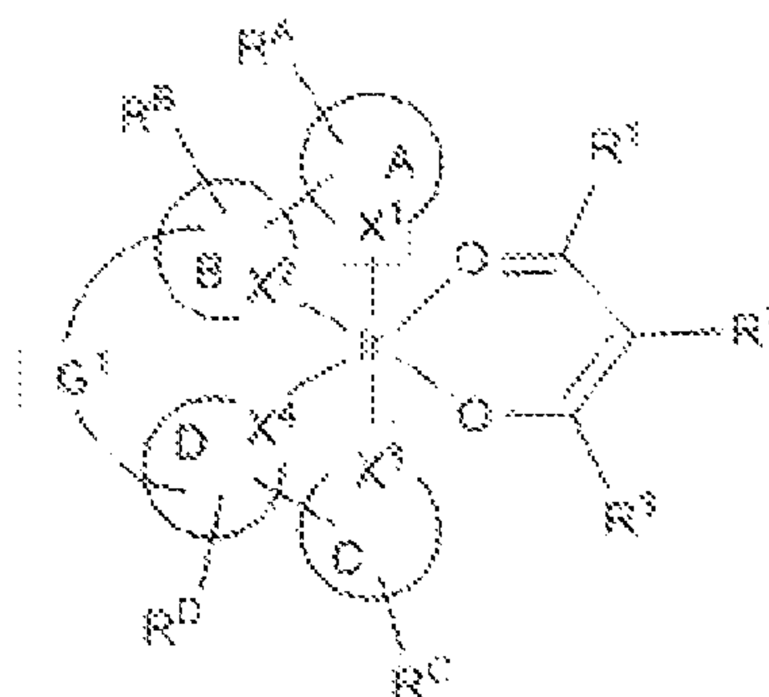
Formula VII
