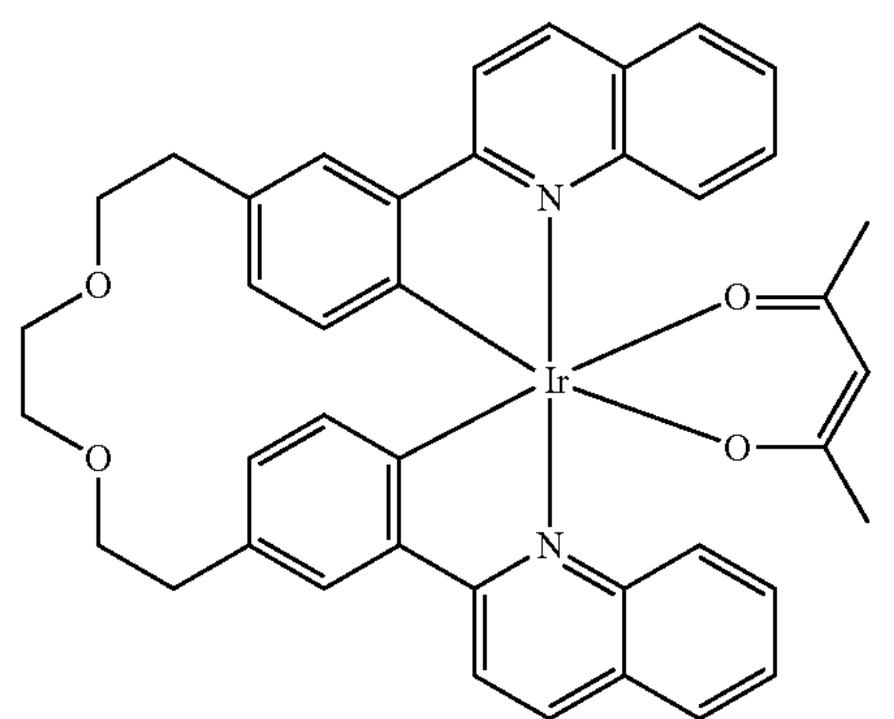
Compound 70
