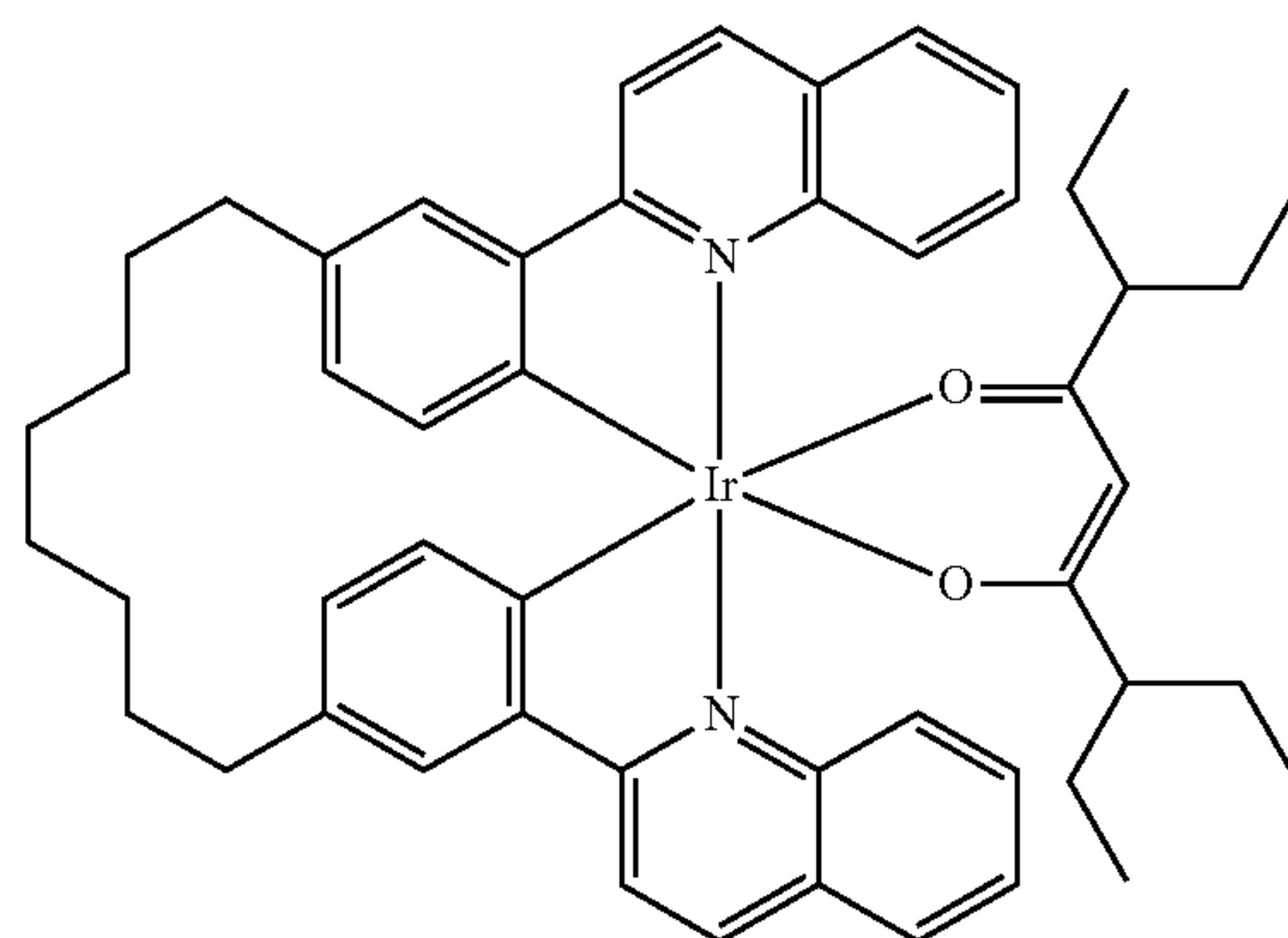
Compound 68
