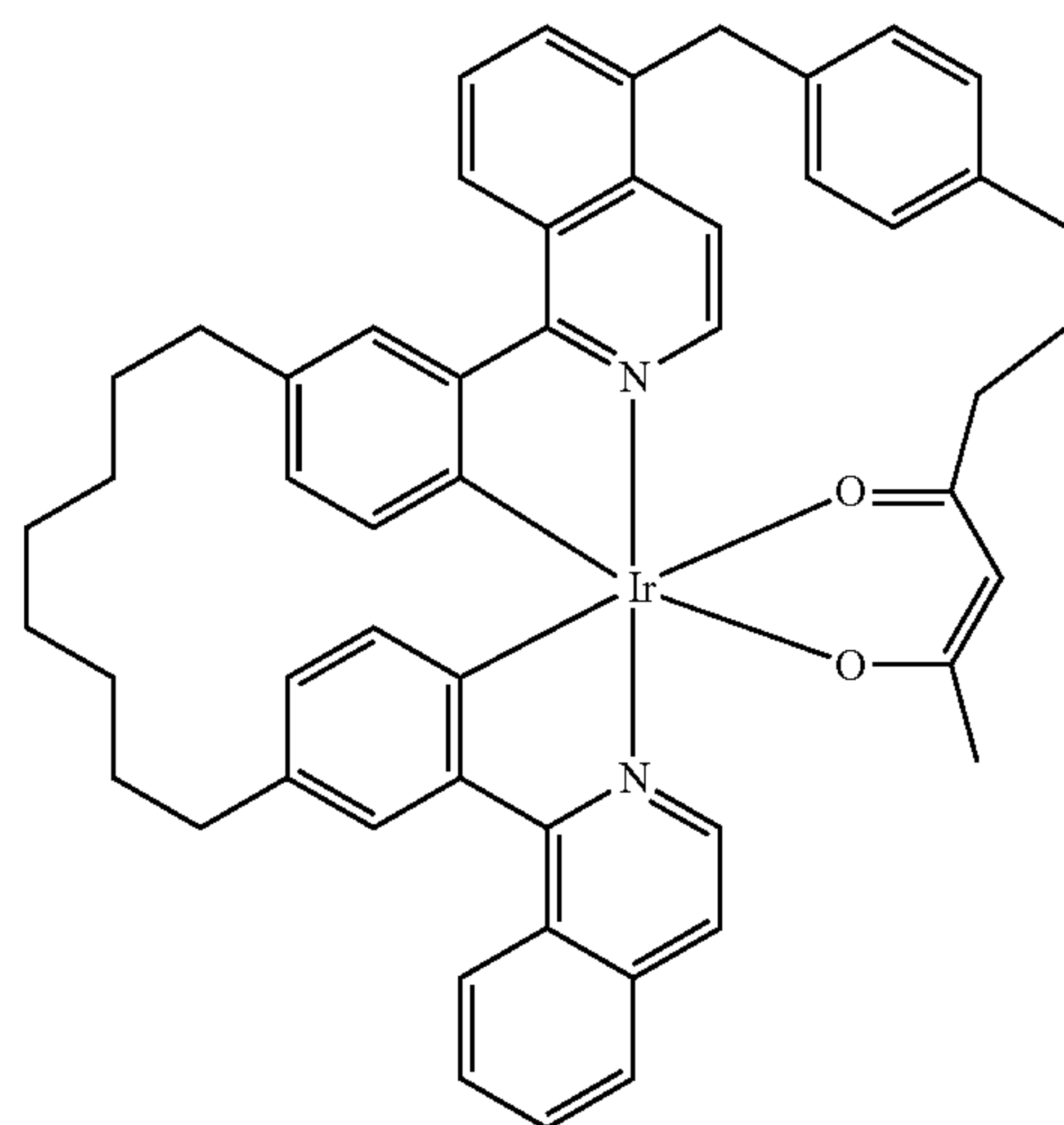
Compound 102
