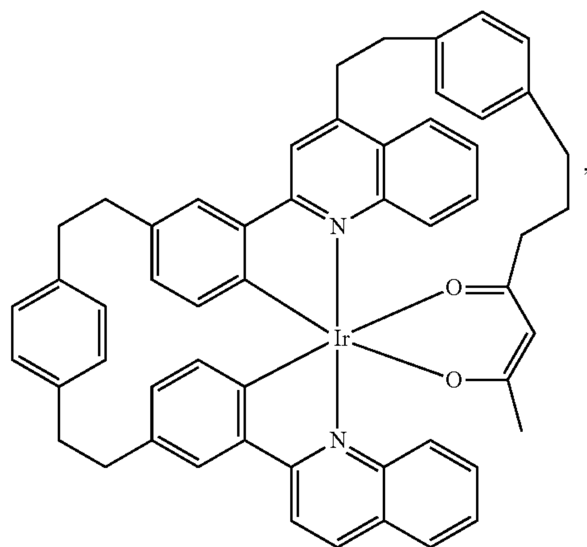
Compound 53
