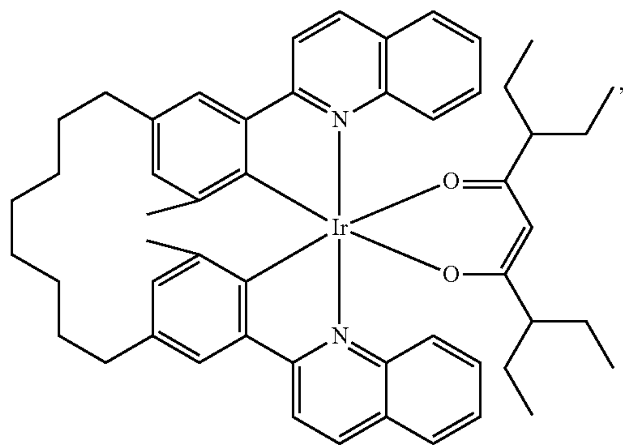
Compound 74
