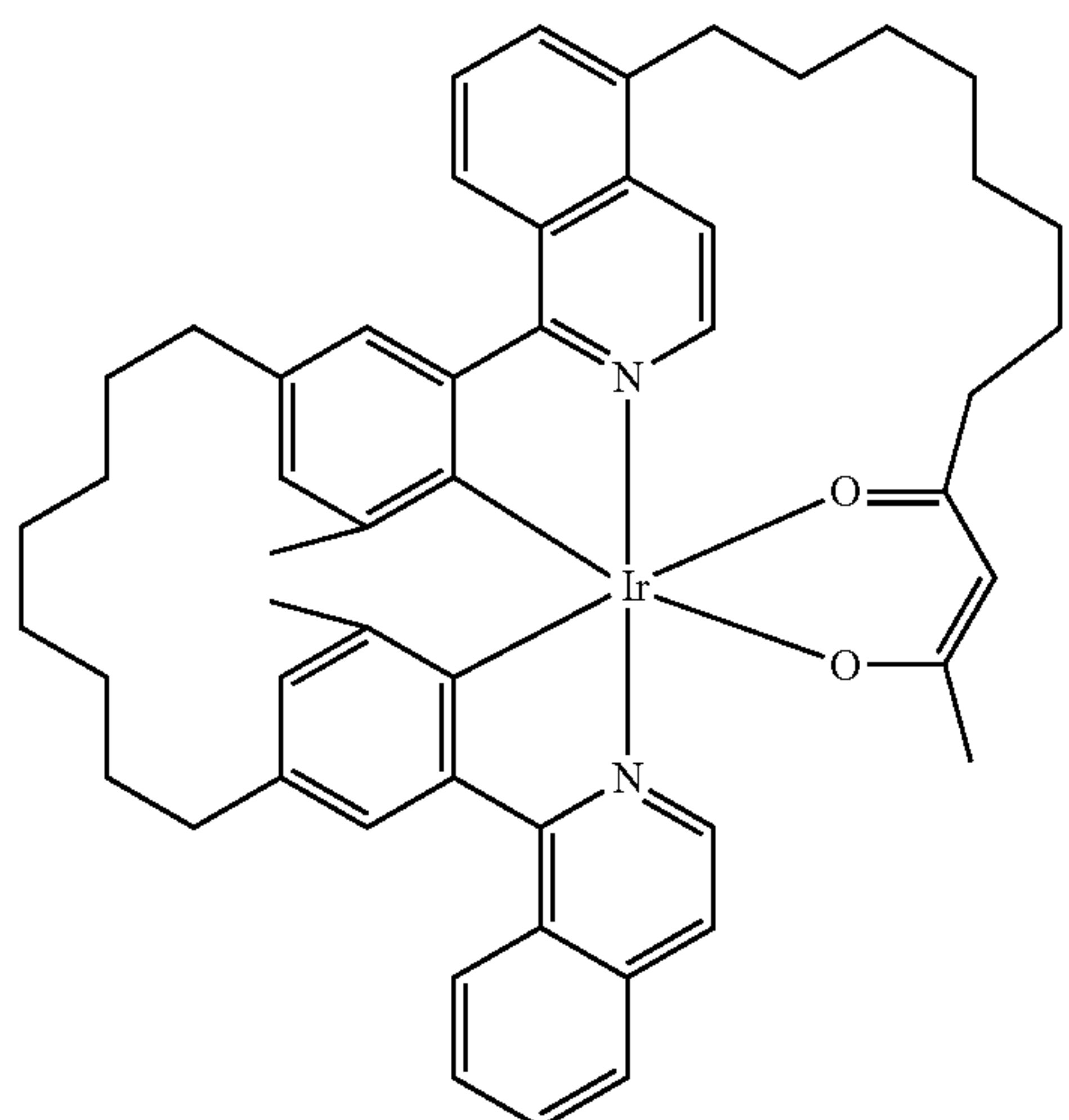
Compound 110
