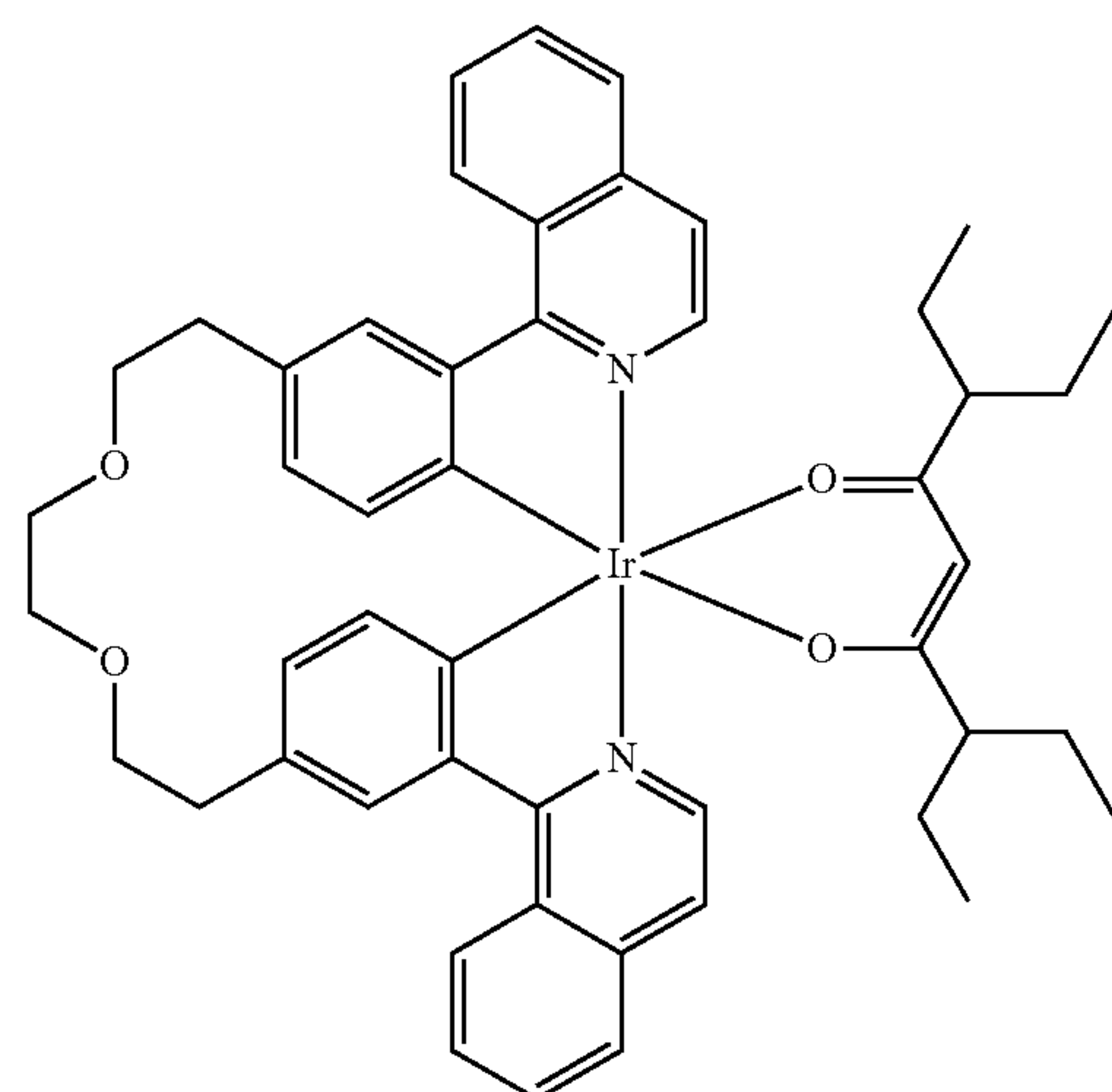
Compound 118
