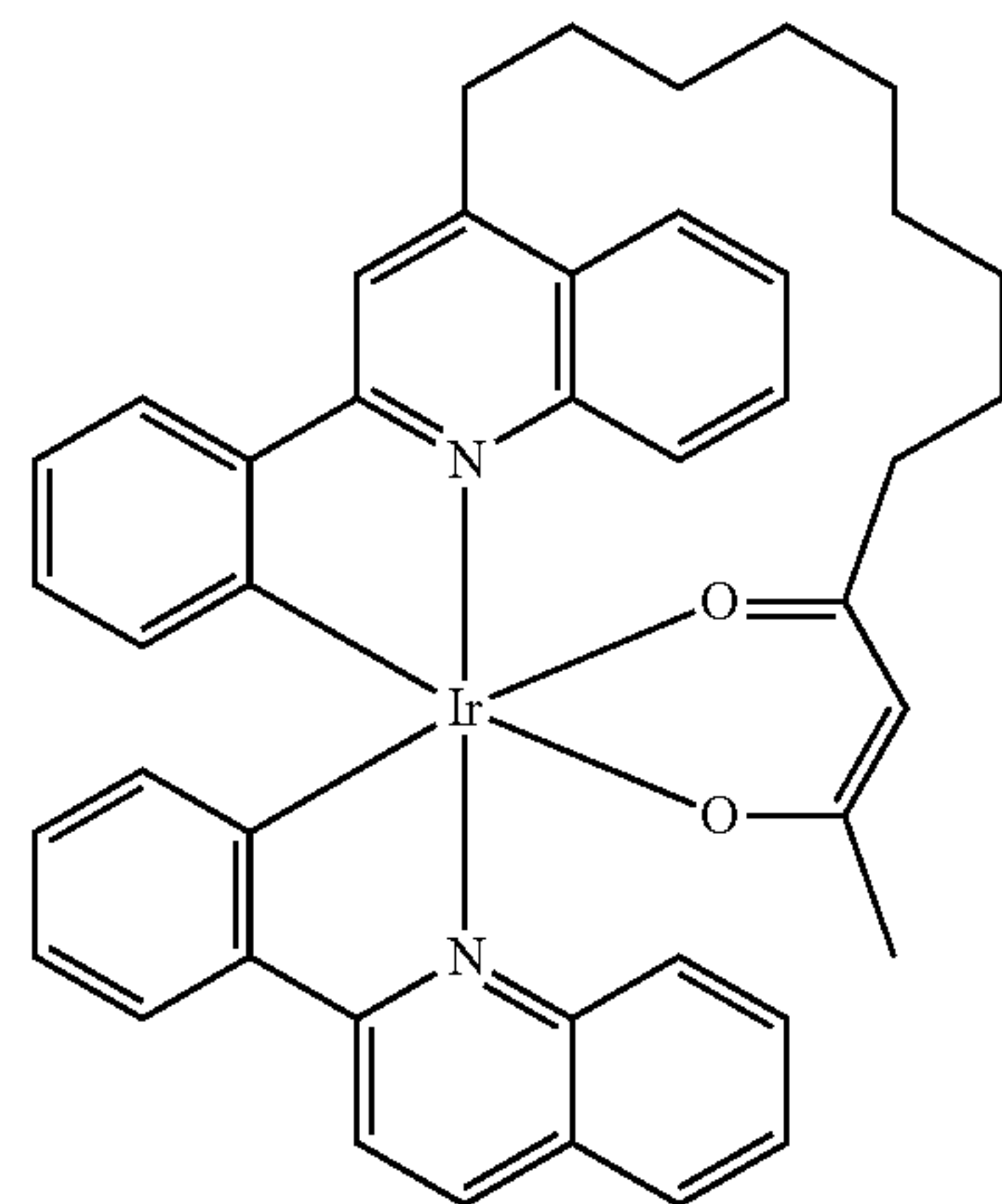
Compound 78
