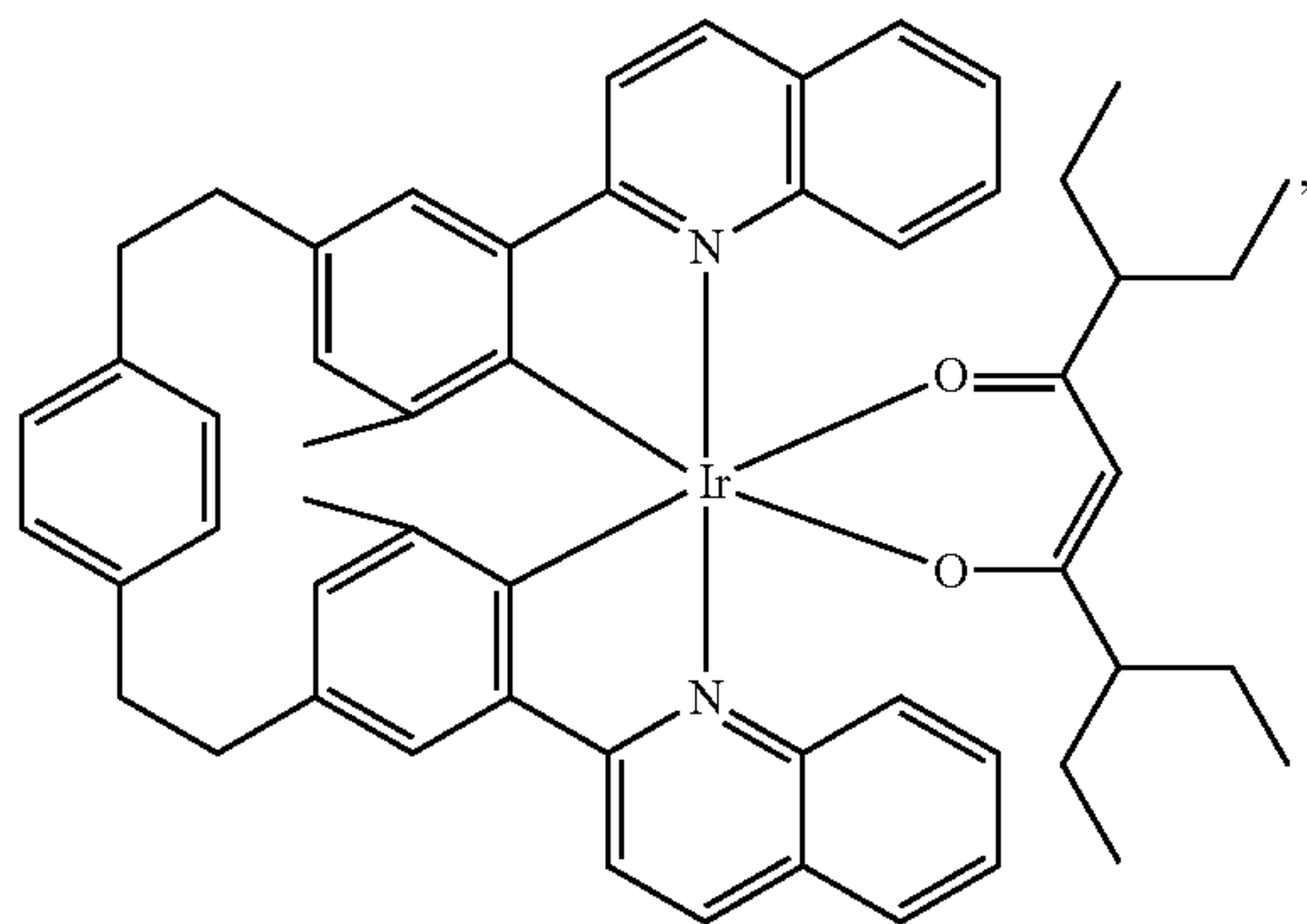
Compound 72
