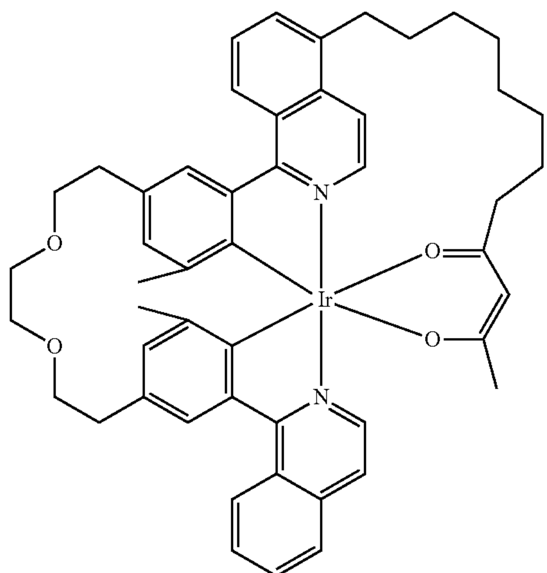
Compound 111
