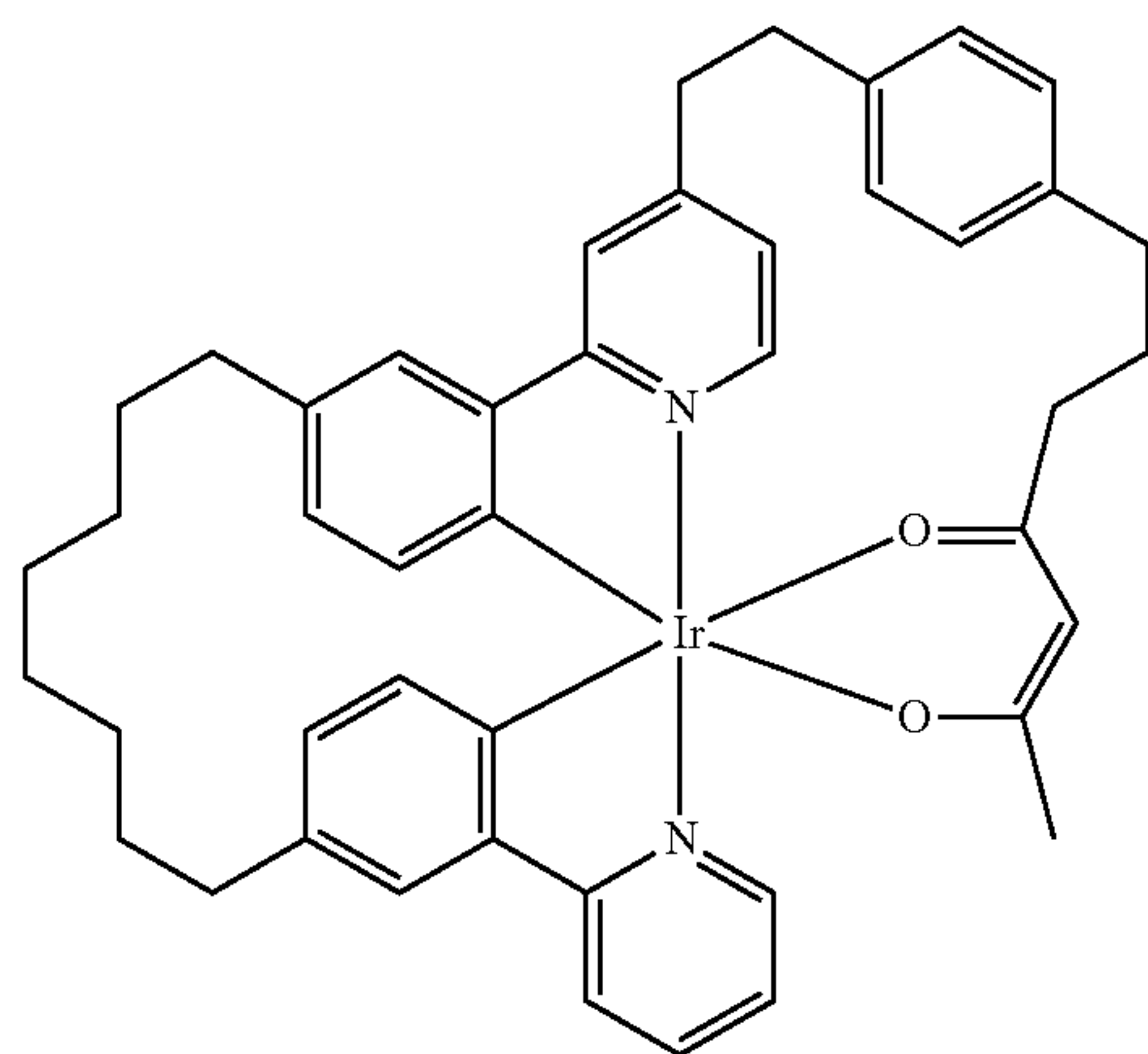
Compound 11
