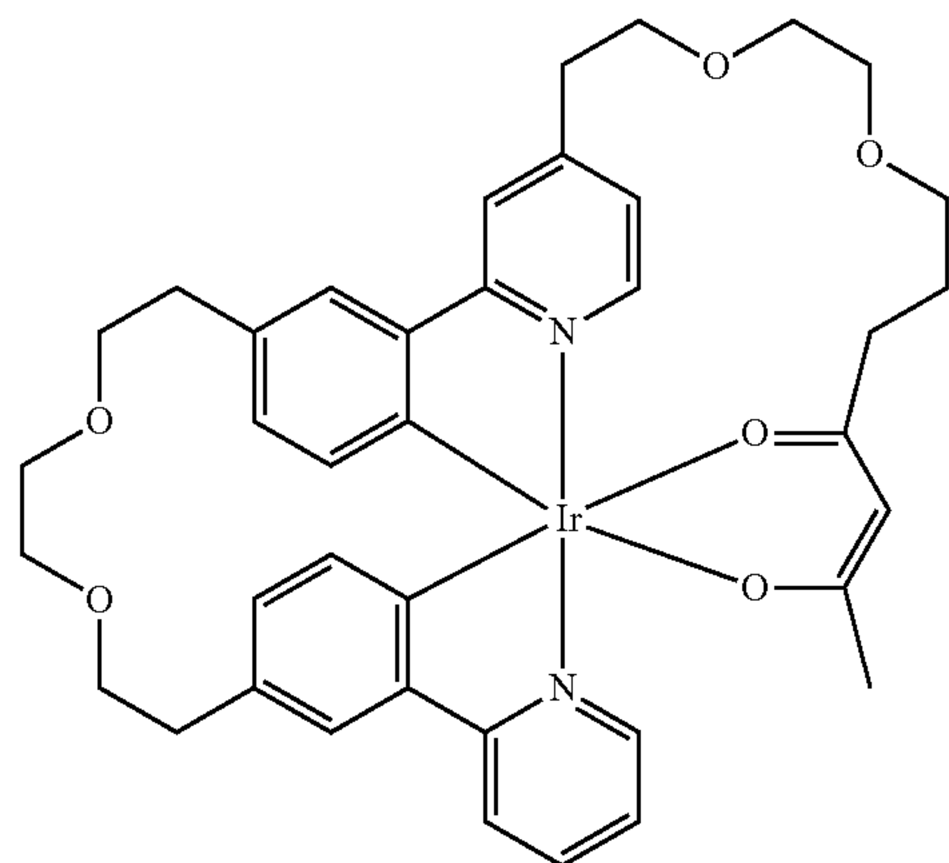
Compound 15
