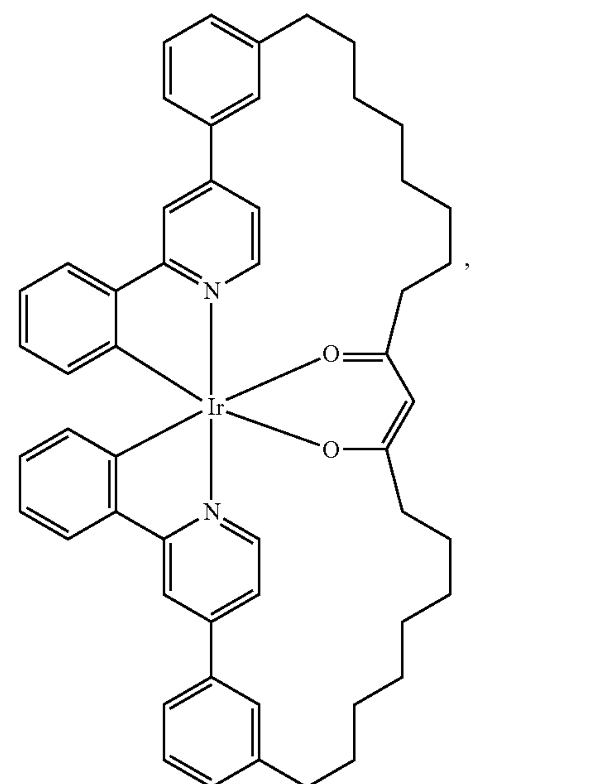
Compound 29
