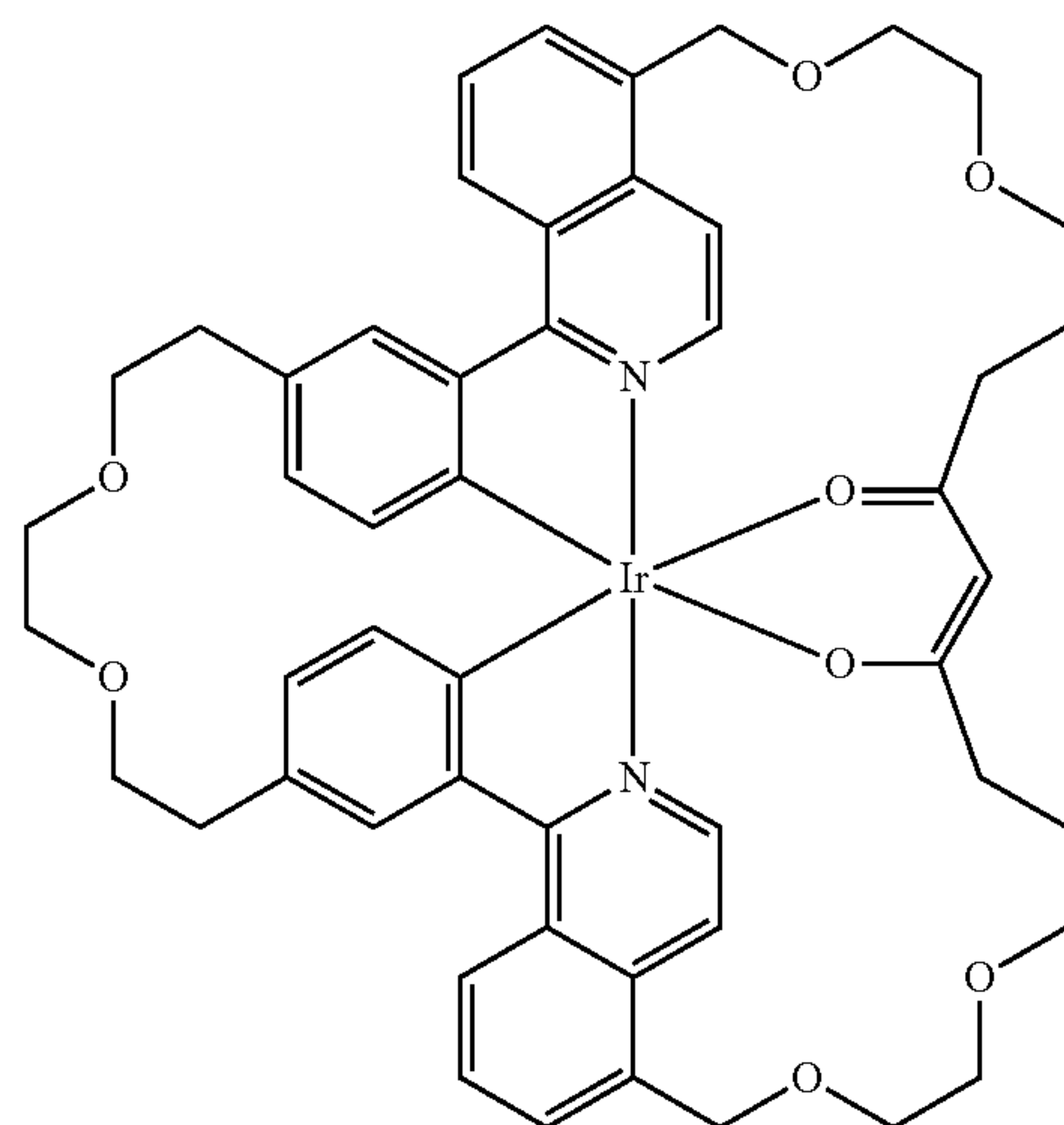
Compound 88
