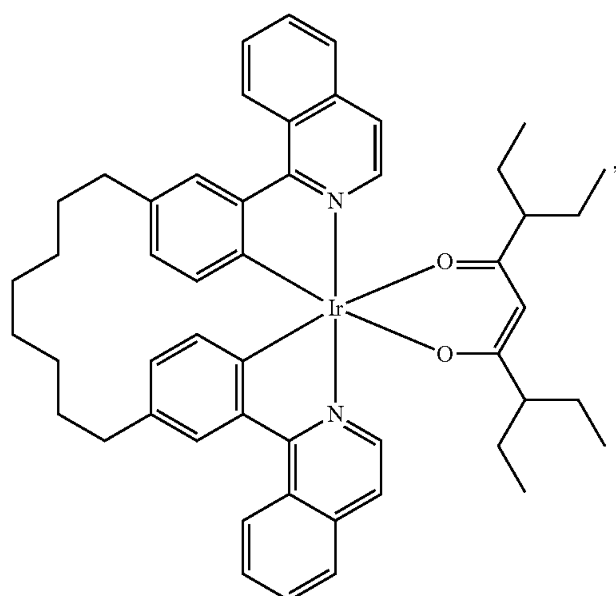
Compound 116
