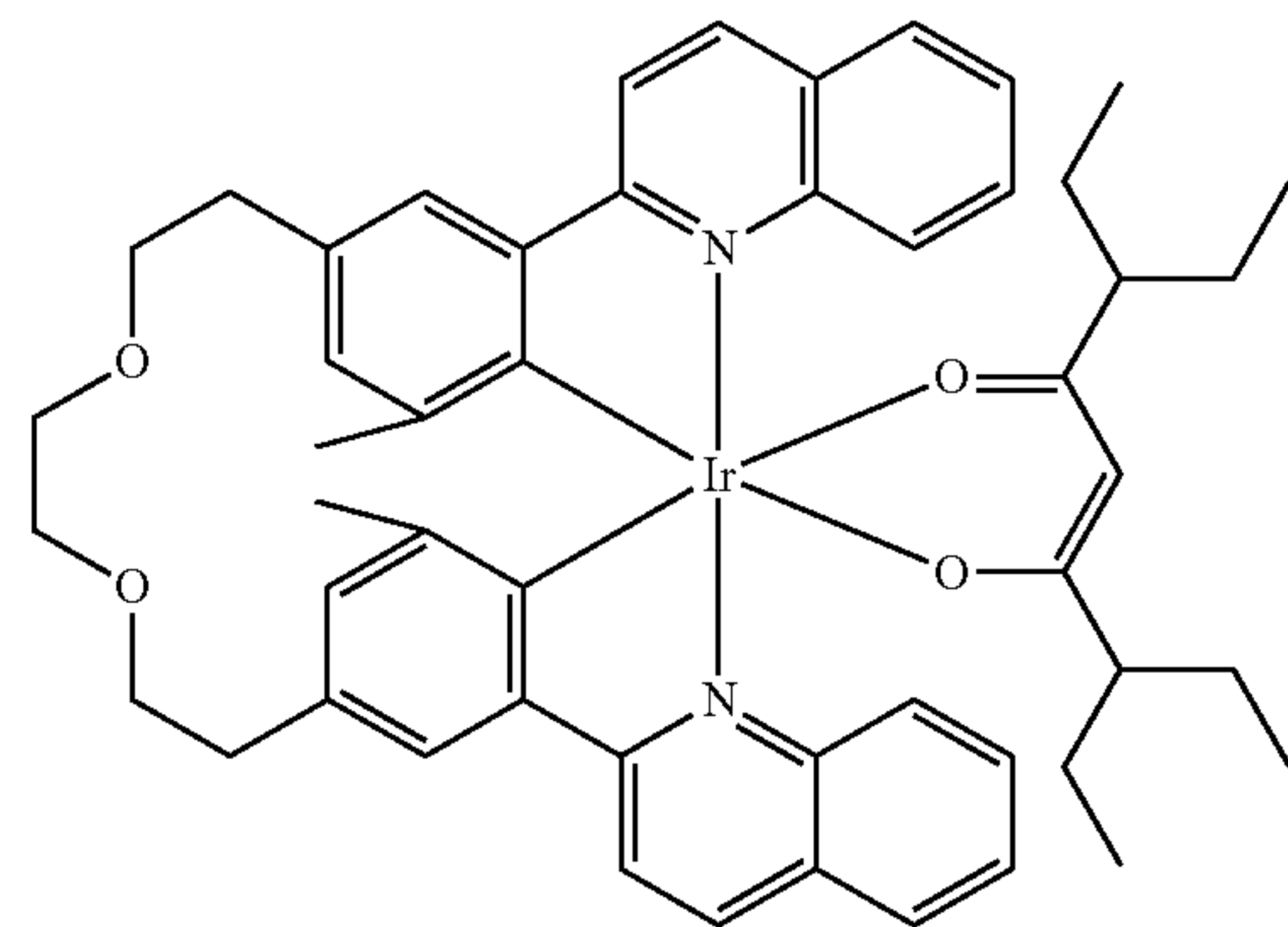
Compound 76
