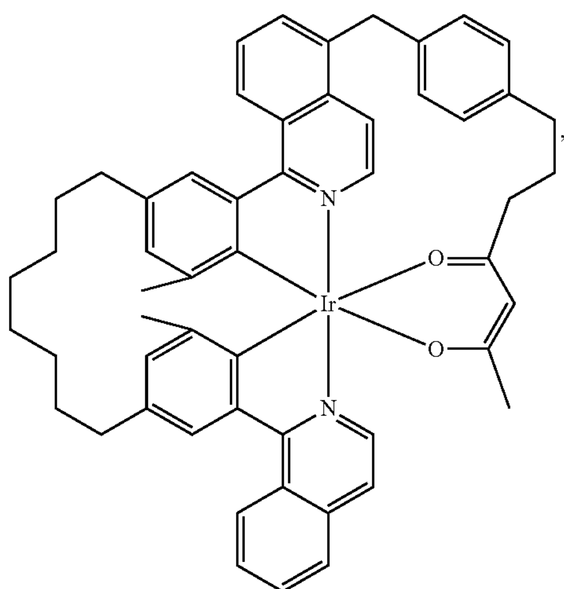
Compound 104
