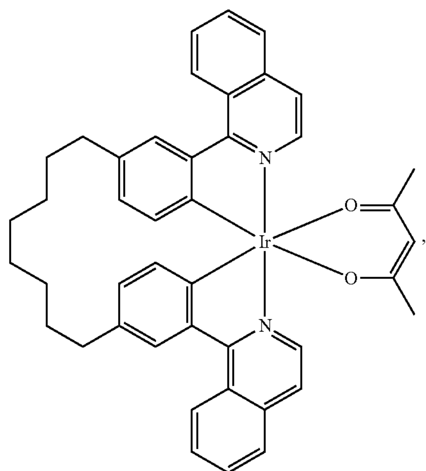
Compound 115
