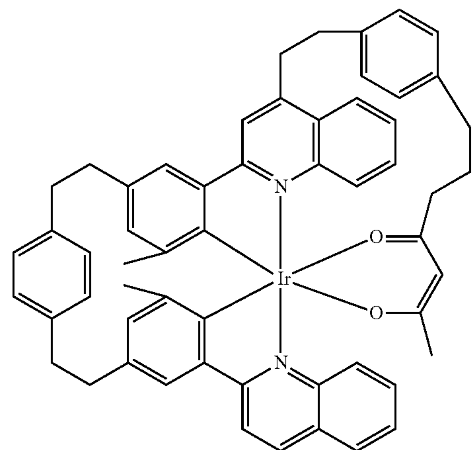
Compound 55
