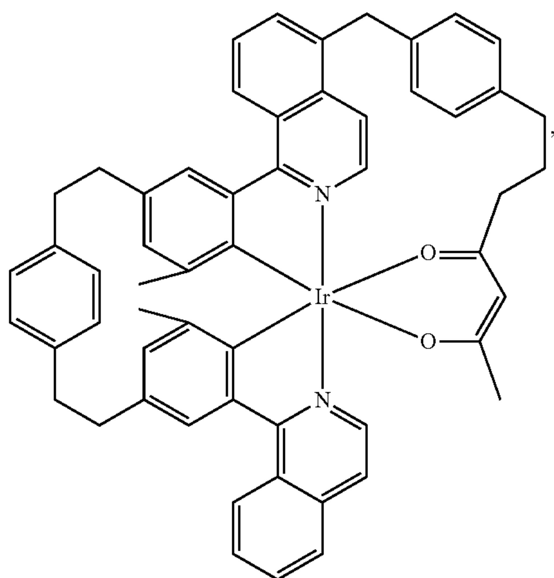
Compound 103
