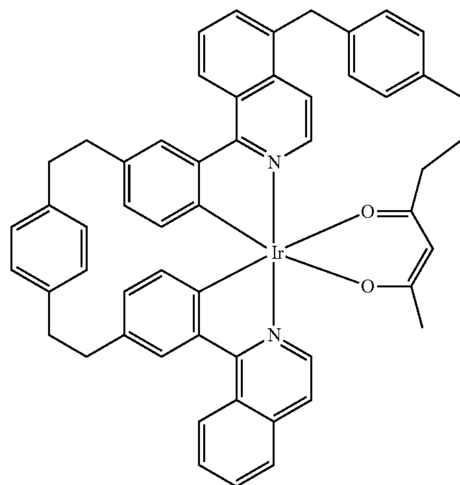
Compound 101
