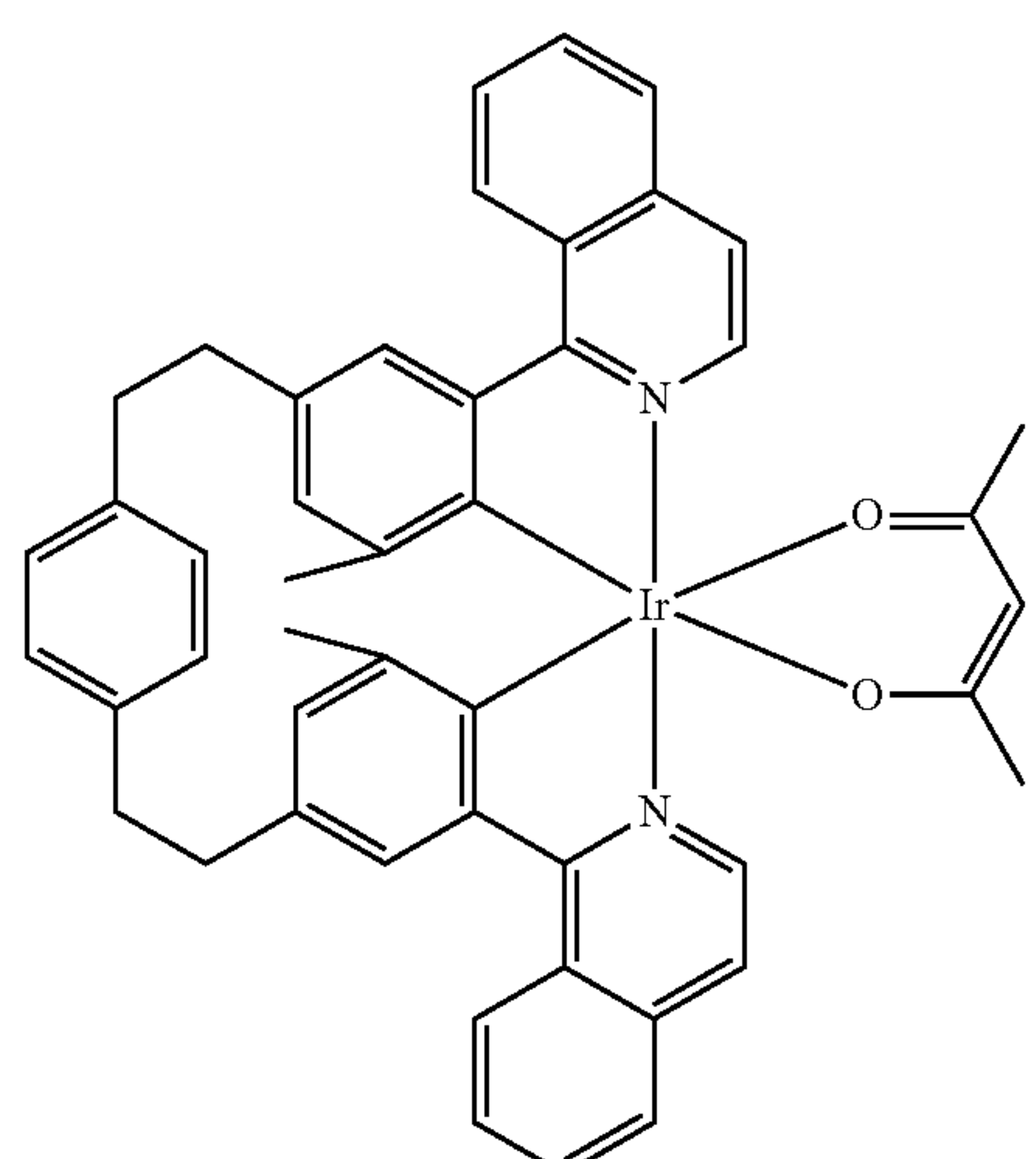
Compound 119
