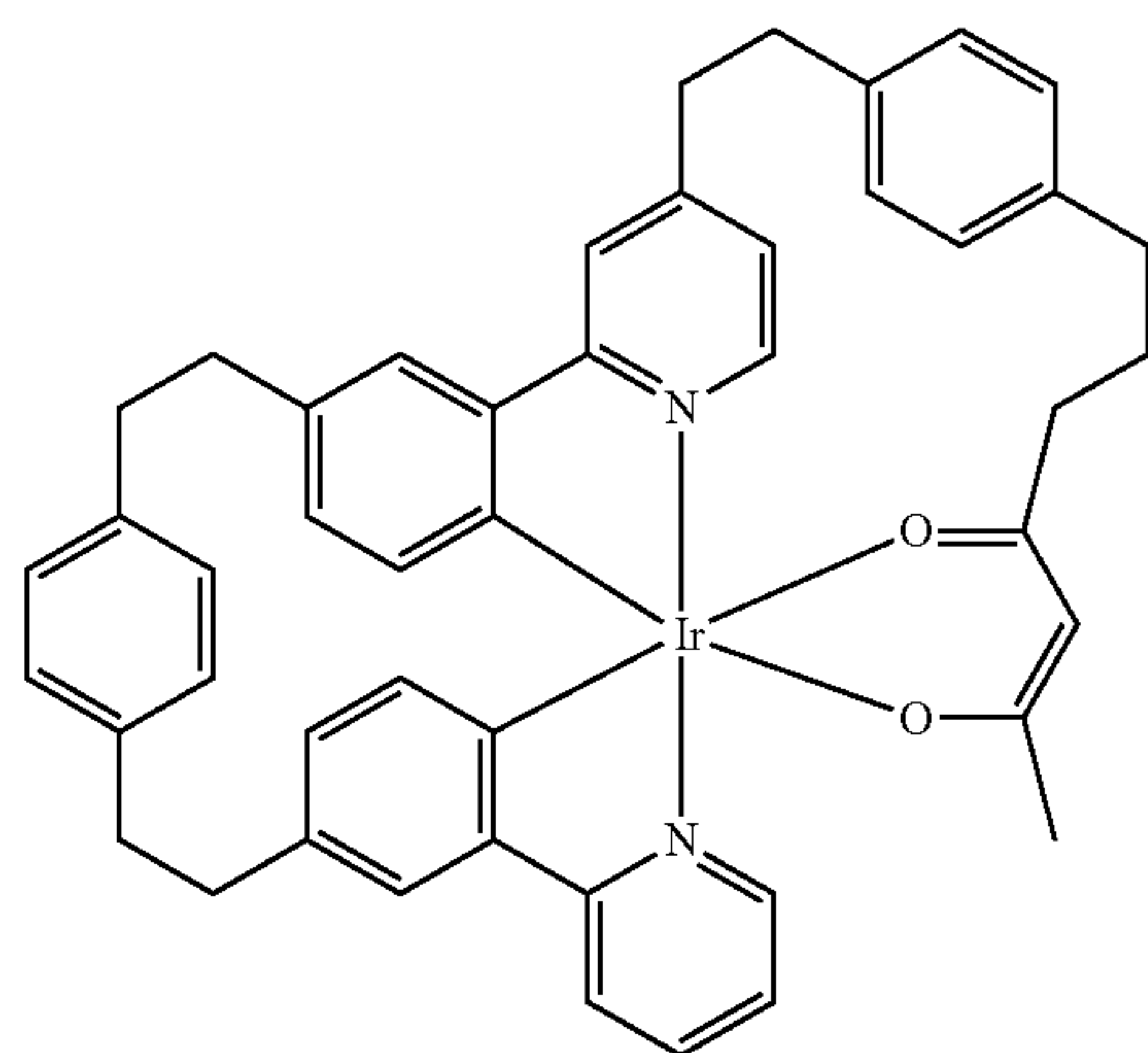
Compound 10
