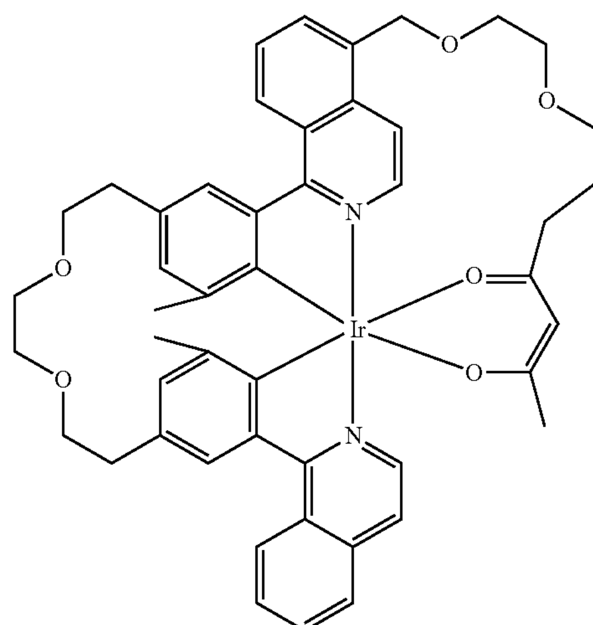
Compound 112
