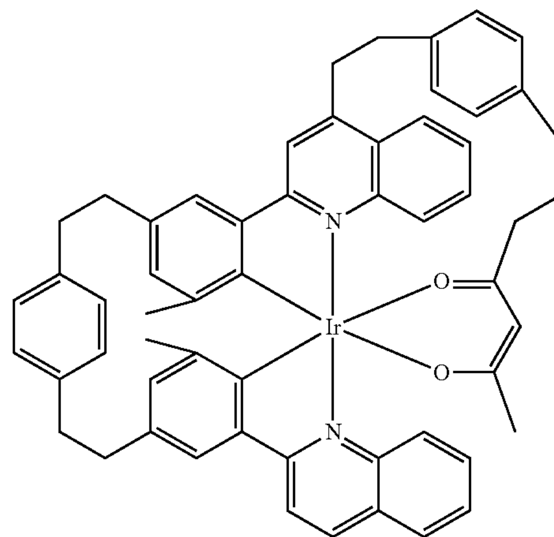
Compound 55
