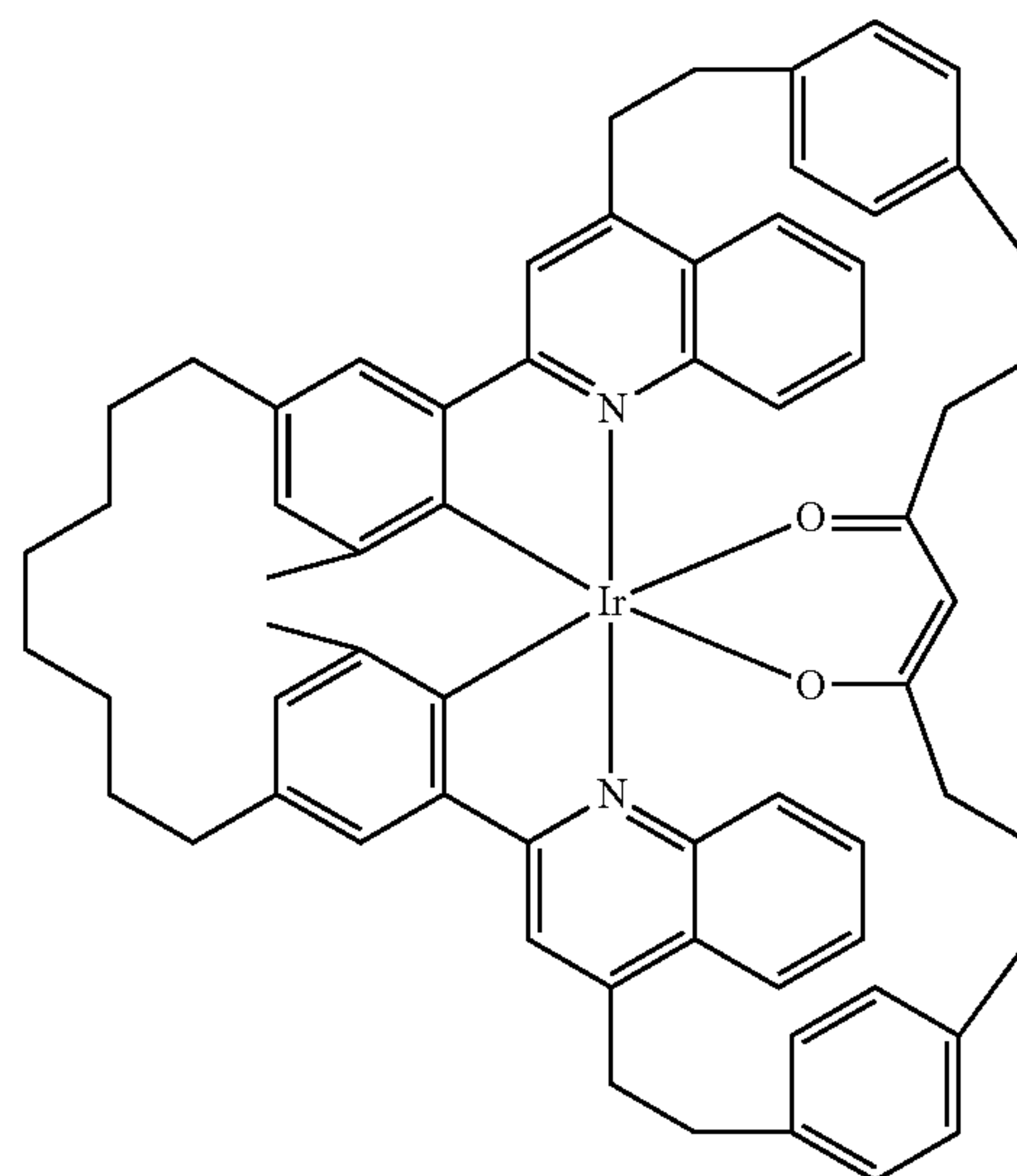
Compound 44
