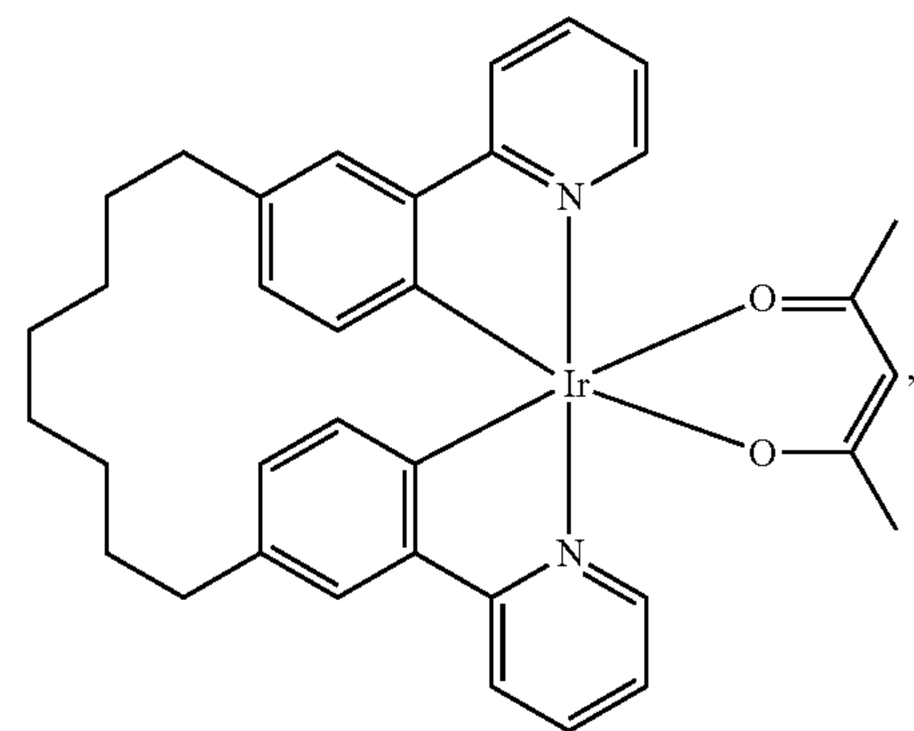
Compound 18
