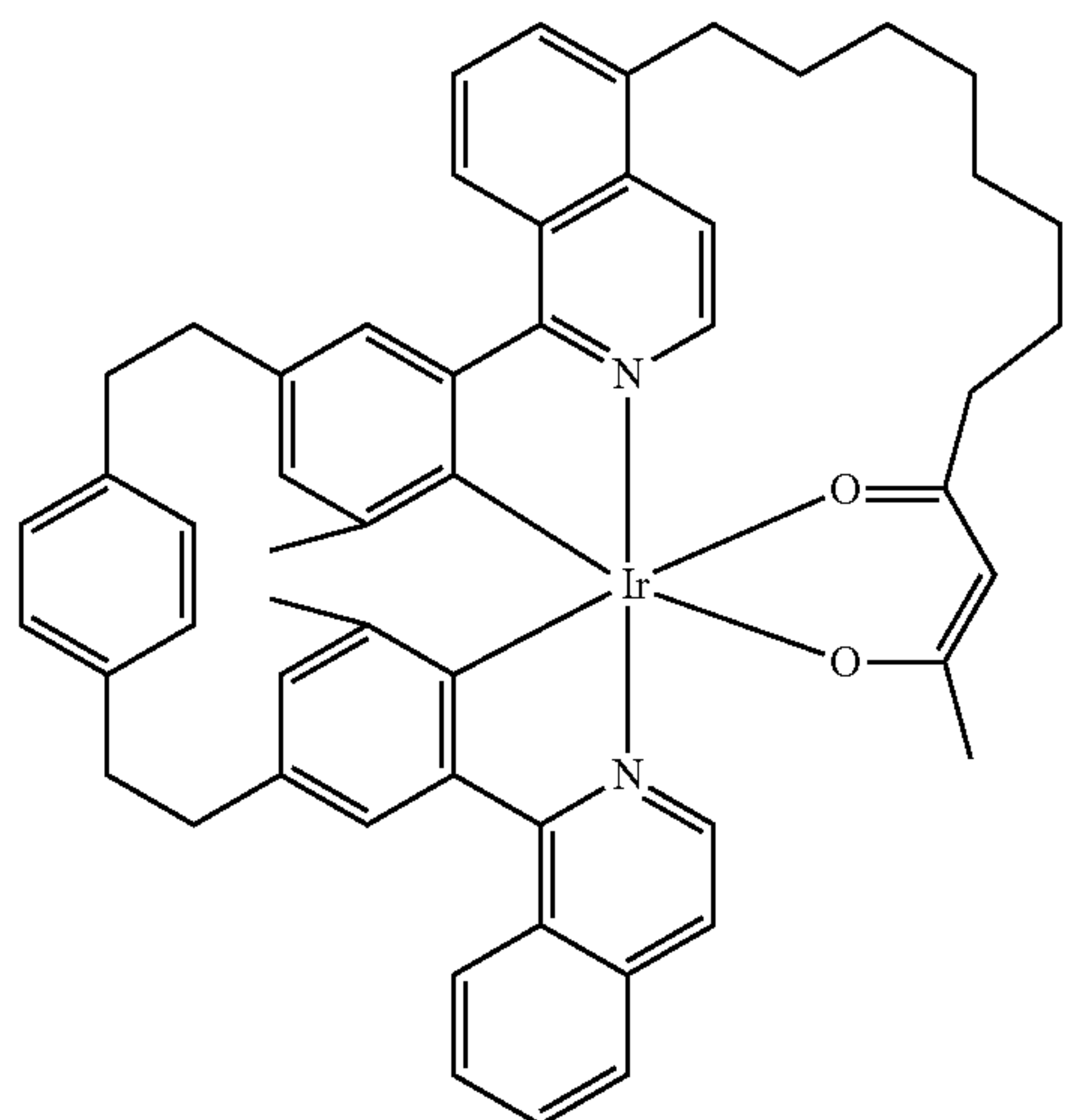
Compound 109
