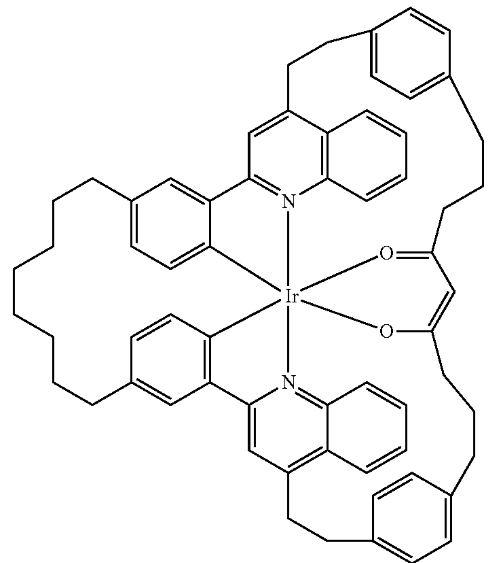
Compound 36
