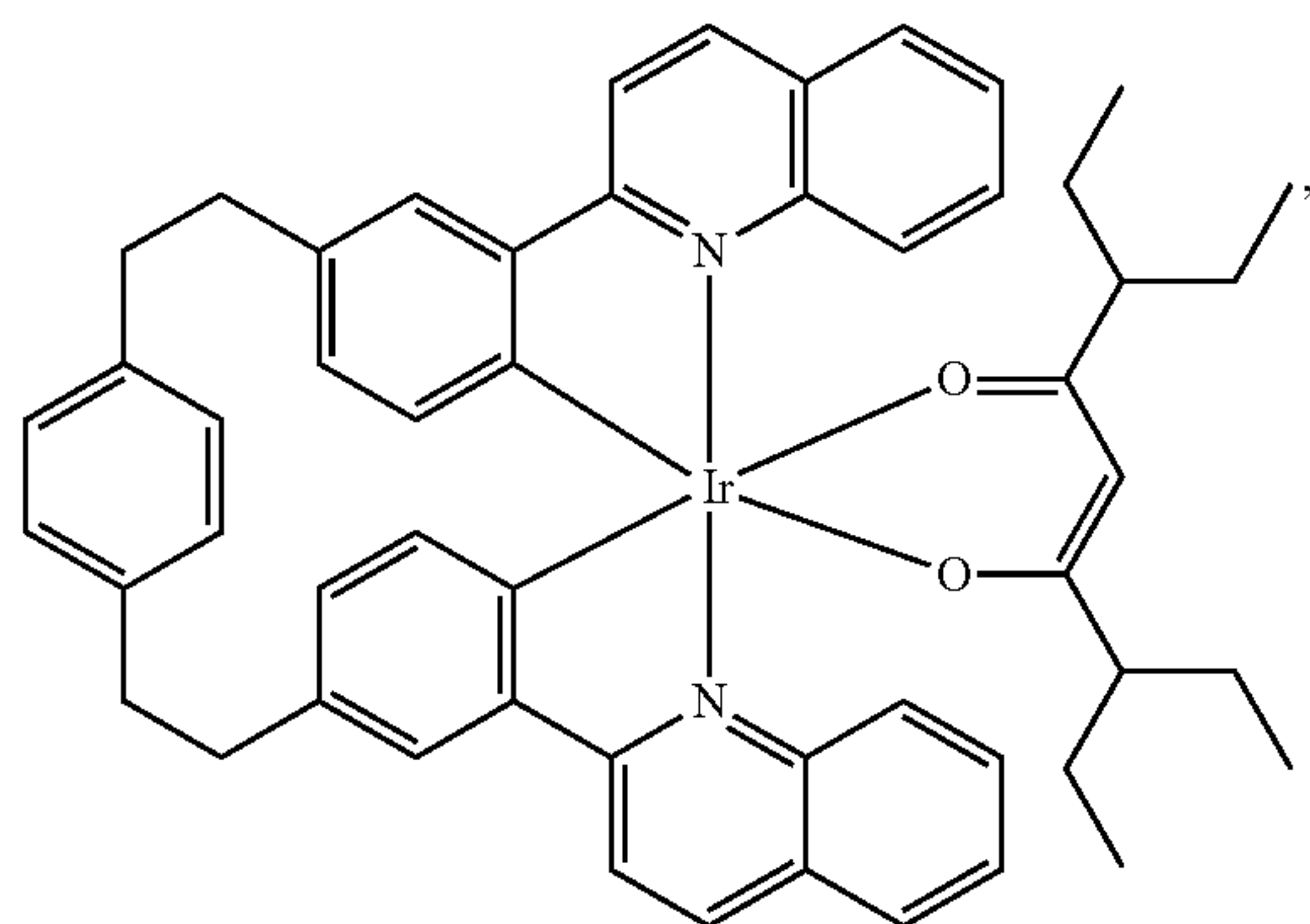
Compound 66
