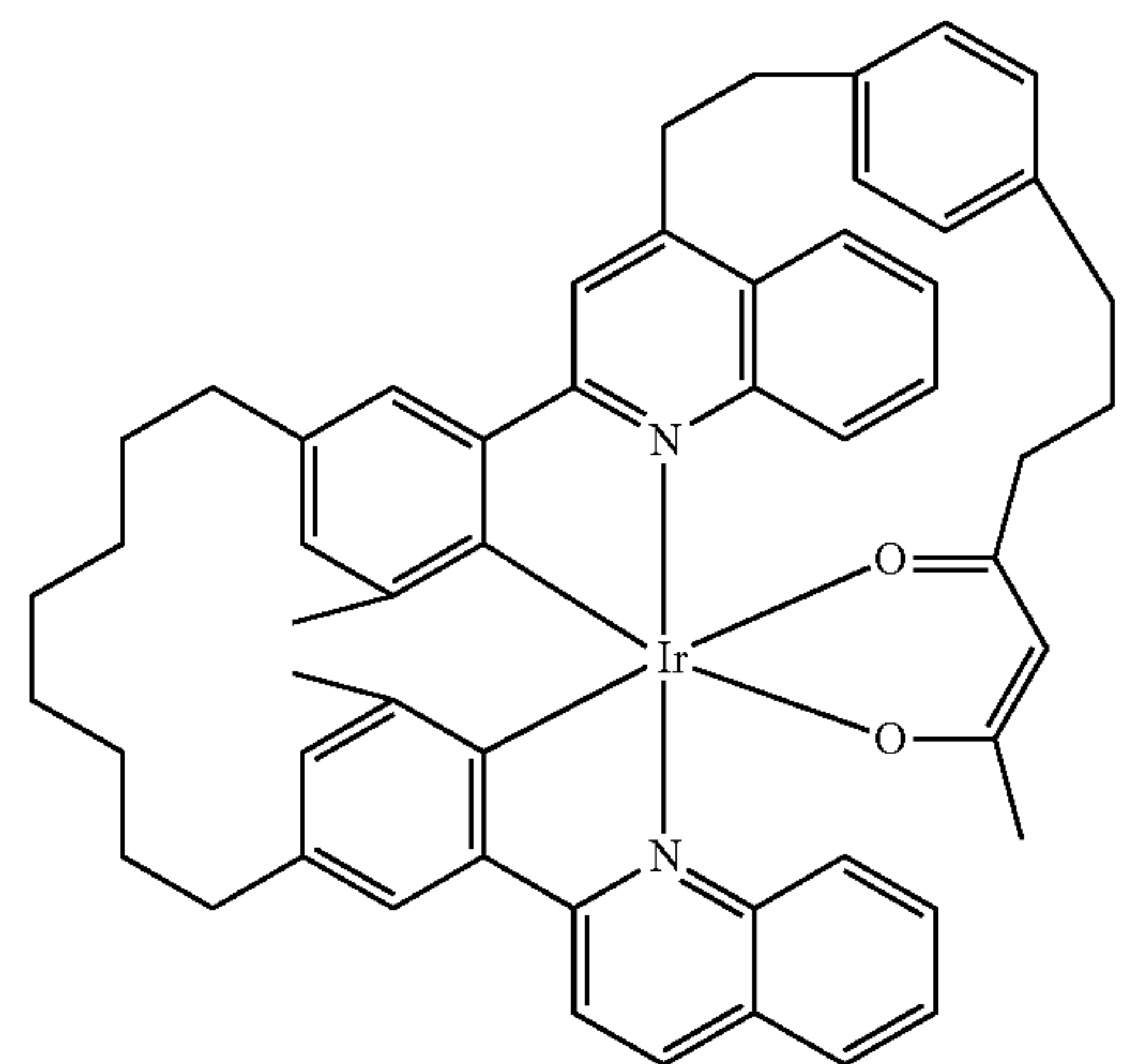
Compound 56
