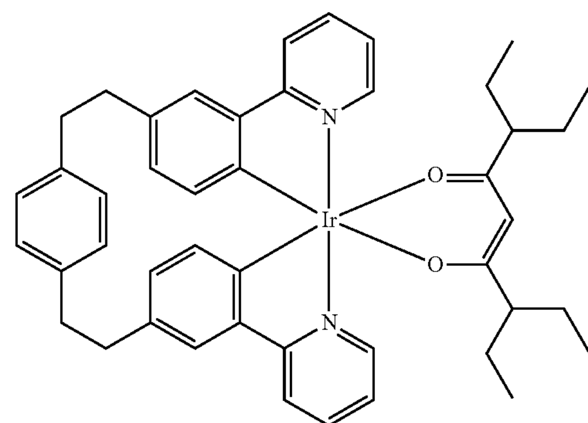
Compound 17
