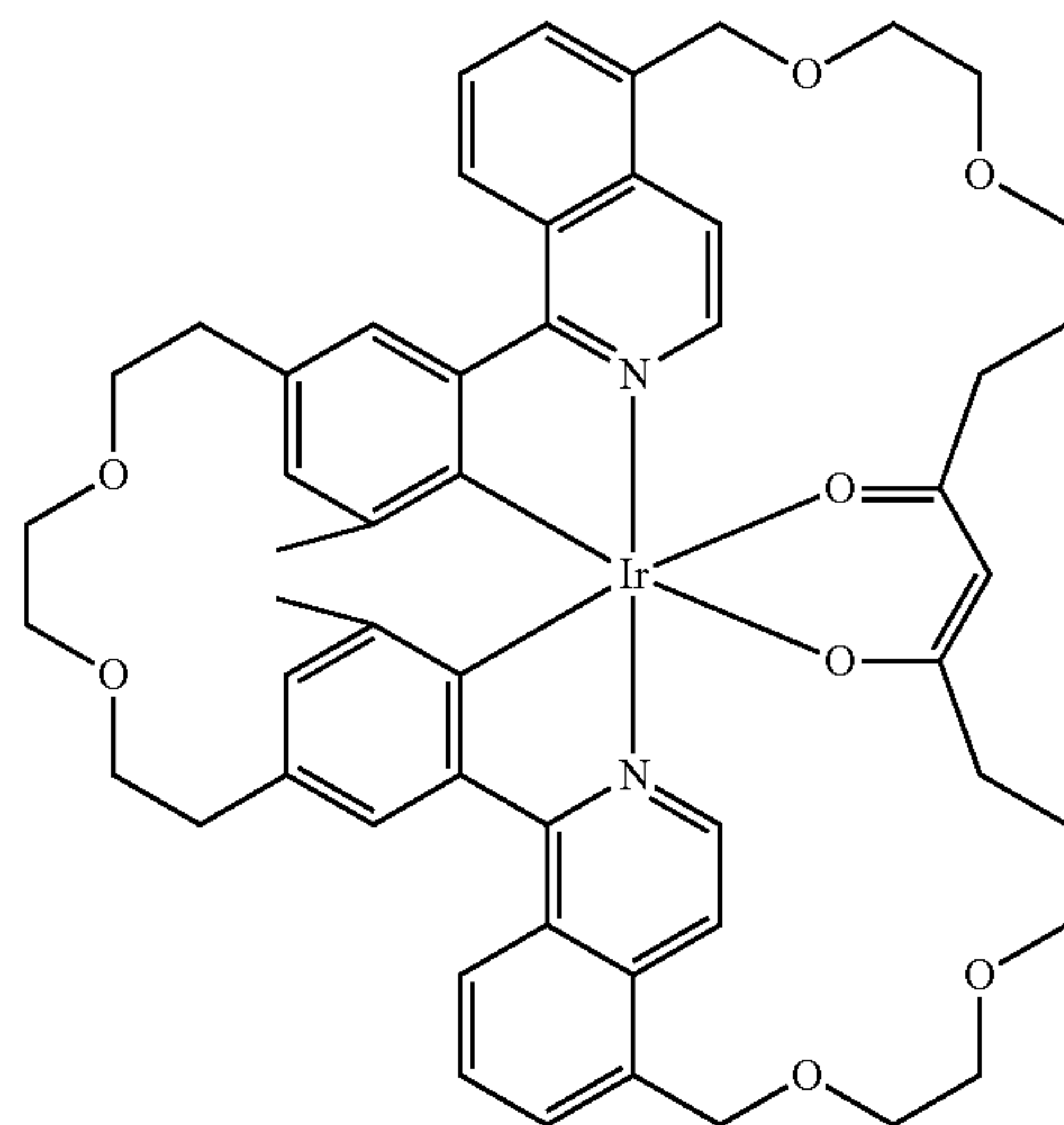
Compound 90
