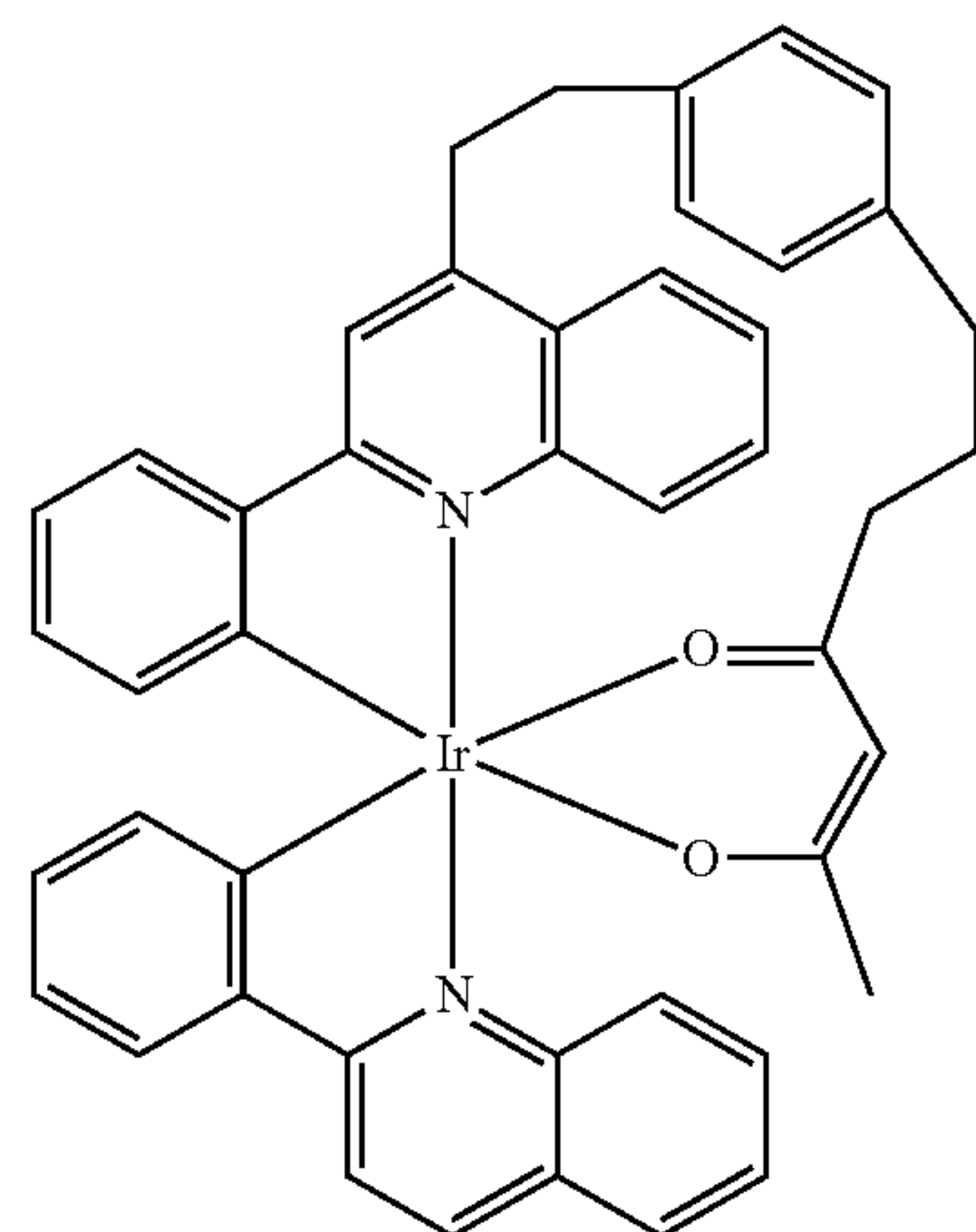
Compound 78
