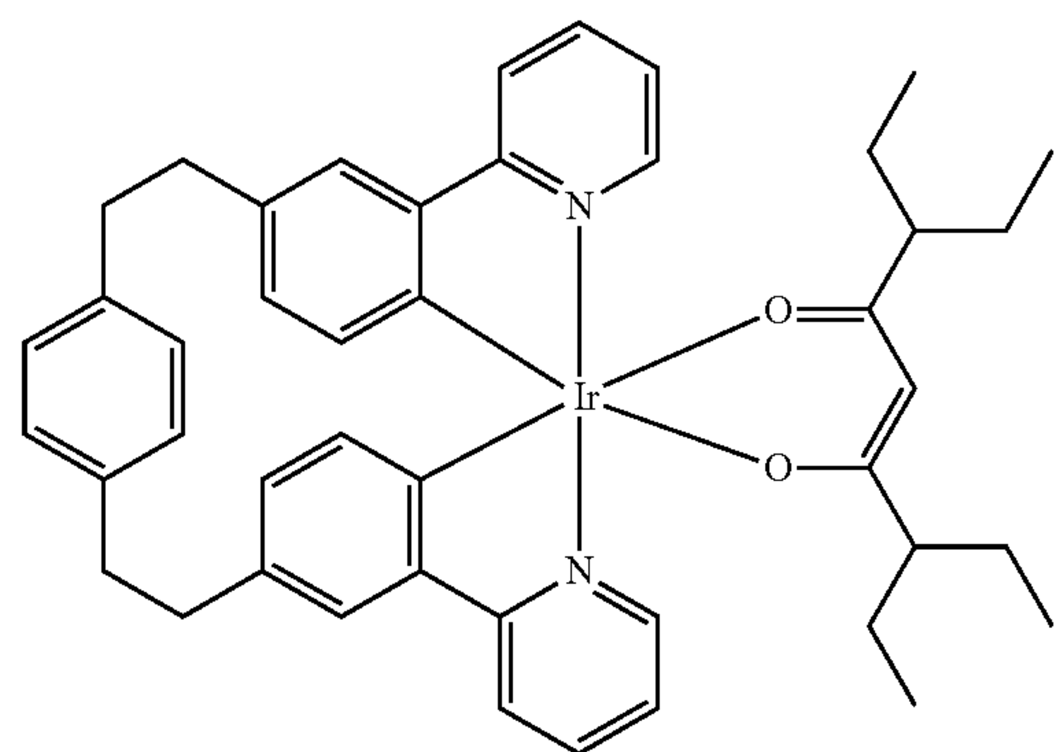
Compound 18
