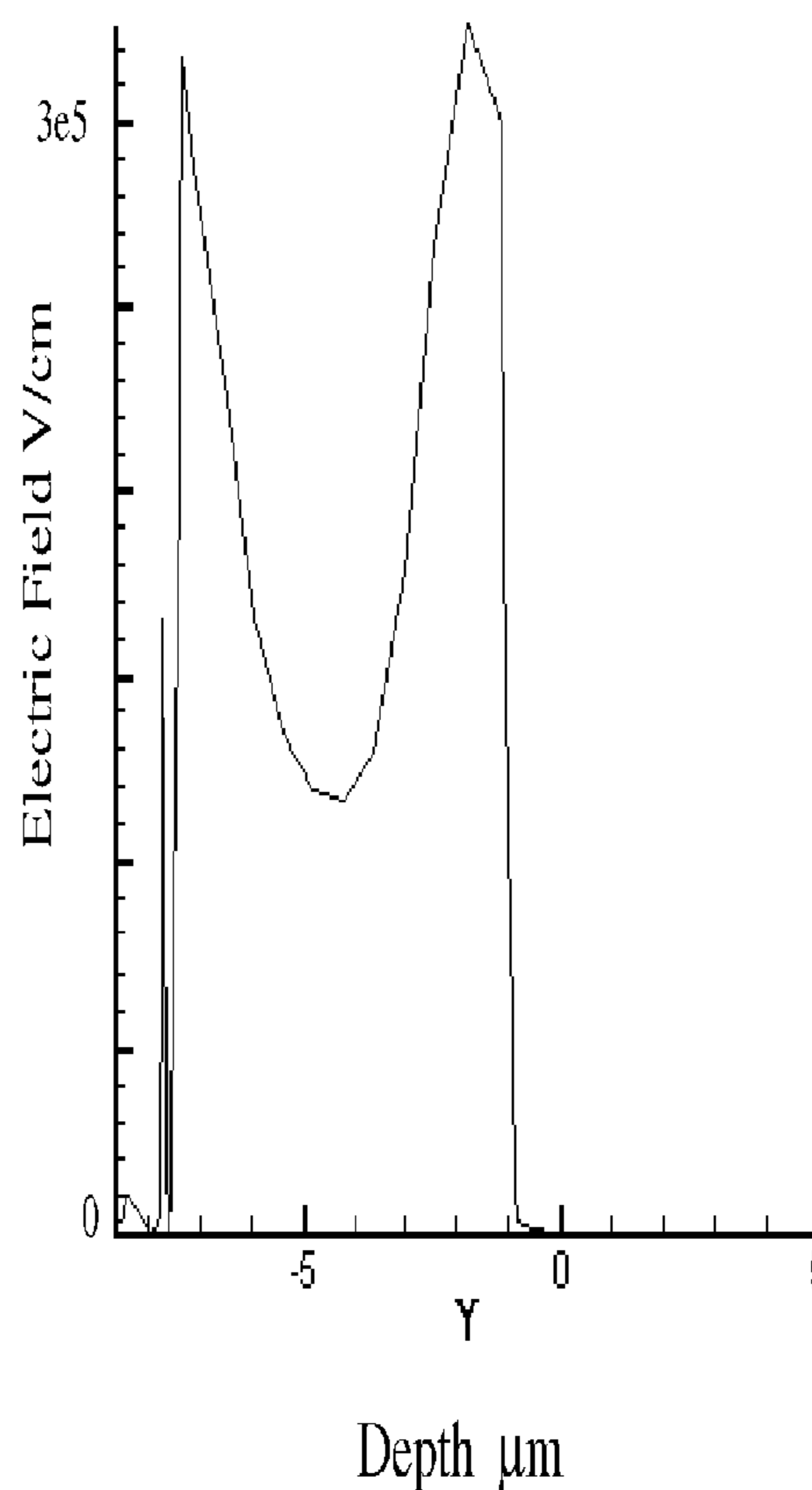
Electric Field vs. depth
