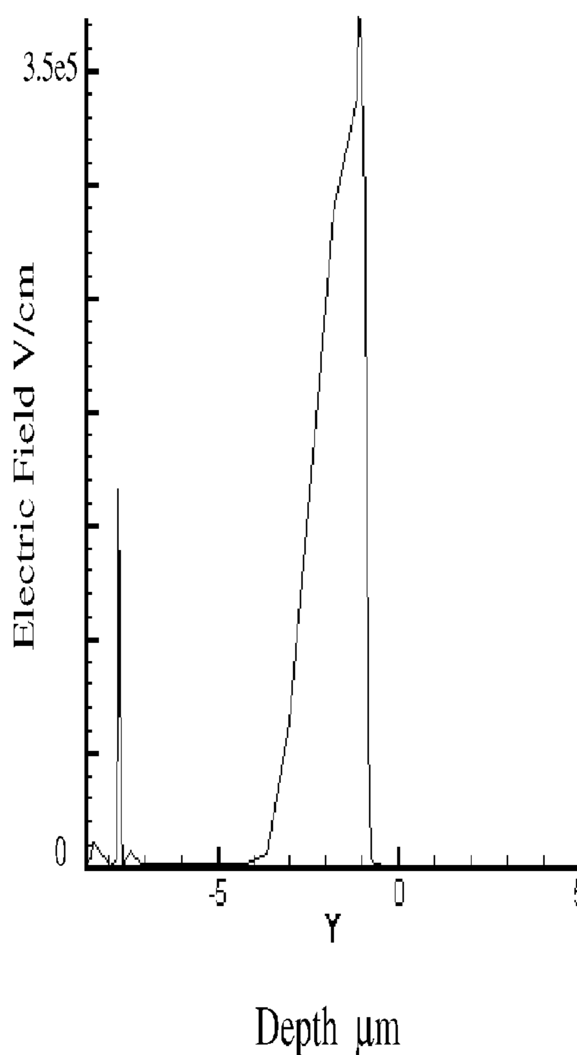
Electric Field vs. depth \mu\text{m}
