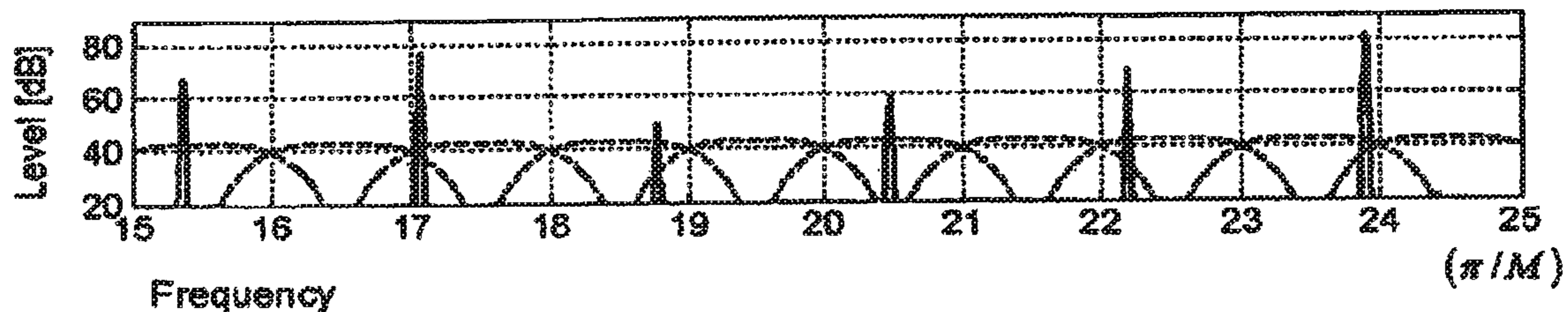
Spectral envelope adjustment using gain grouping in a real valued filterbank
