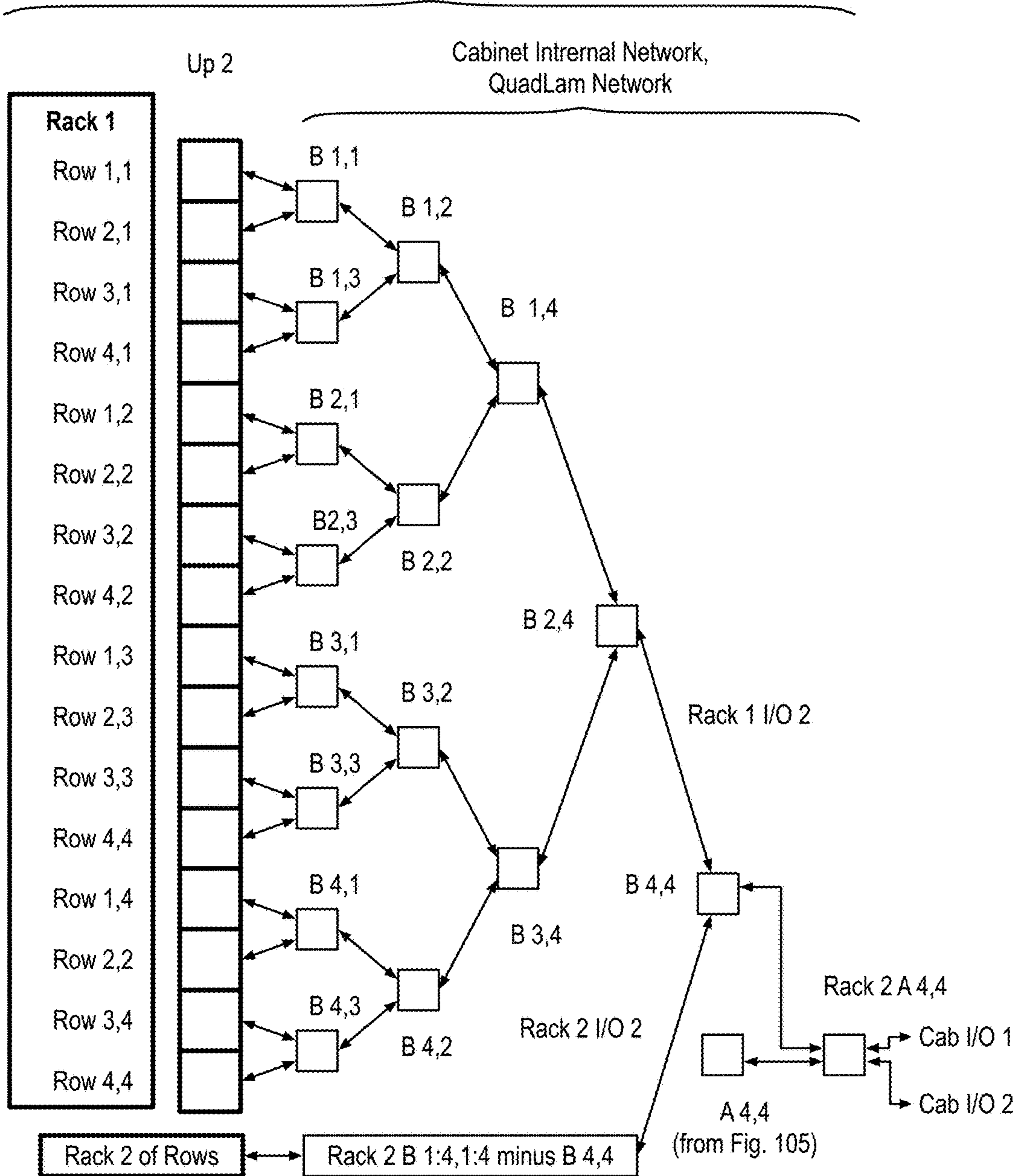
Rows and Racks of a Cabinet
