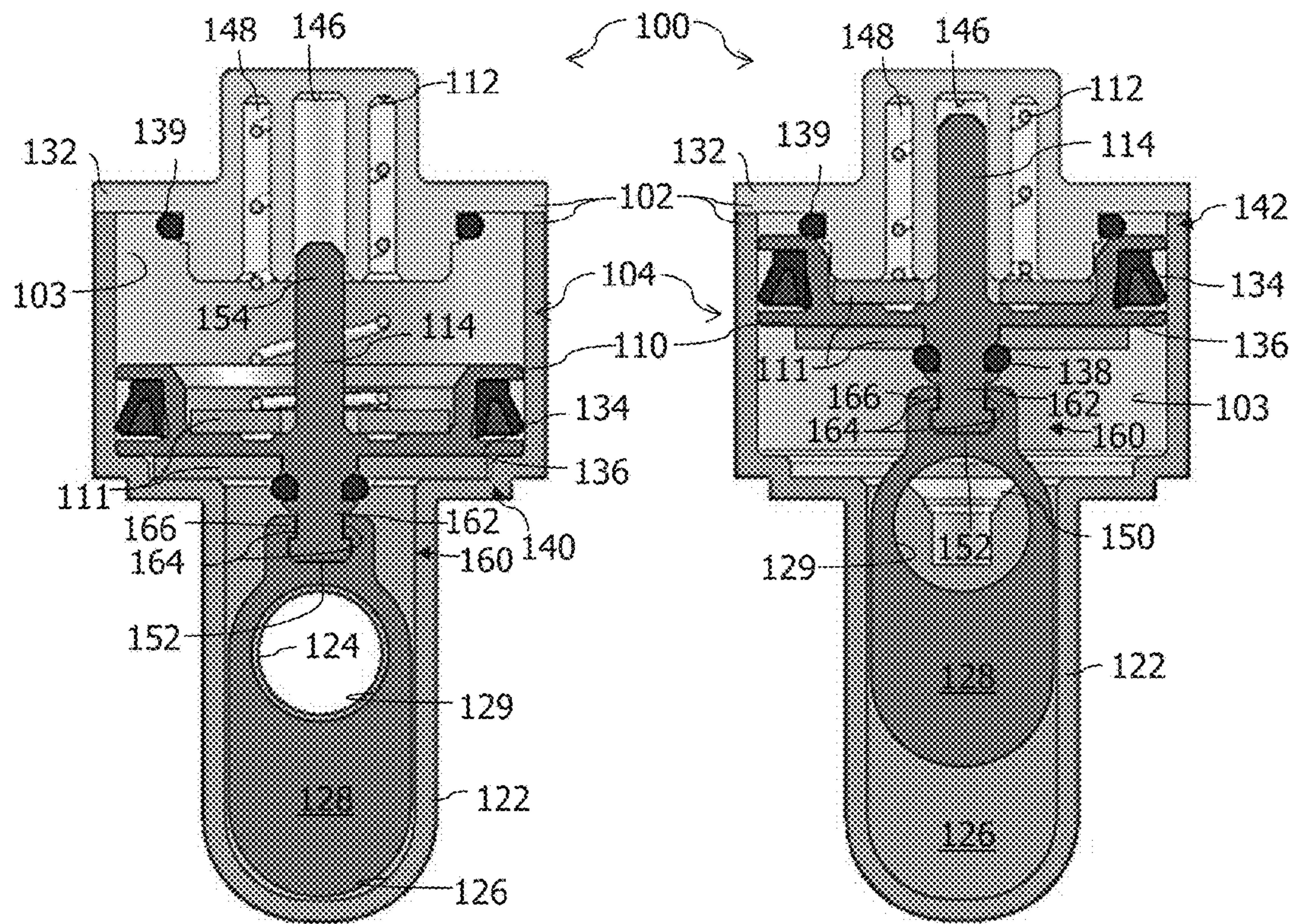
FIG. 3 (PRIOR ART)
