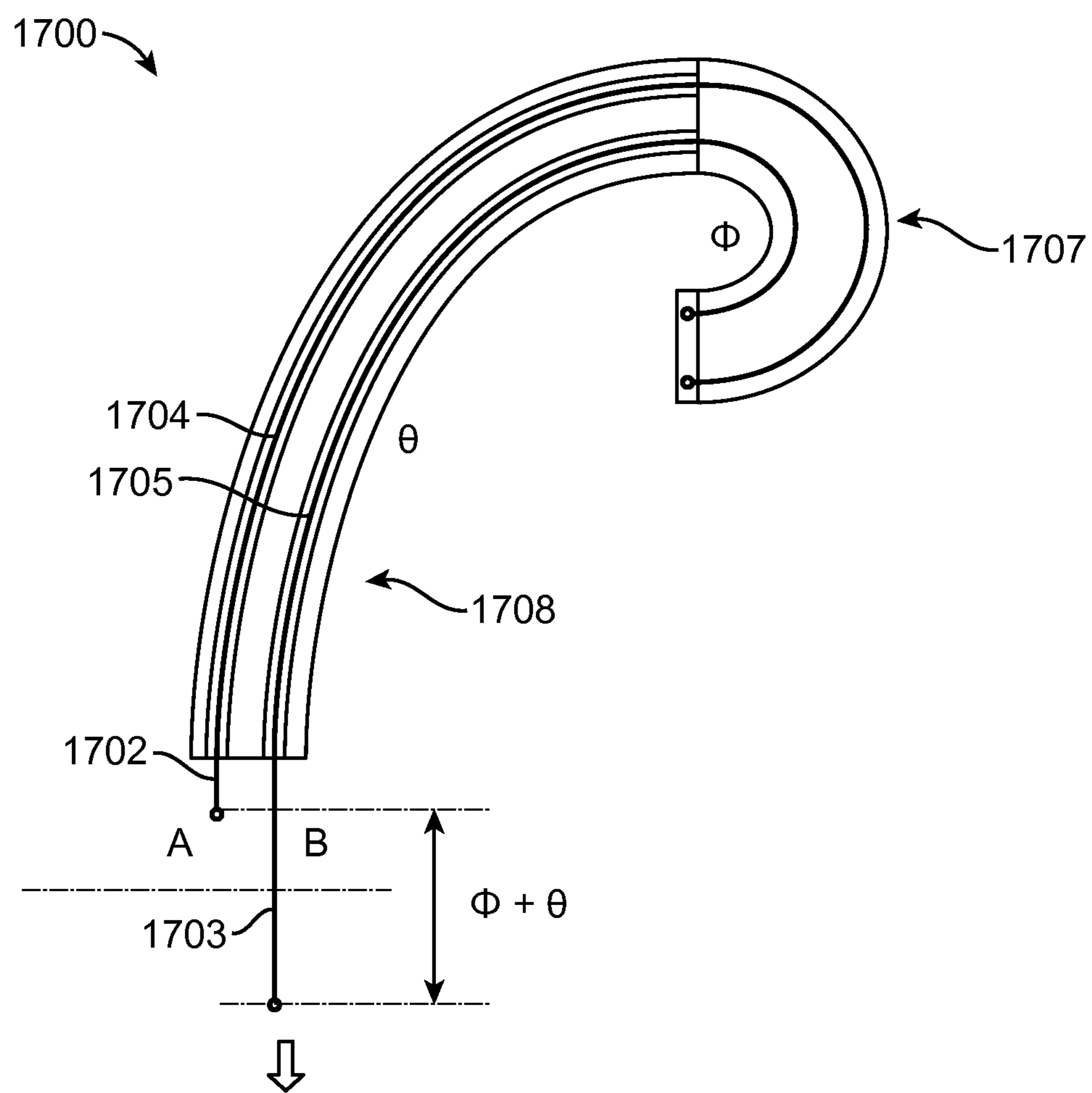
FIG. 17C (PRIOR ART)
