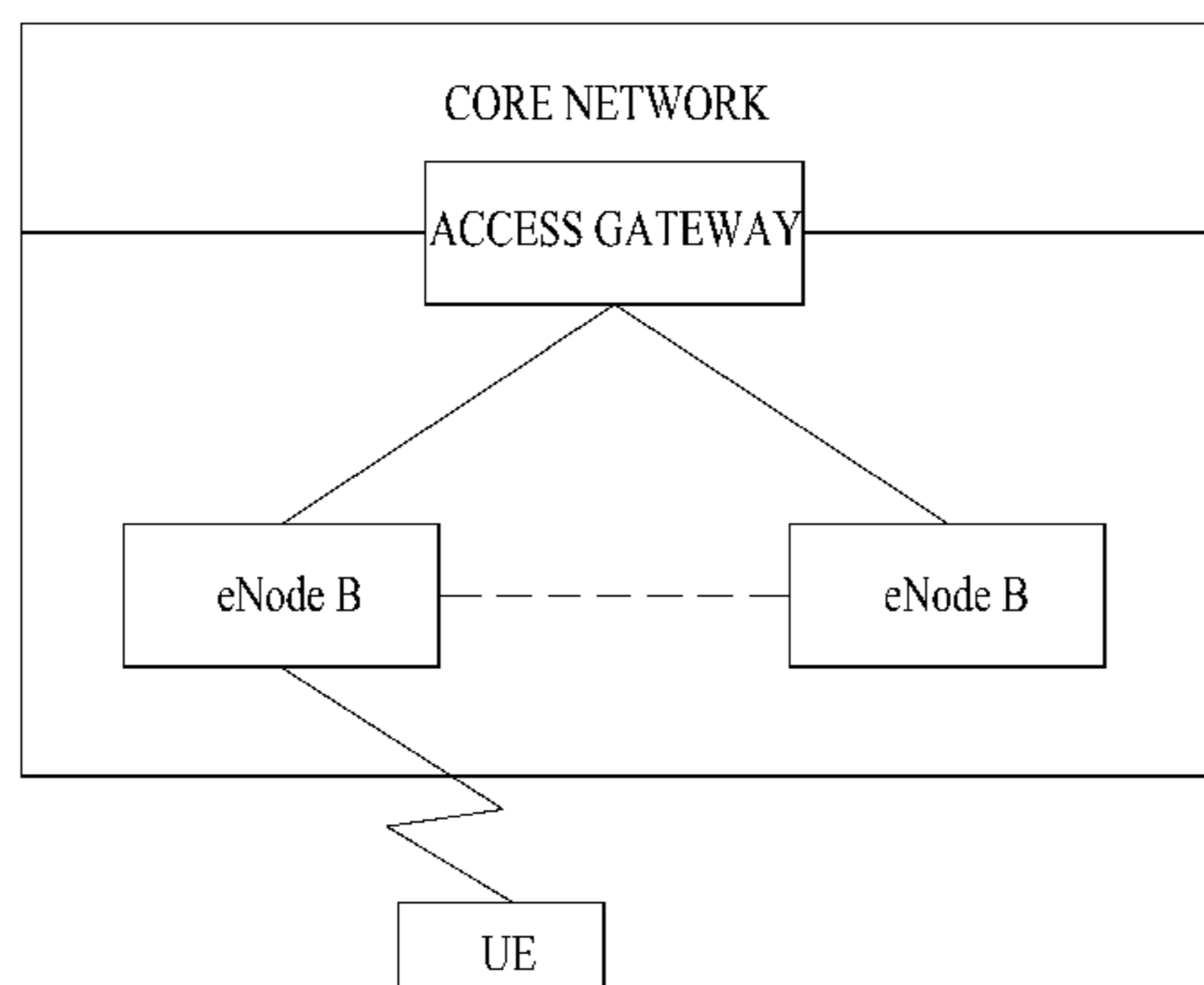
E-UMTS
