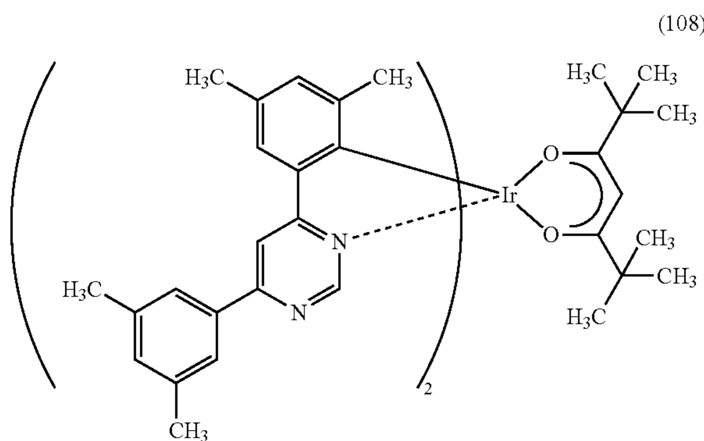
[Ir(dmdppm) 2 (dpm)]
