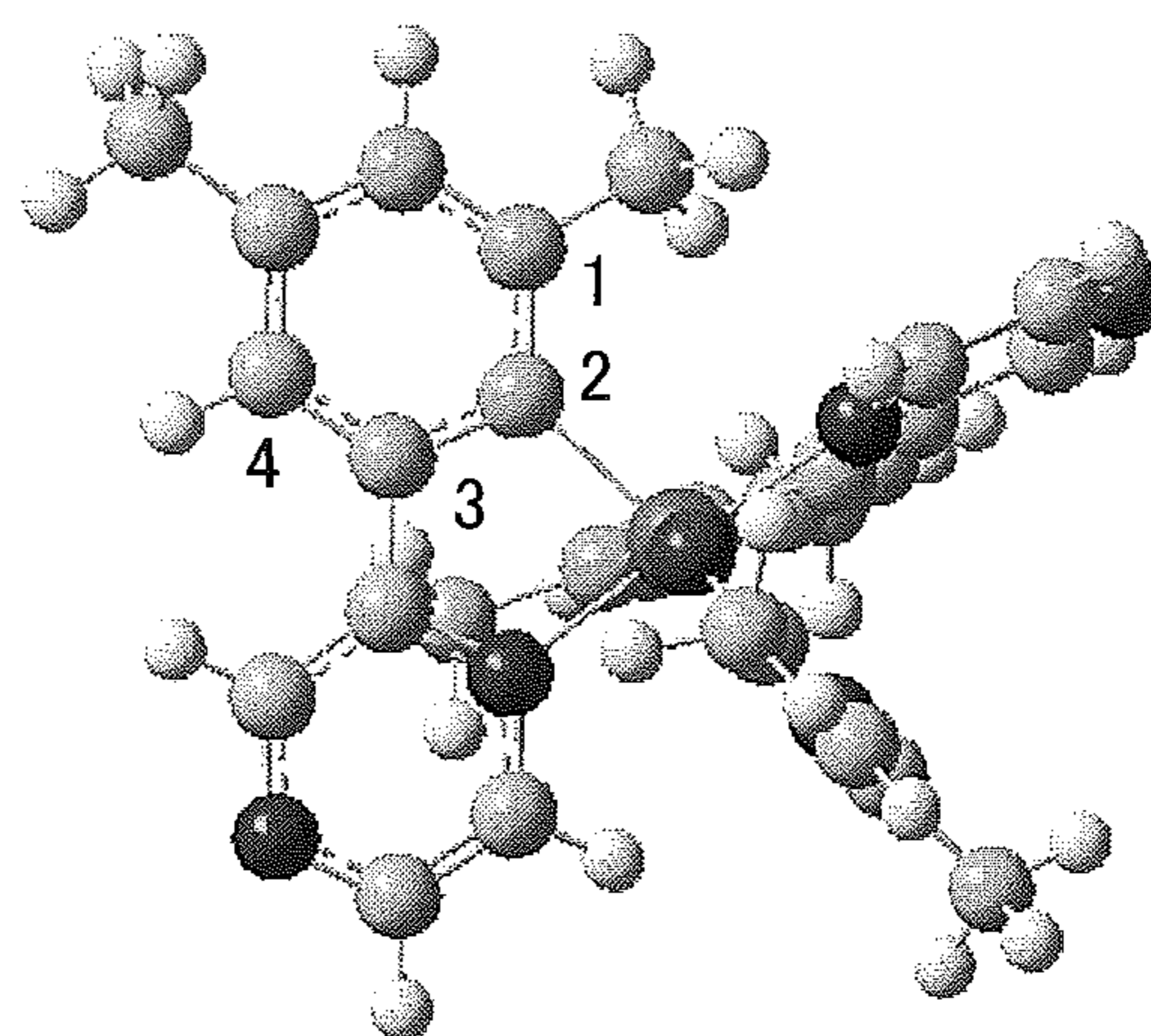
[\text{Ir}(\text{dmppr})_2(\text{acac})]
