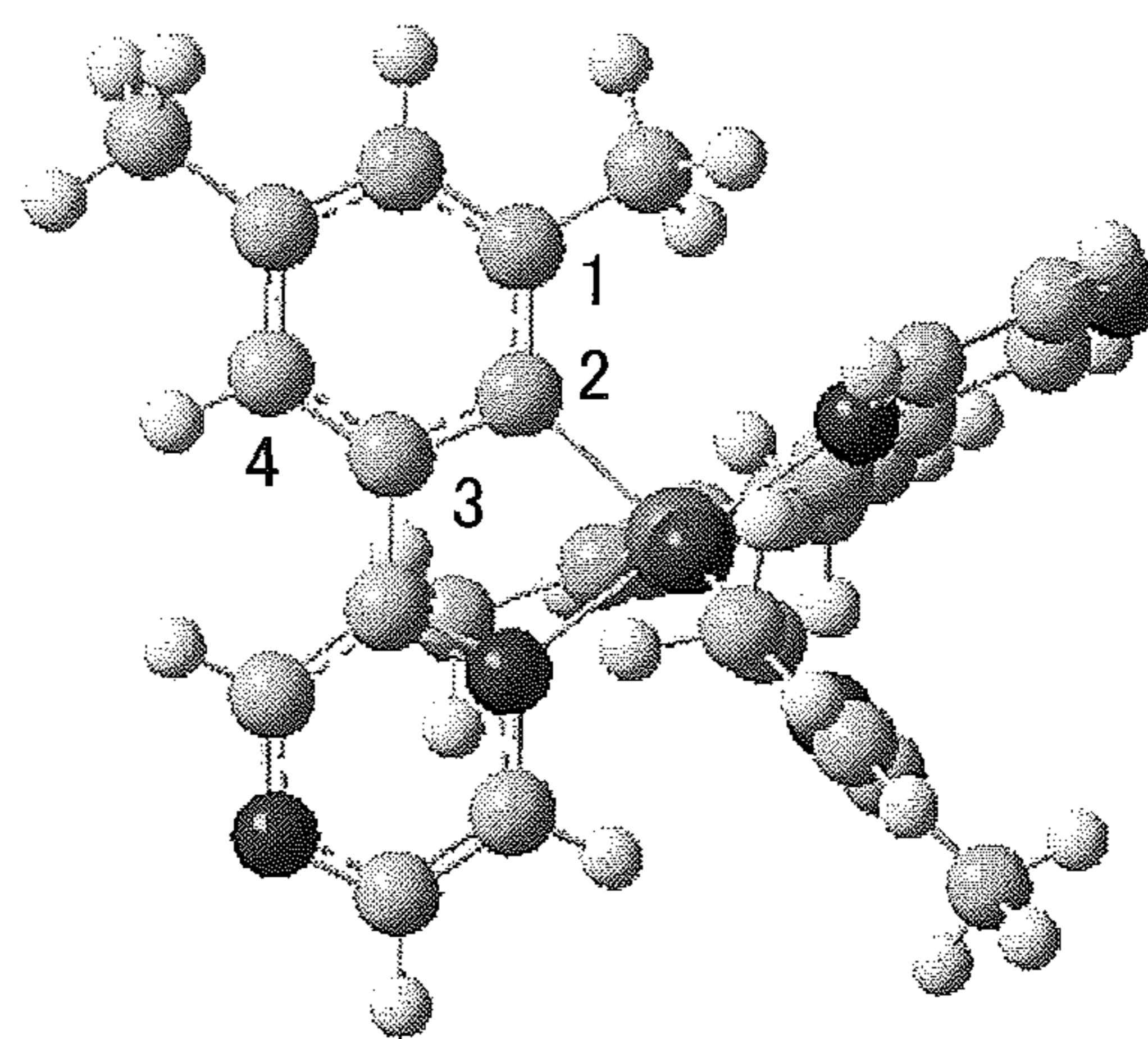
[\text{Ir}(\text{dmppr})_2(\text{acac})]
