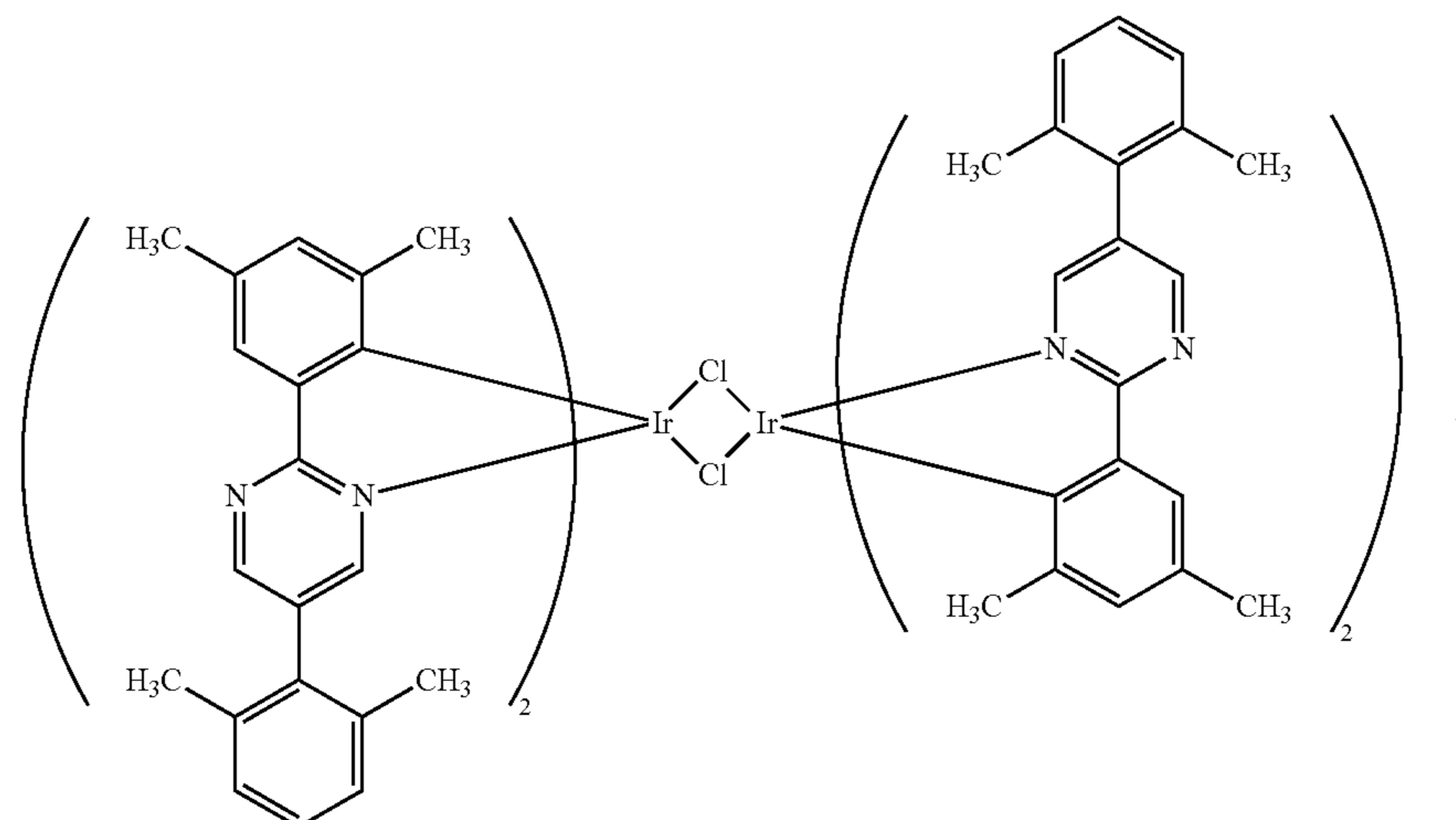
[Ir(dmppmm2-dmp) 2 Cl] 2
