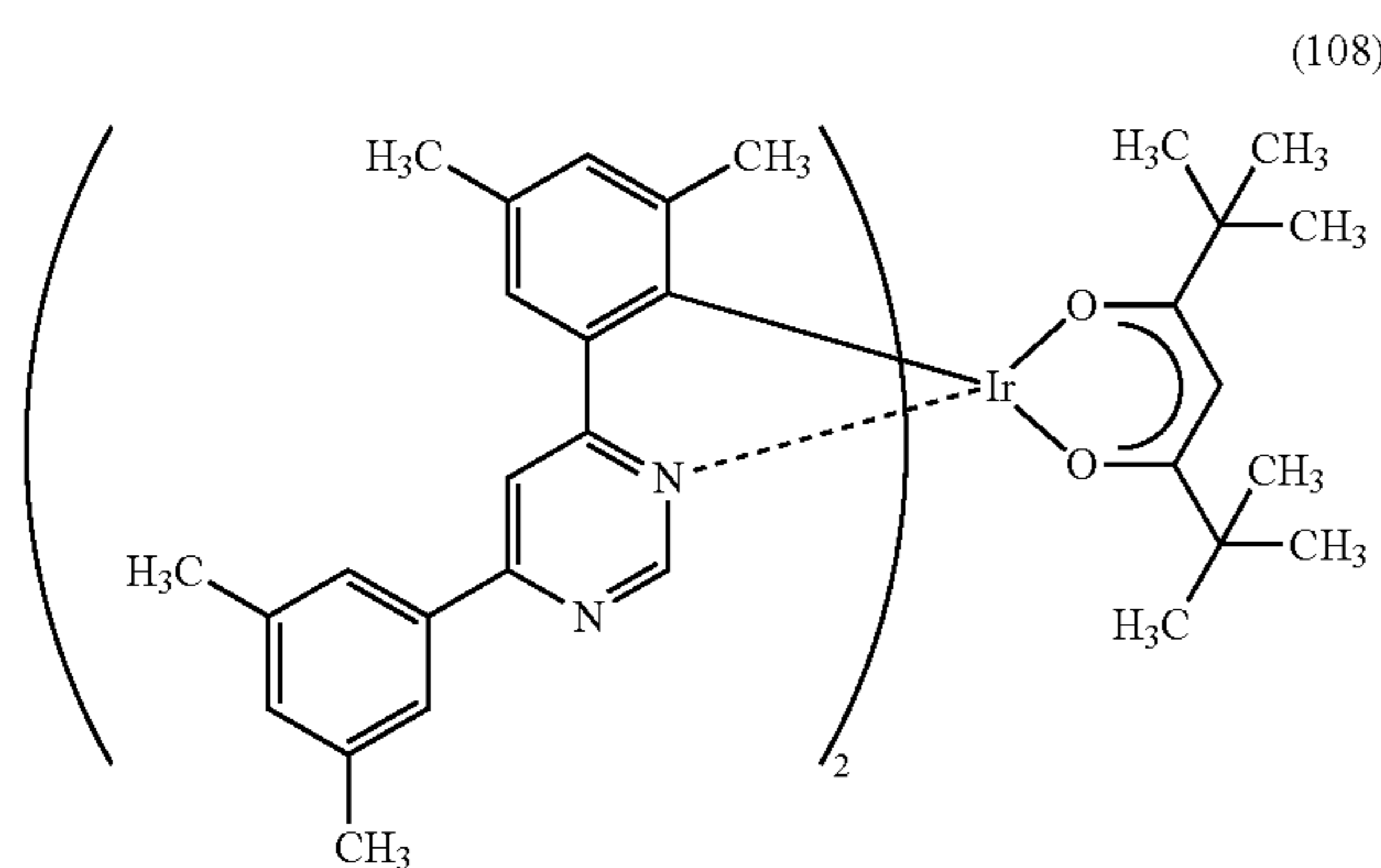
[Ir(dmdppm) 2 (dpm)]
