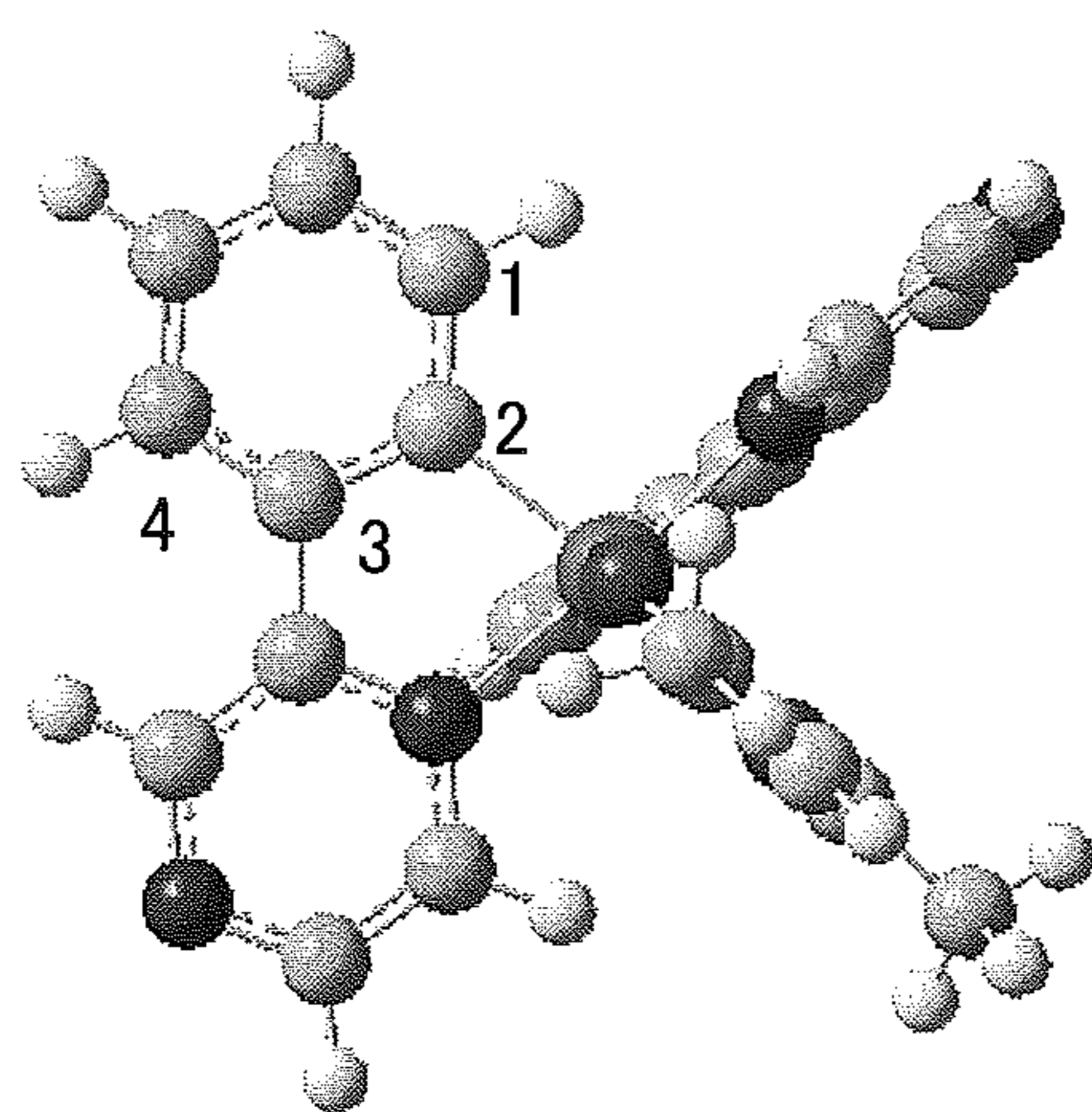
[\text{Ir}(\text{ppr})_2(\text{acac})]
