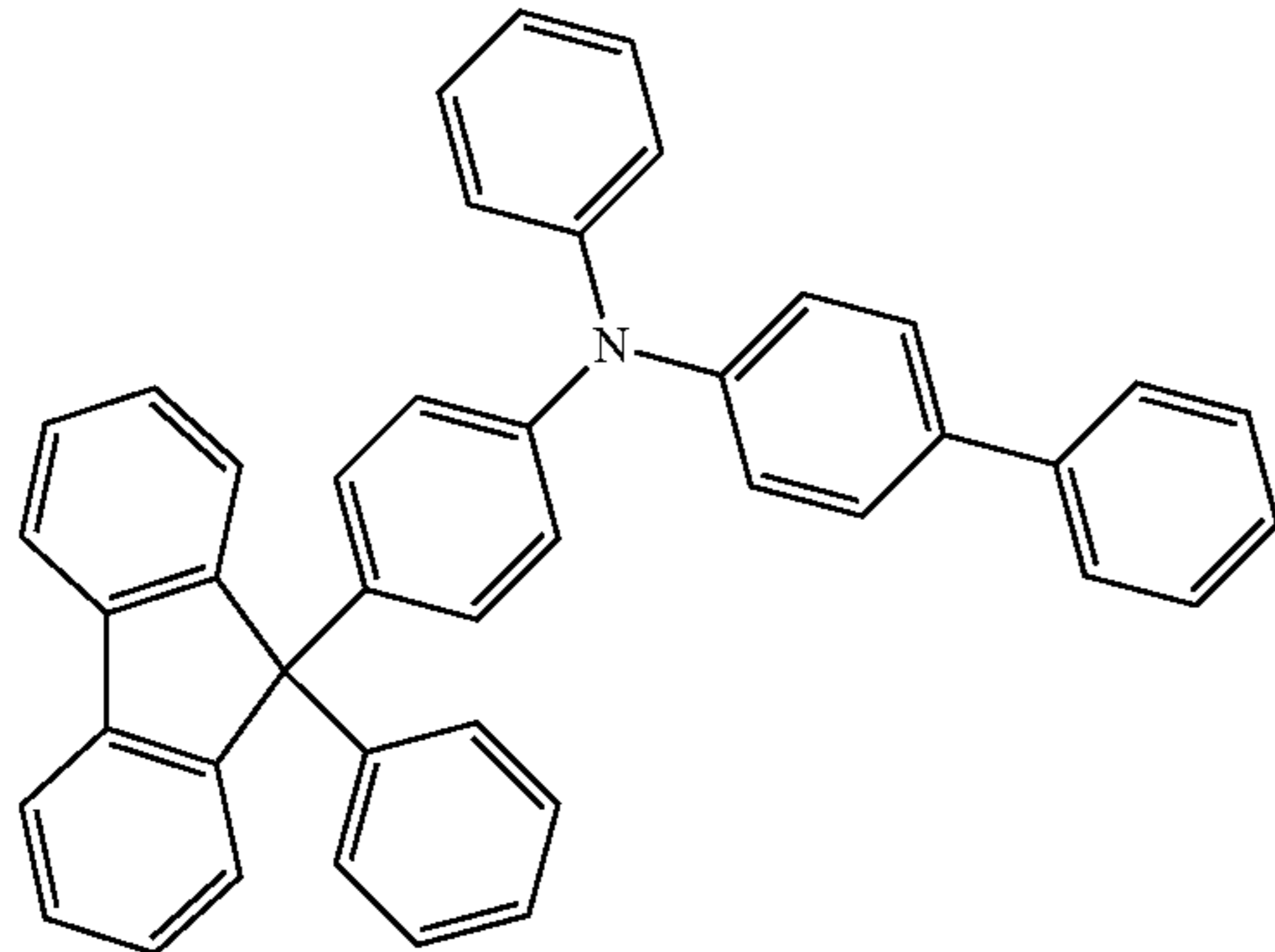
BPAFLP
