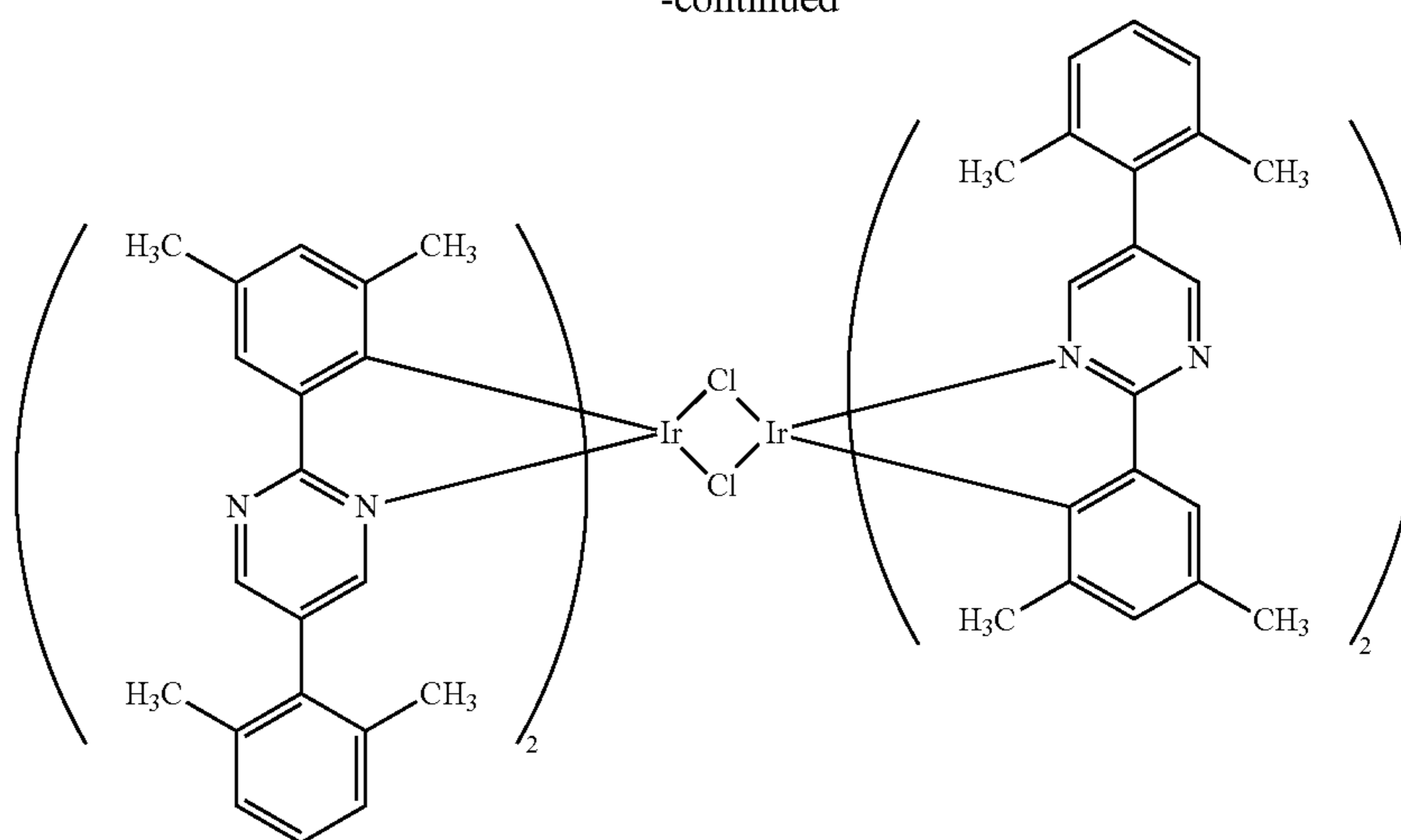
[Ir(dmppm2-dmp) 2 Cl] 2
