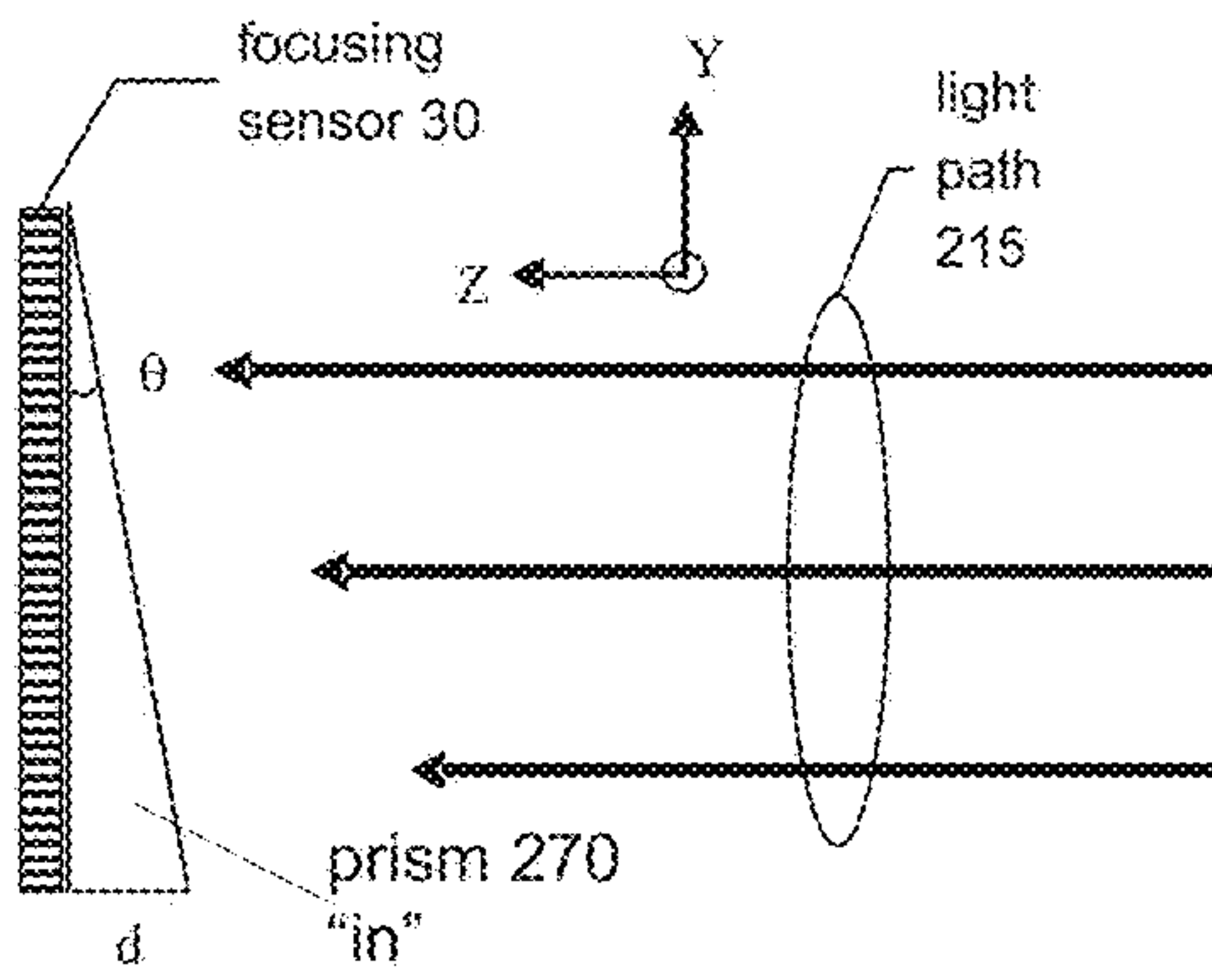
FIG. 7A focusing during stage retrace
