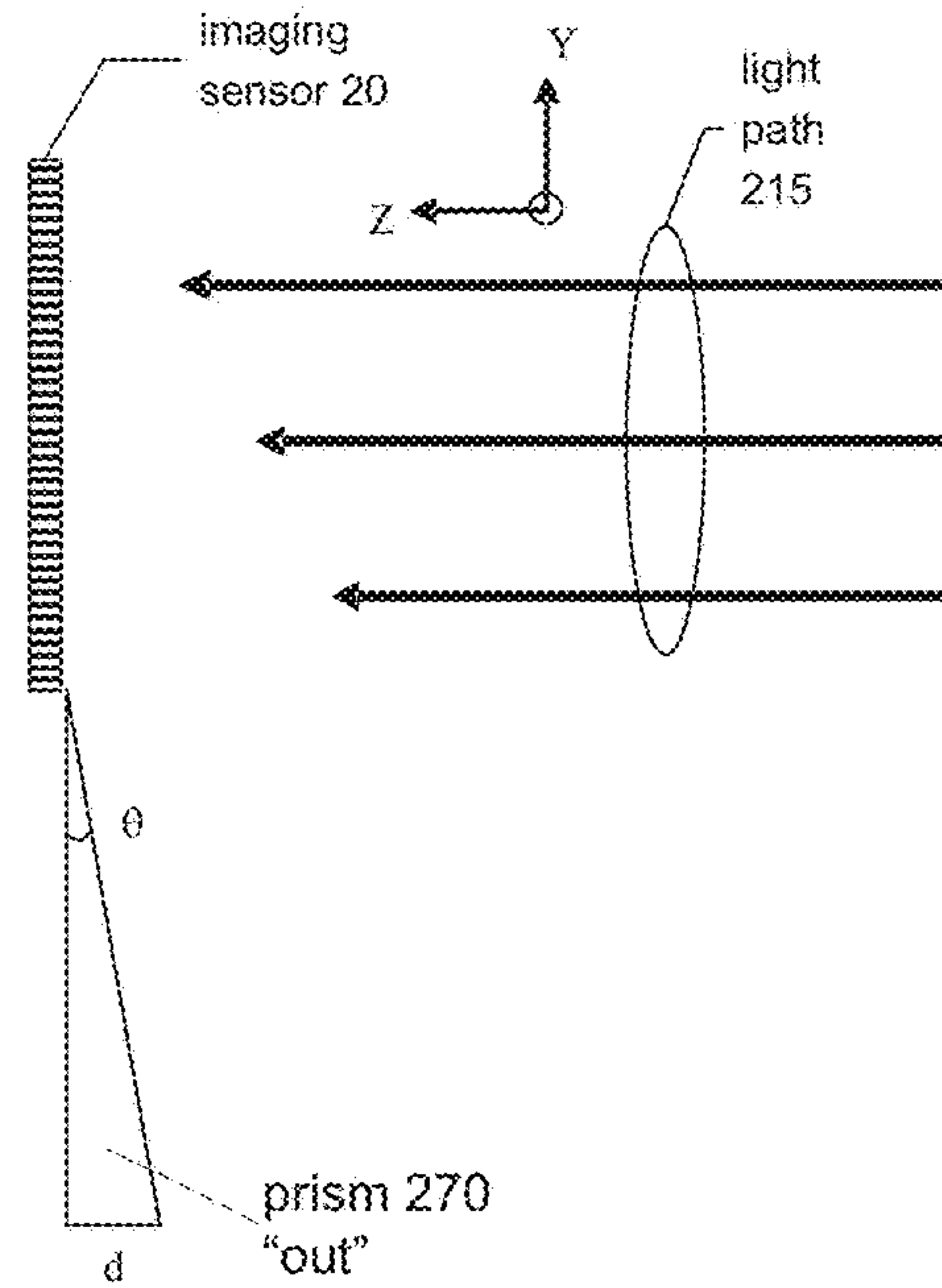
FIG. 7B imaging during scan
