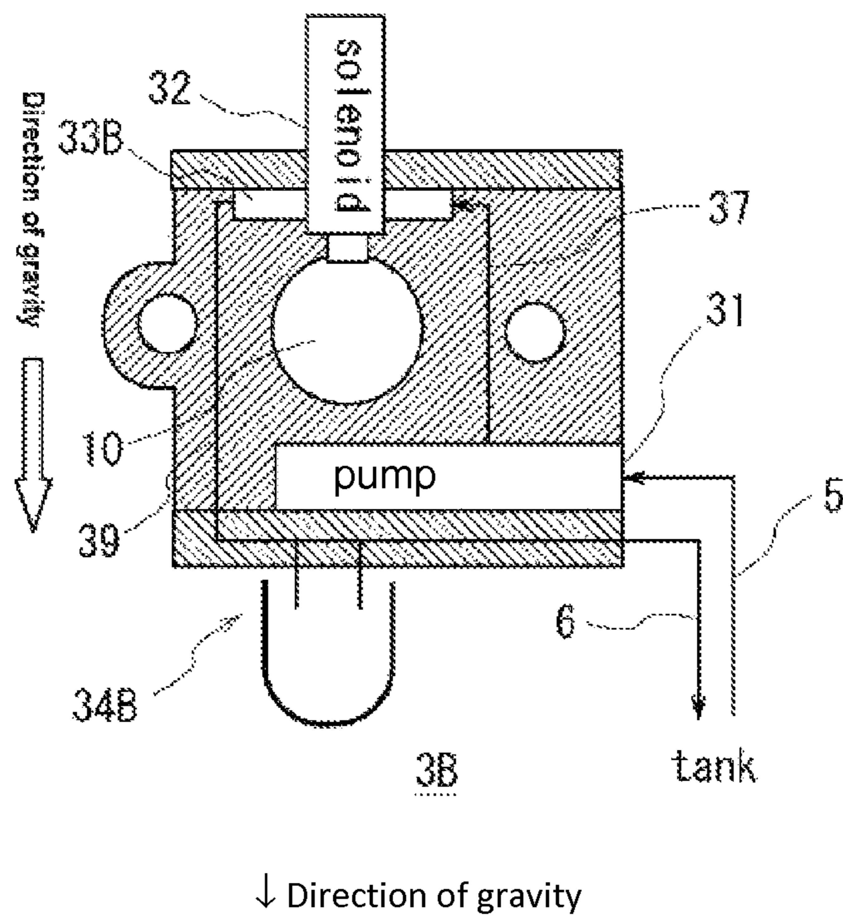
Fig. 3 (Prior Art)
