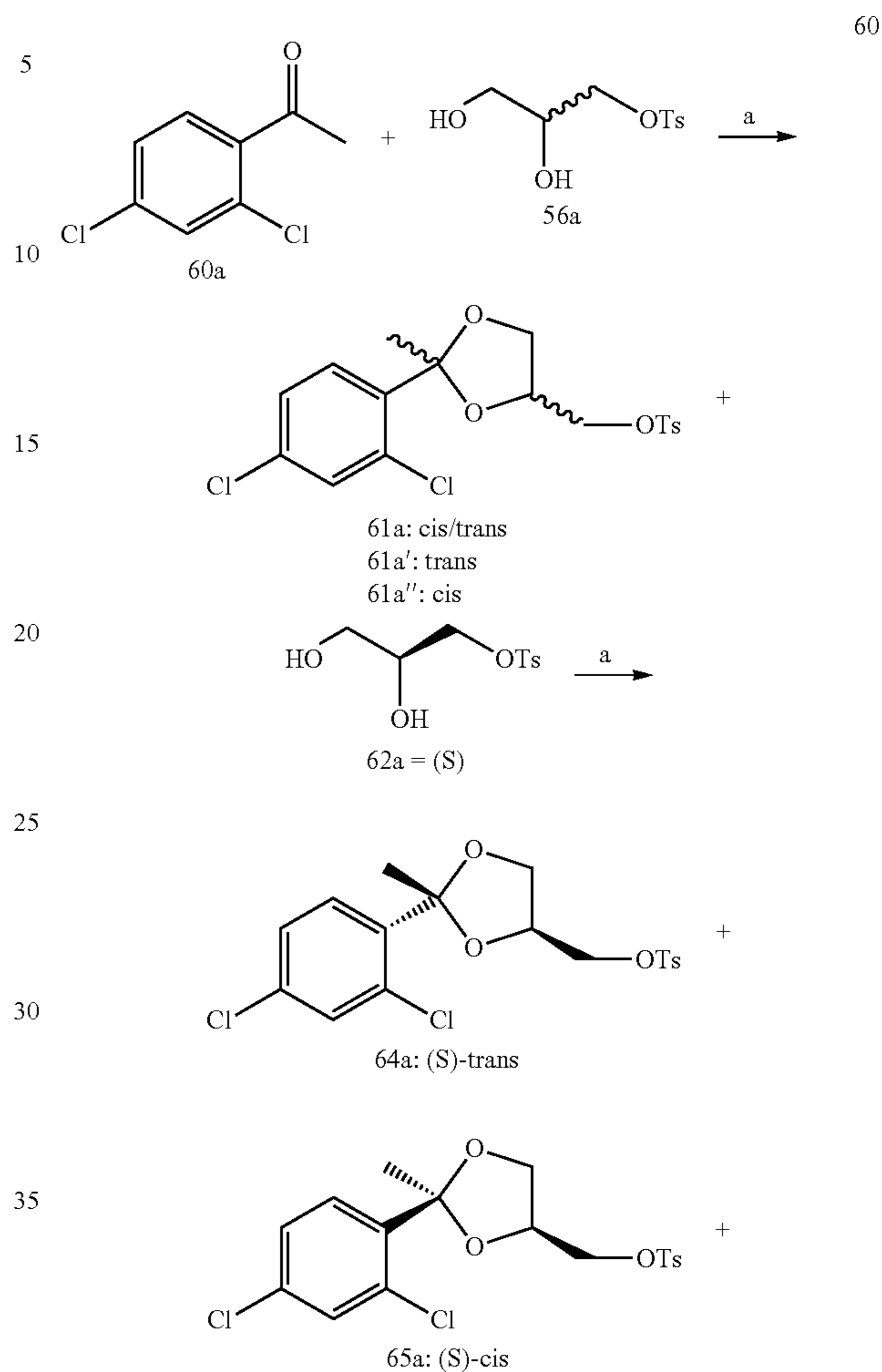
Scheme 4a. Synthesis of des-triazole dioxolane region intermediates. a
