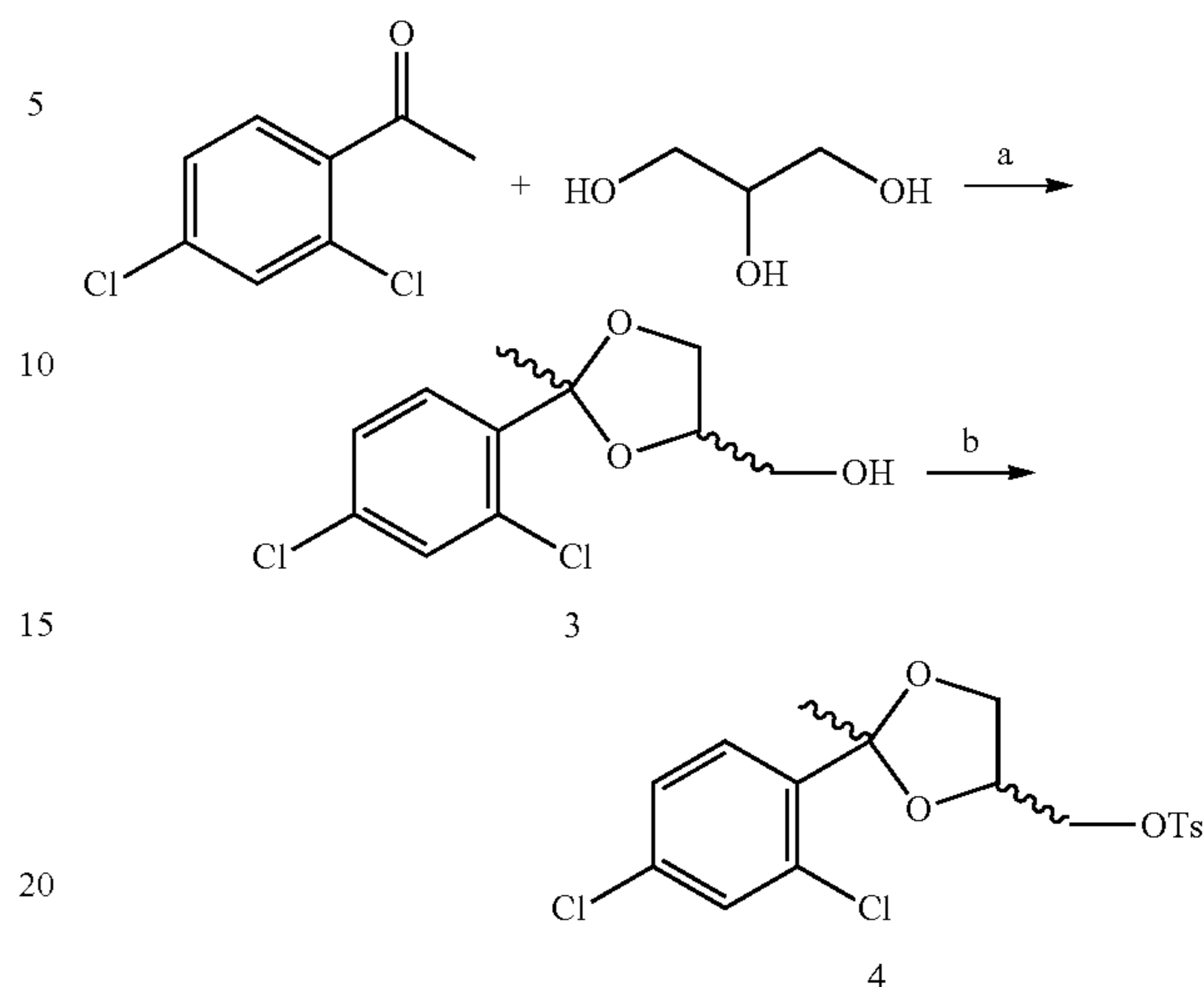
Scheme 1. Preparation of key des-triazole intermediate. a
