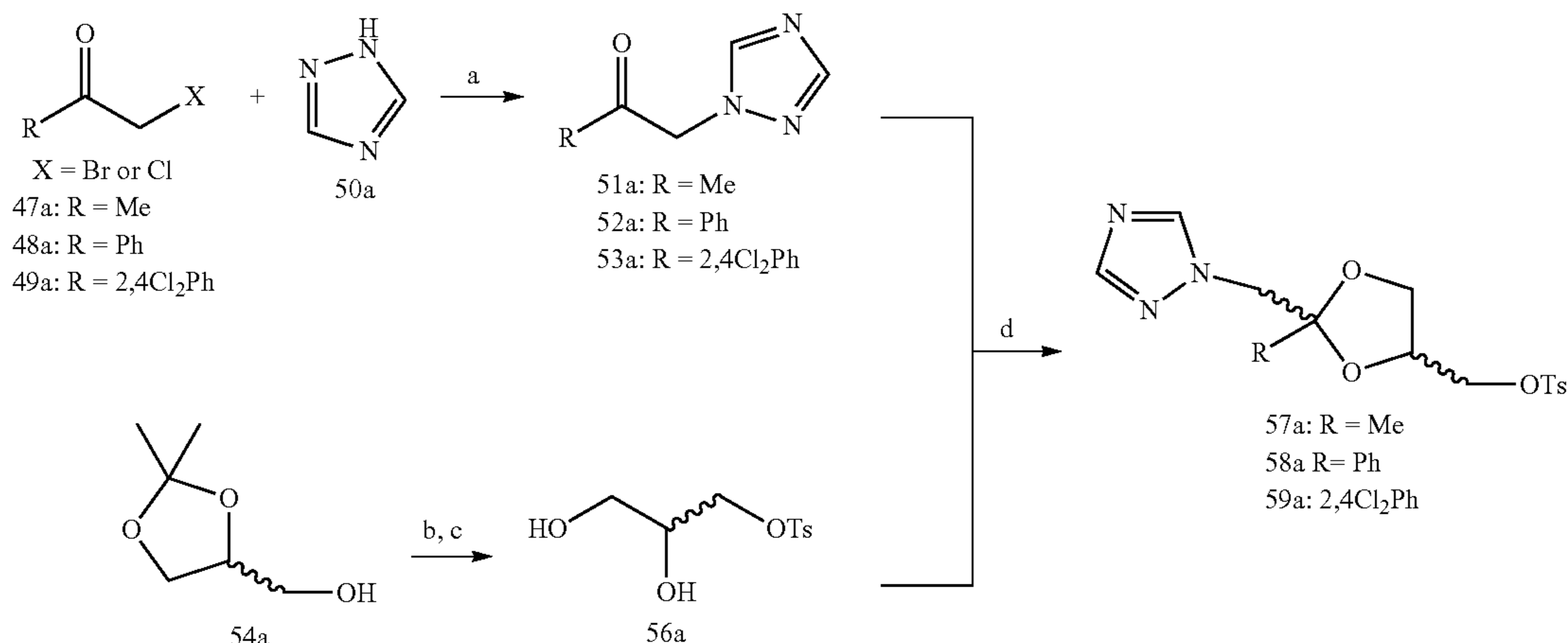
Scheme 3a. Synthesis of triazole-containing dioxane region intermediates. a
