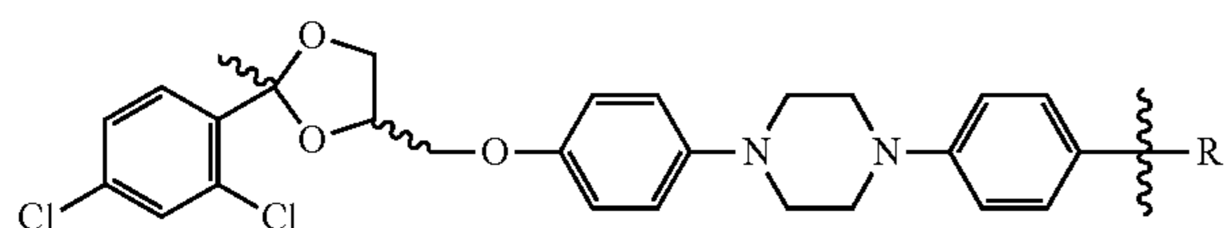
Scheme 8: Side chain reaction analogues
