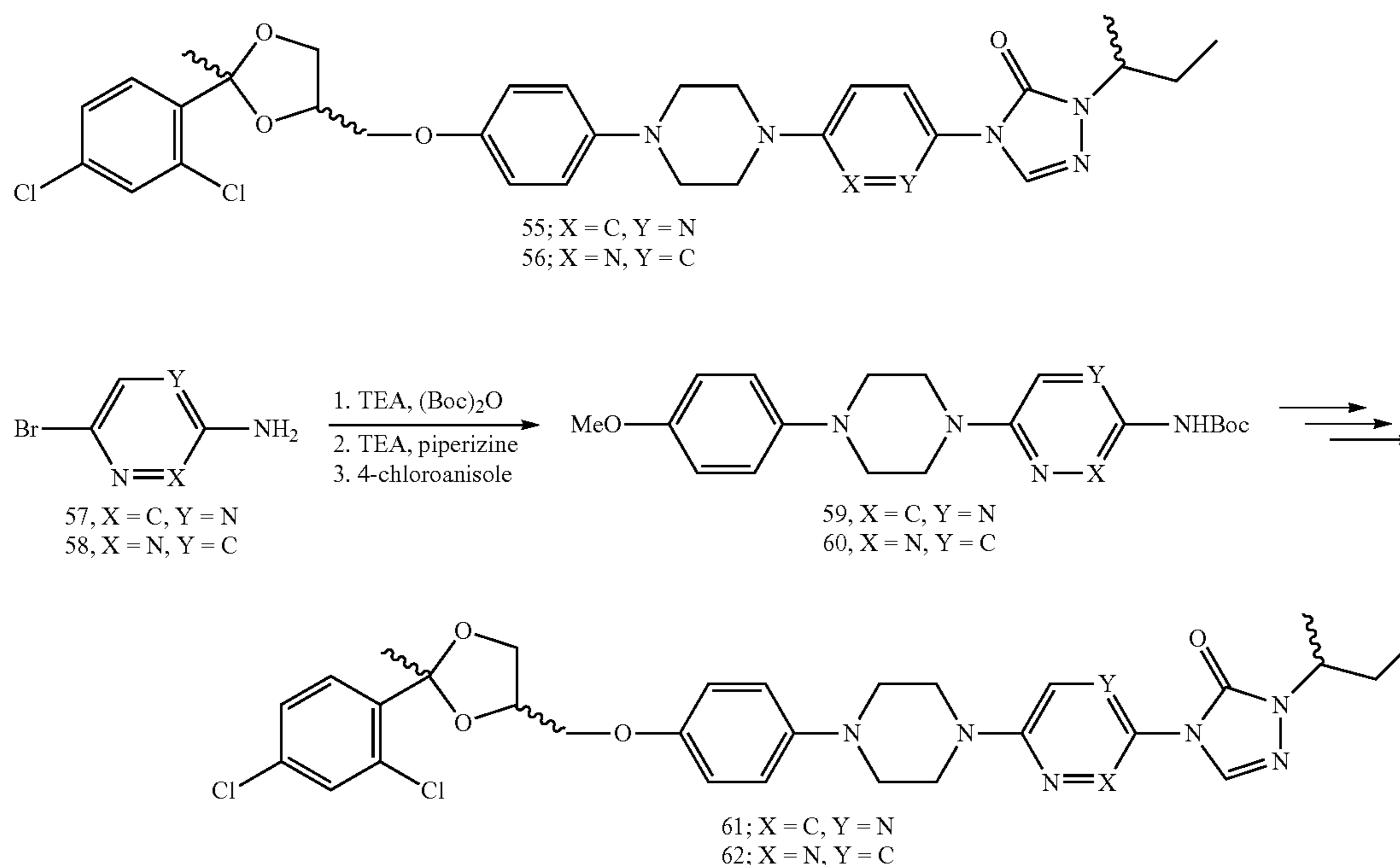
Scheme 9. ITZ analogues incorporating heterocycles adjacent to the des-triazole region.
