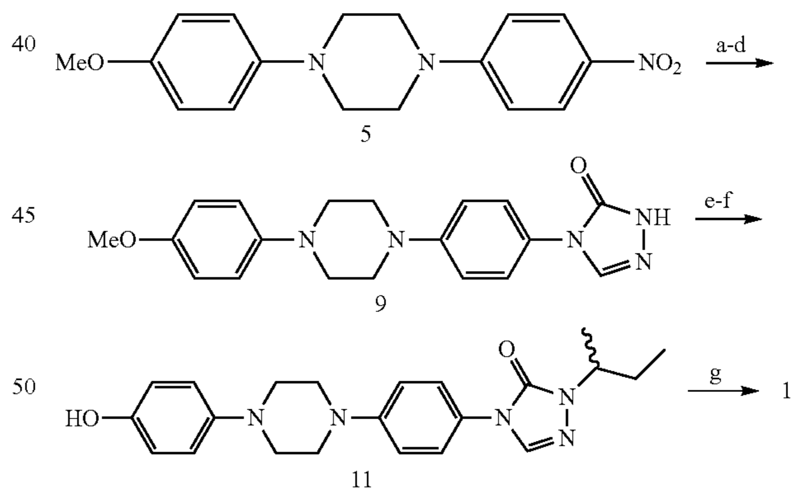
Scheme 2. Preparation of des-triazole ITZ analogue 1. a
