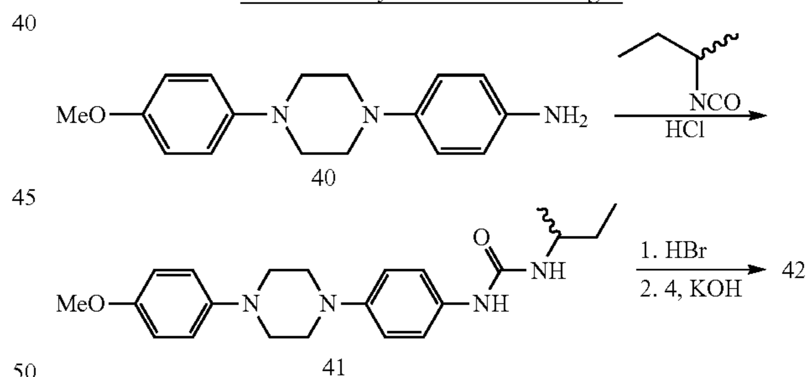
Scheme 6. Acyclic triazolone analogue
