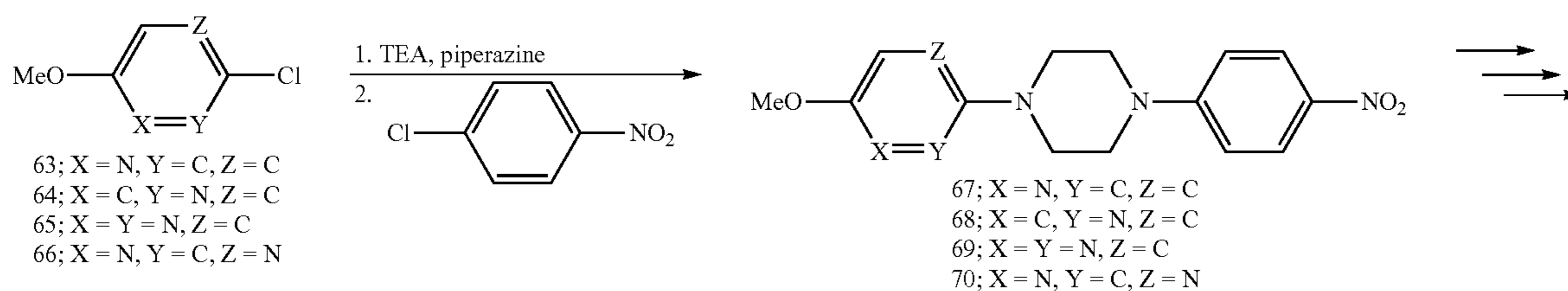
Scheme 10. ITZ analogues incorporating heterocycles adjacent to the triazole region.
