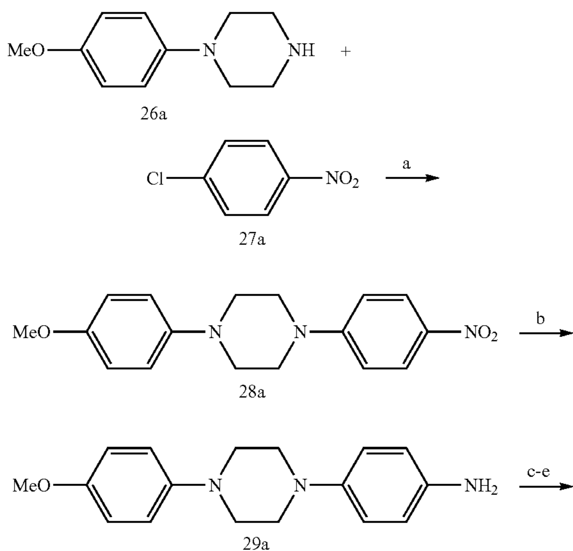
Scheme 1a. Synthesis of linker region intermediate. a
