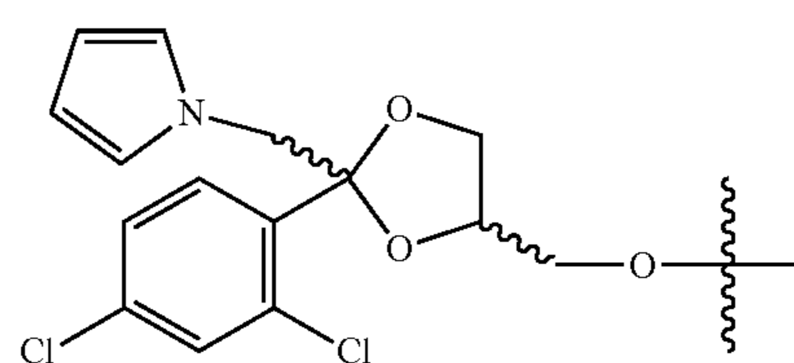
Scheme 11: ITS analogues with triazole mimics
