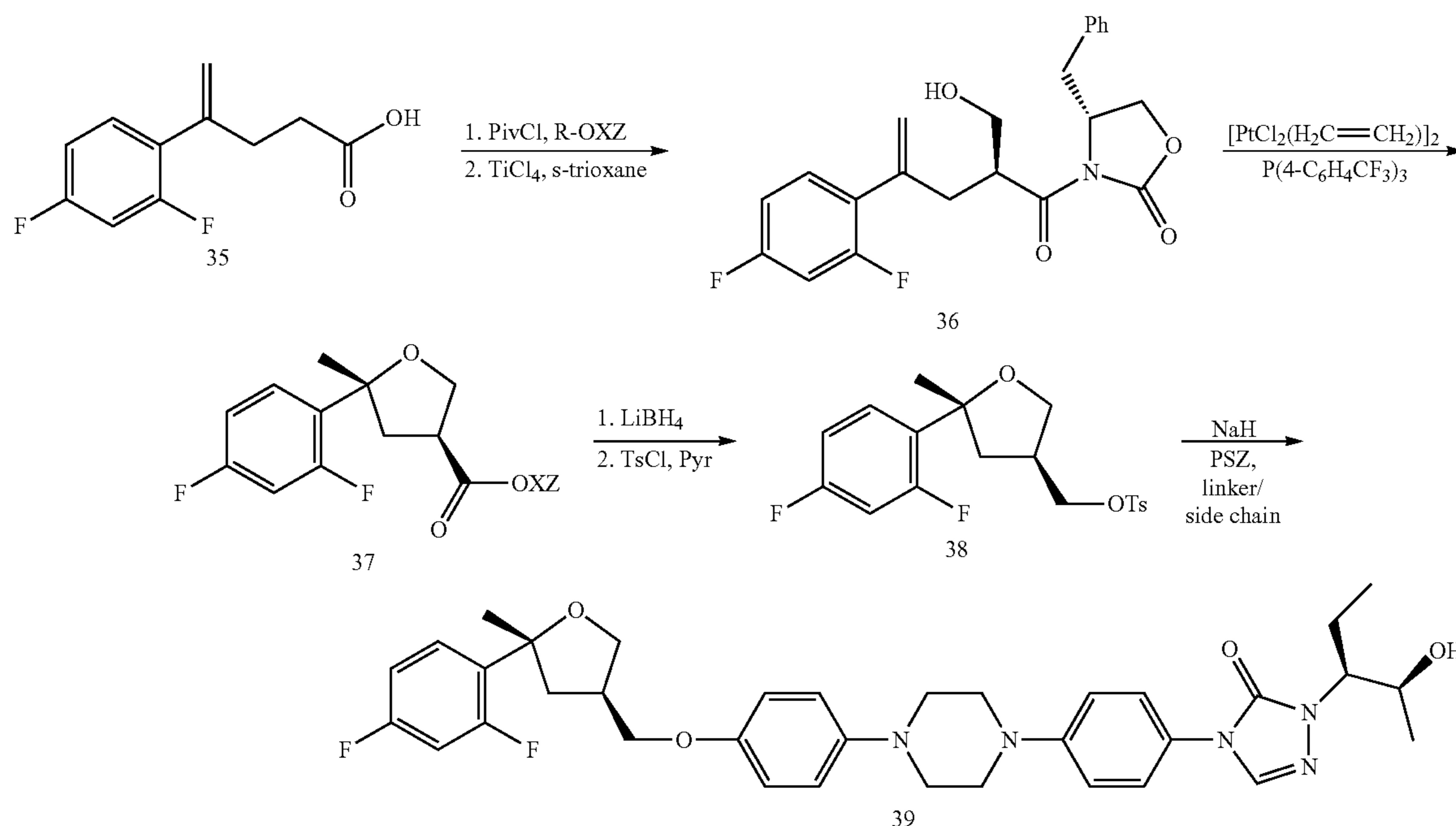
Scheme 5. Synthesis of des-triazole PSZ analogue 39
