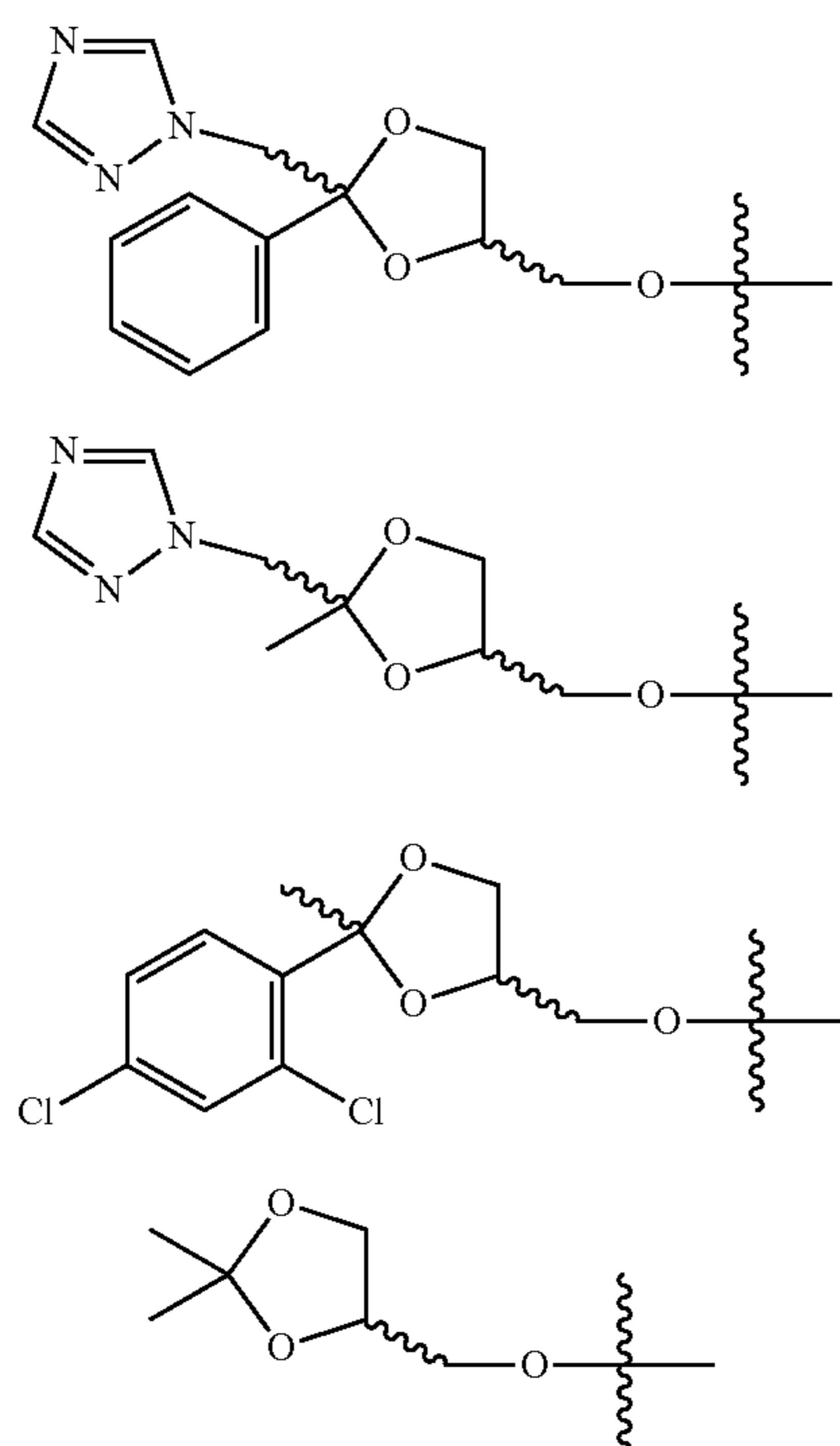
Scheme 14. Truncated triazole region ITZ analogues
