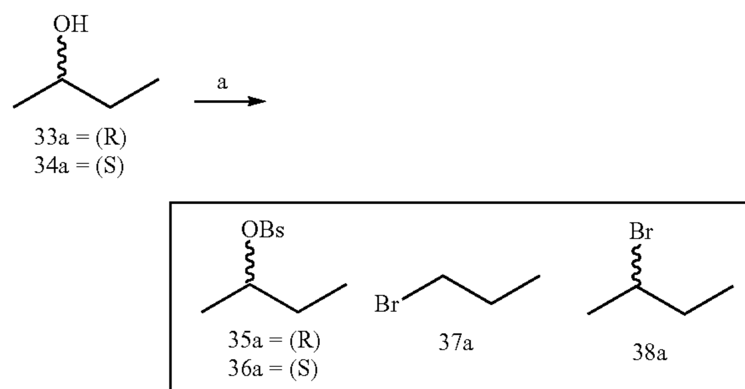
Scheme 2a. Synthesis of linker/triazolone/side chain intermediates. a
