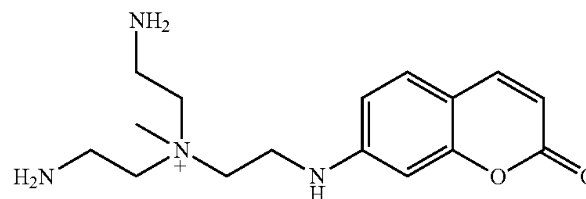
Formula V
